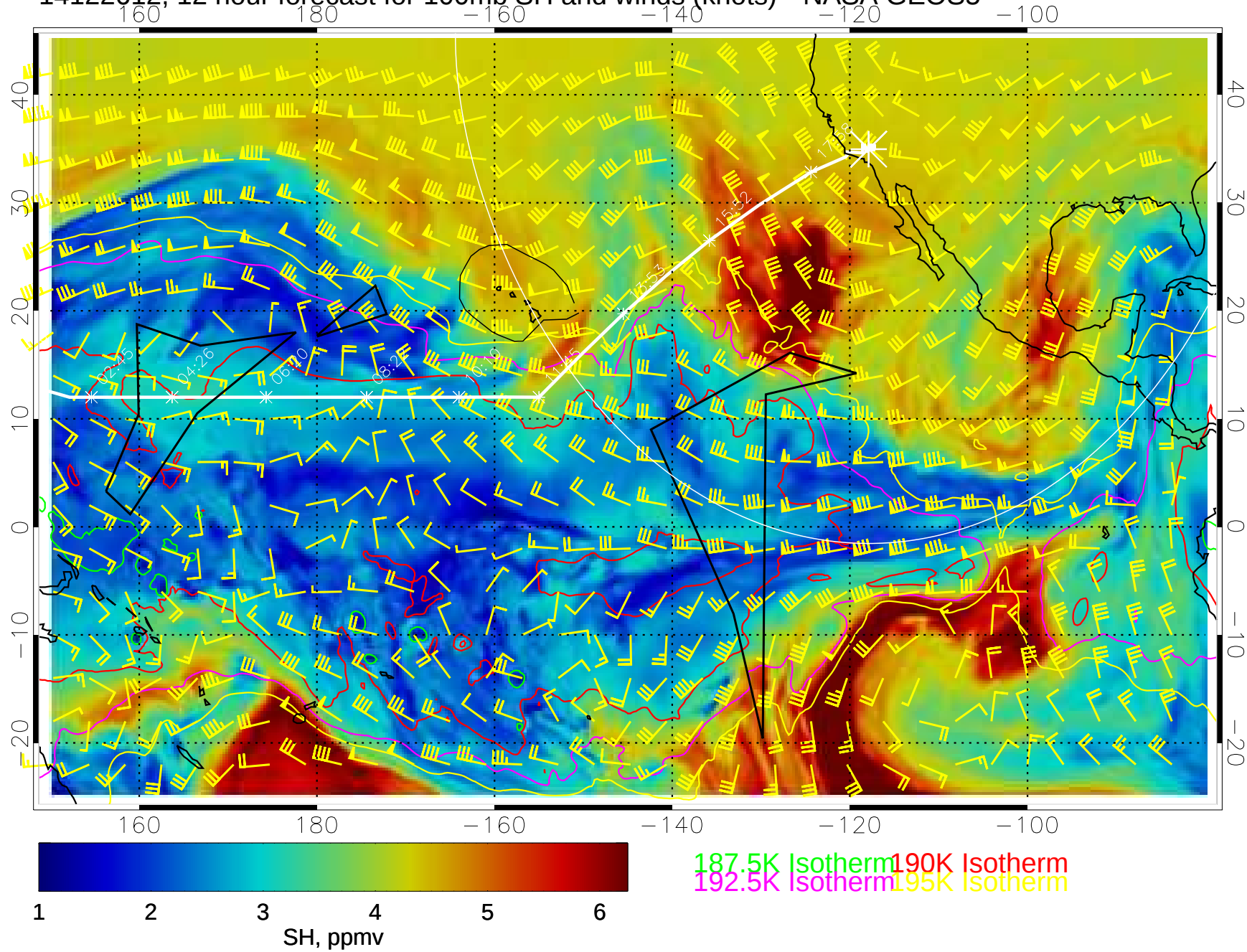
14122612, 12 hour forecast for 100mb SH and winds (knots)-- NASA GEOS5
