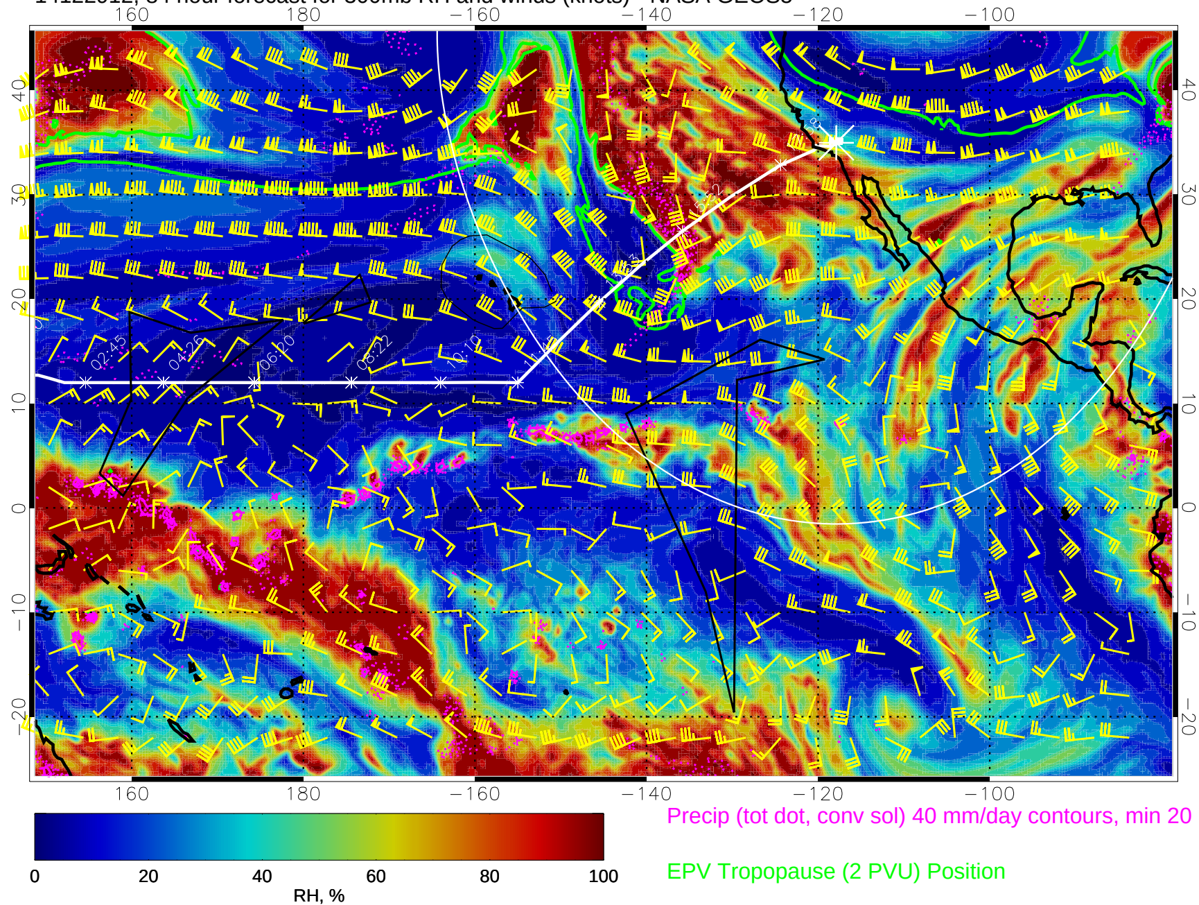
14122912, 84 hour forecast for 300mb RH and winds (knots) - NASA GEOS5
