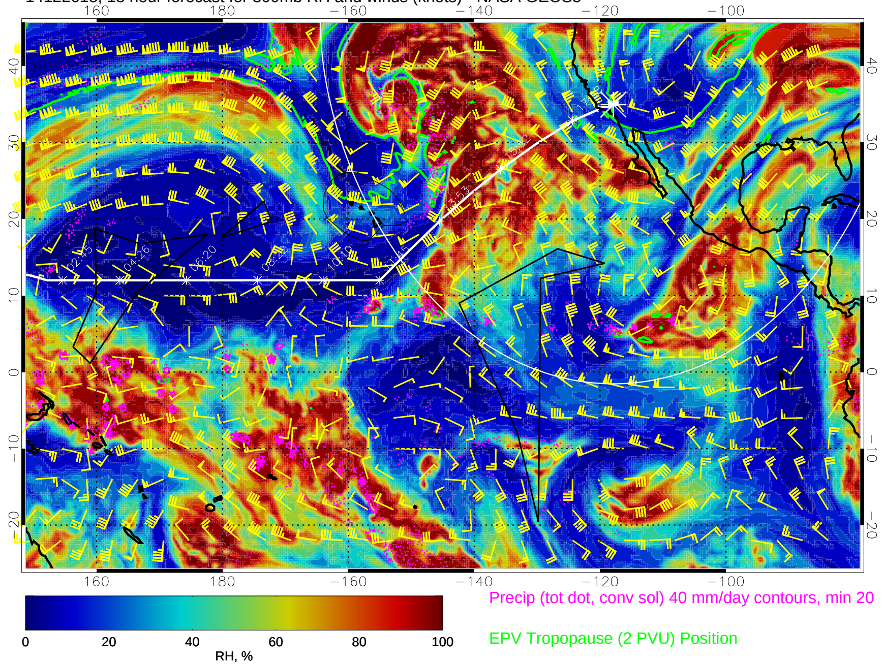
14122618, 18 hour forecast for 300mb RH and winds (knots) - NASA GEOS5
