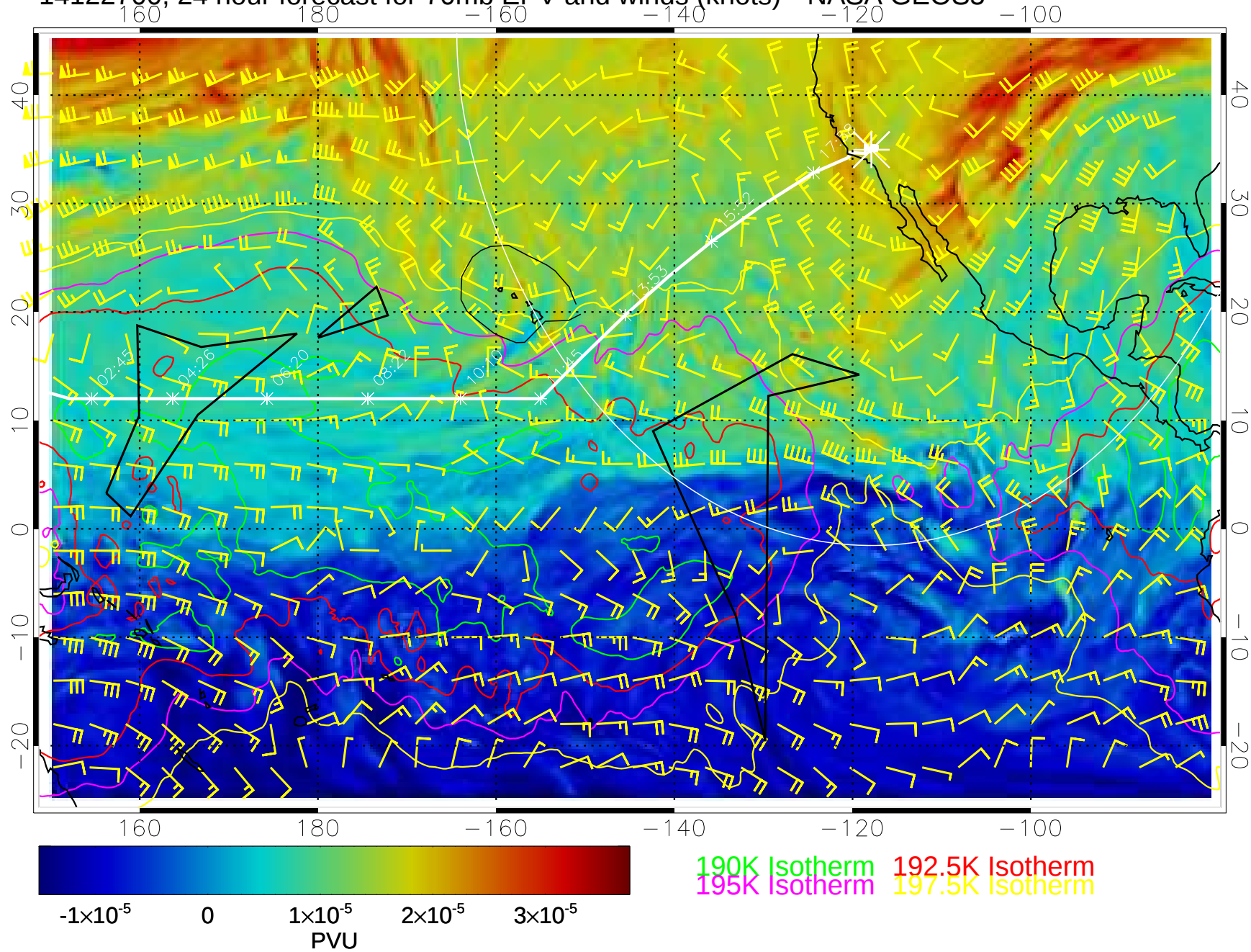
14122700, 24 hour forecast for 70mb EPV and winds (knots)-- NASA GEOS5
