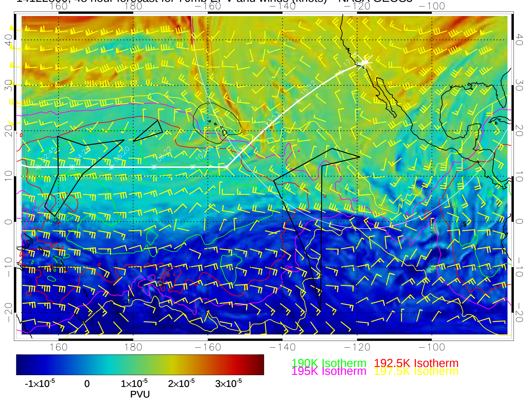
14122800, 48 hour forecast for 70mb EPV and winds (knots)-- NASA GEOS5
