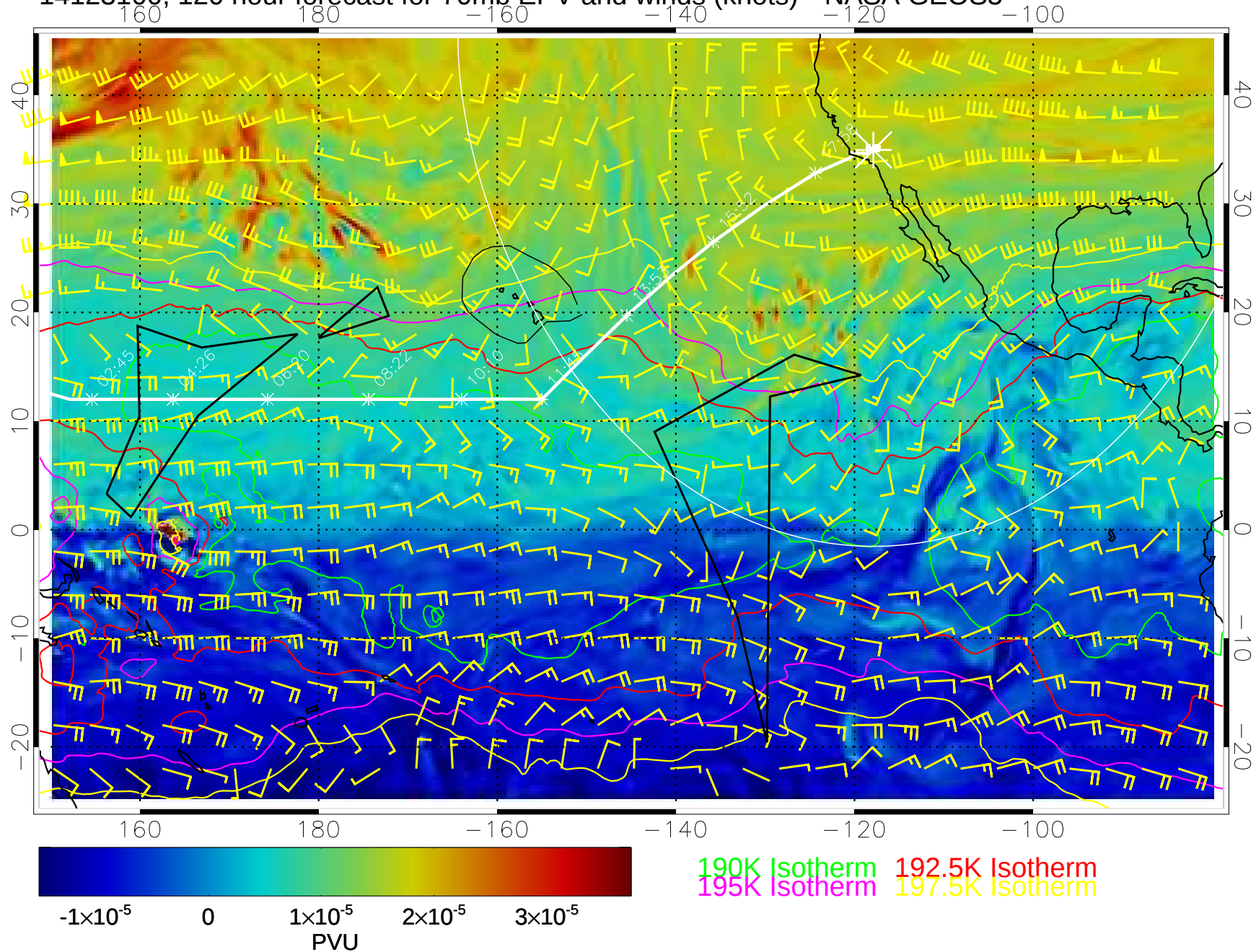
14123100, 120 hour forecast for 70mb EPV and winds (knots)-- NASA GEOS5
