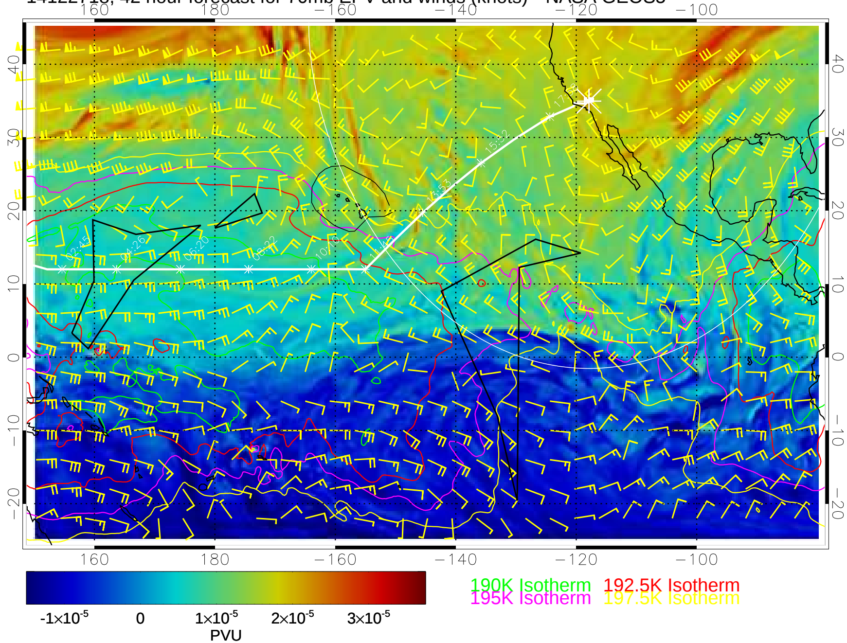
14122718, 42 hour forecast for 70mb EPV and winds (knots)-- NASA GEOS5
