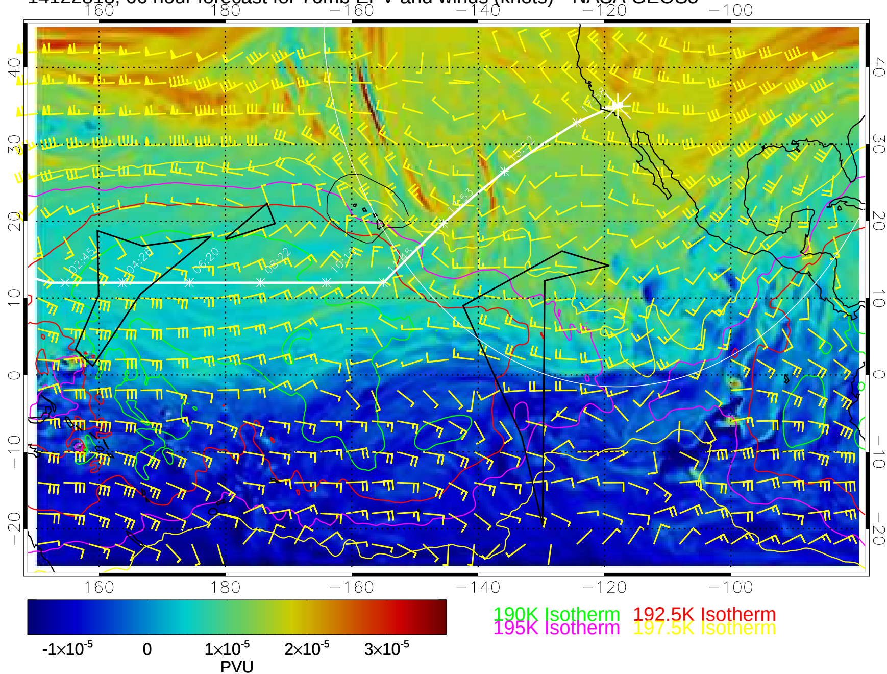
14122818, 66 hour forecast for 70mb EPV and winds (knots)-- NASA GEOS5
