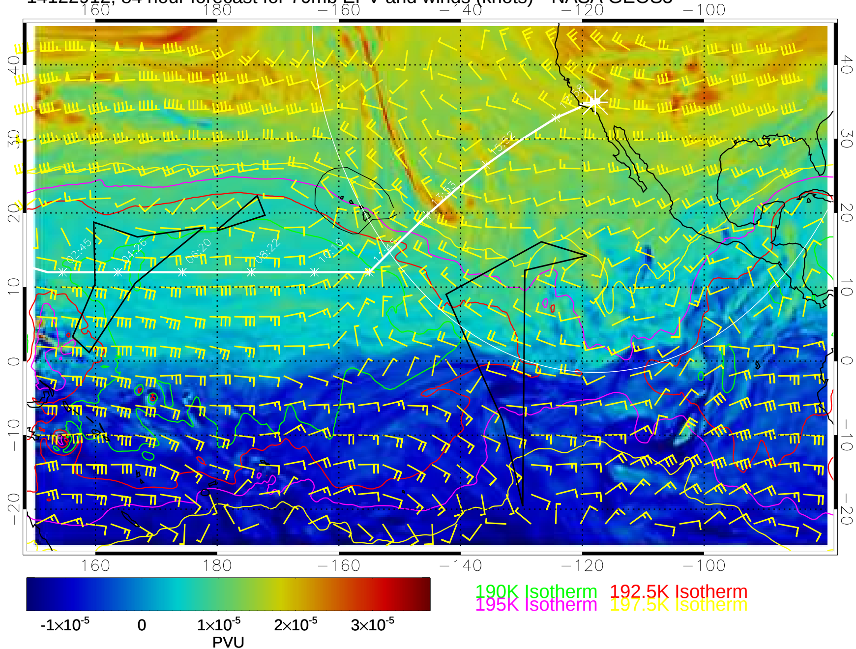
14122912, 84 hour forecast for 70mb EPV and winds (knots)-- NASA GEOS5
