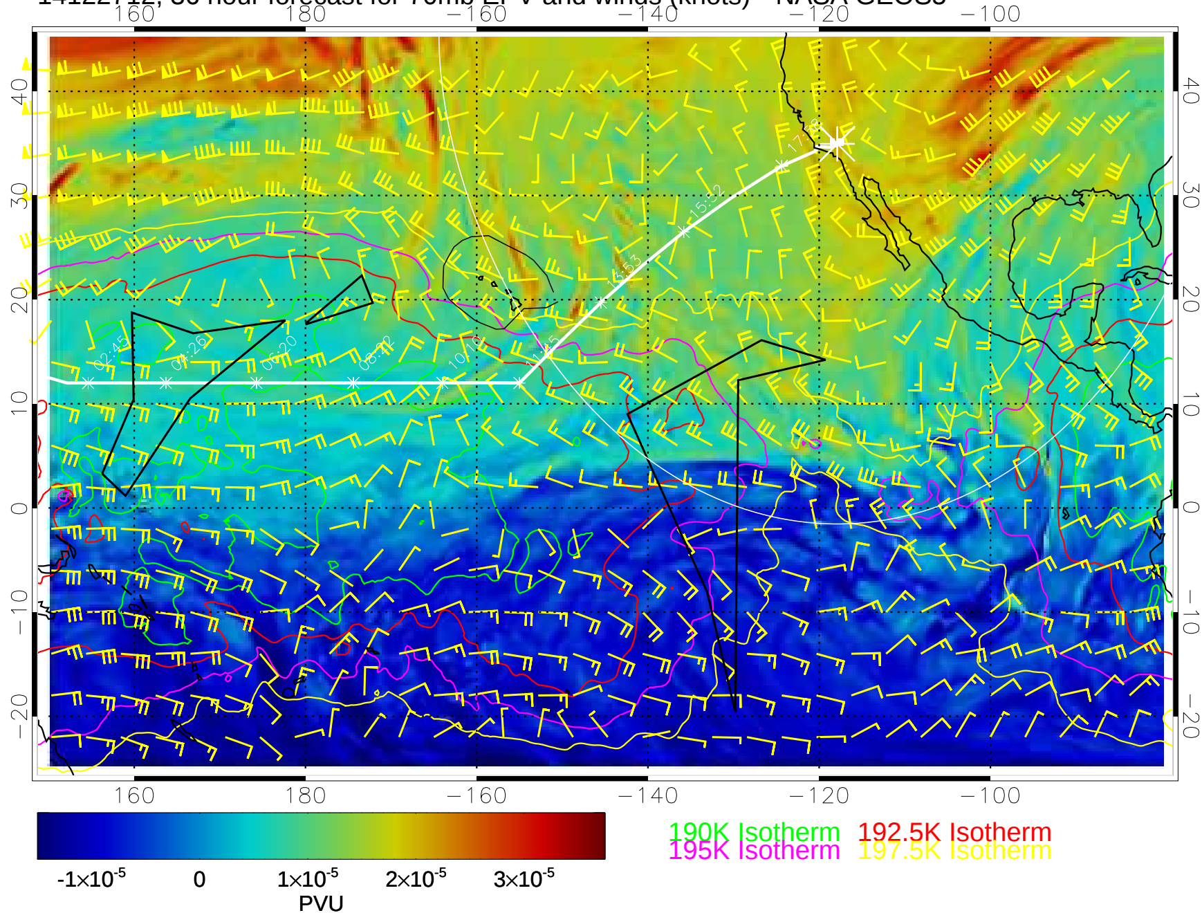
14122712, 36 hour forecast for 70mb EPV and winds (knots)-- NASA GEOS5
