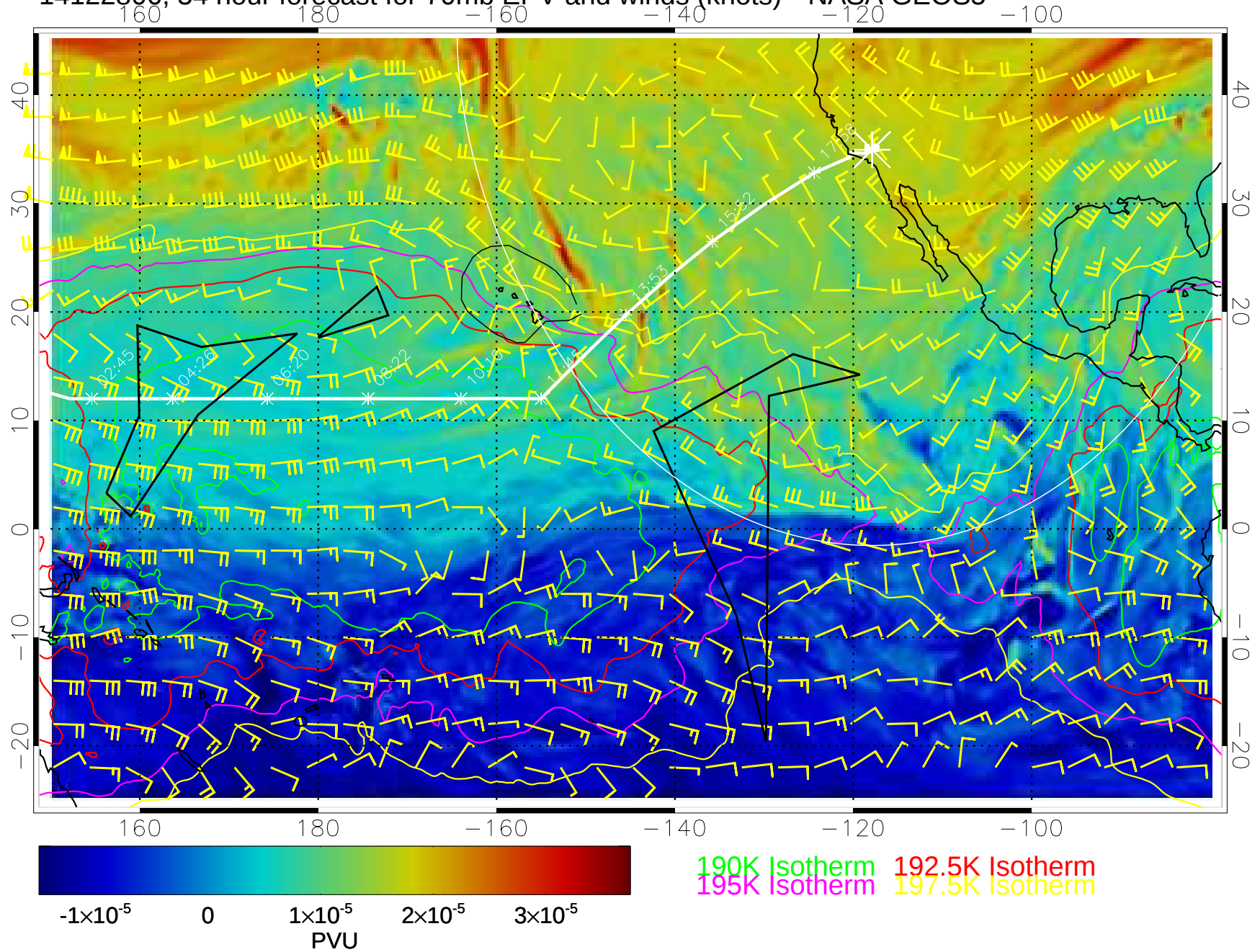
14122806, 54 hour forecast for 70mb EPV and winds (knots)-- NASA GEOS5
