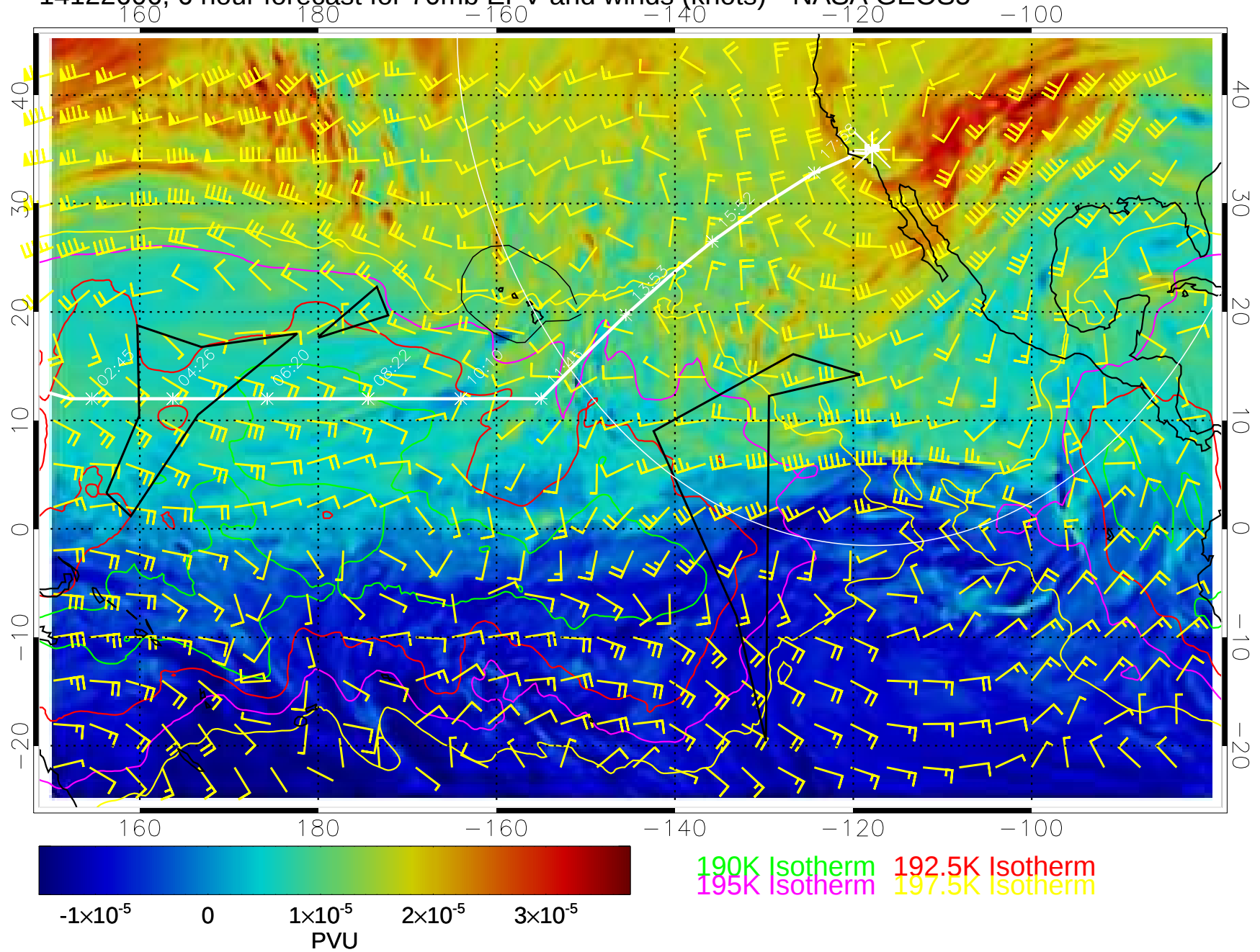
14122606, 6 hour forecast for 70mb EPV and winds (knots)-- NASA GEOS5
