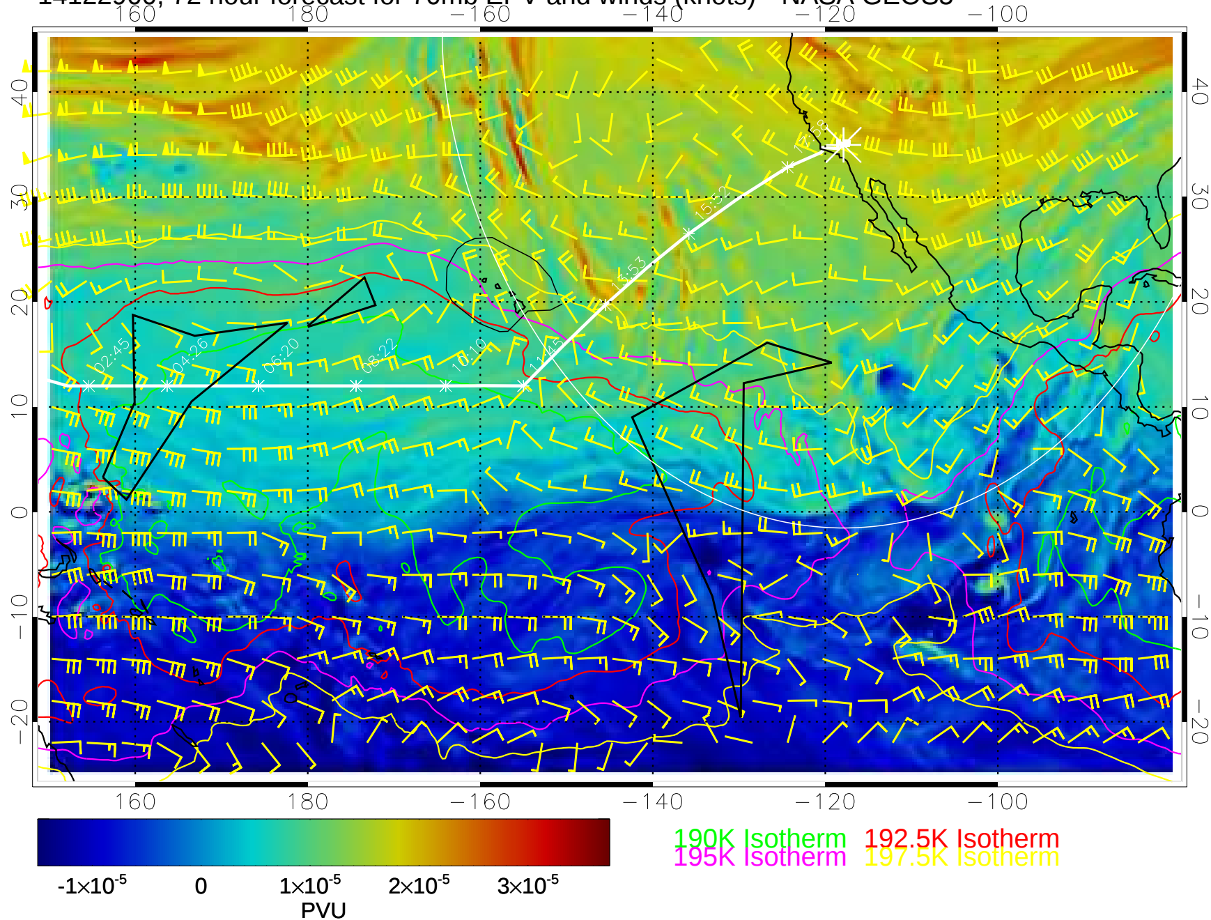
14122900, 72 hour forecast for 70mb EPV and winds (knots)-- NASA GEOS5
