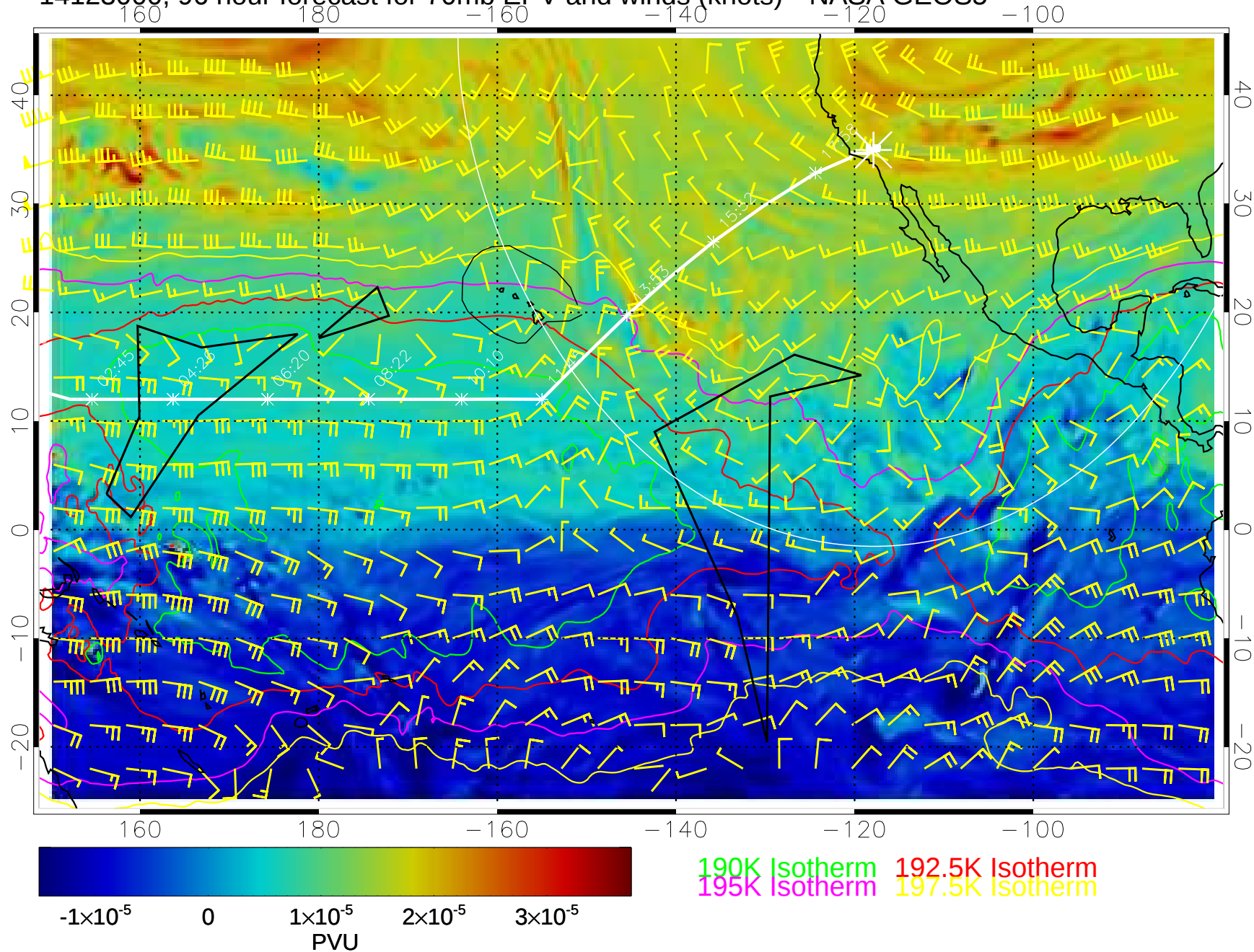
14123000, 96 hour forecast for 70mb EPV and winds (knots)-- NASA GEOS5
