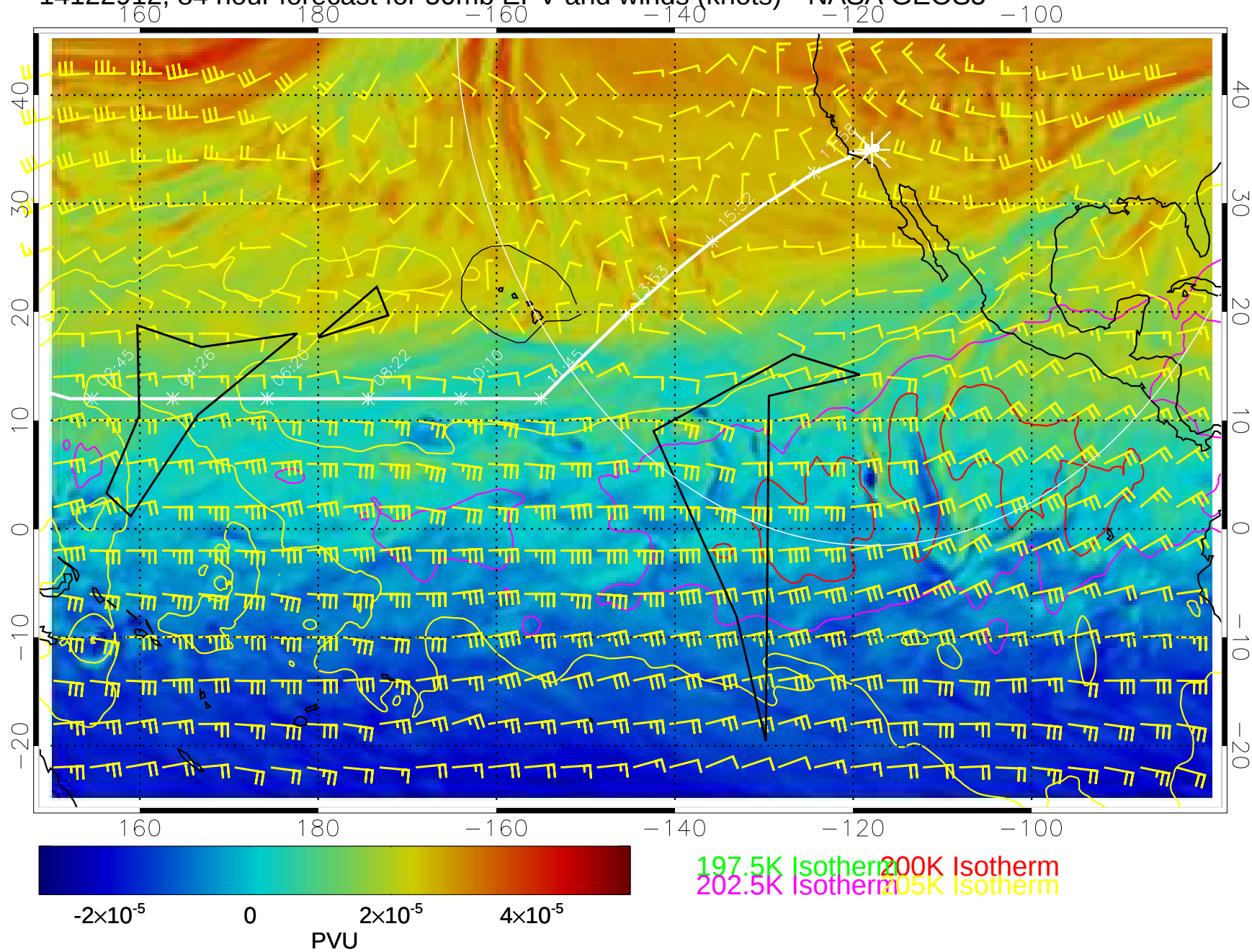
14122912, 84 hour forecast for 50mb EPV and winds (knots)-- NASA GEOS5
