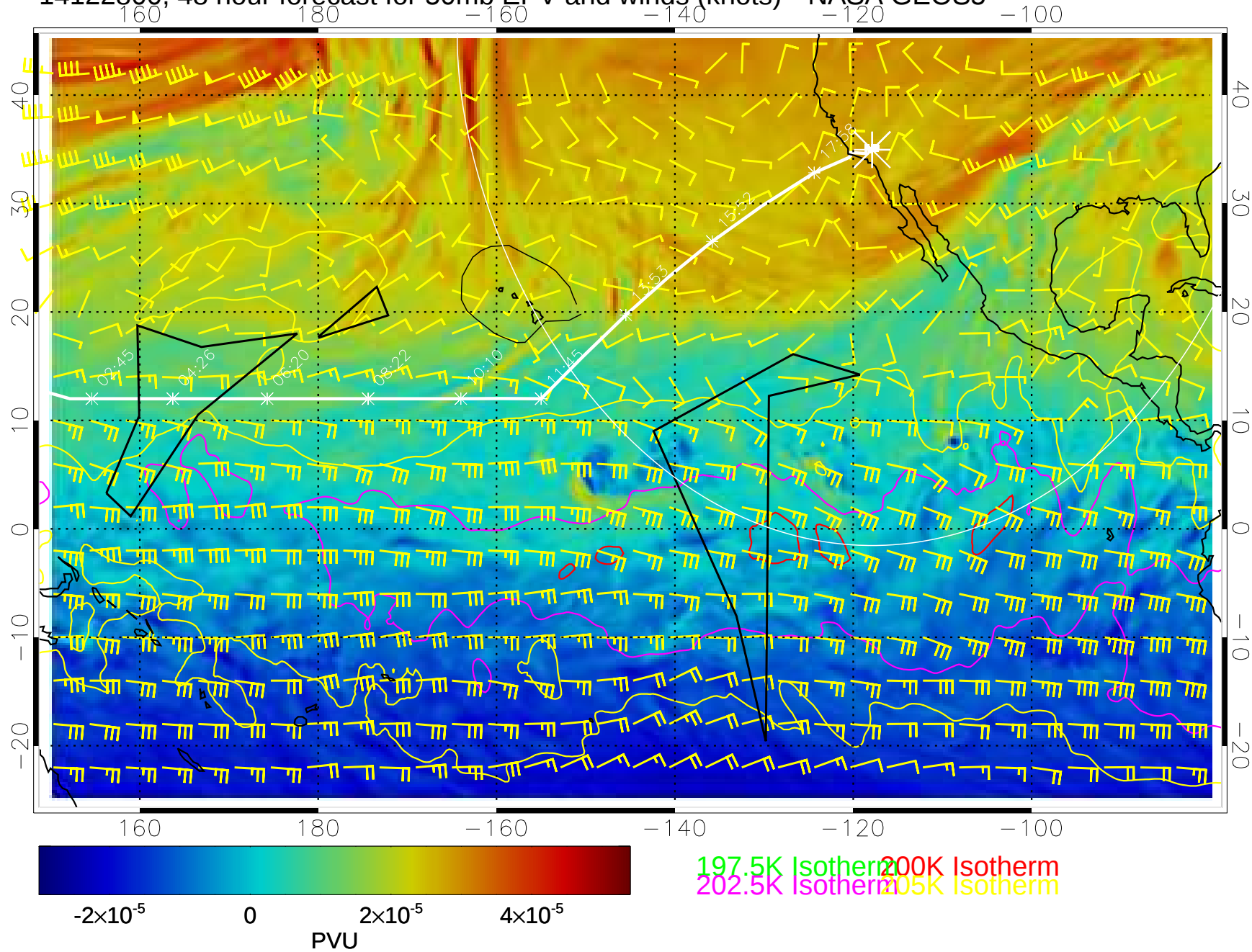
14122800, 48 hour forecast for 50mb EPV and winds (knots)-- NASA GEOS5
