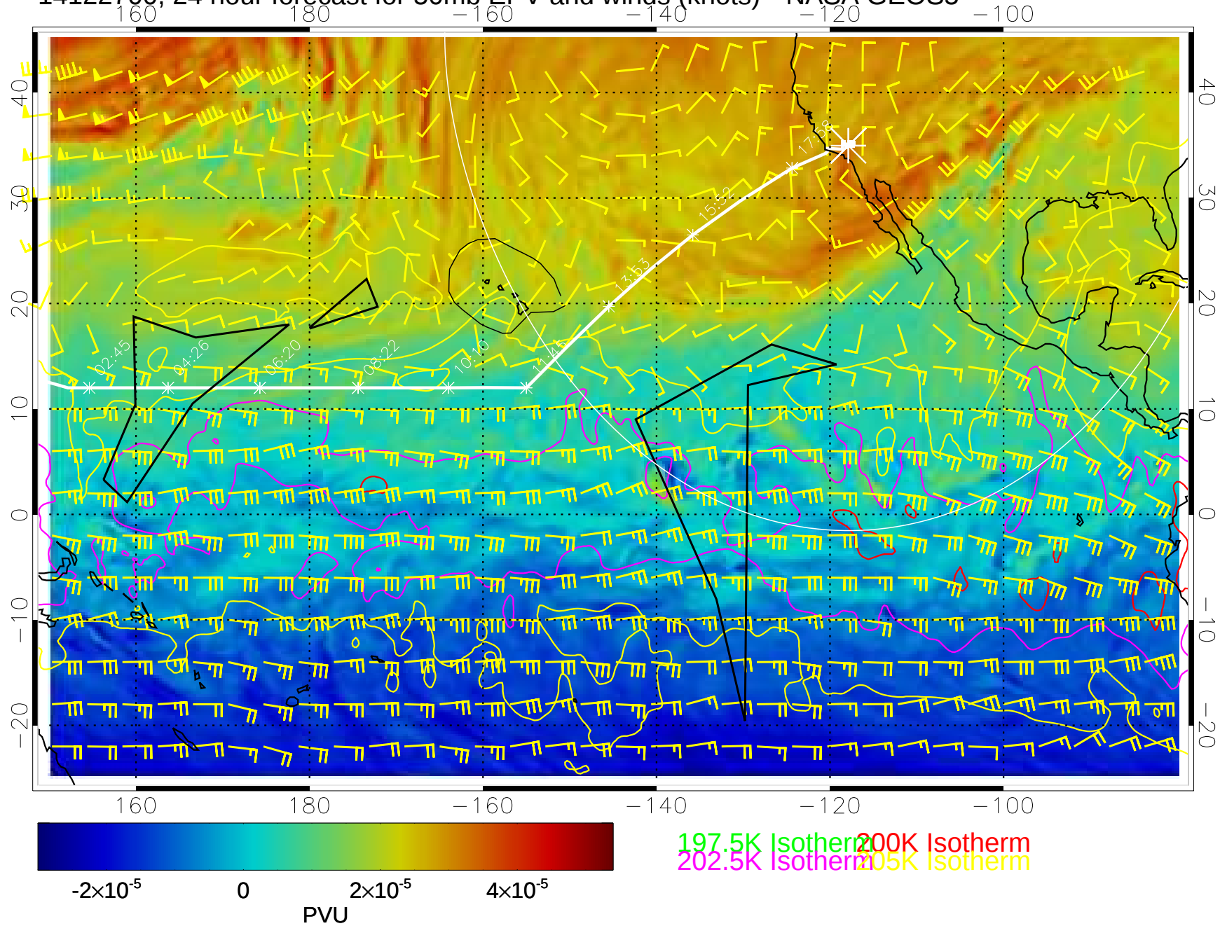
14122700, 24 hour forecast for 50mb EPV and winds (knots)-- NASA GEOS5
