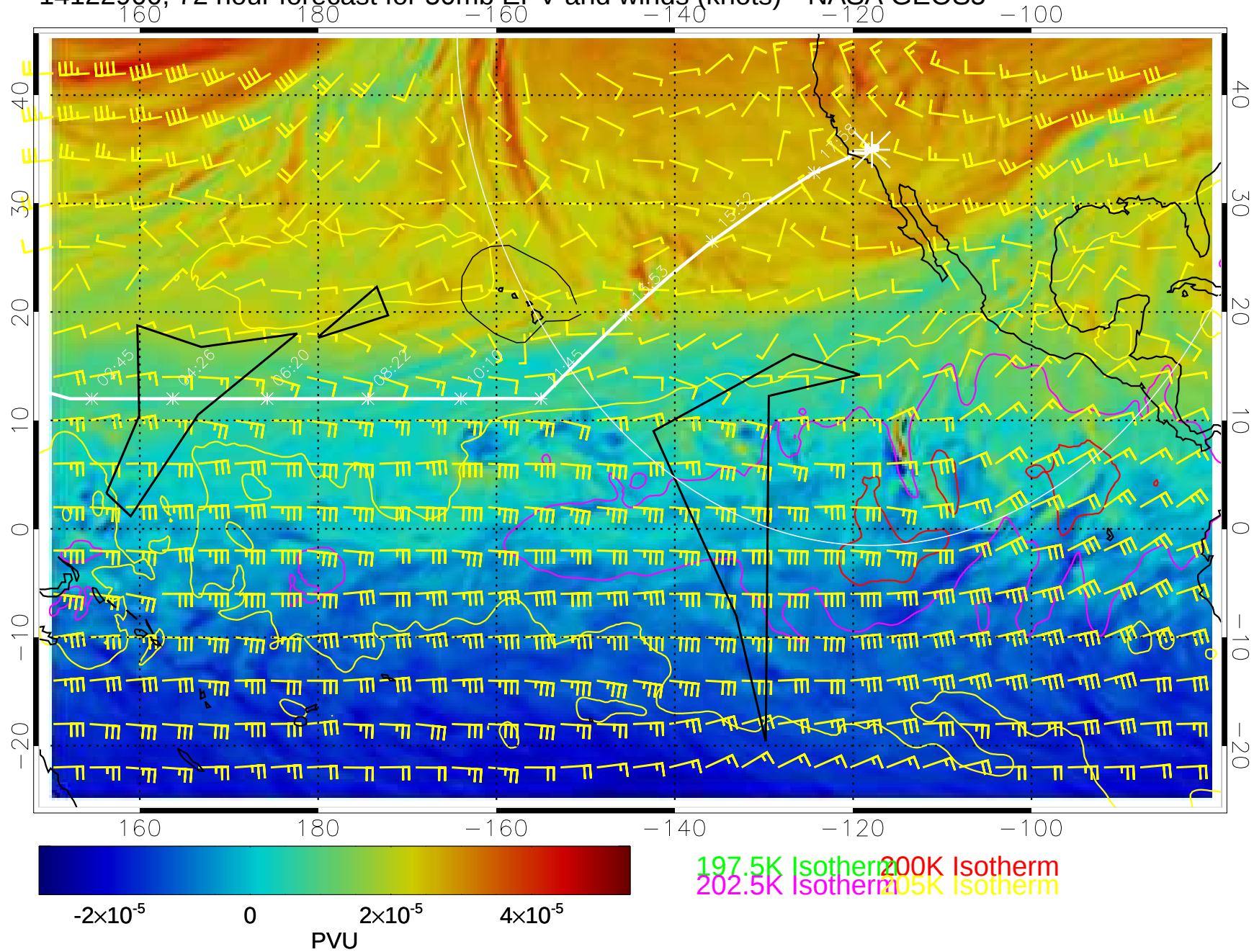
14122900, 72 hour forecast for 50mb EPV and winds (knots)-- NASA GEOS5
