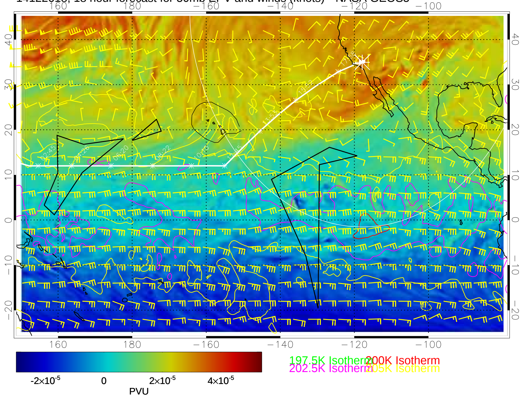
14122618, 18 hour forecast for 50mb EPV and winds (knots)-- NASA GEOS5
