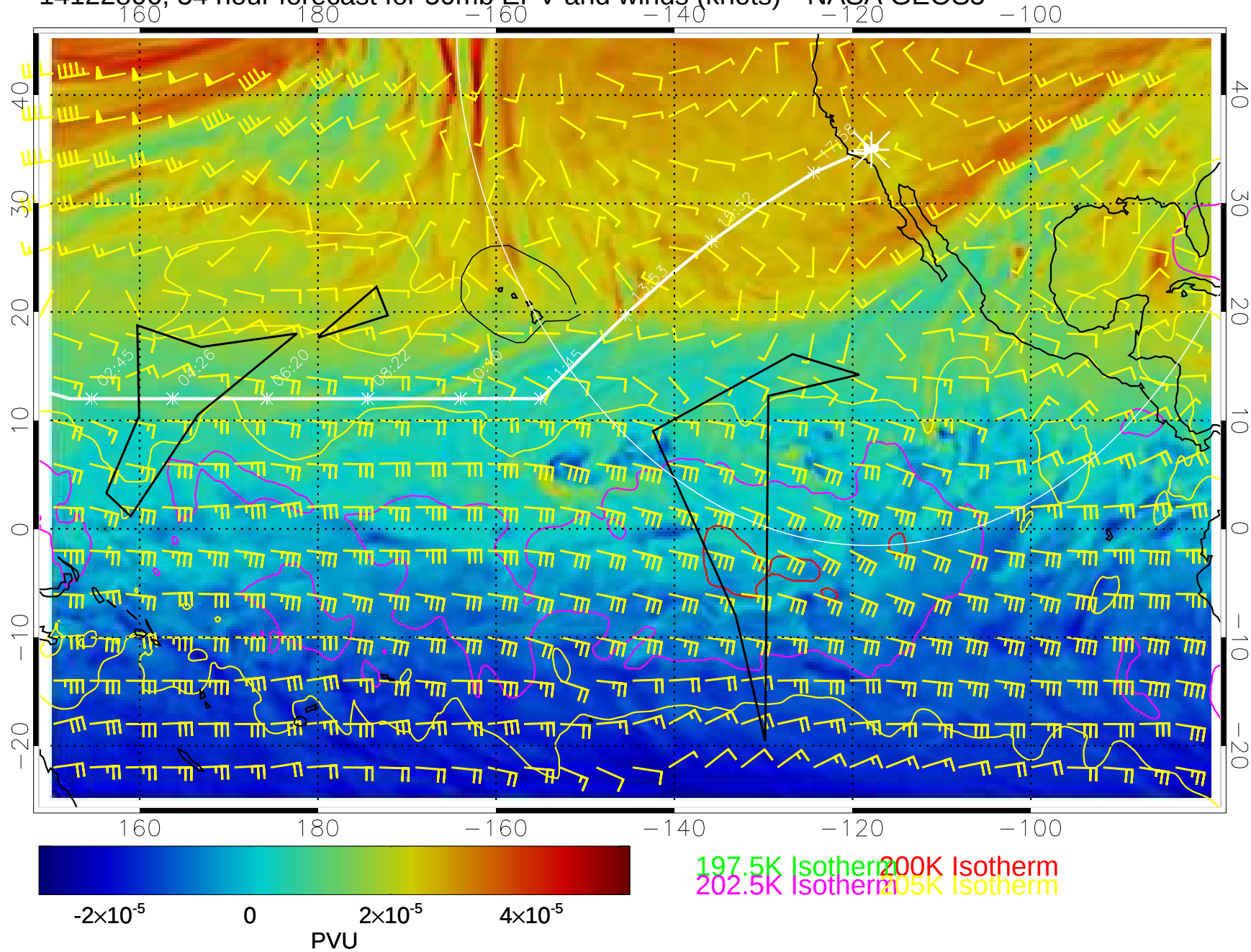
14122806, 54 hour forecast for 50mb EPV and winds (knots)-- NASA GEOS5
