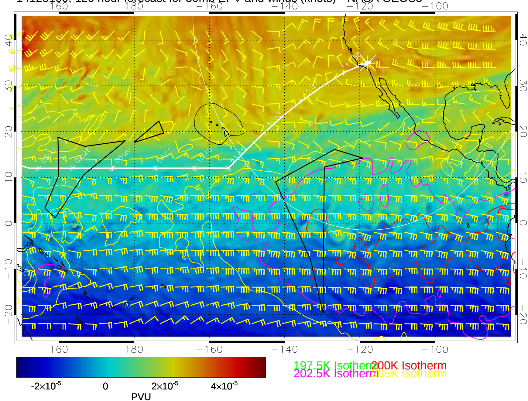
14123100, 120 hour forecast for 50mb EPV and winds (knots)-- NASA GEOS5
