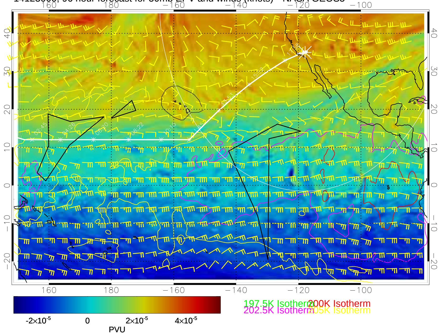
14123000, 96 hour forecast for 50mb EPV and winds (knots)-- NASA GEOS5
