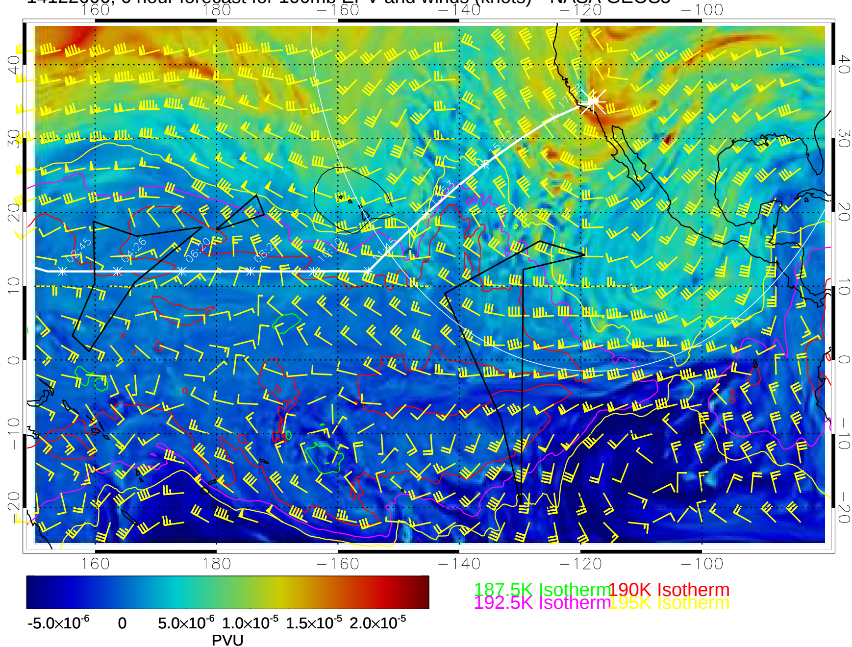
14122606, 6 hour forecast for 100mb EPV and winds (knots)-- NASA GEOS5
