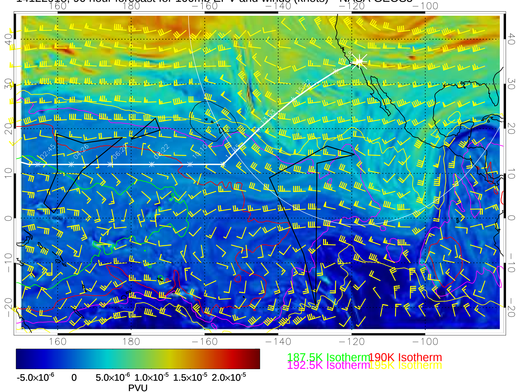
14122918, 90 hour forecast for 100mb EPV and winds (knots)-- NASA GEOS5
