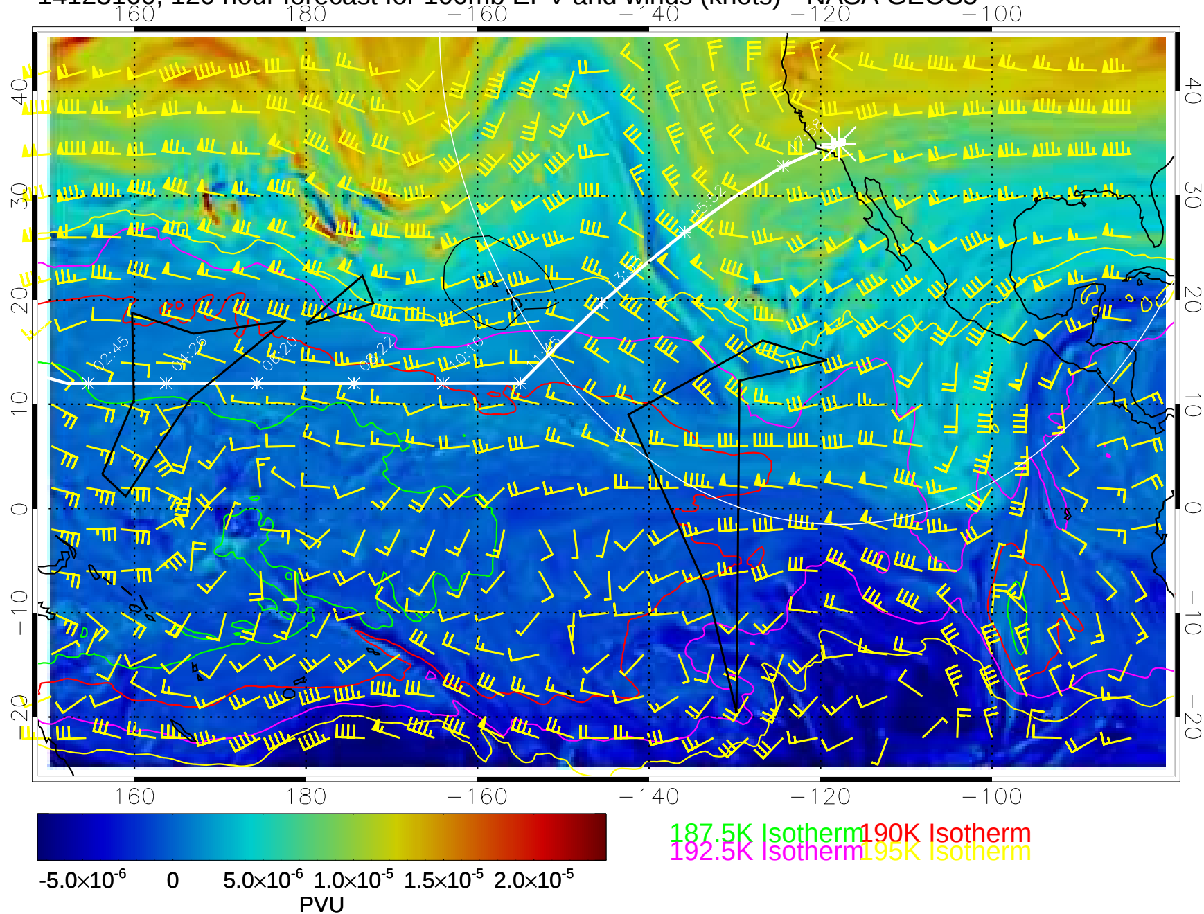
14123100, 120 hour forecast for 100mb EPV and winds (knots)-- NASA GEOS5
