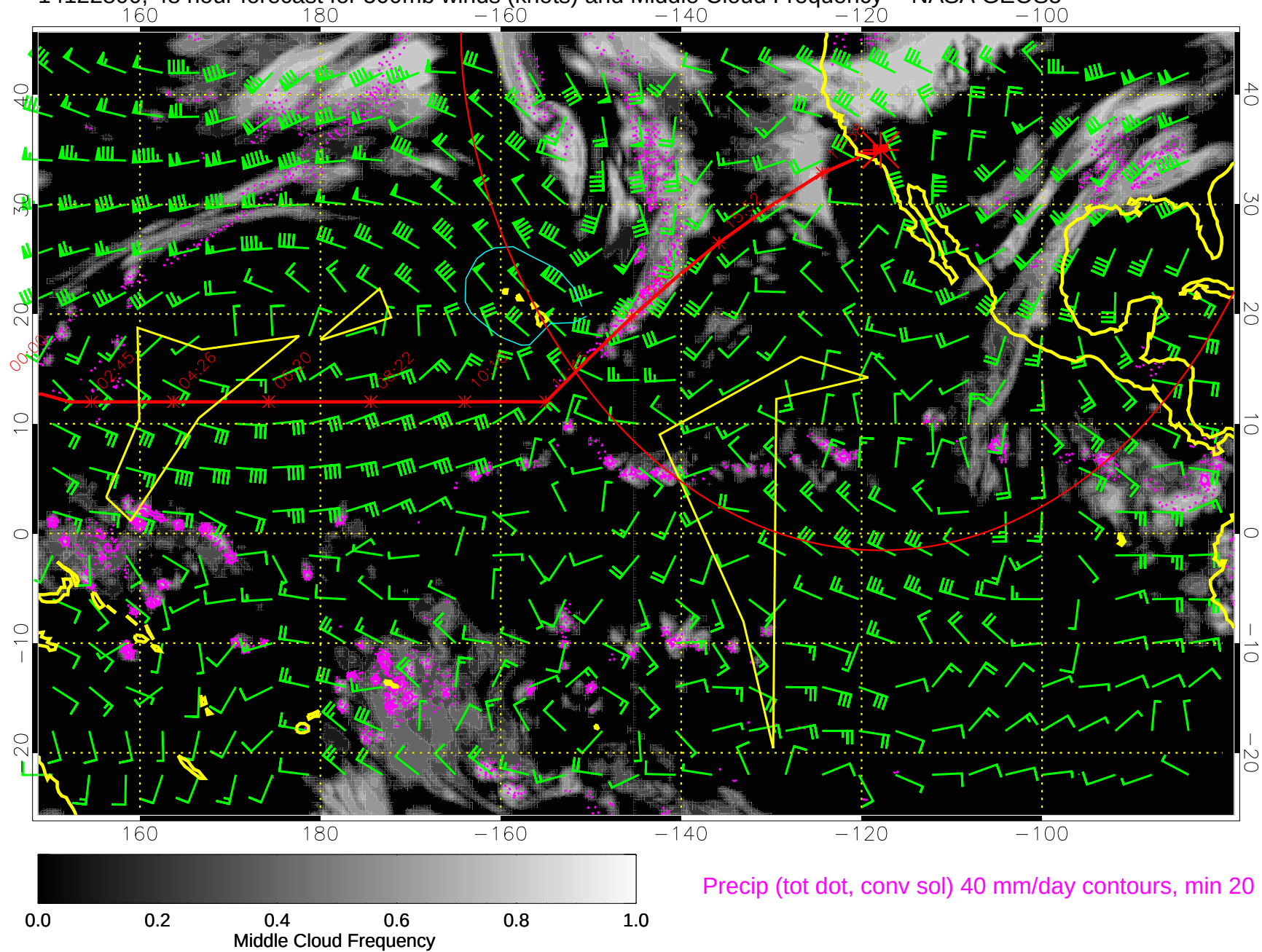
14122800, 48 hour forecast for 500mb winds (knots) and Middle Cloud Frequency -- NASA GEOS5
