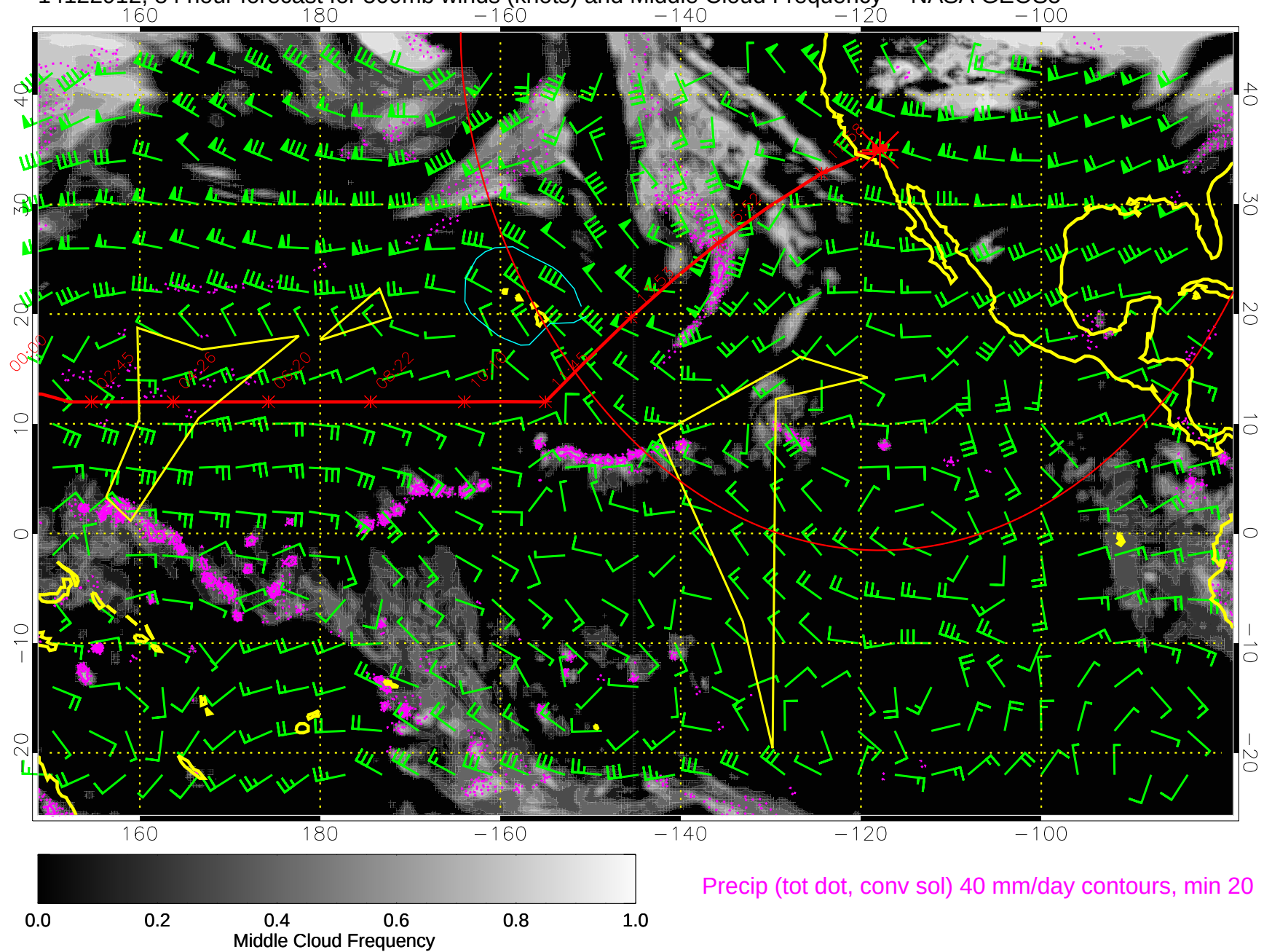
14122912, 84 hour forecast for 500mb winds (knots) and Middle Cloud Frequency -- NASA GEOS5
