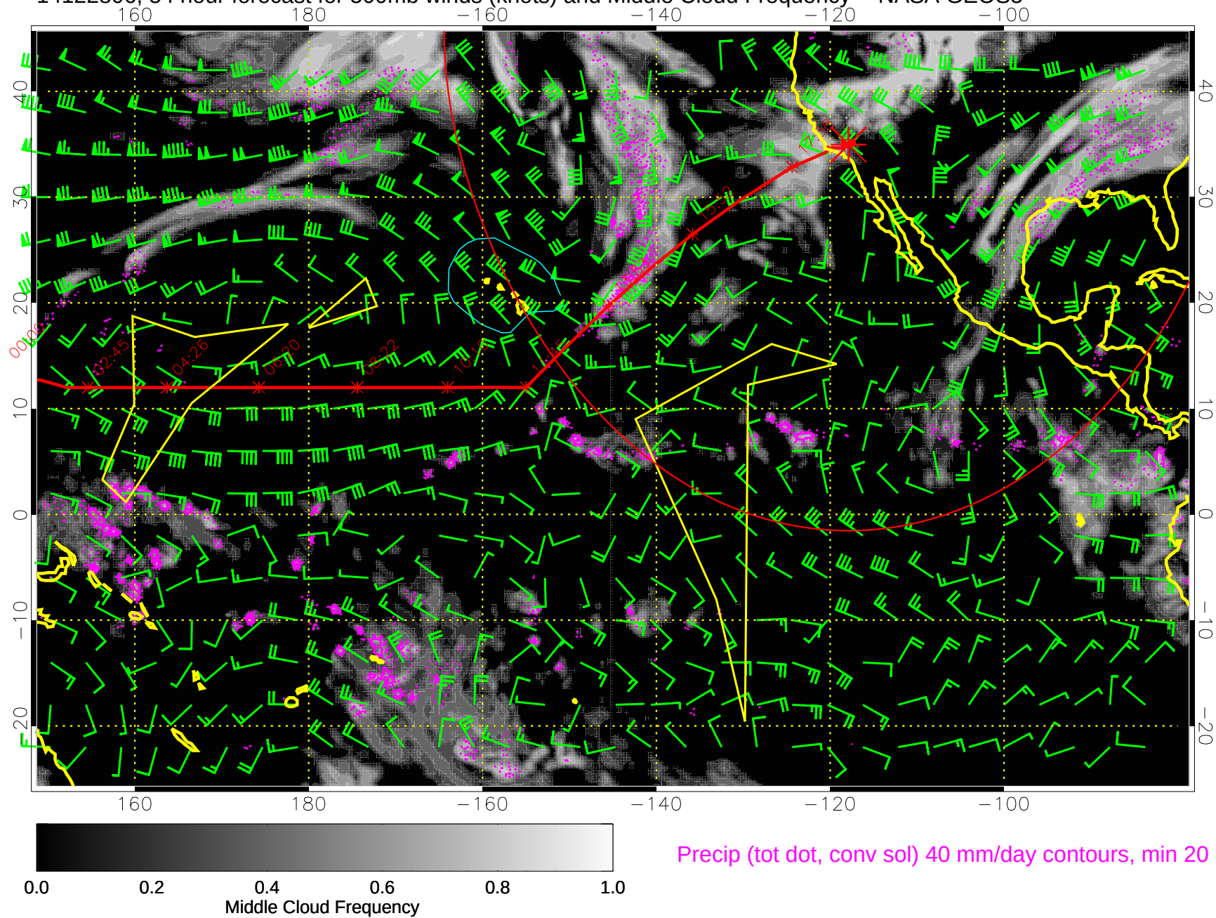
14122806, 54 hour forecast for 500mb winds (knots) and Middle Cloud Frequency -- NASA GEOS5
