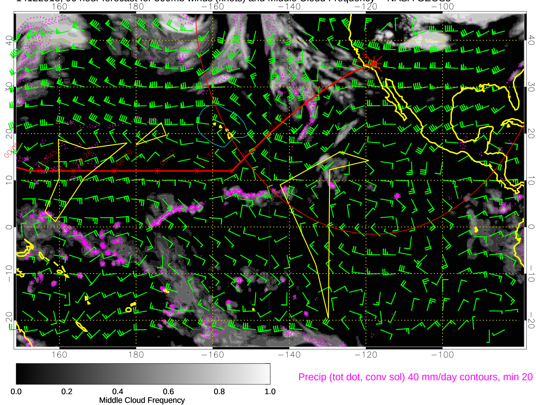
14122918, 90 hour forecast for 500mb winds (knots) and Middle Cloud Frequency -- NASA GEOS5
