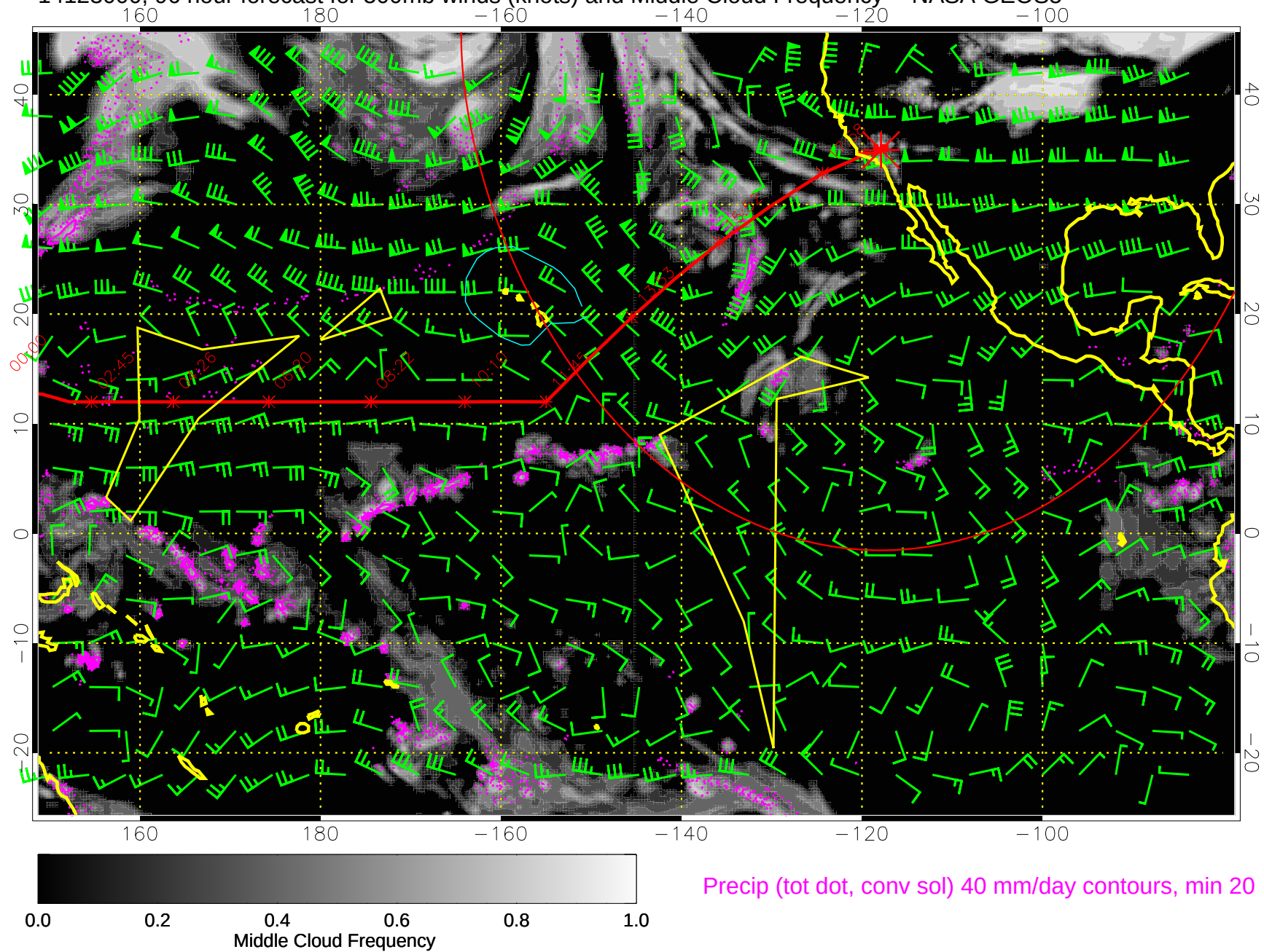
14123000, 96 hour forecast for 500mb winds (knots) and Middle Cloud Frequency -- NASA GEOS5
