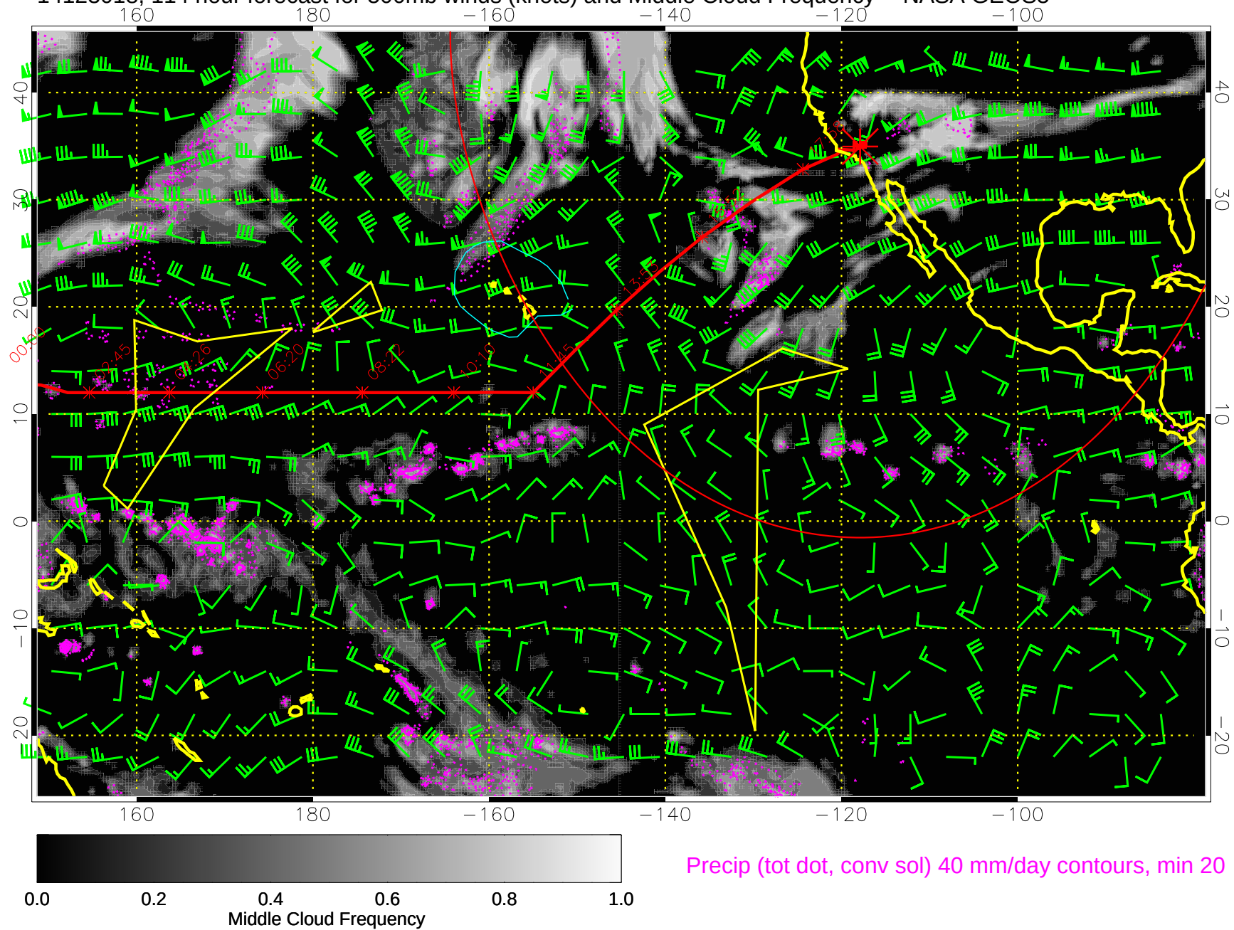
14123018, 114 hour forecast for 500mb winds (knots) and Middle Cloud Frequency -- NASA GEOS5
