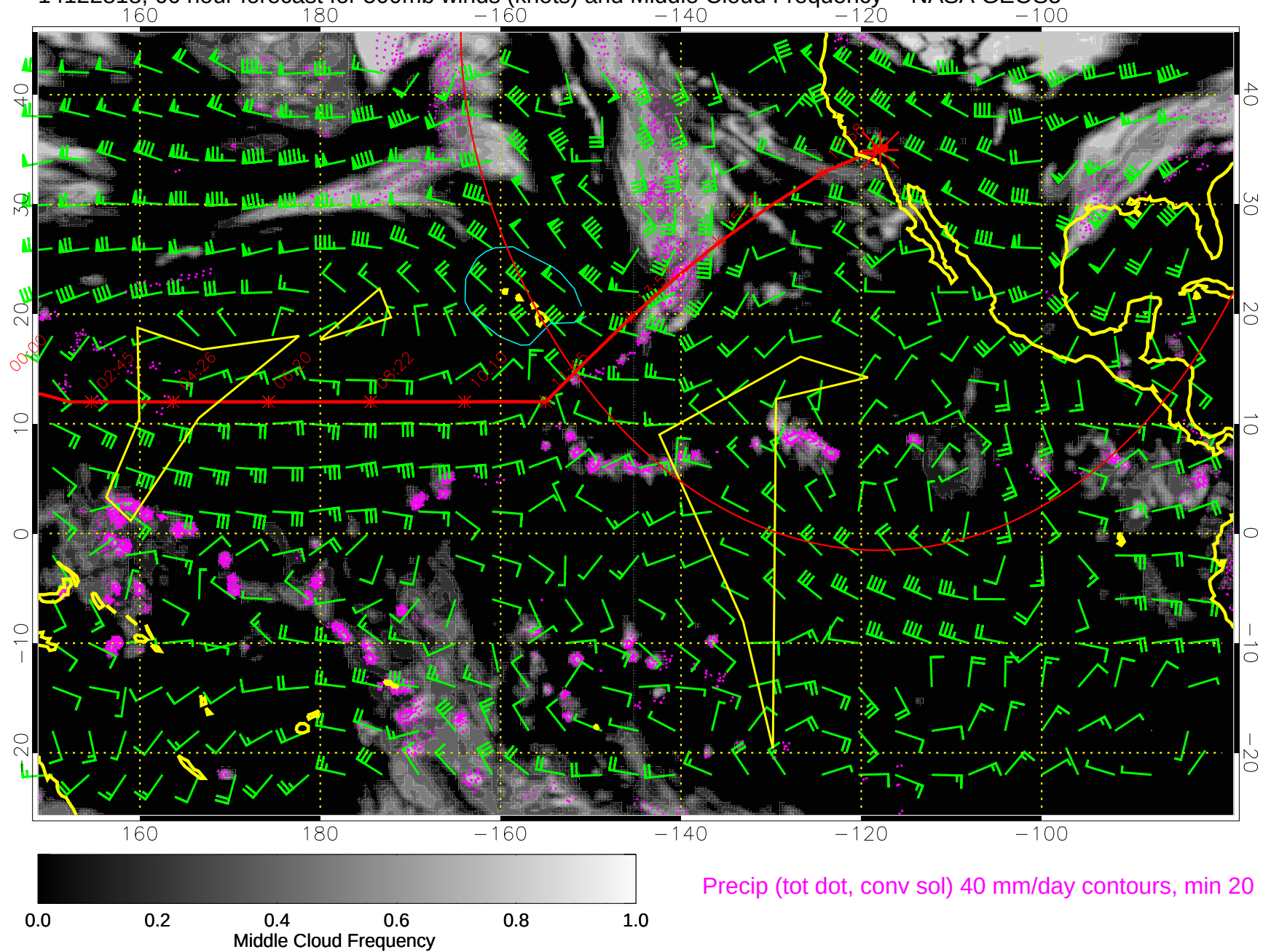
14122818, 66 hour forecast for 500mb winds (knots) and Middle Cloud Frequency -- NASA GEOS5
