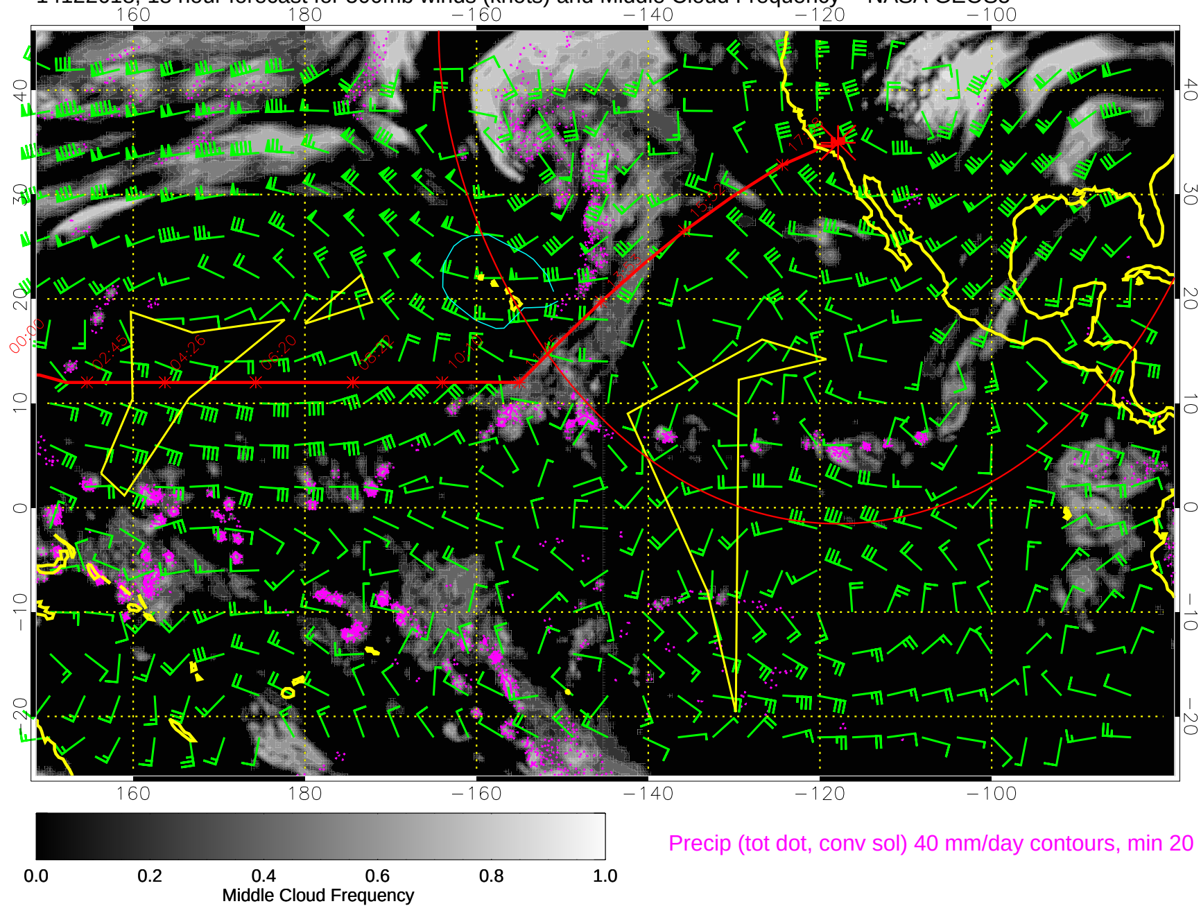
14122618, 18 hour forecast for 500mb winds (knots) and Middle Cloud Frequency -- NASA GEOS5
