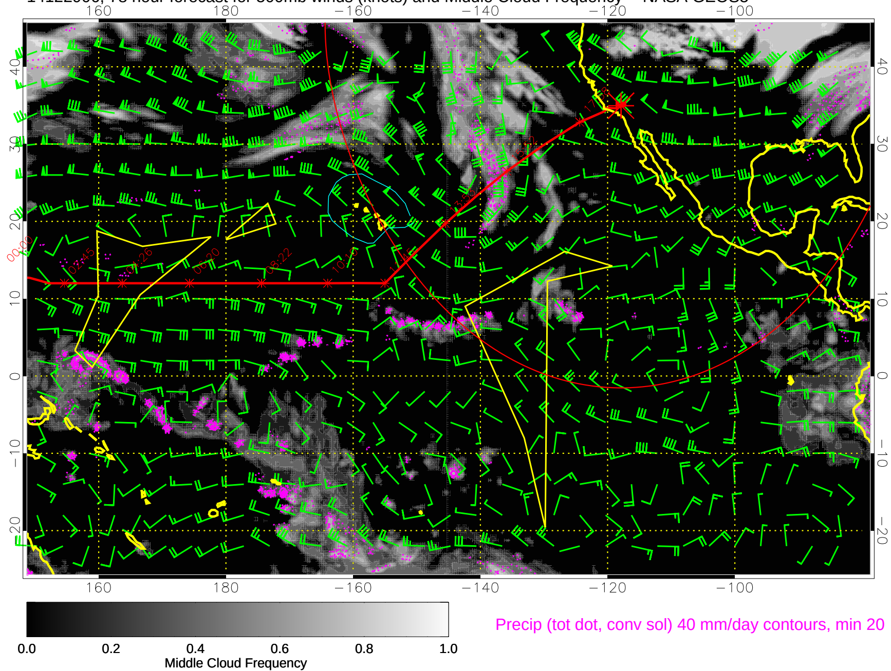
14122906, 78 hour forecast for 500mb winds (knots) and Middle Cloud Frequency -- NASA GEOS5
