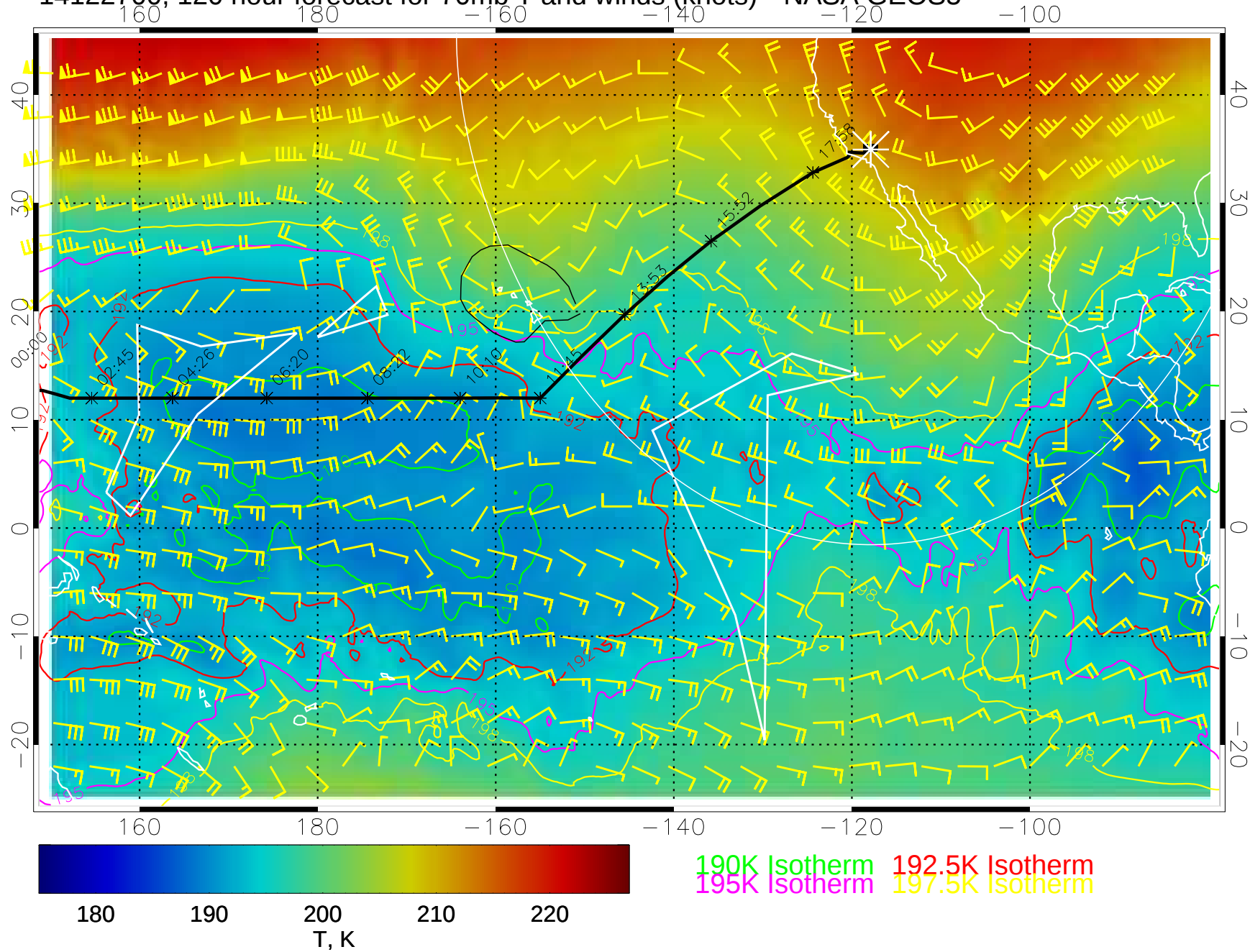
14122700, 120 hour forecast for 70mb T and winds (knots)-- NASA GEOS5
