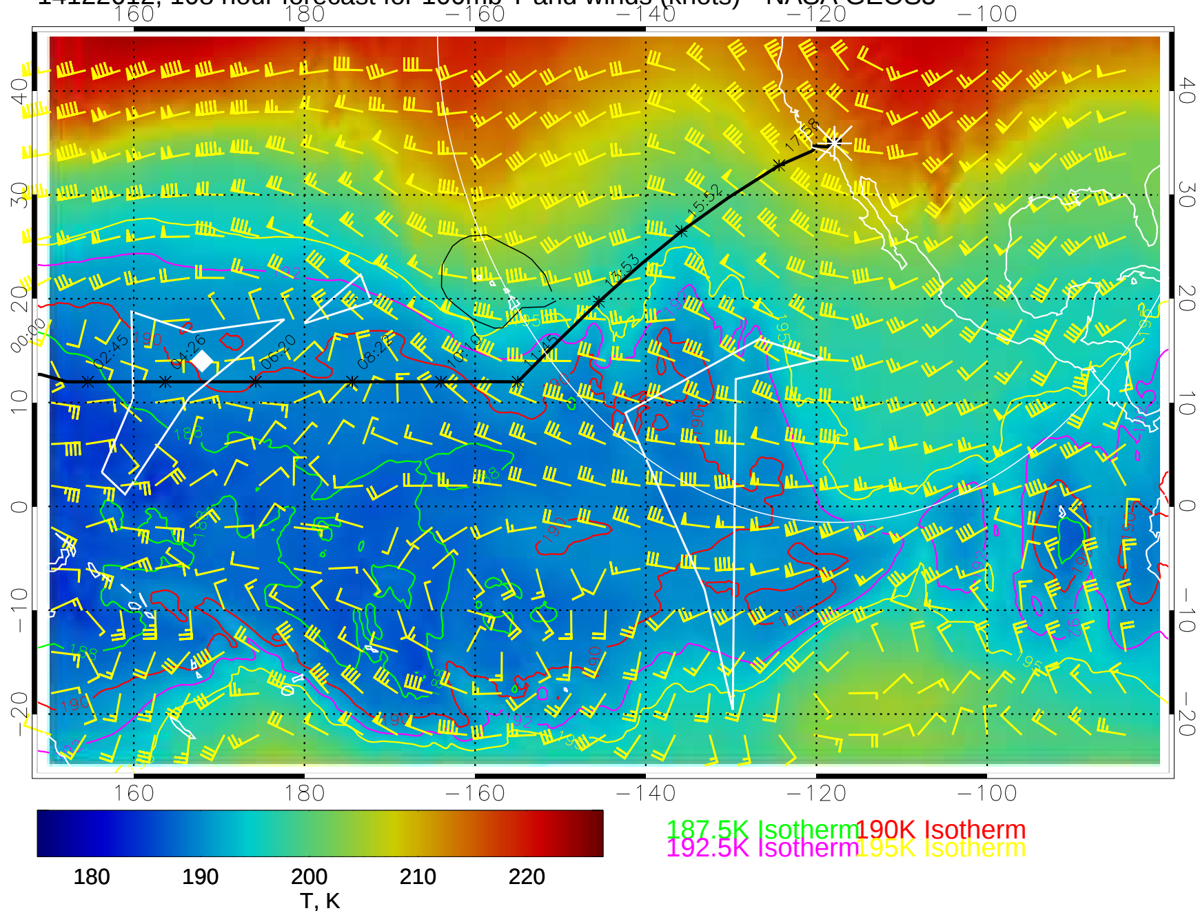
14122612, 108 hour forecast for 100mb T and winds (knots)-- NASA GEOS5
