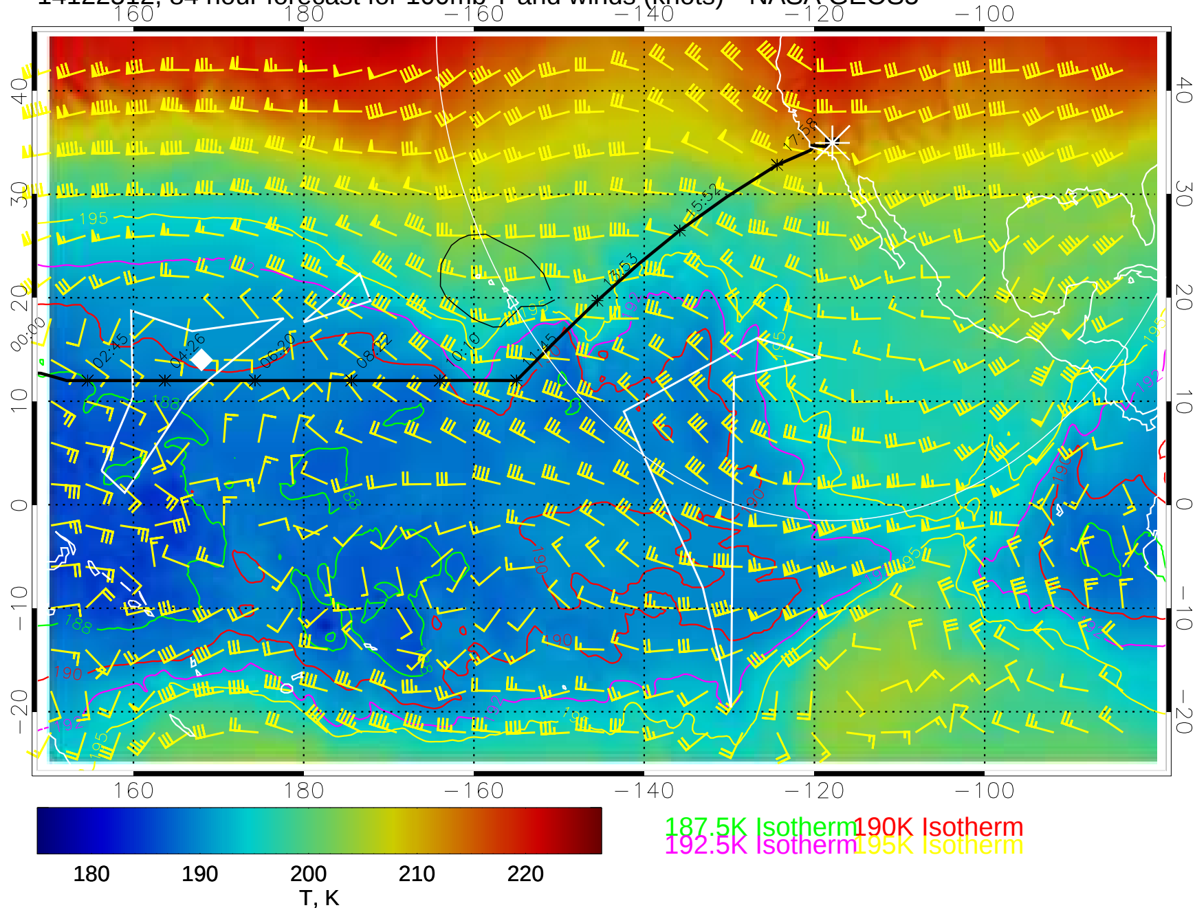
14122512, 84 hour forecast for 100mb T and winds (knots)-- NASA GEOS5
