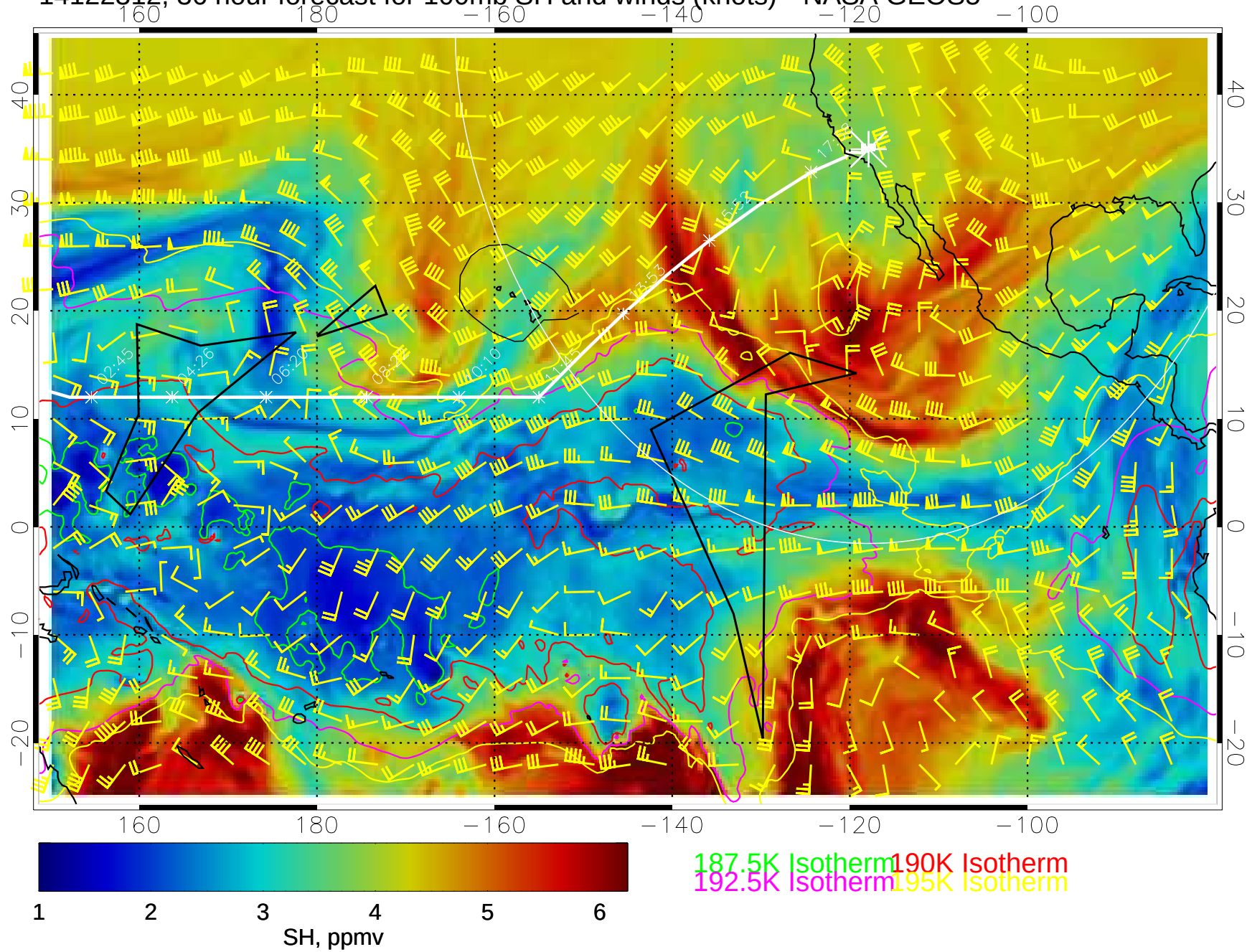
14122312, 36 hour forecast for 100mb SH and winds (knots)-- NASA GEOS5
