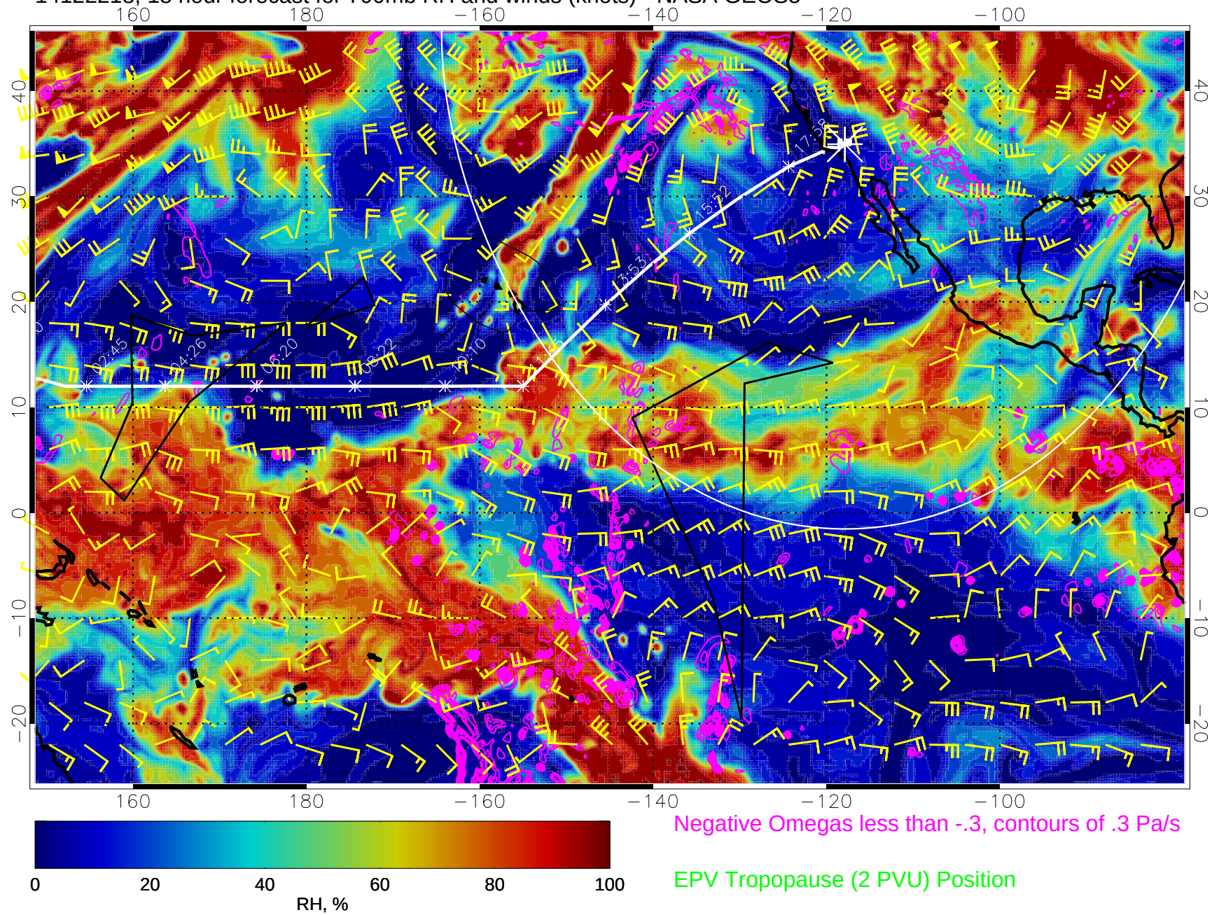
14122218, 18 hour forecast for 700mb RH and winds (knots) - NASA GEOS5
