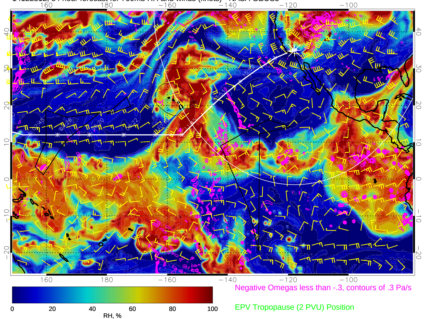
14122512, 84 hour forecast for 700mb RH and winds (knots) - NASA GEOS5
