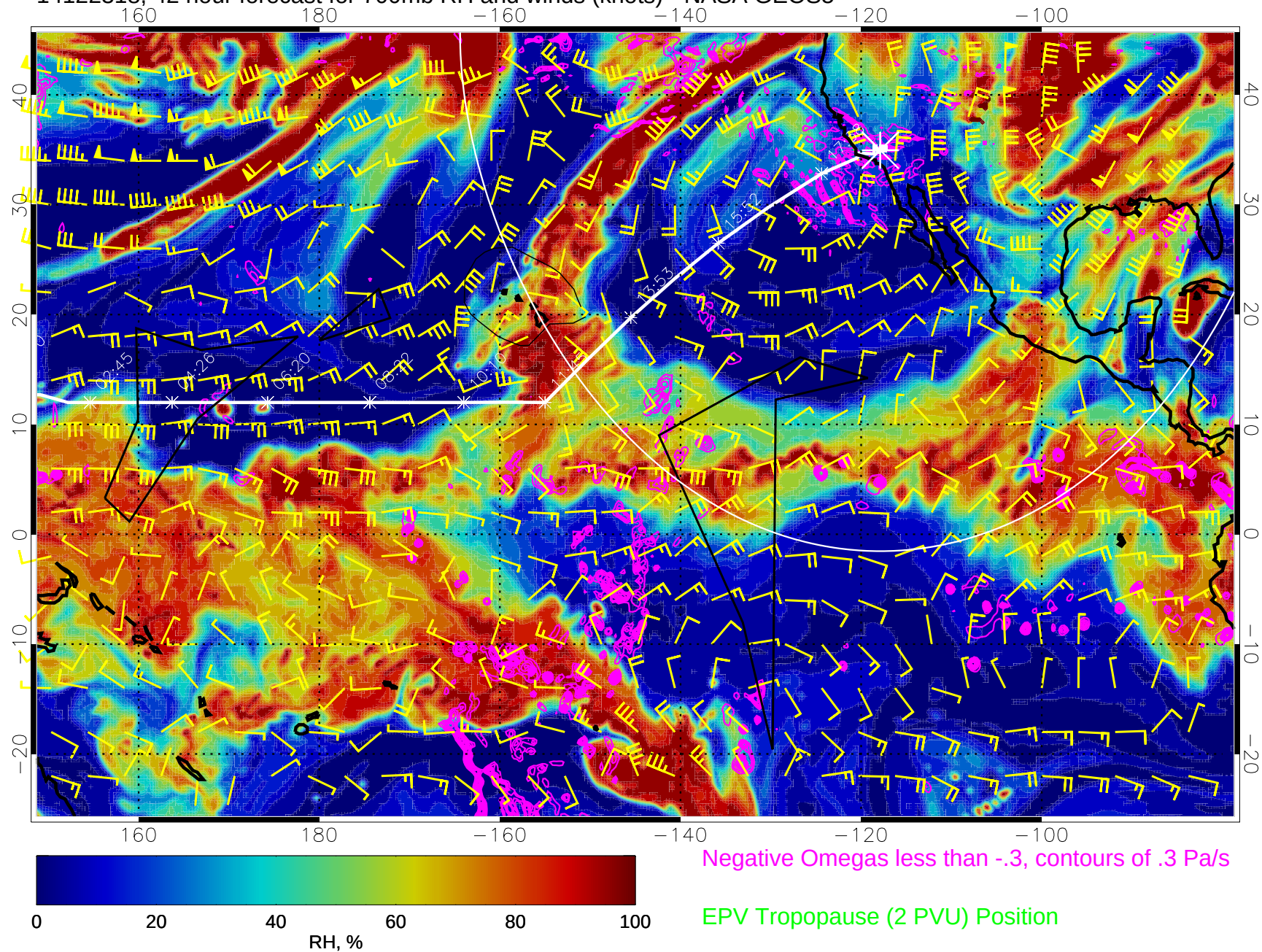
14122318, 42 hour forecast for 700mb RH and winds (knots) - NASA GEOS5
