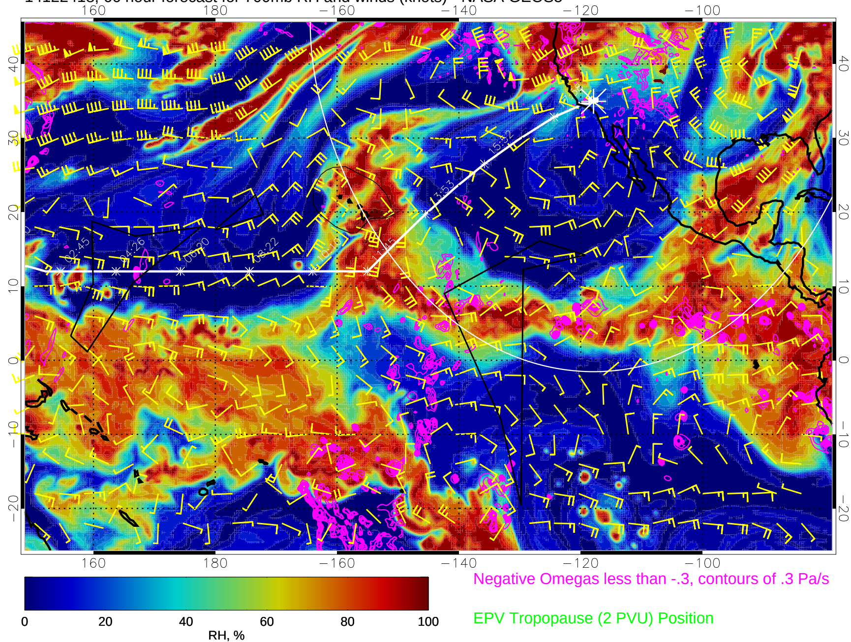
14122418, 66 hour forecast for 700mb RH and winds (knots) - NASA GEOS5
