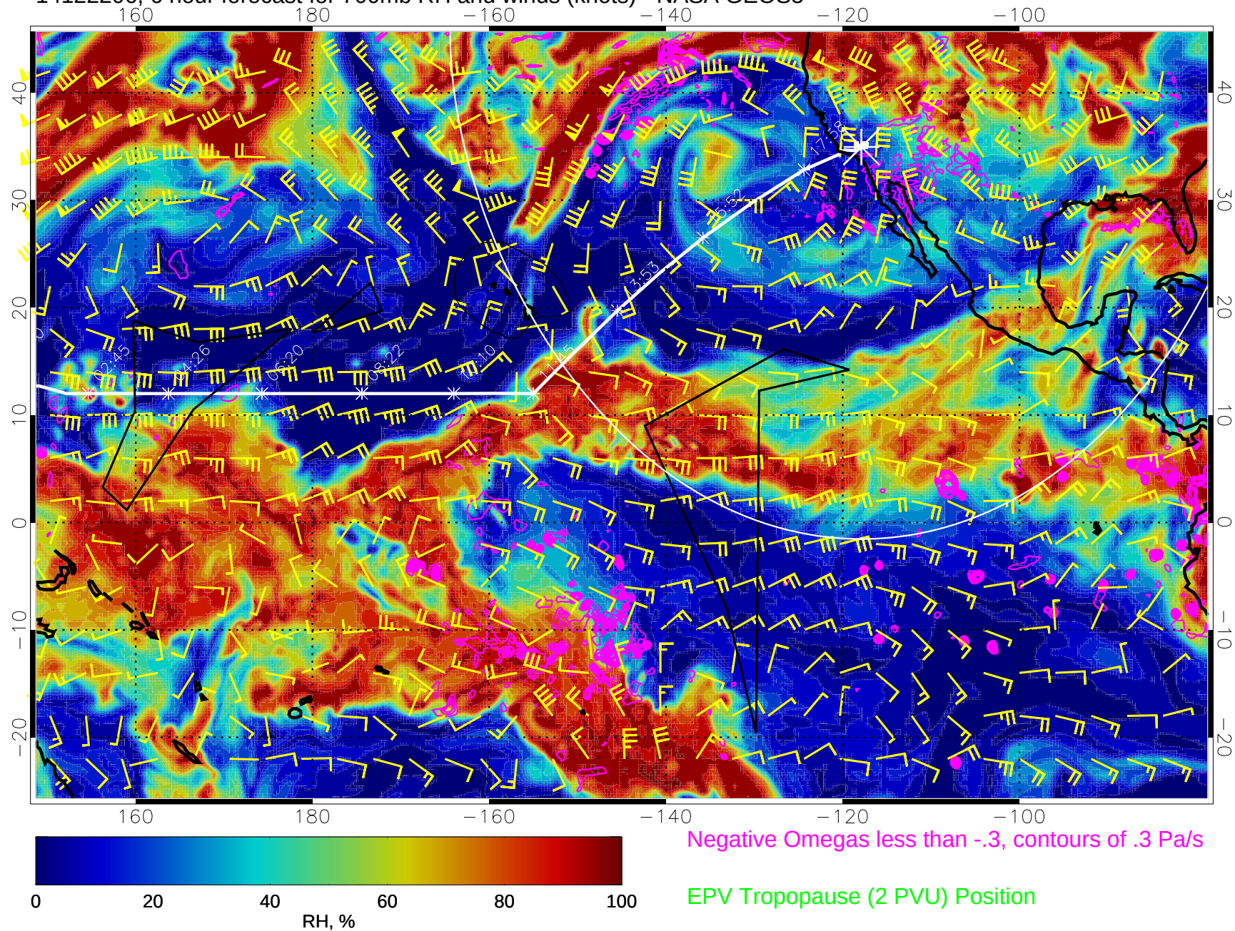
14122206, 6 hour forecast for 700mb RH and winds (knots) - NASA GEOS5
