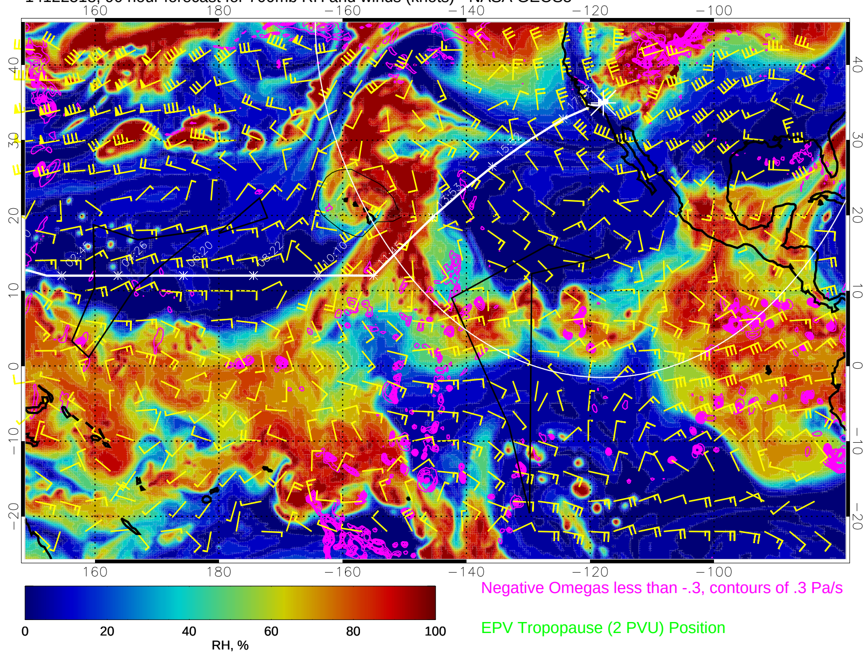
14122518, 90 hour forecast for 700mb RH and winds (knots) - NASA GEOS5
