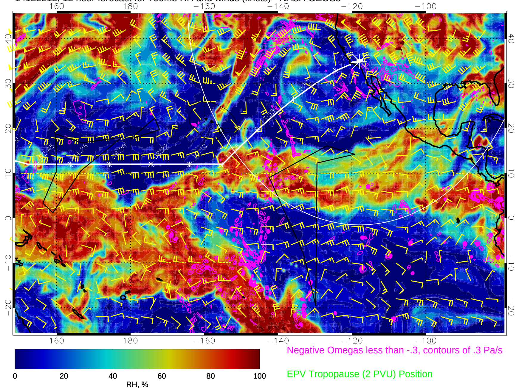
14122212, 12 hour forecast for 700mb RH and winds (knots) - NASA GEOS5
