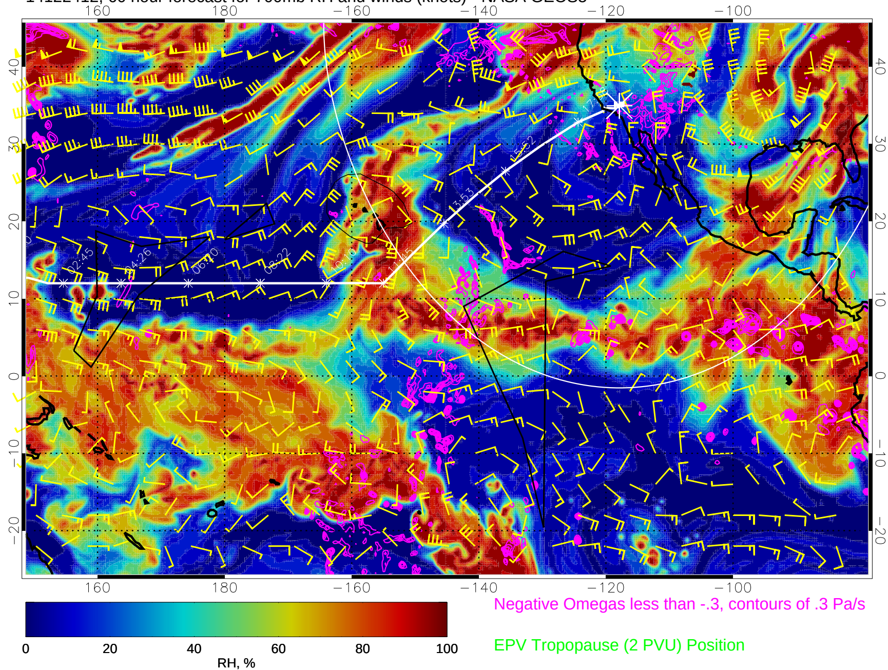
14122412, 60 hour forecast for 700mb RH and winds (knots) - NASA GEOS5
