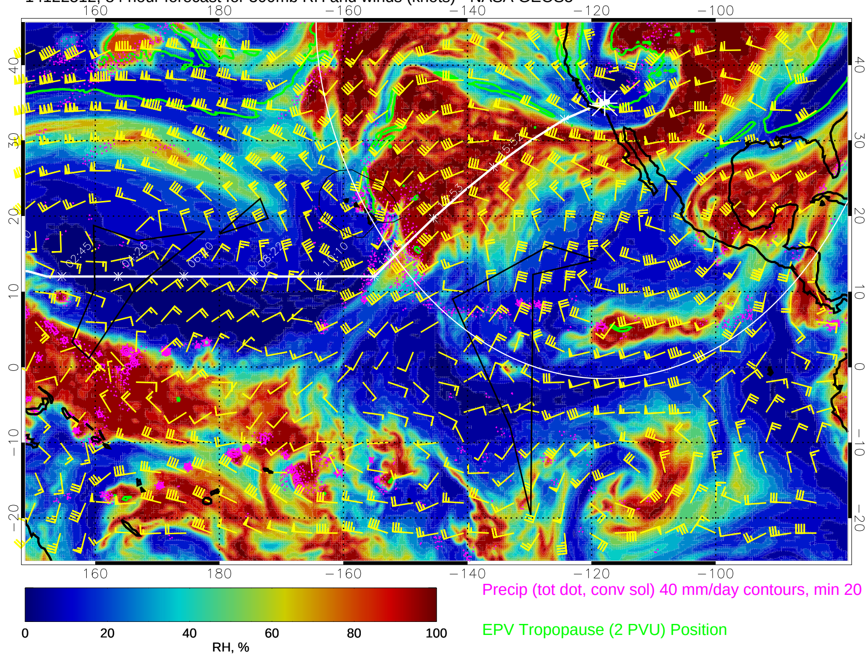
14122512, 84 hour forecast for 300mb RH and winds (knots) - NASA GEOS5
