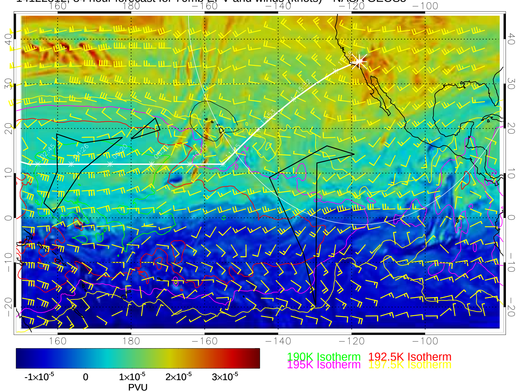
14122512, 84 hour forecast for 70mb EPV and winds (knots)-- NASA GEOS5
