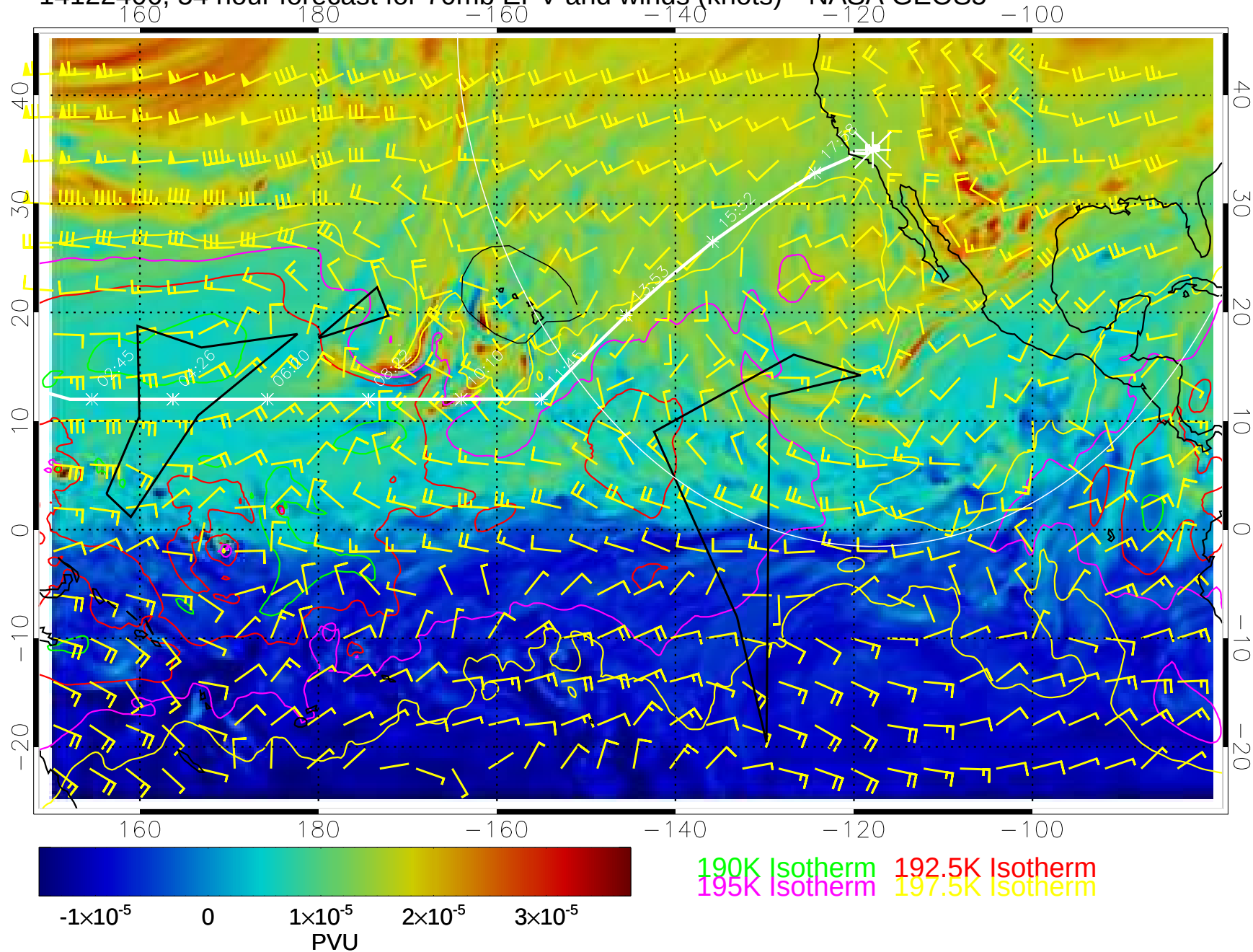
14122406, 54 hour forecast for 70mb EPV and winds (knots)-- NASA GEOS5
