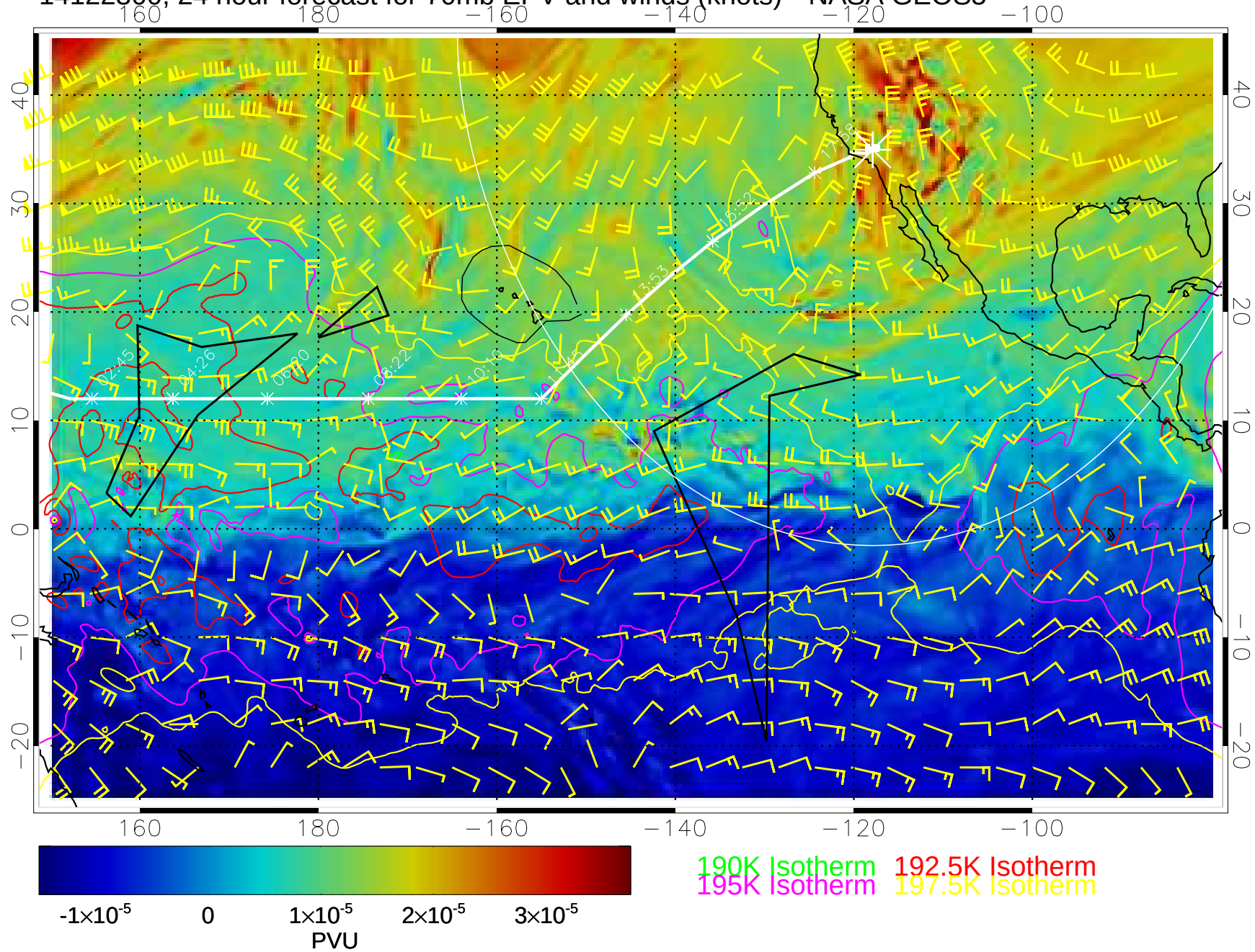
14122300, 24 hour forecast for 70mb EPV and winds (knots)-- NASA GEOS5
