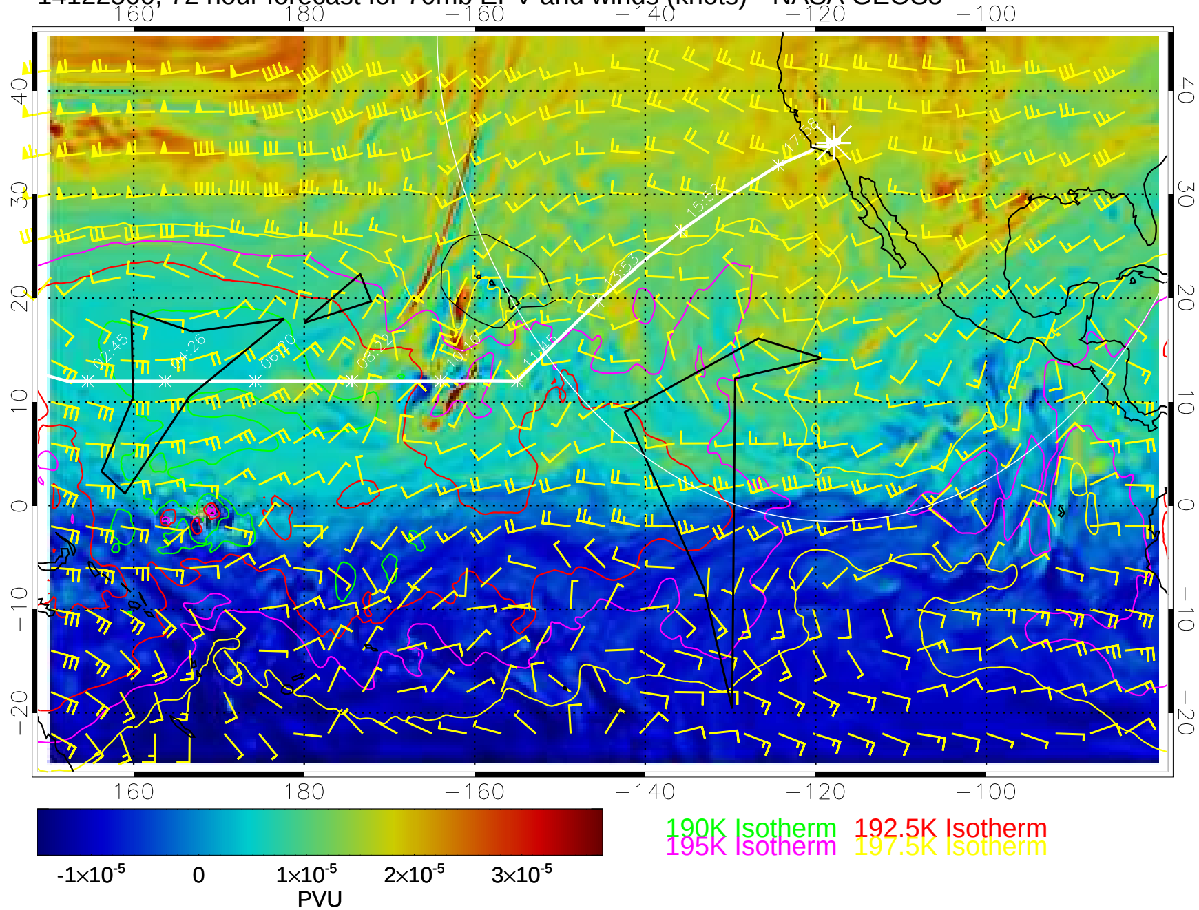
14122500, 72 hour forecast for 70mb EPV and winds (knots)-- NASA GEOS5
