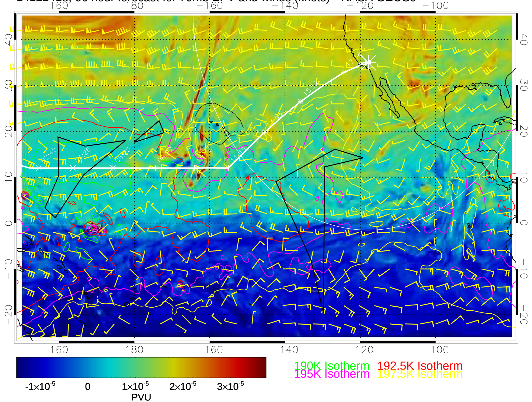
14122418, 66 hour forecast for 70mb EPV and winds (knots)-- NASA GEOS5
