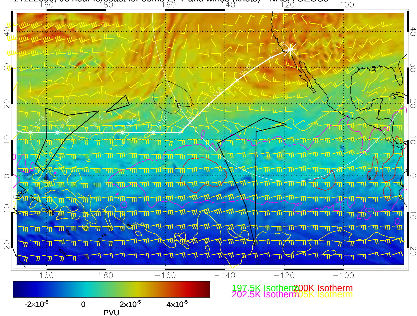
14122600, 96 hour forecast for 50mb EPV and winds (knots)-- NASA GEOS5
