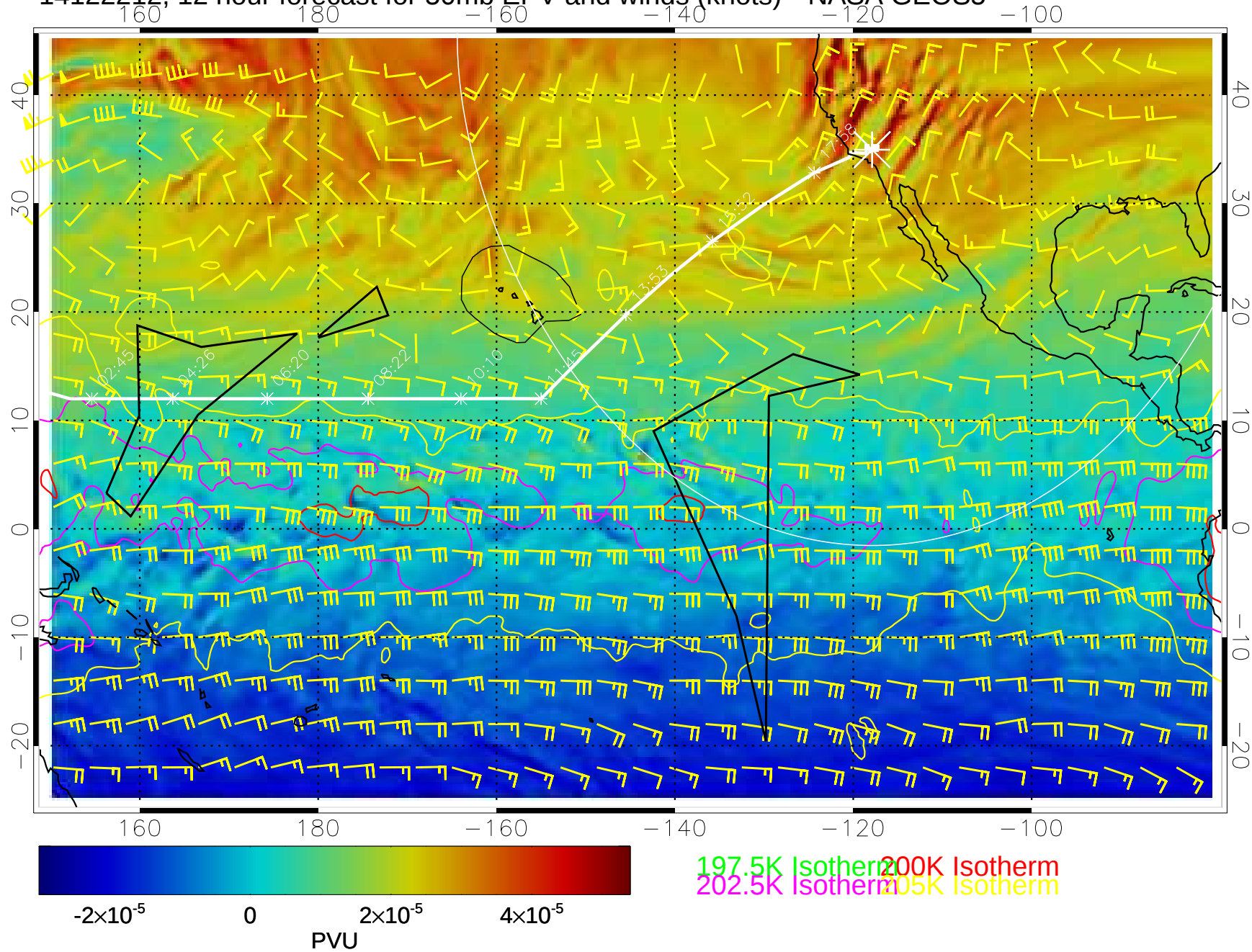
14122212, 12 hour forecast for 50mb EPV and winds (knots)-- NASA GEOS5
