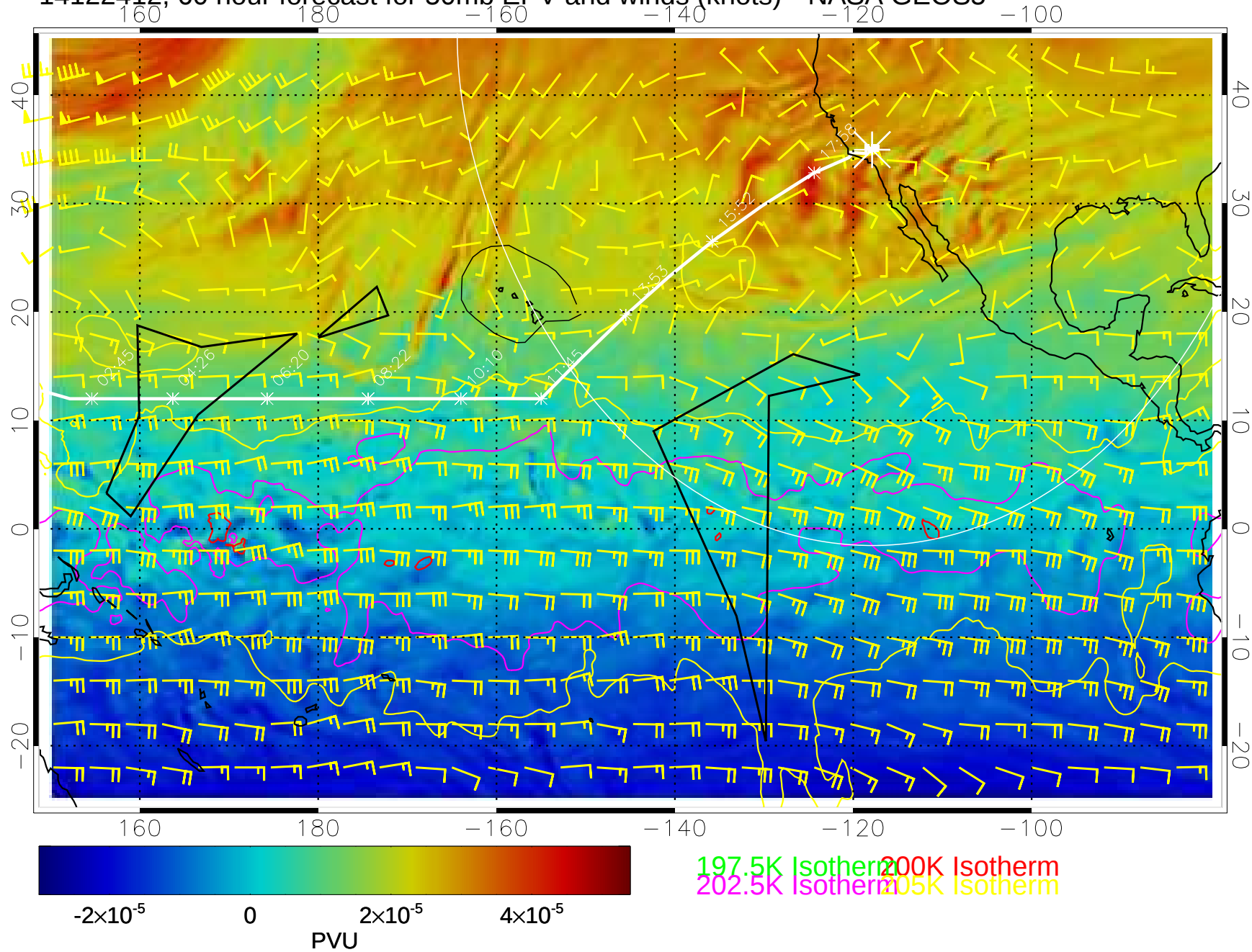
14122412, 60 hour forecast for 50mb EPV and winds (knots)-- NASA GEOS5
