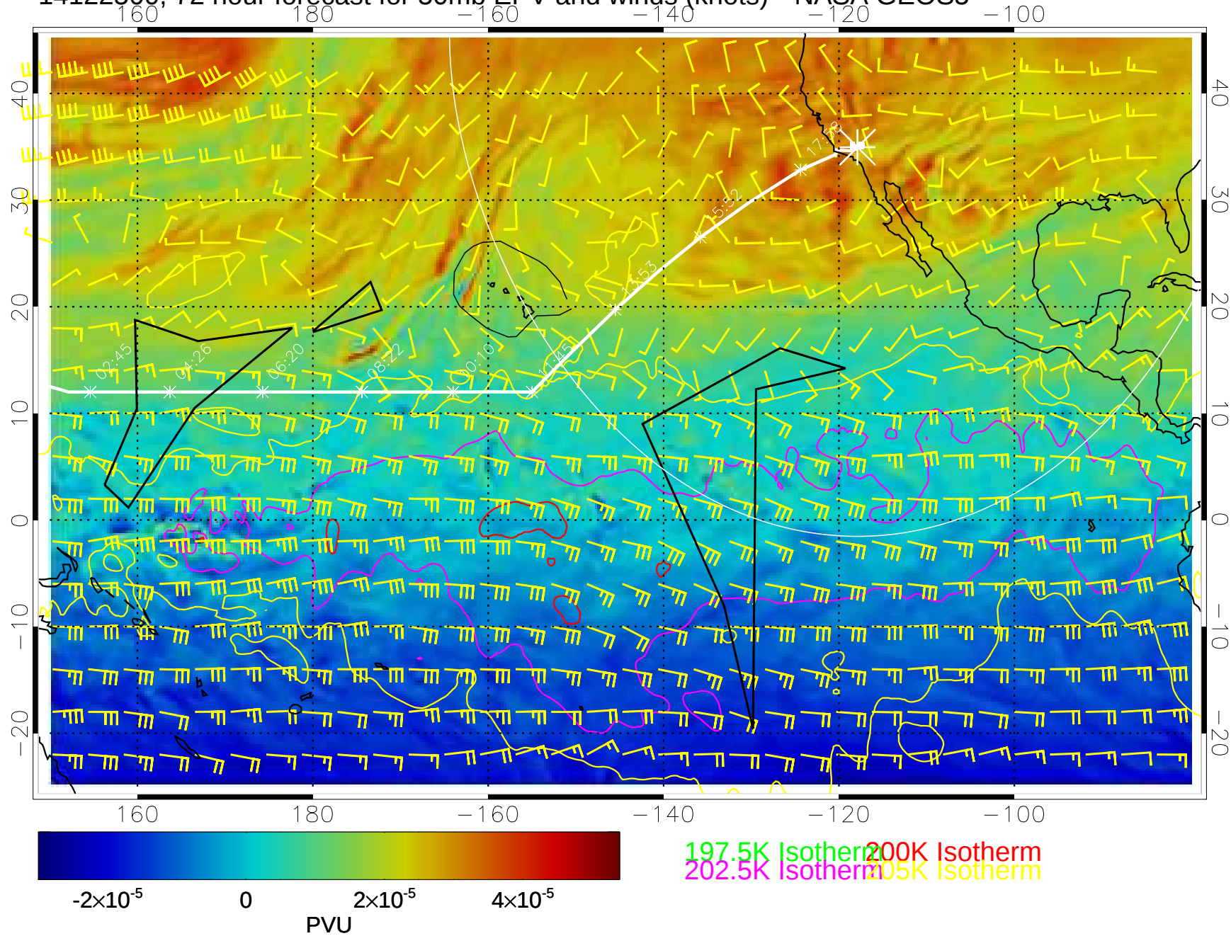
14122500, 72 hour forecast for 50mb EPV and winds (knots)-- NASA GEOS5
