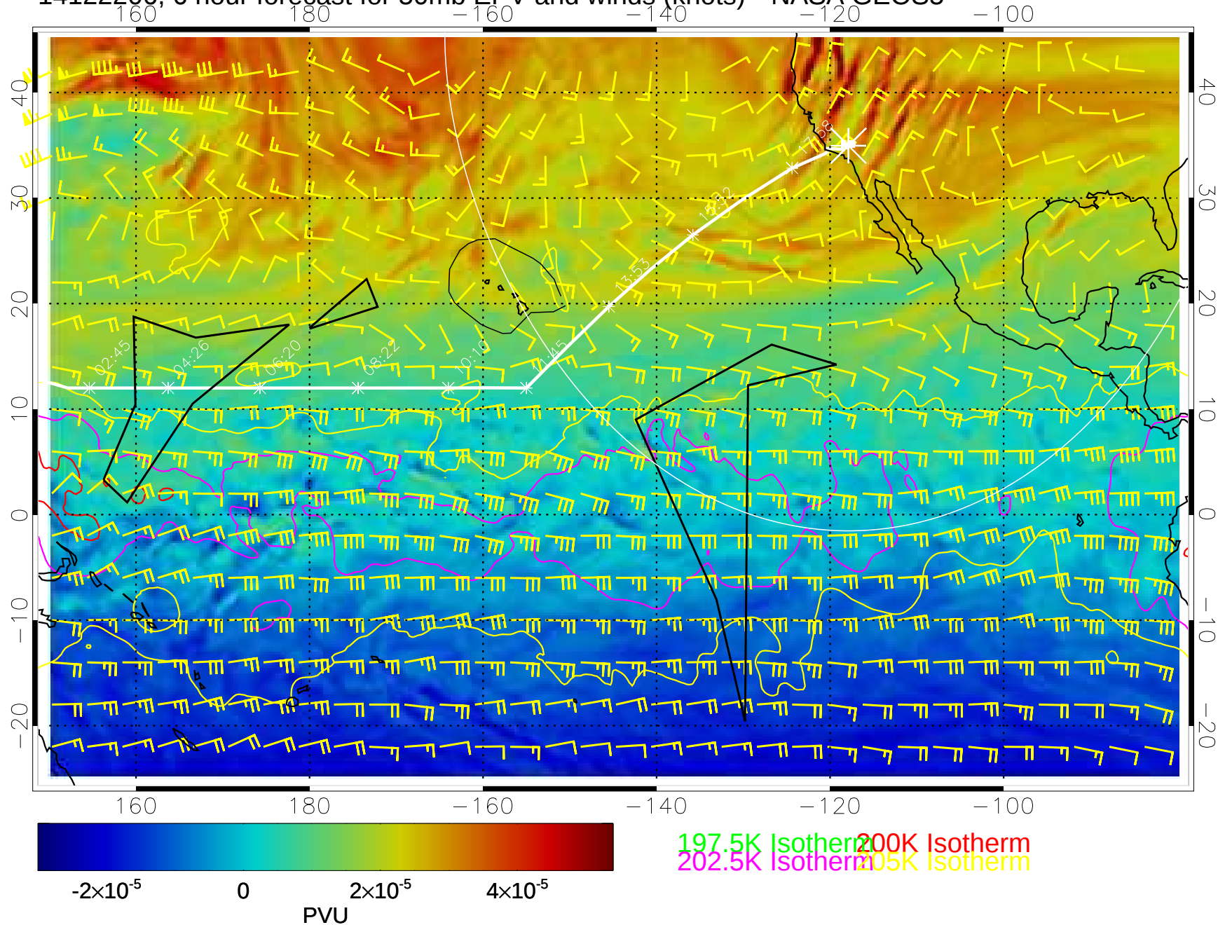
14122206, 6 hour forecast for 50mb EPV and winds (knots)-- NASA GEOS5
