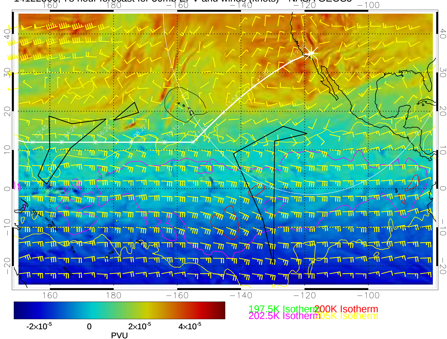
14122506, 78 hour forecast for 50mb EPV and winds (knots)-- NASA GEOS5
