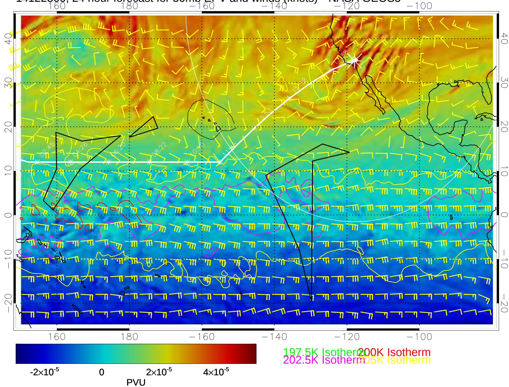
14122300, 24 hour forecast for 50mb EPV and winds (knots)-- NASA GEOS5
