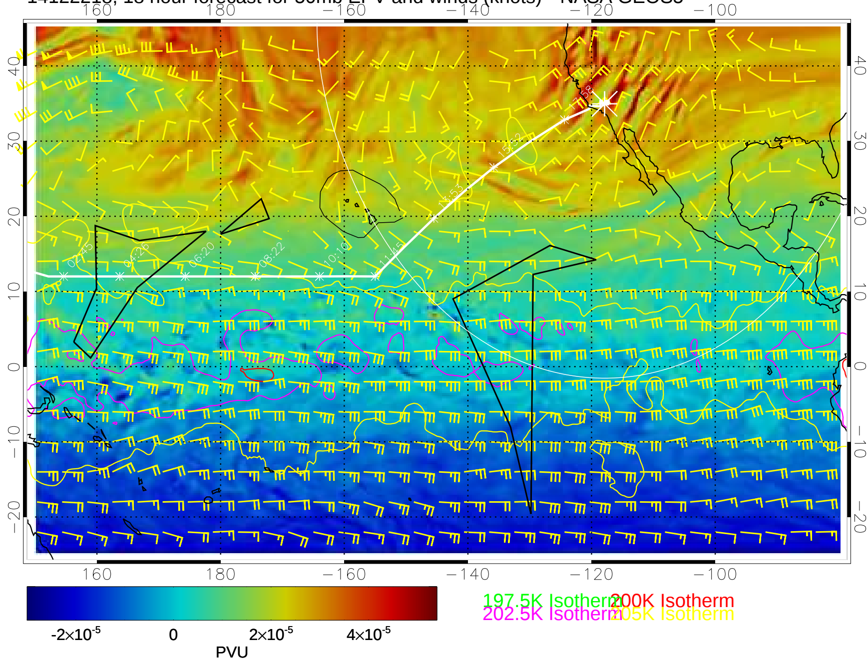
14122218, 18 hour forecast for 50mb EPV and winds (knots)-- NASA GEOS5
