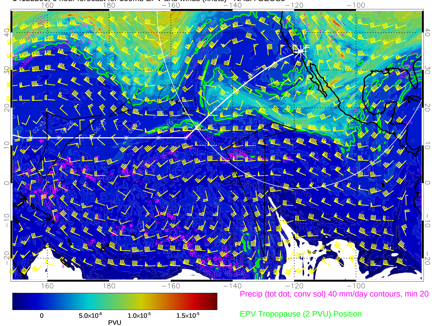
14122206, 6 hour forecast for 150mb EPV and winds (knots) - NASA GEOS5
