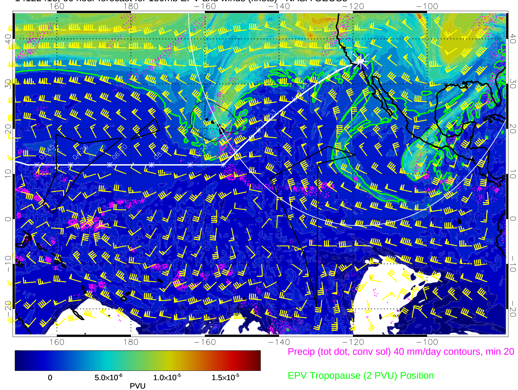
14122418, 66 hour forecast for 150mb EPV and winds (knots) - NASA GEOS5
