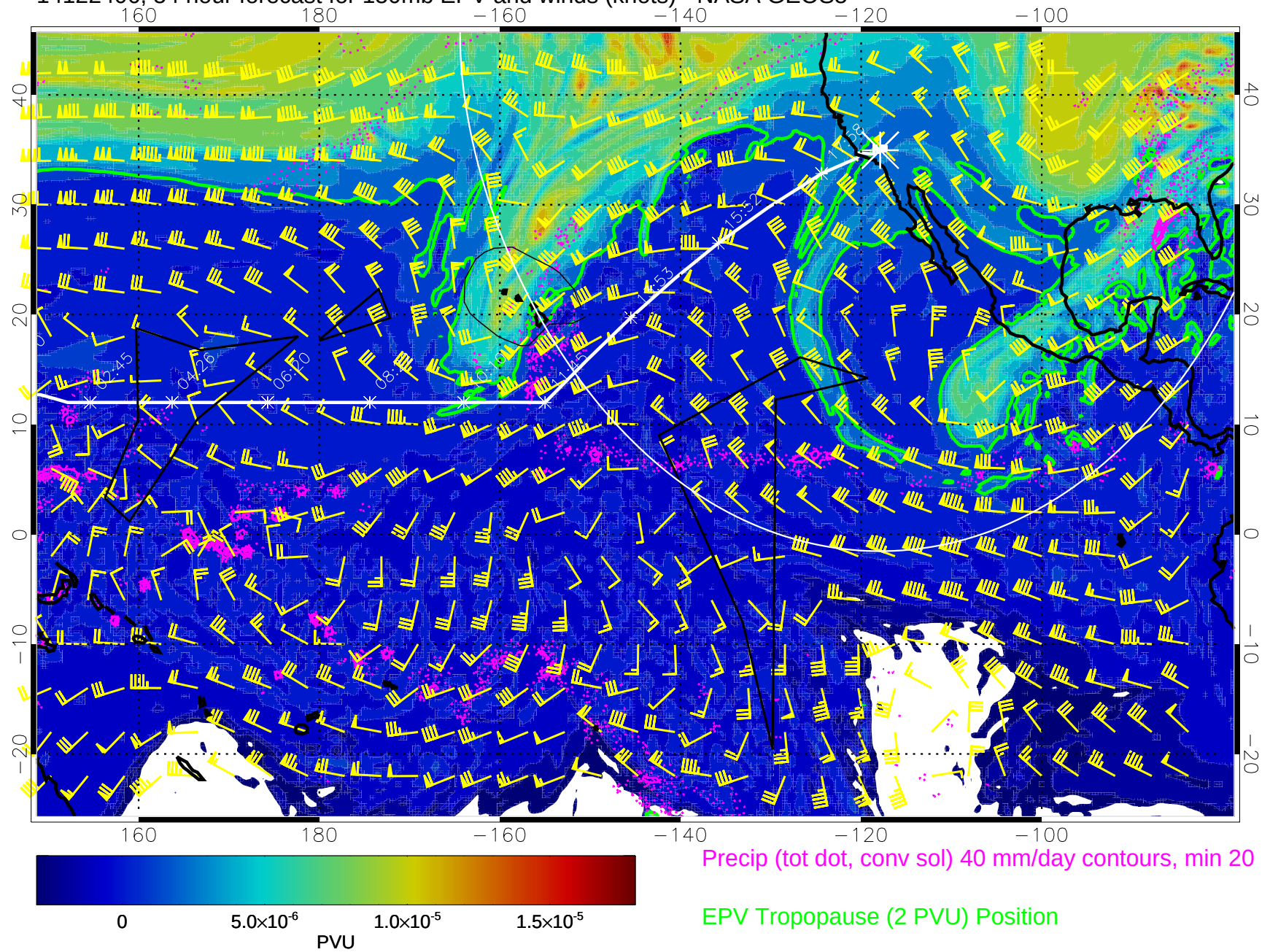
14122406, 54 hour forecast for 150mb EPV and winds (knots) - NASA GEOS5
