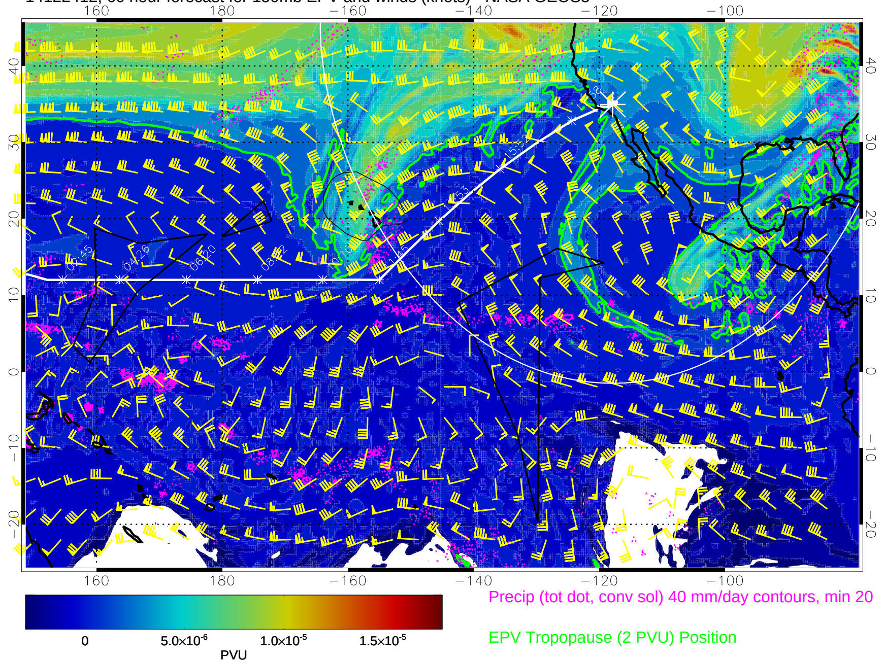
14122412, 60 hour forecast for 150mb EPV and winds (knots) - NASA GEOS5
