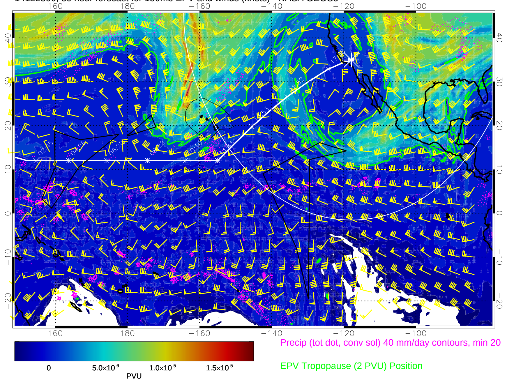
14122306, 30 hour forecast for 150mb EPV and winds (knots) - NASA GEOS5
