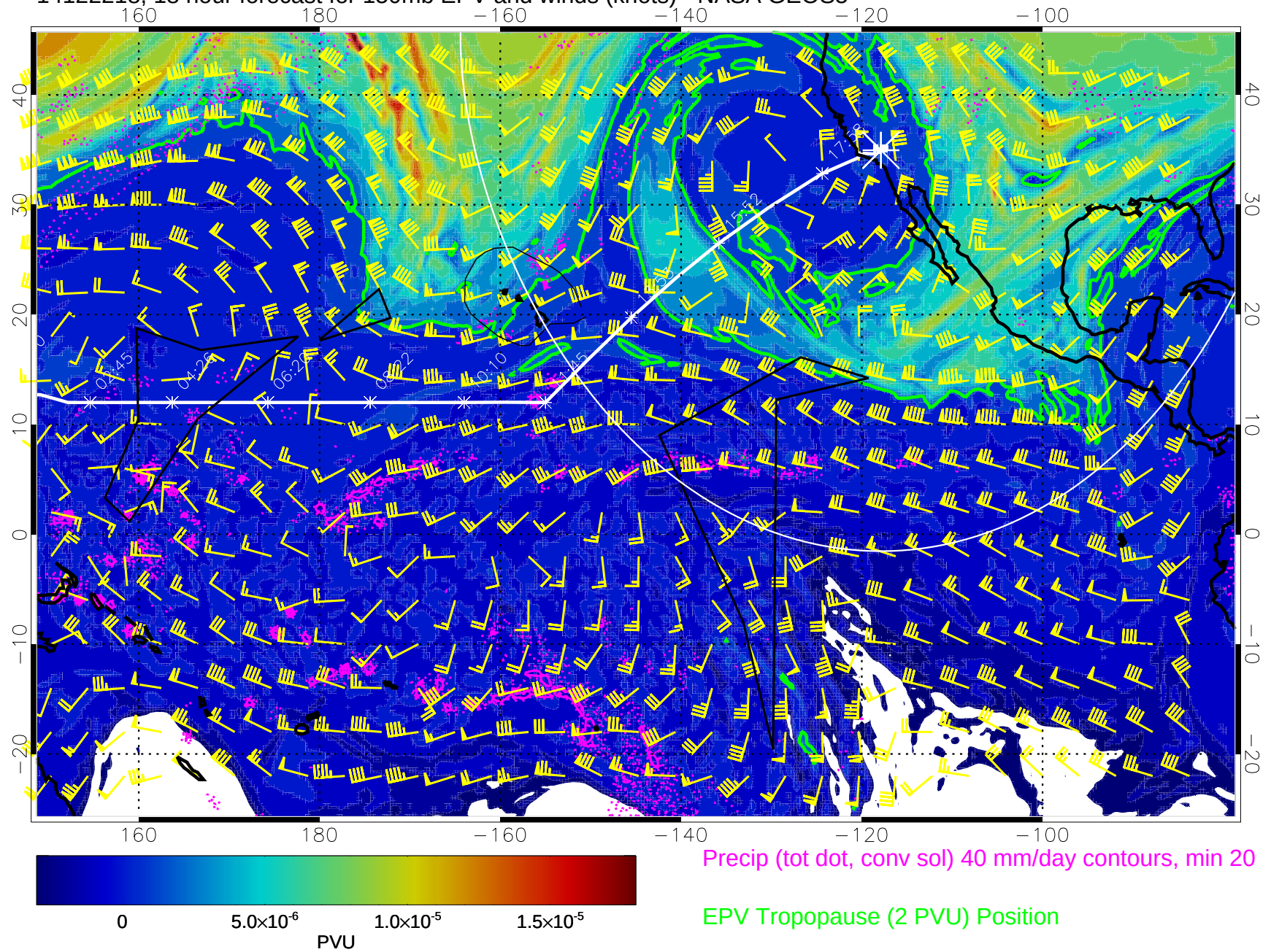
14122218, 18 hour forecast for 150mb EPV and winds (knots) - NASA GEOS5
