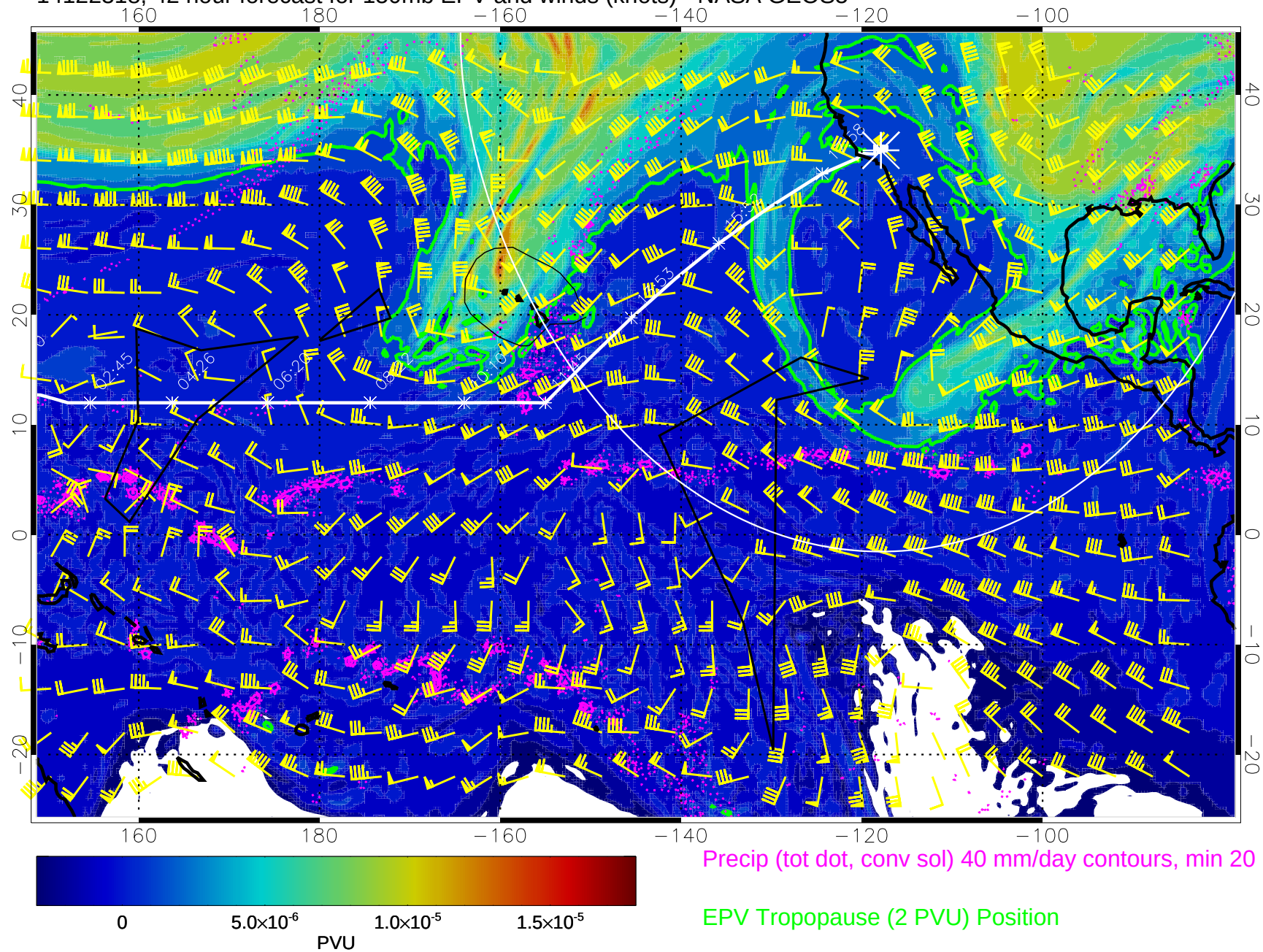
14122318, 42 hour forecast for 150mb EPV and winds (knots) - NASA GEOS5
