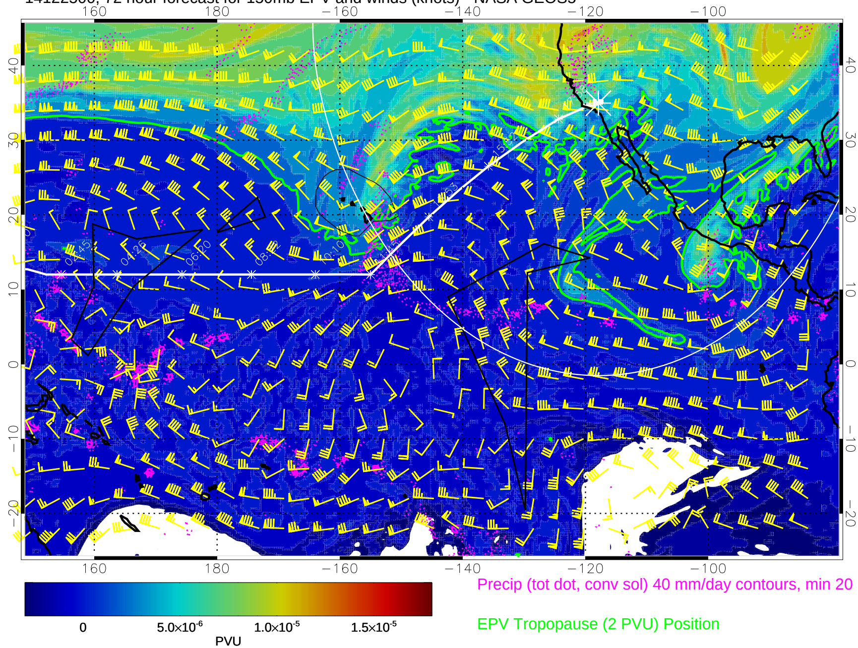
14122500, 72 hour forecast for 150mb EPV and winds (knots) - NASA GEOS5
