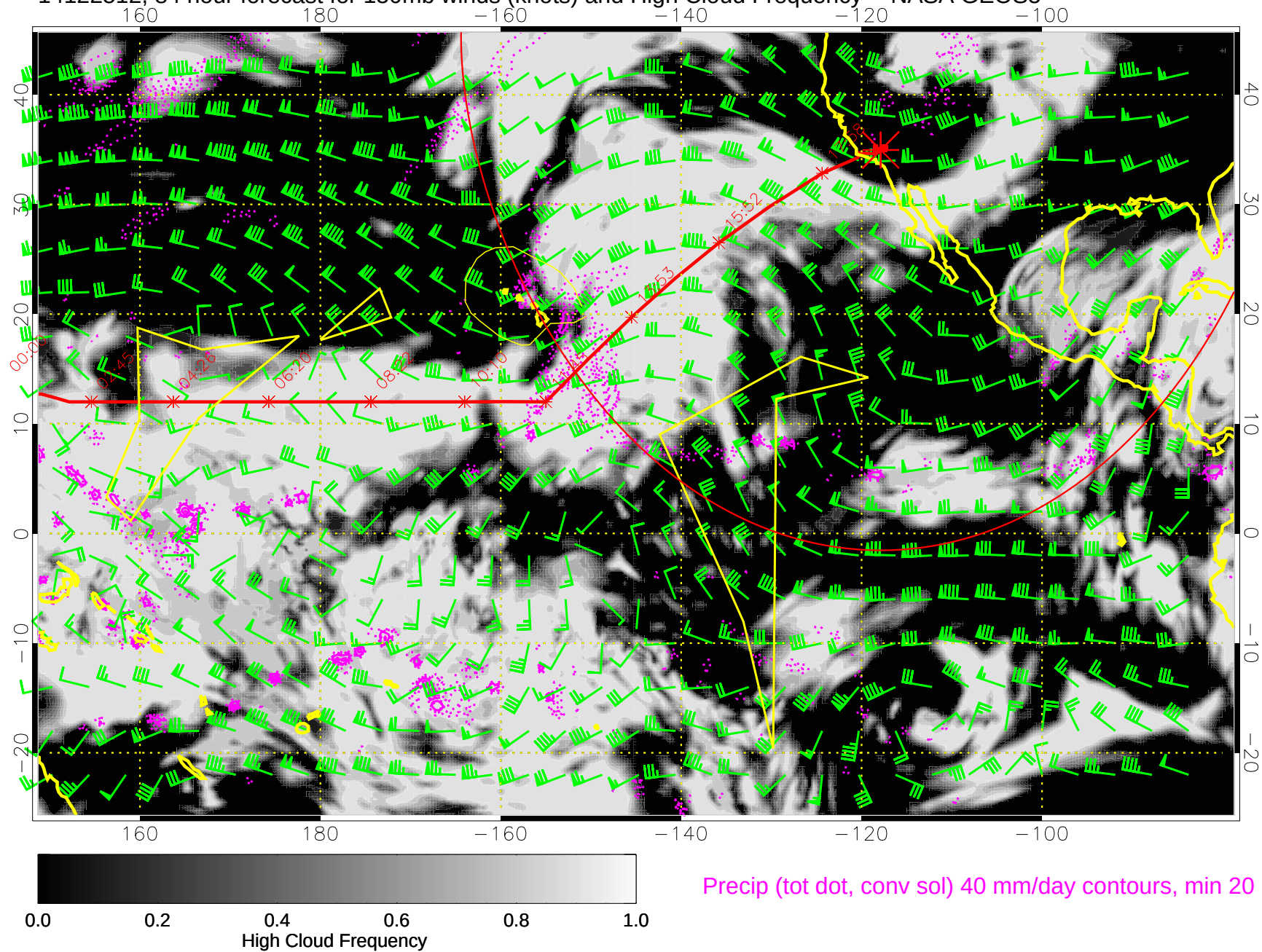
14122512, 84 hour forecast for 150mb winds (knots) and High Cloud Frequency -- NASA GEOS5
