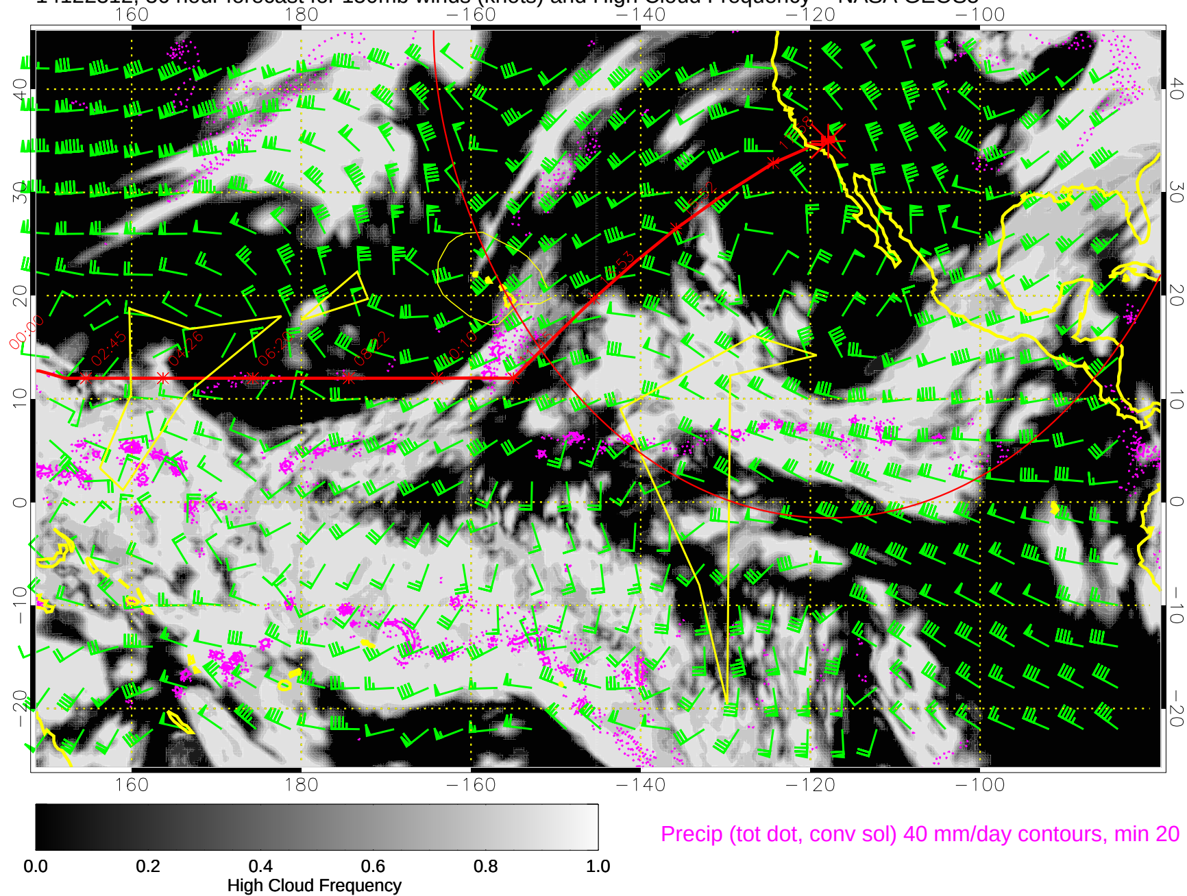
14122312, 36 hour forecast for 150mb winds (knots) and High Cloud Frequency -- NASA GEOS5
