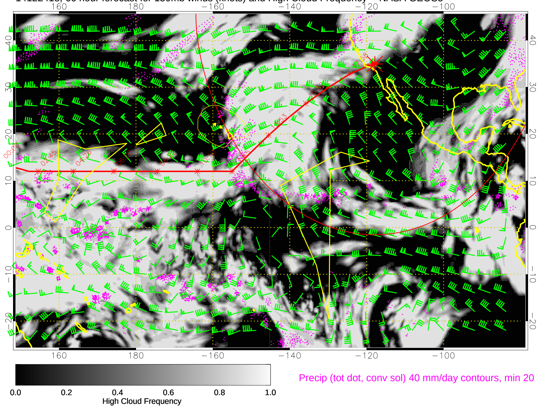
14122418, 66 hour forecast for 150mb winds (knots) and High Cloud Frequency -- NASA GEOS5
