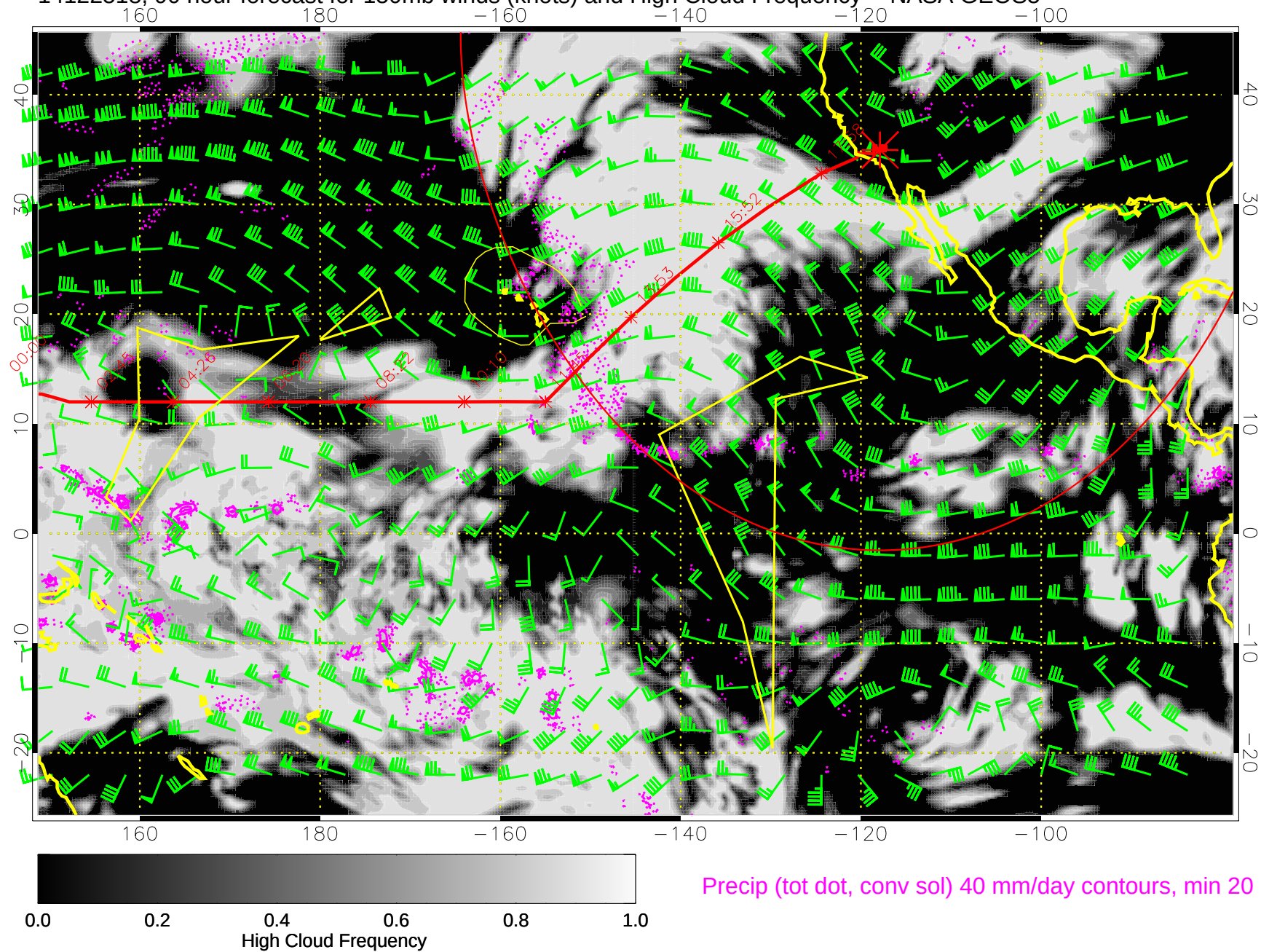
14122518, 90 hour forecast for 150mb winds (knots) and High Cloud Frequency -- NASA GEOS5
