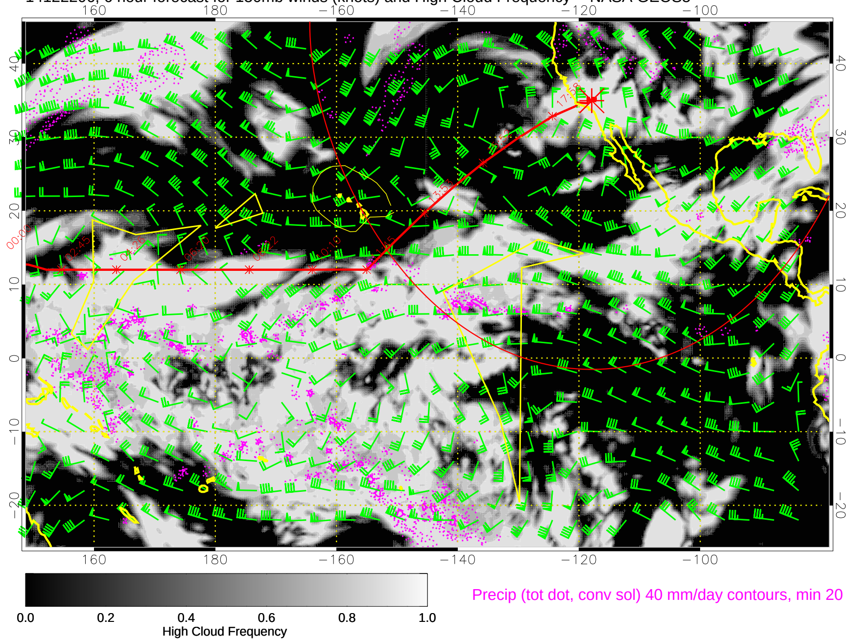
14122206, 6 hour forecast for 150mb winds (knots) and High Cloud Frequency -- NASA GEOS5
