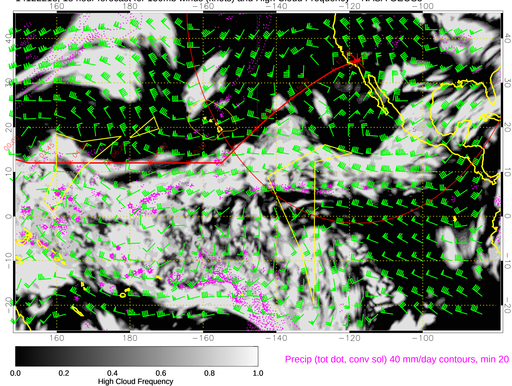
14122218, 18 hour forecast for 150mb winds (knots) and High Cloud Frequency -- NASA GEOS5
