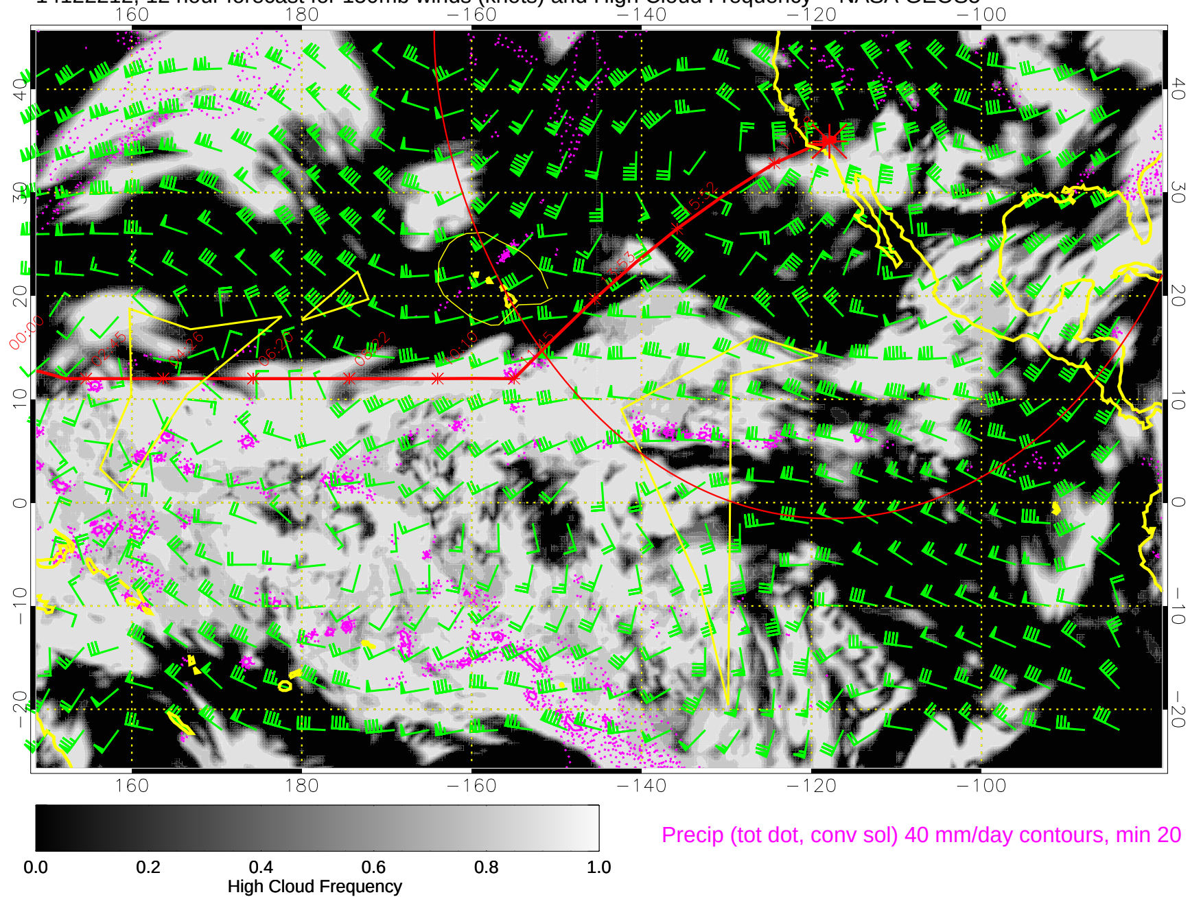
14122212, 12 hour forecast for 150mb winds (knots) and High Cloud Frequency -- NASA GEOS5
