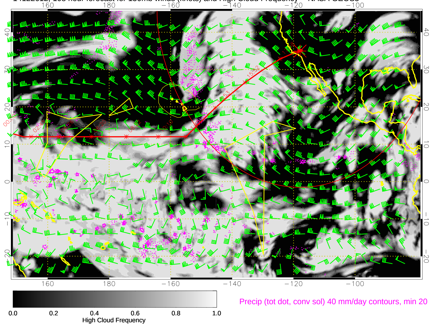
14122612, 108 hour forecast for 150mb winds (knots) and High Cloud Frequency -- NASA GEOS5
