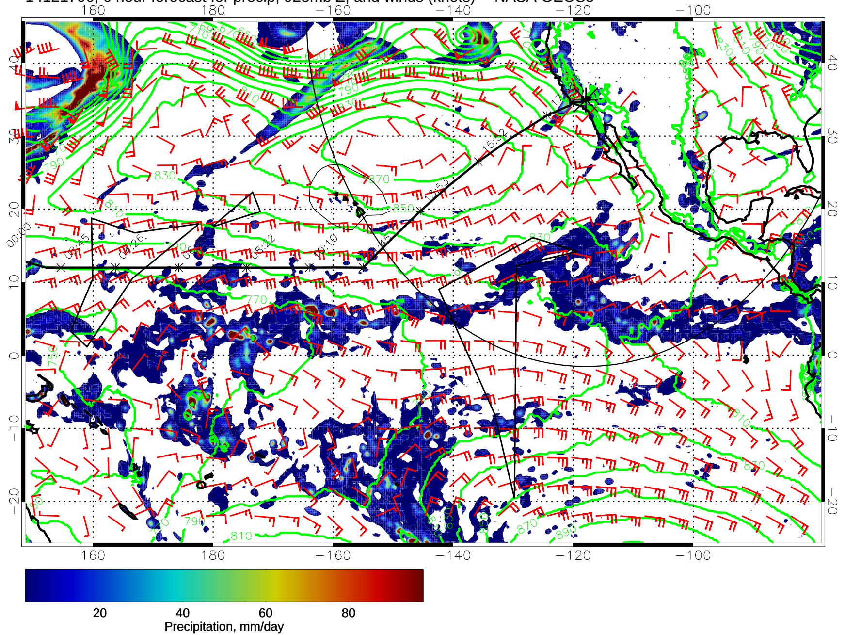
14121706, 6 hour forecast for precip, 925mb Z, and winds (knots) -- NASA GEOS5
