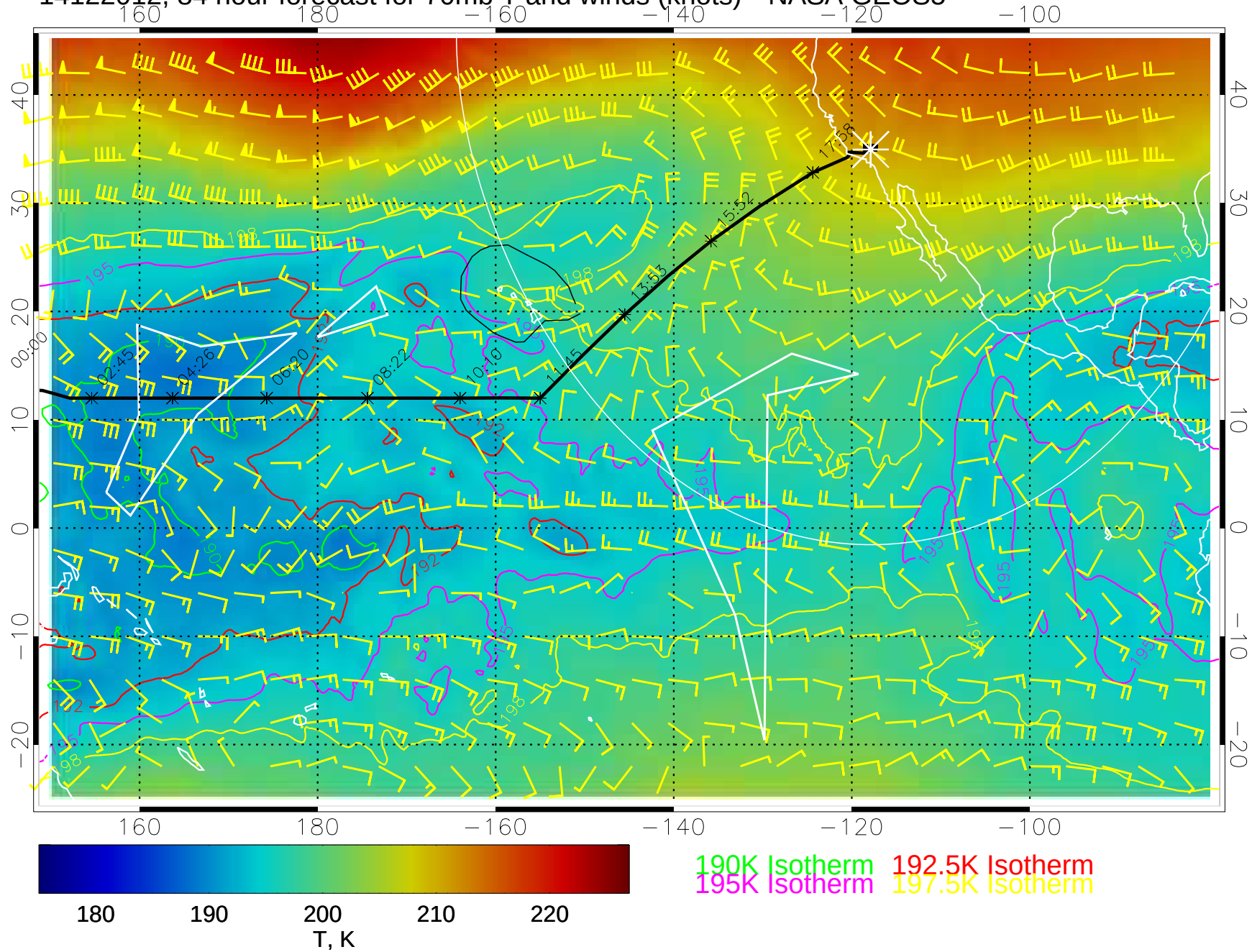
14122012, 84 hour forecast for 70mb T and winds (knots)-- NASA GEOS5
