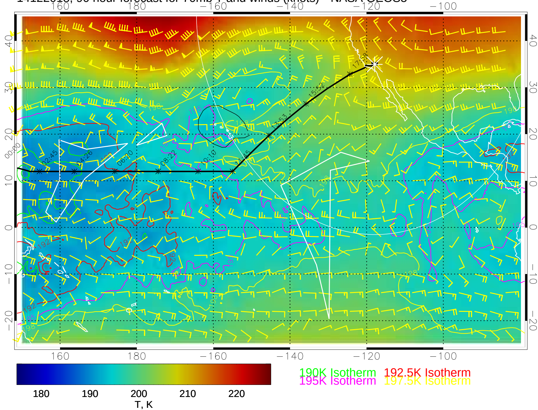
14122018, 90 hour forecast for 70mb T and winds (knots)-- NASA GEOS5
