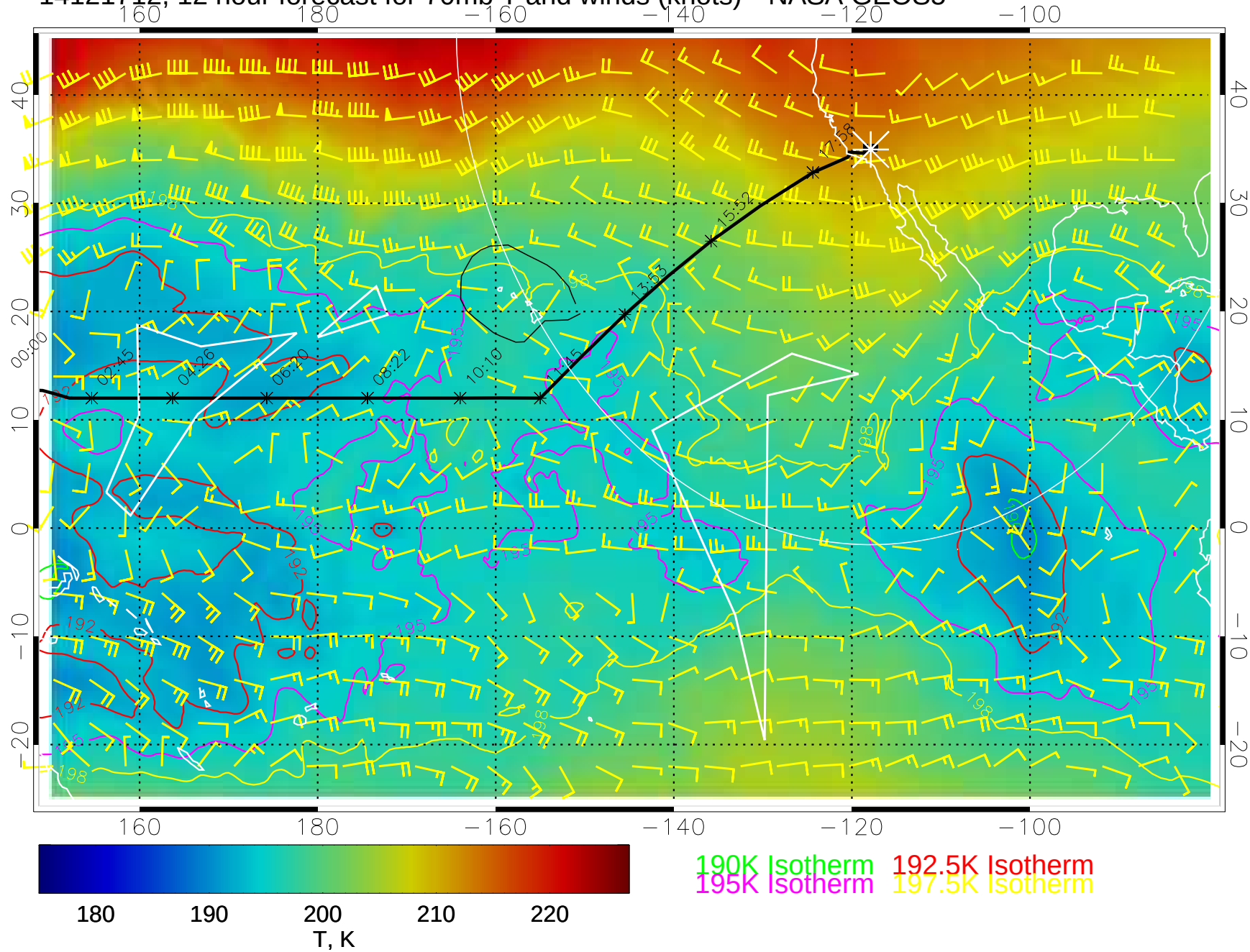
14121712, 12 hour forecast for 70mb T and winds (knots)-- NASA GEOS5
