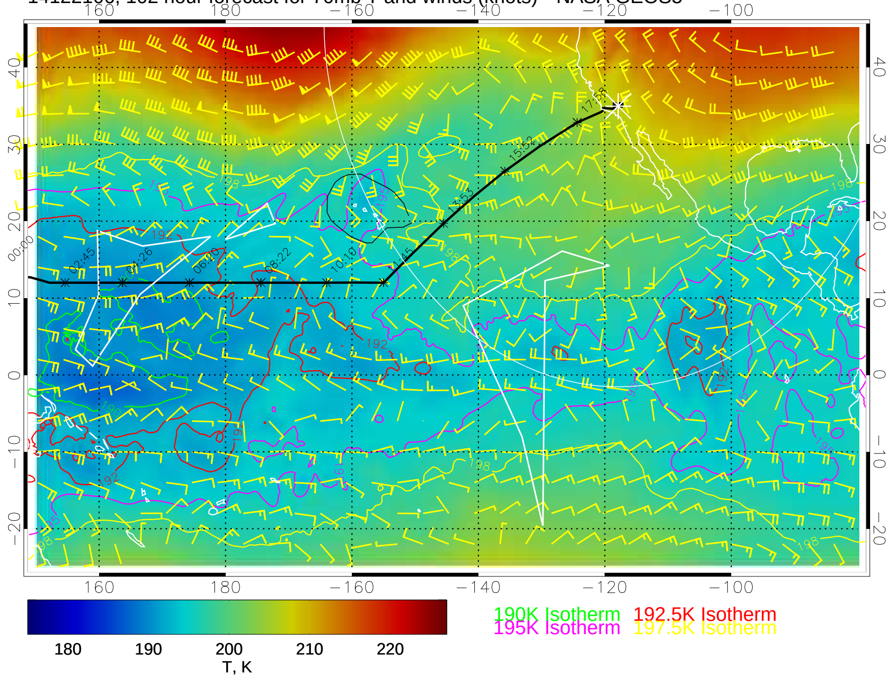
14122106, 102 hour forecast for 70mb T and winds (knots)-- NASA GEOS5
