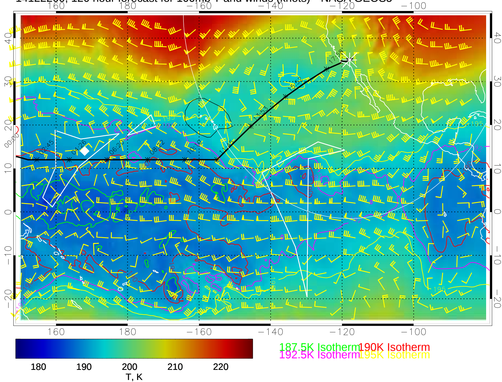
14122200, 120 hour forecast for 100mb T and winds (knots)-- NASA GEOS5
