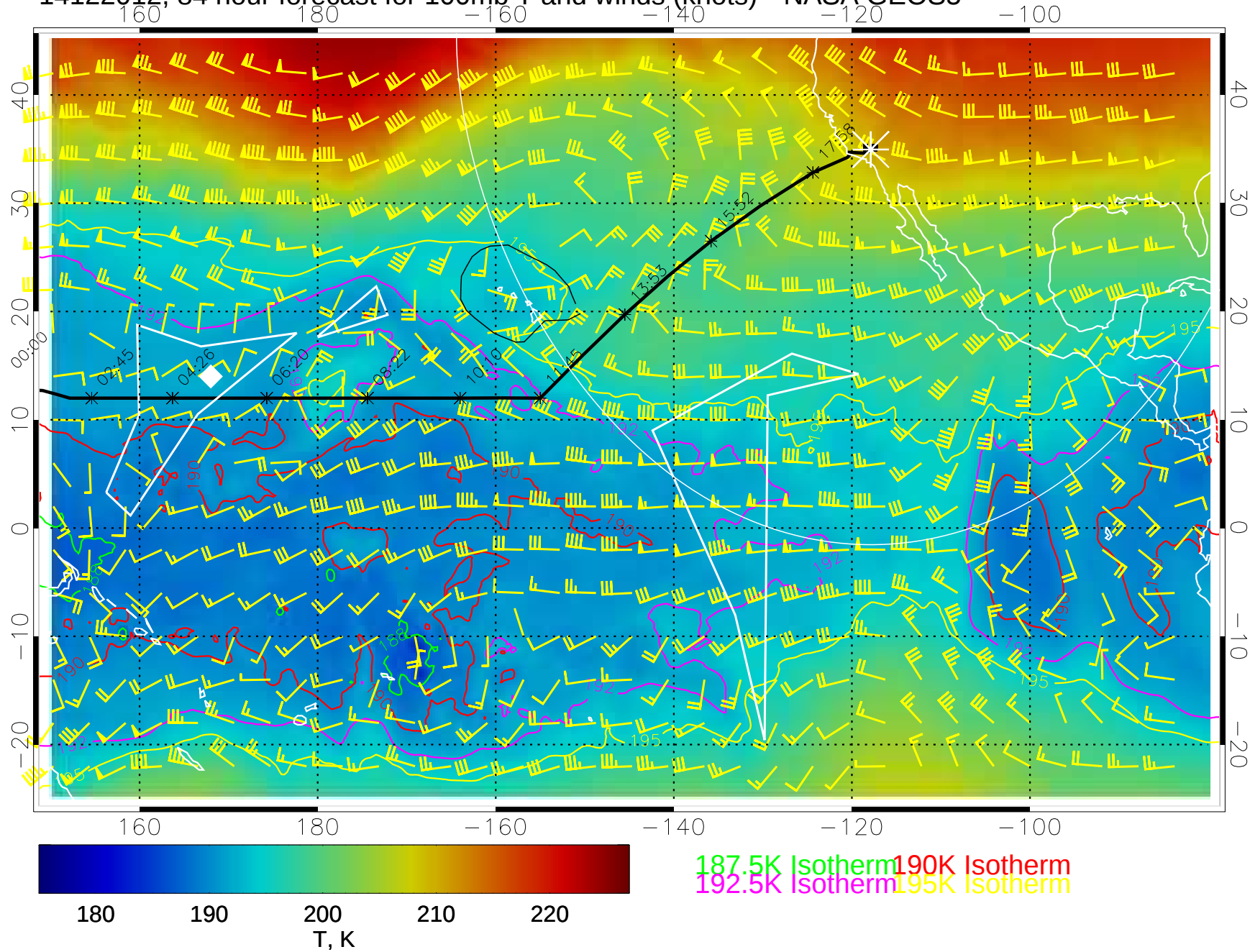
14122012, 84 hour forecast for 100mb T and winds (knots)-- NASA GEOS5
