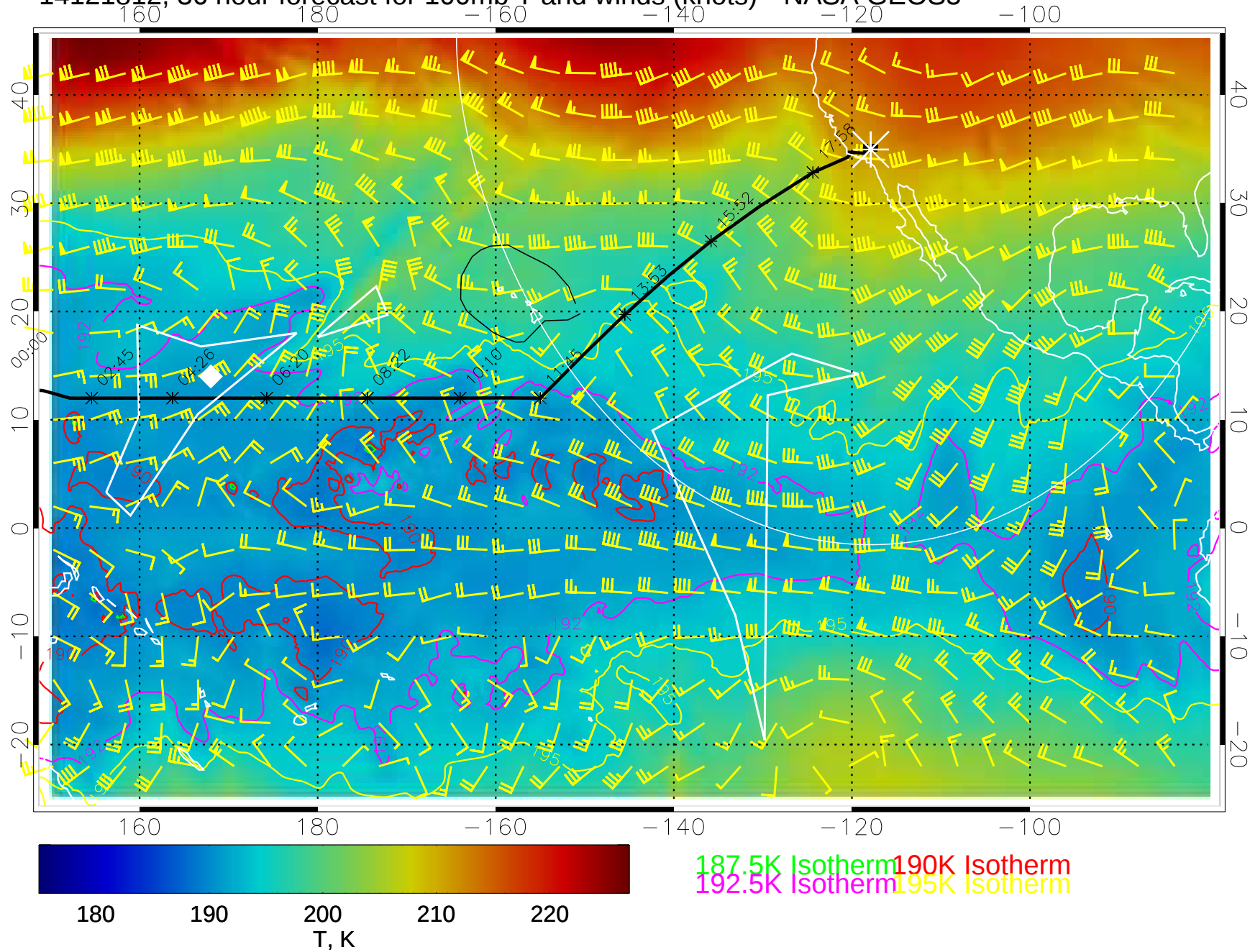
14121812, 36 hour forecast for 100mb T and winds (knots)-- NASA GEOS5
