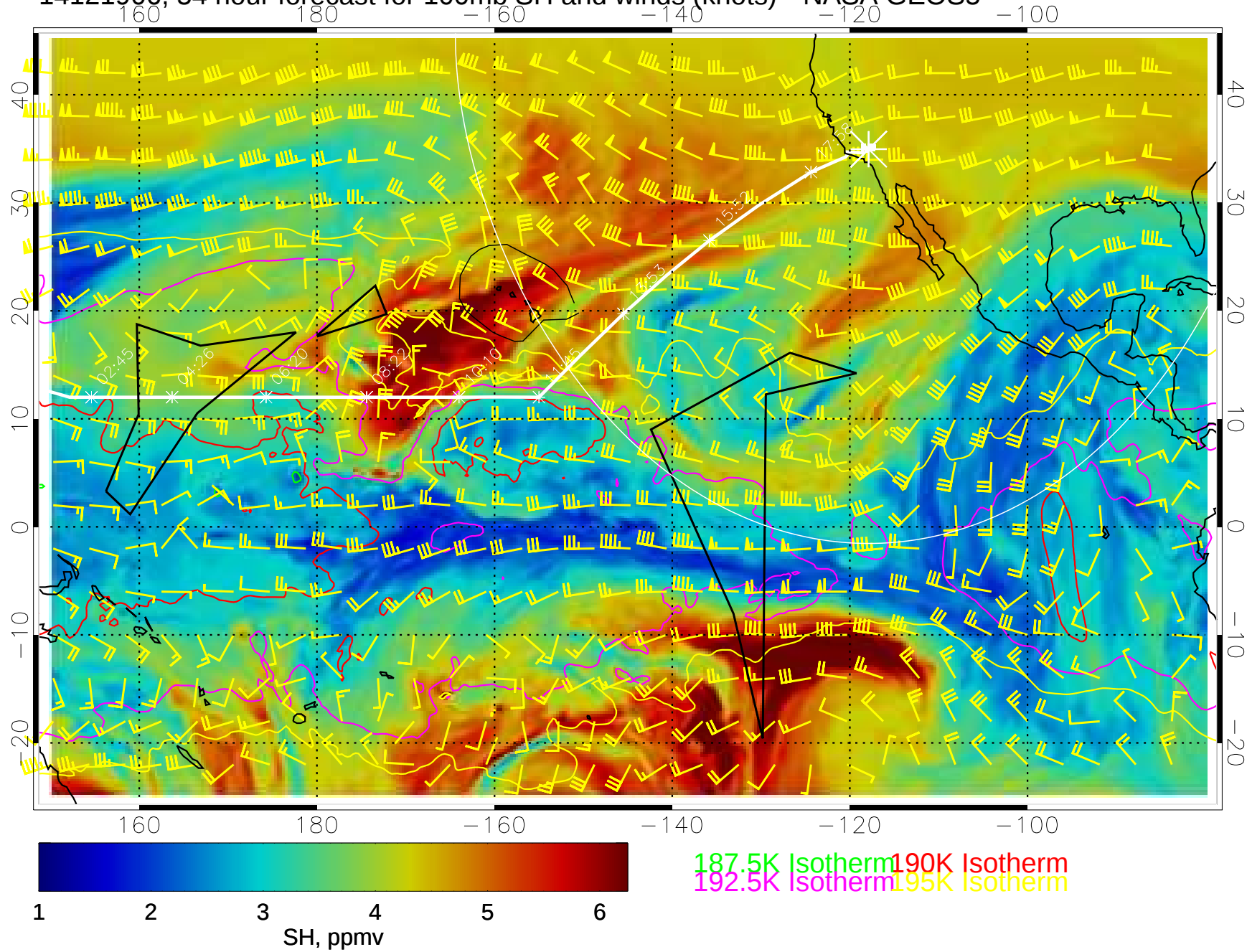
14121906, 54 hour forecast for 100mb SH and winds (knots)-- NASA GEOS5
