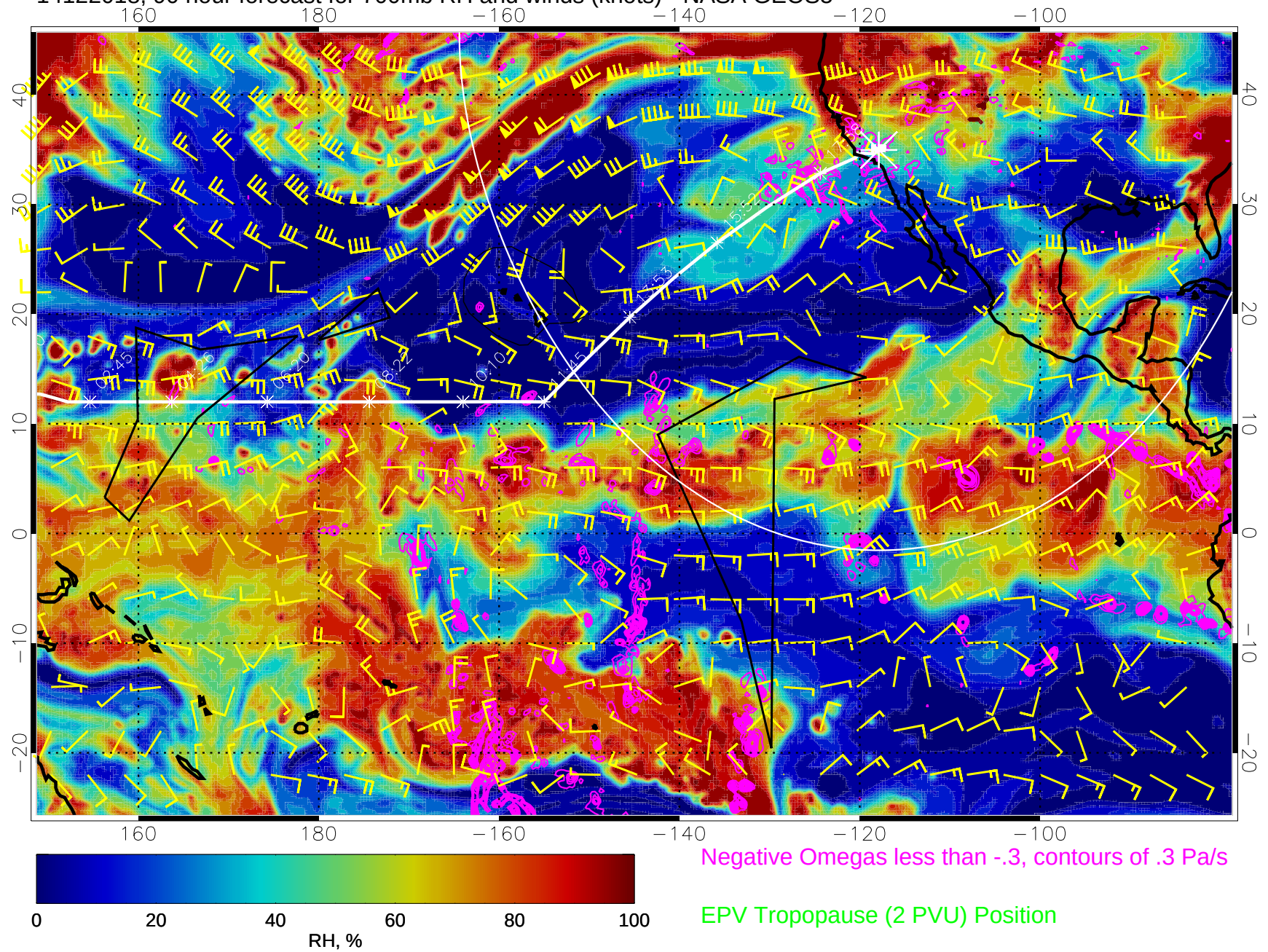
14122018, 90 hour forecast for 700mb RH and winds (knots) - NASA GEOS5
