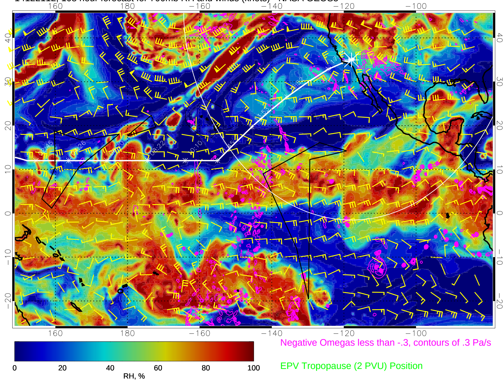
14122112, 108 hour forecast for 700mb RH and winds (knots) - NASA GEOS5
