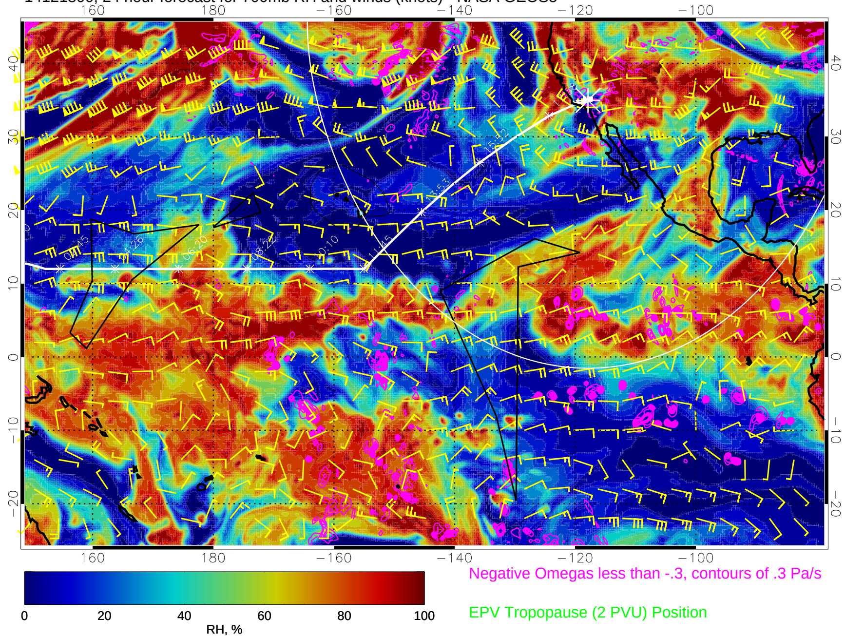
14121800, 24 hour forecast for 700mb RH and winds (knots) - NASA GEOS5
