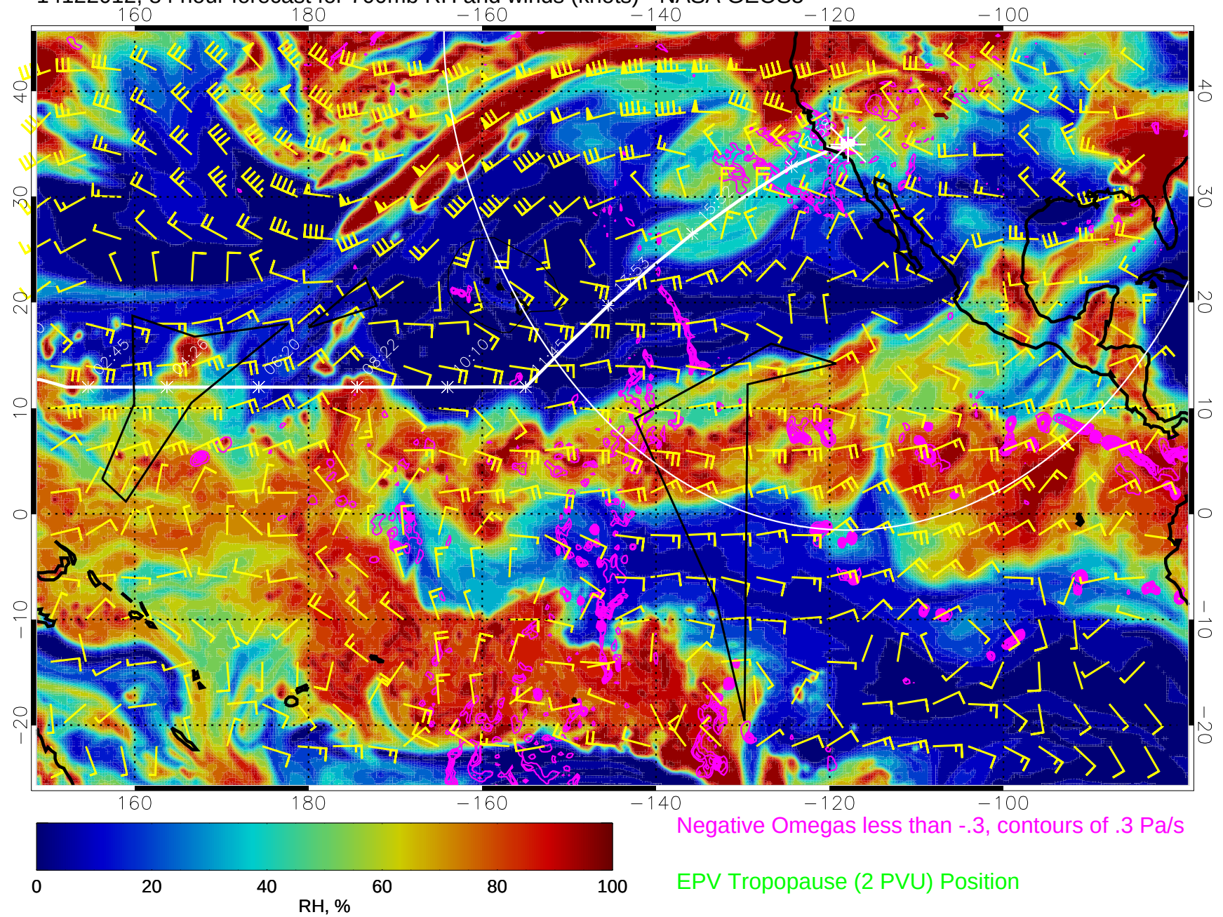
14122012, 84 hour forecast for 700mb RH and winds (knots) - NASA GEOS5
