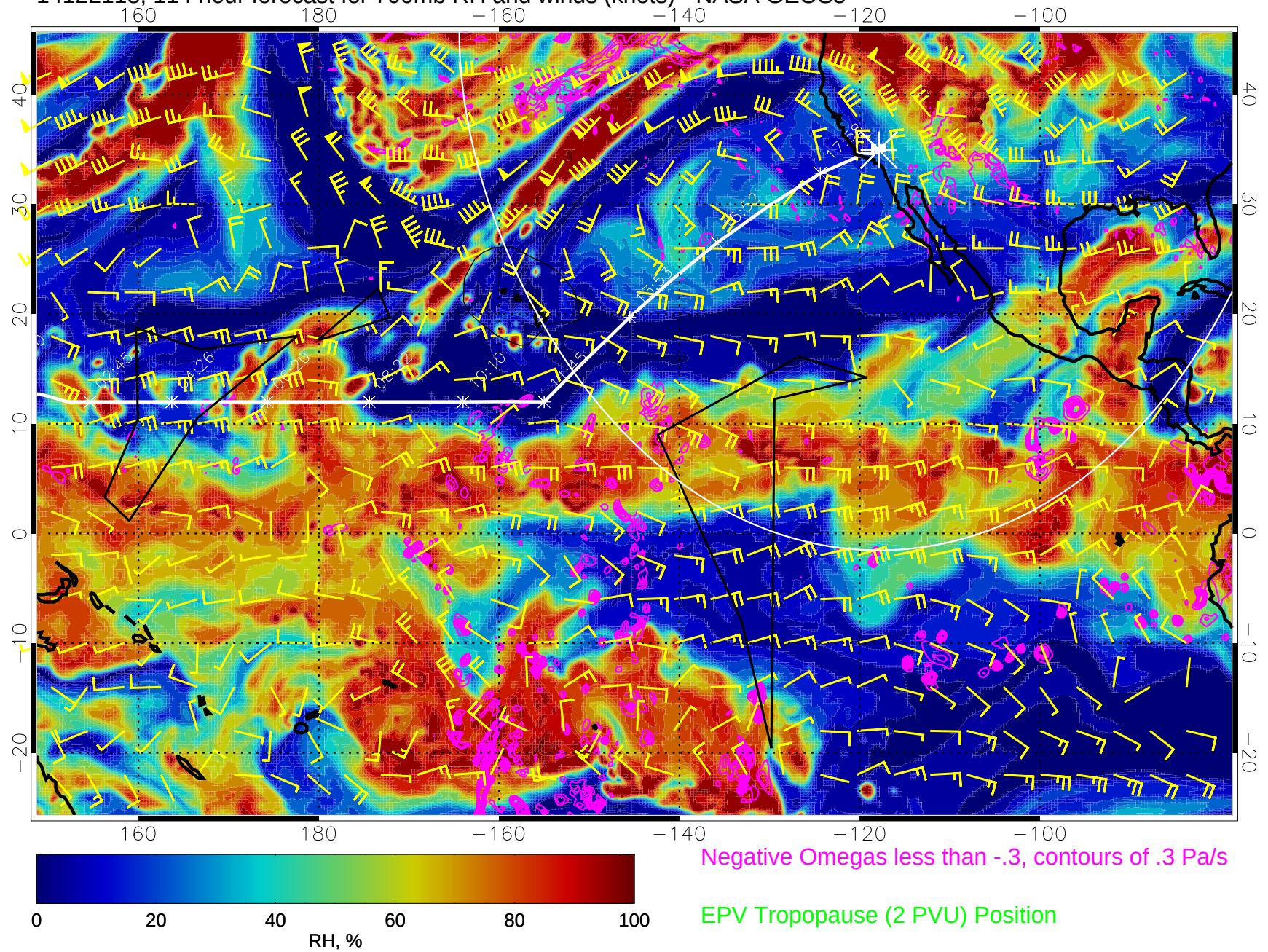
14122118, 114 hour forecast for 700mb RH and winds (knots) - NASA GEOS5
