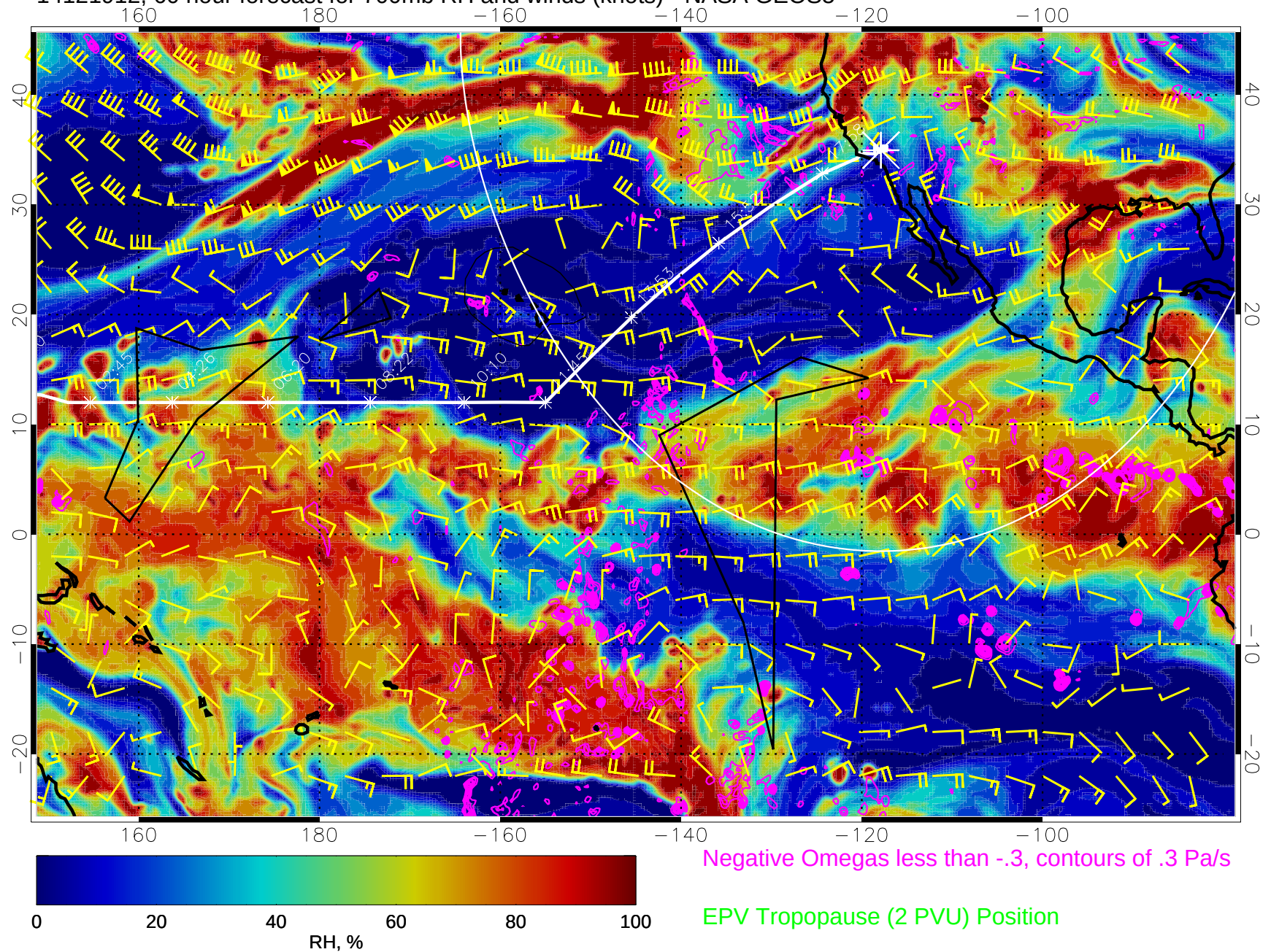
14121912, 60 hour forecast for 700mb RH and winds (knots) - NASA GEOS5
