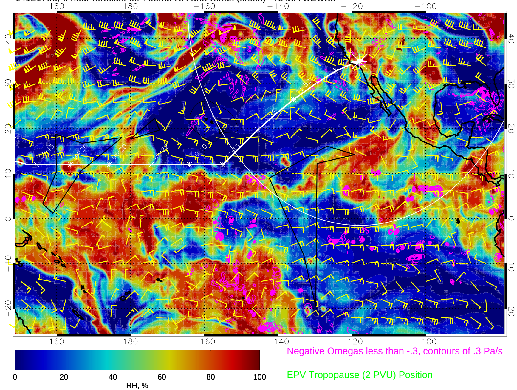
14121706, 6 hour forecast for 700mb RH and winds (knots) - NASA GEOS5
