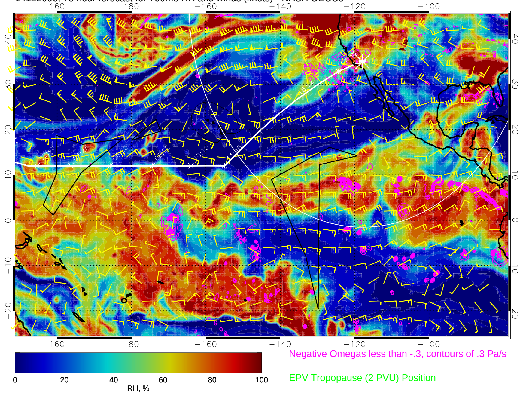
14122006, 78 hour forecast for 700mb RH and winds (knots) - NASA GEOS5
