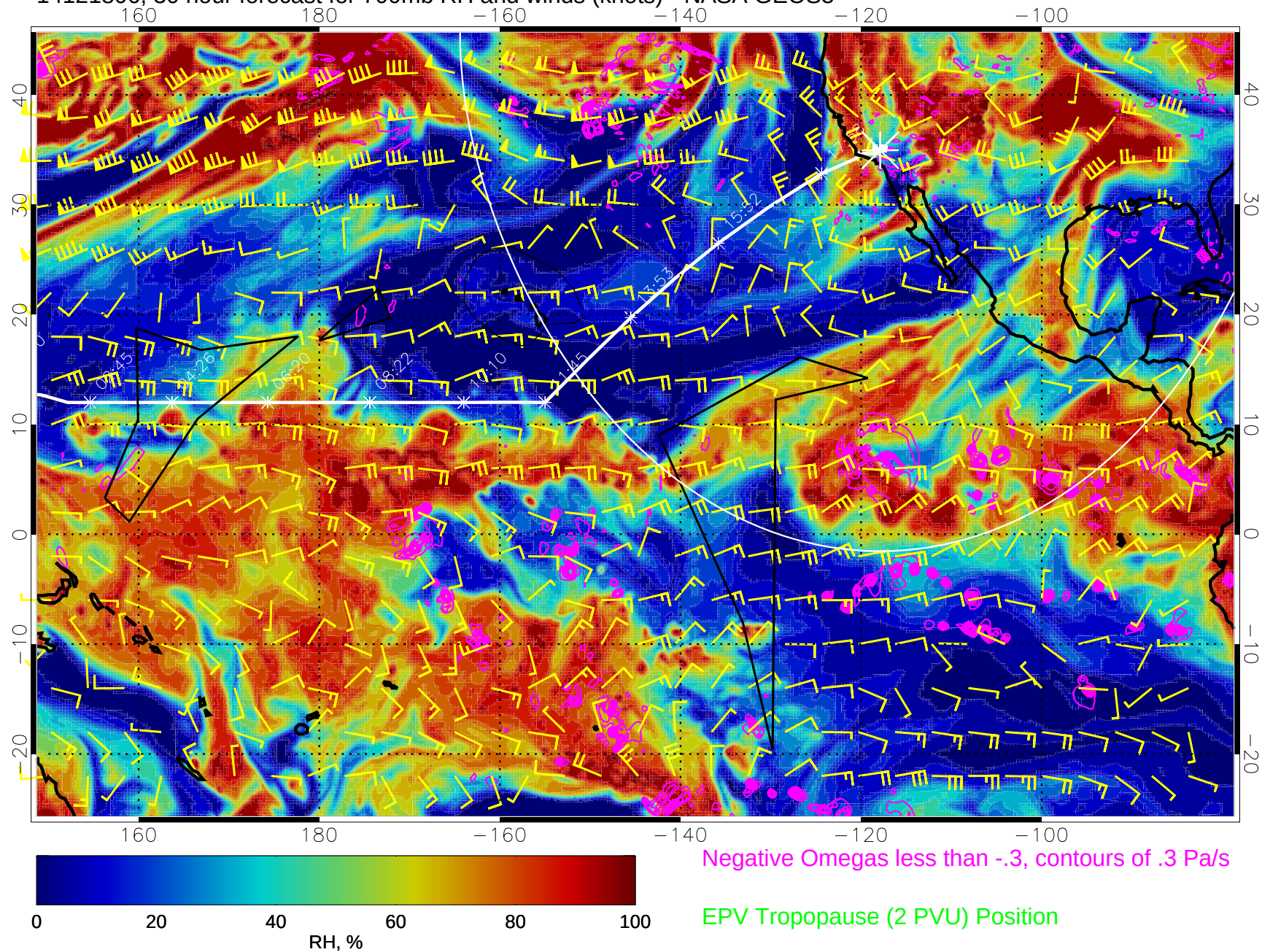
14121806, 30 hour forecast for 700mb RH and winds (knots) - NASA GEOS5
