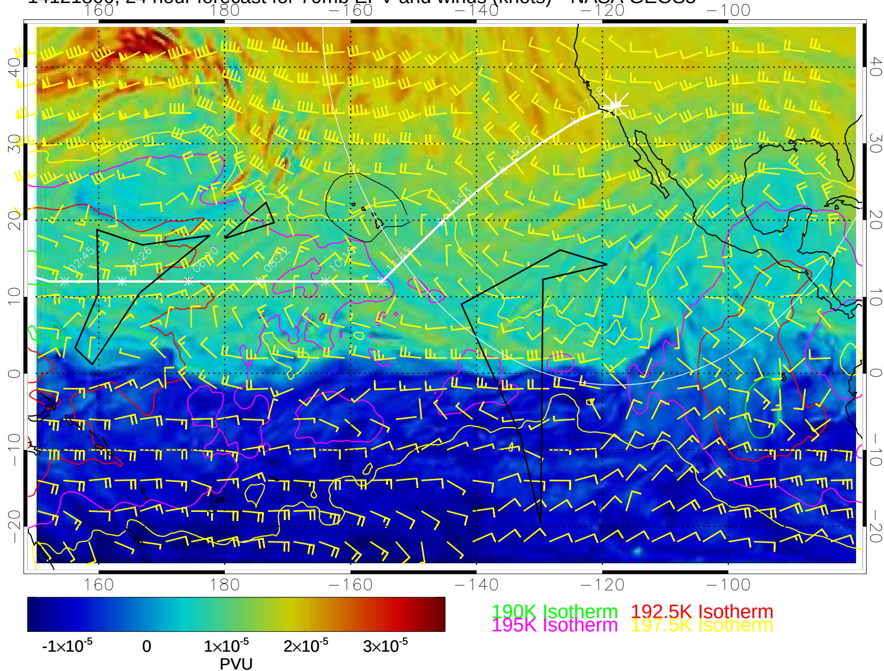
14121800, 24 hour forecast for 70mb EPV and winds (knots)-- NASA GEOS5
