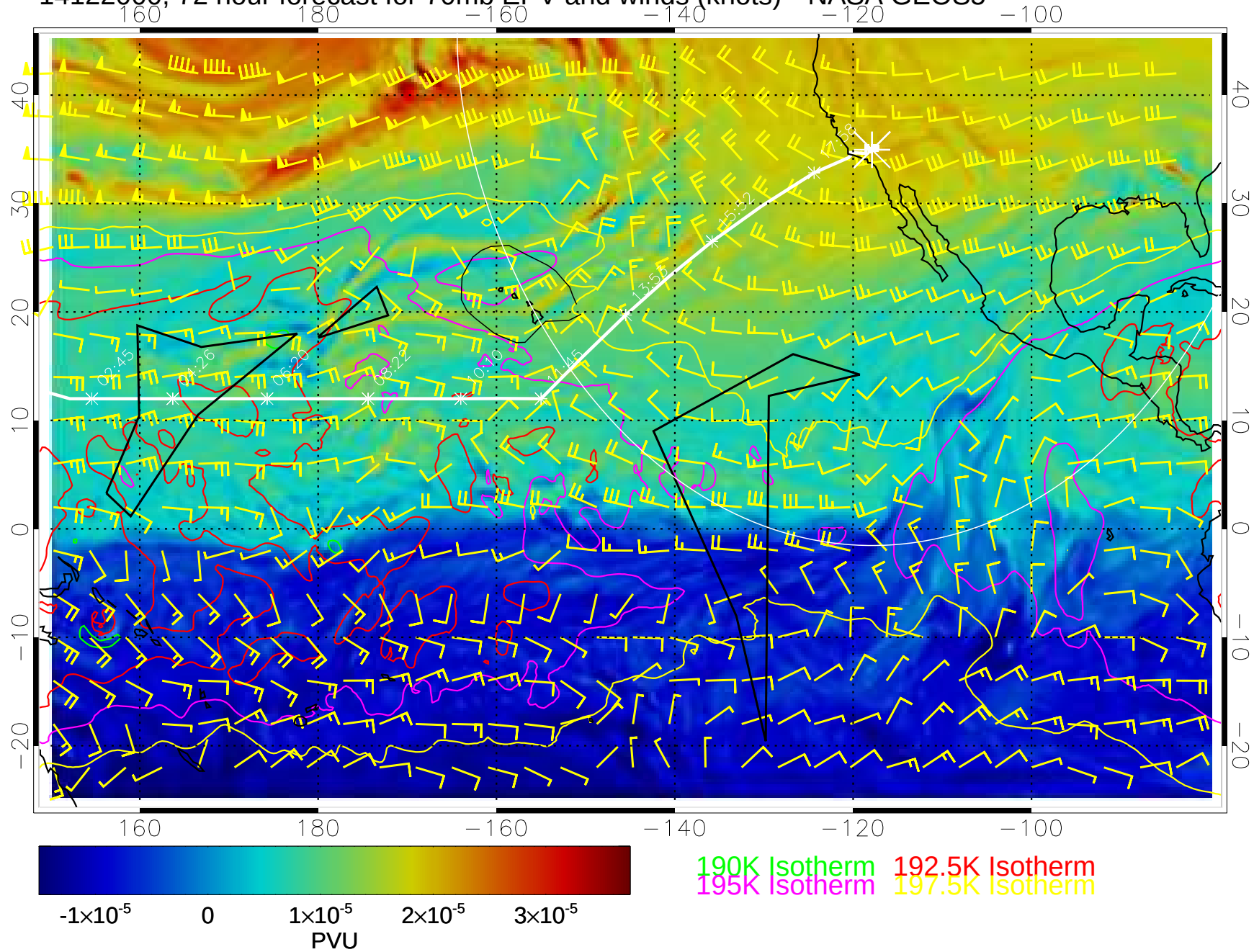
14122000, 72 hour forecast for 70mb EPV and winds (knots)-- NASA GEOS5
