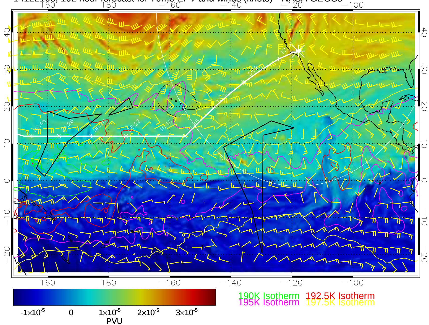
14122106, 102 hour forecast for 70mb EPV and winds (knots)-- NASA GEOS5
