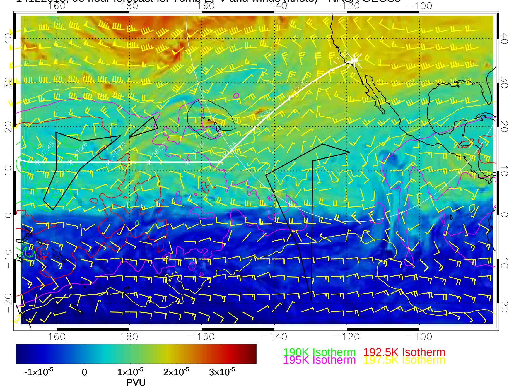
14122018, 90 hour forecast for 70mb EPV and winds (knots)-- NASA GEOS5
