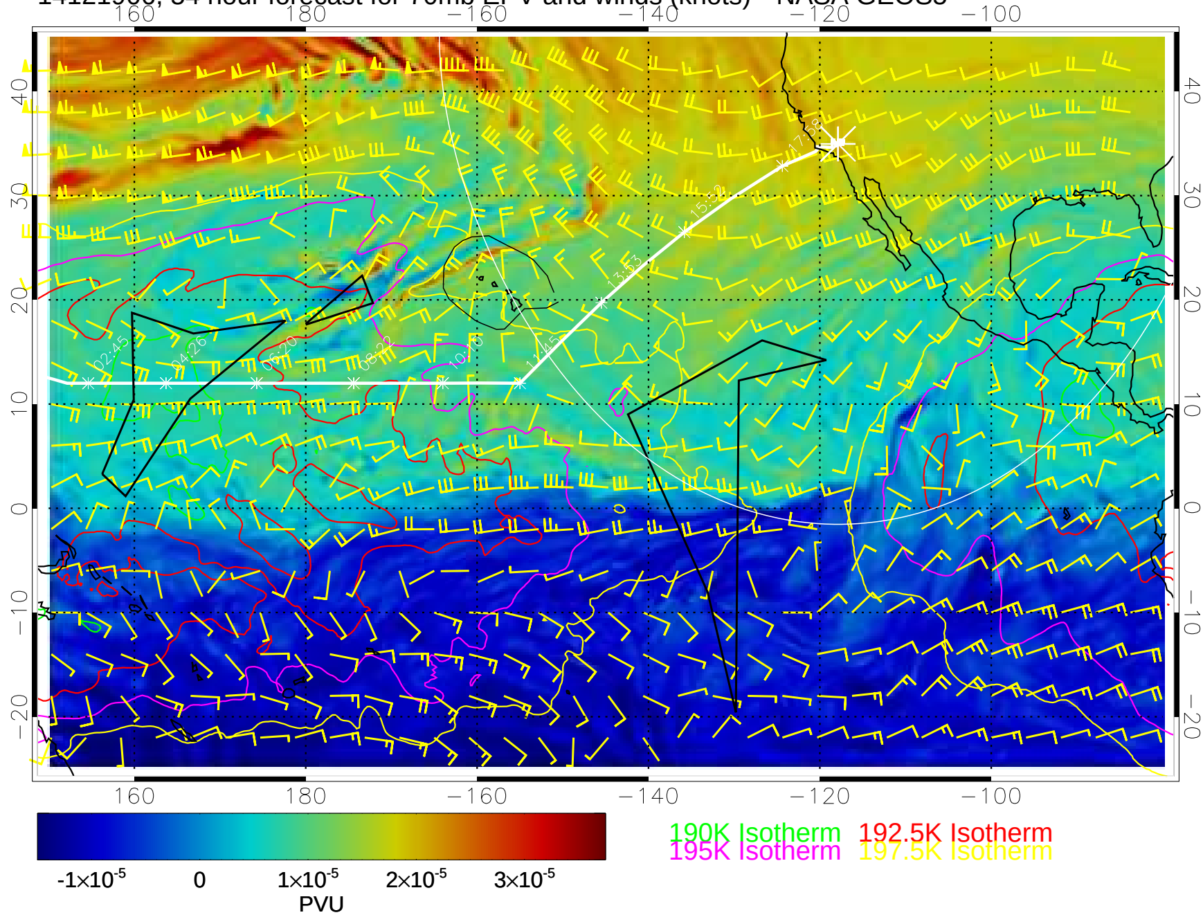
14121906, 54 hour forecast for 70mb EPV and winds (knots)-- NASA GEOS5
