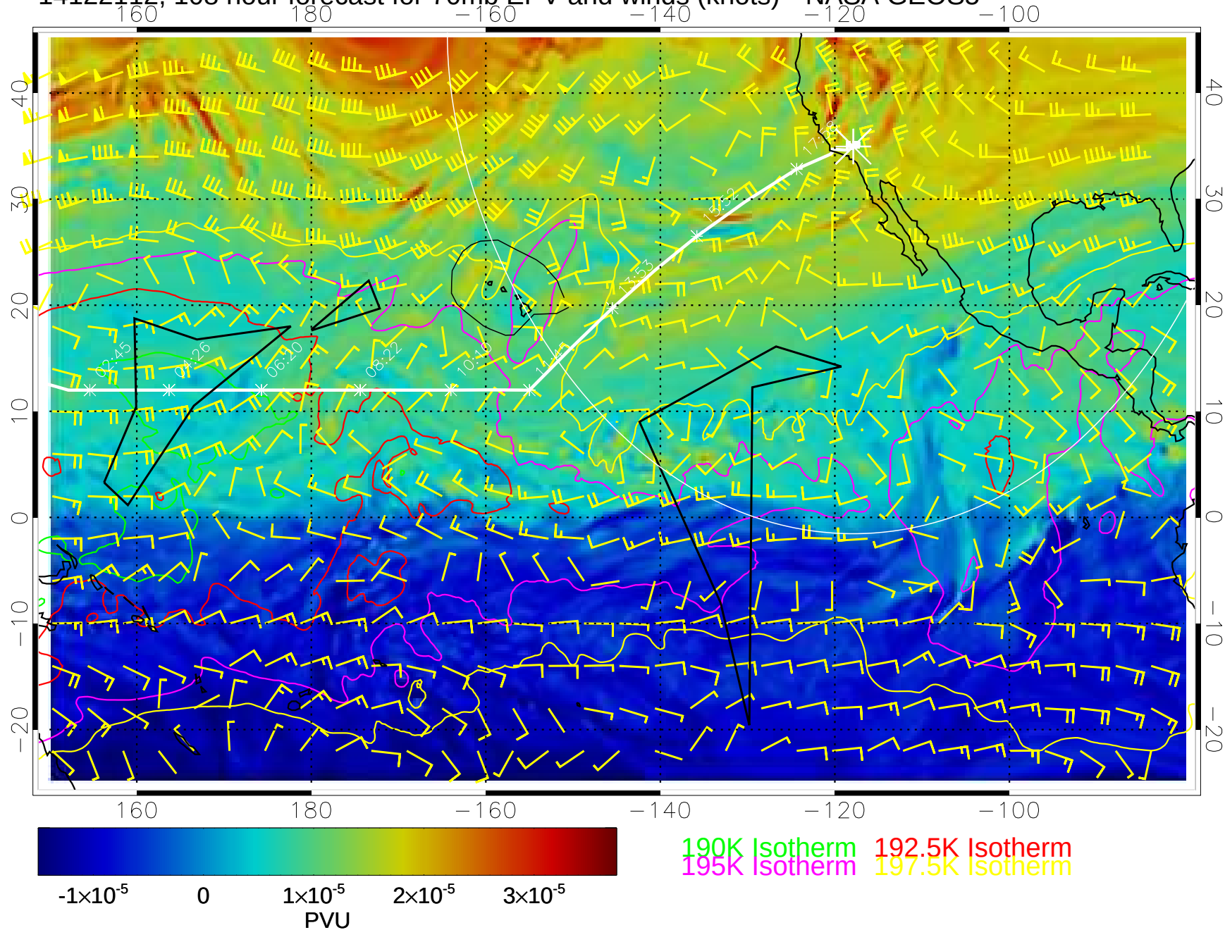
14122112, 108 hour forecast for 70mb EPV and winds (knots)-- NASA GEOS5
