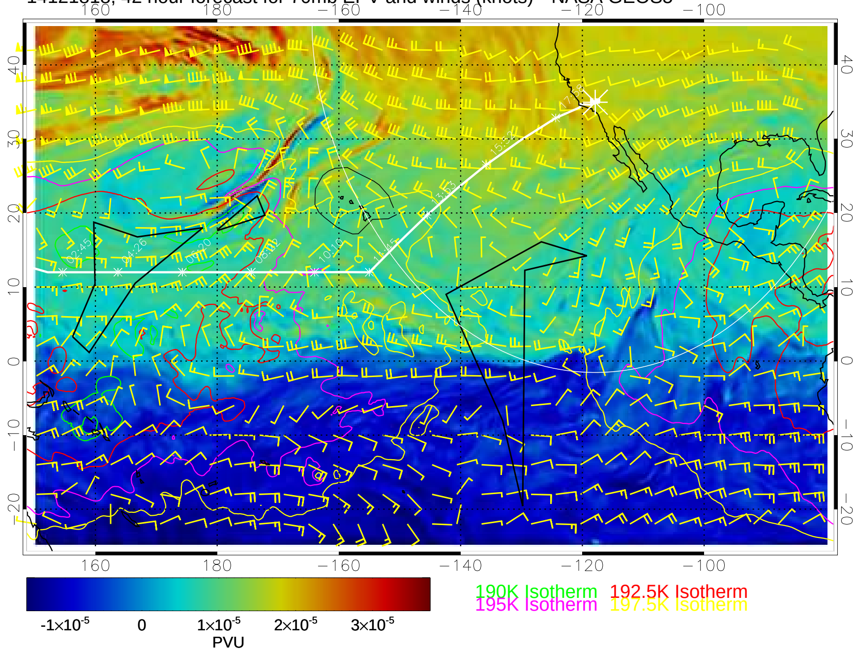
14121818, 42 hour forecast for 70mb EPV and winds (knots)-- NASA GEOS5
