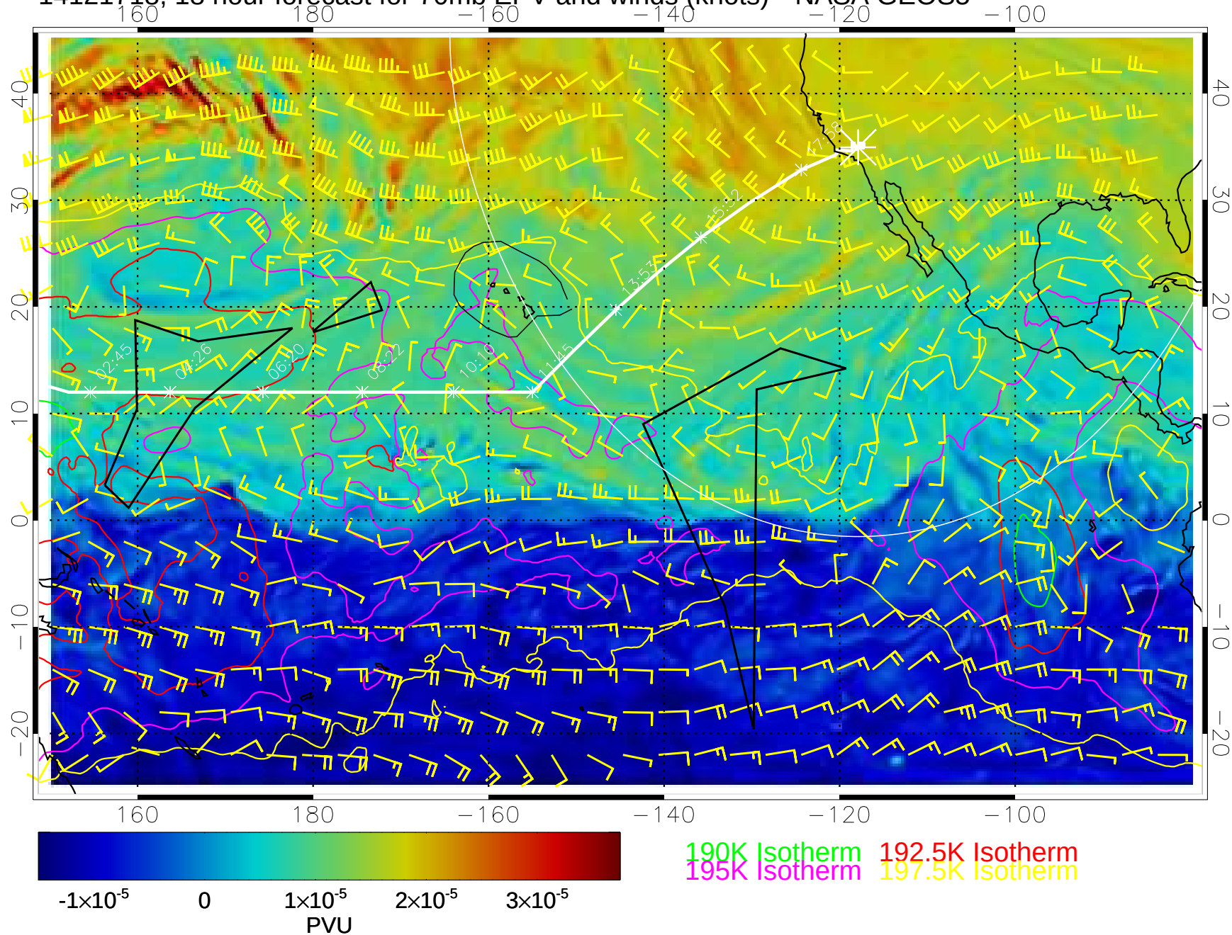
14121718, 18 hour forecast for 70mb EPV and winds (knots)-- NASA GEOS5
