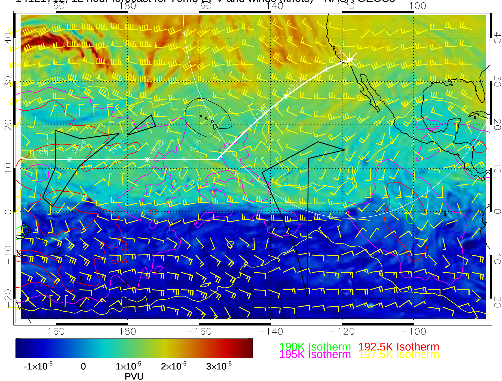
14121712, 12 hour forecast for 70mb EPV and winds (knots)-- NASA GEOS5
