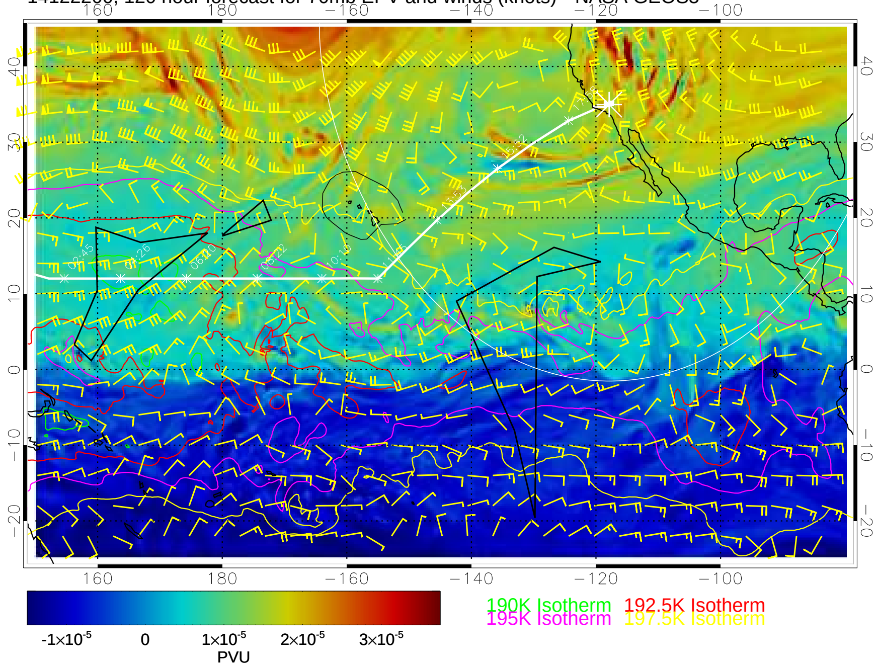
14122200, 120 hour forecast for 70mb EPV and winds (knots)-- NASA GEOS5
