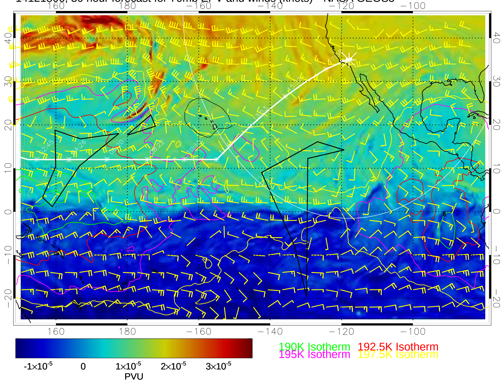
14121806, 30 hour forecast for 70mb EPV and winds (knots)-- NASA GEOS5
