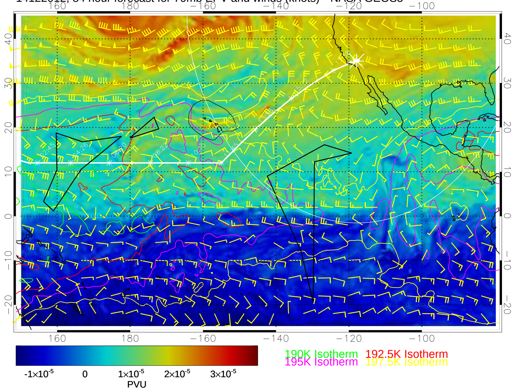
14122012, 84 hour forecast for 70mb EPV and winds (knots)-- NASA GEOS5
