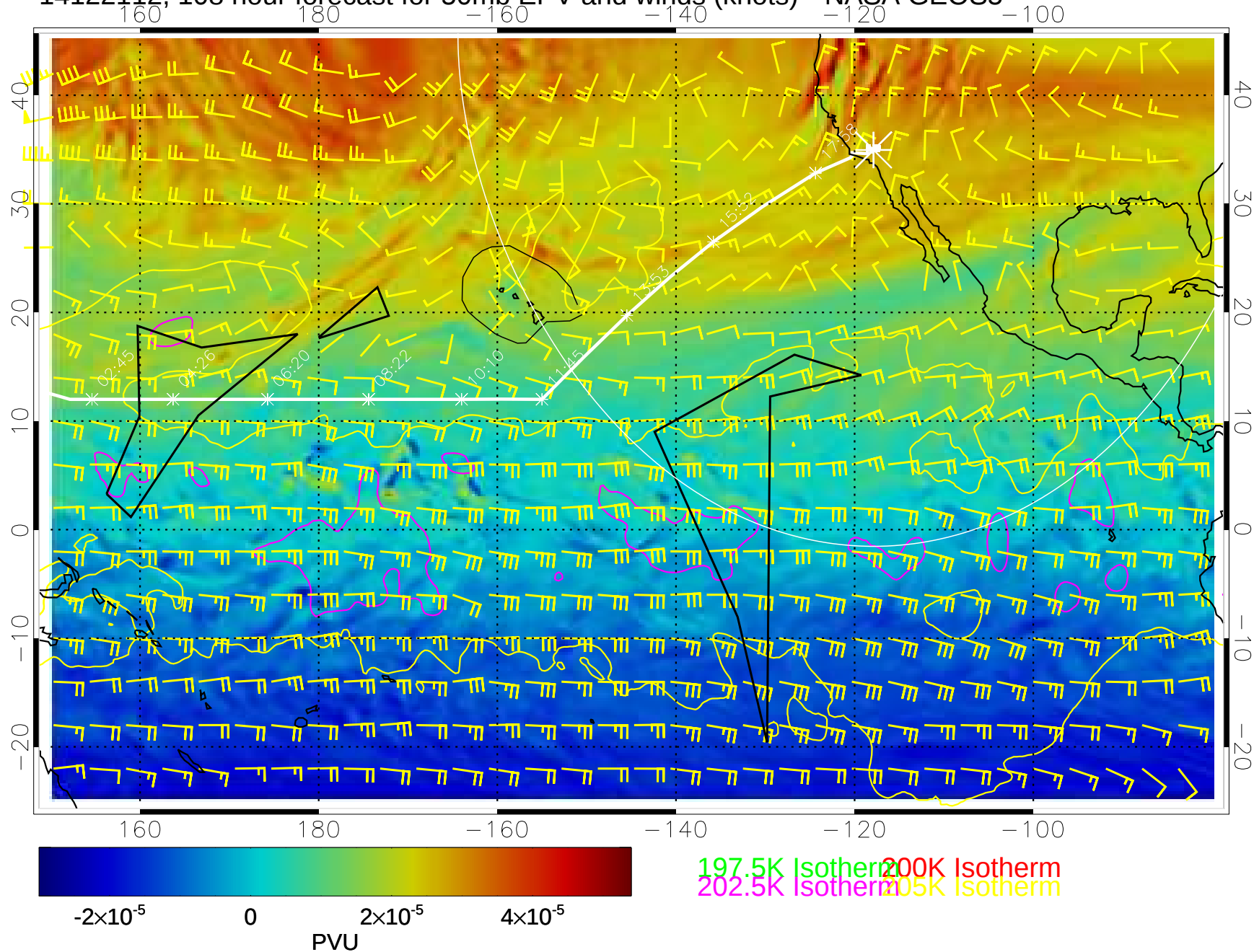
14122112, 108 hour forecast for 50mb EPV and winds (knots)-- NASA GEOS5
