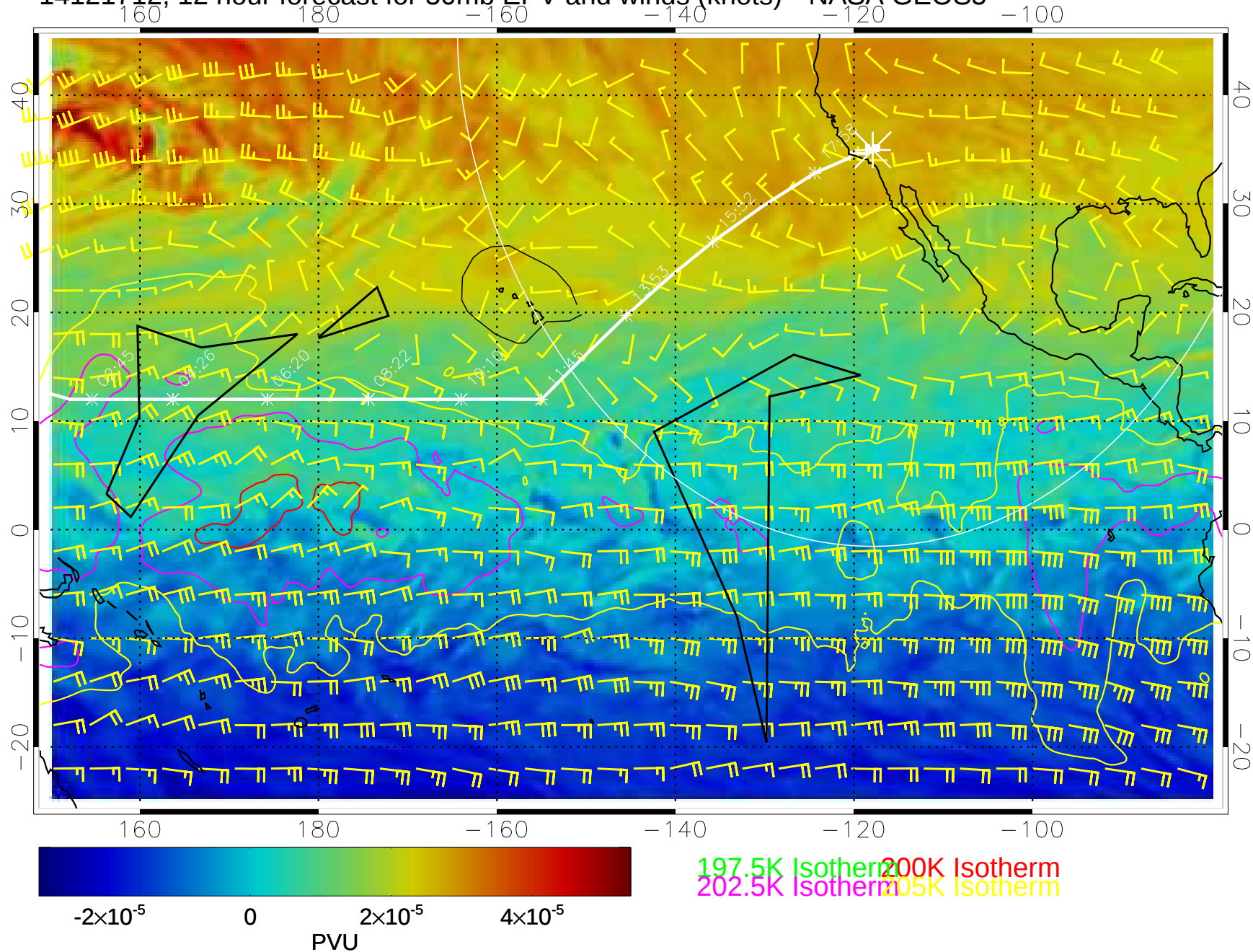
14121712, 12 hour forecast for 50mb EPV and winds (knots)-- NASA GEOS5
