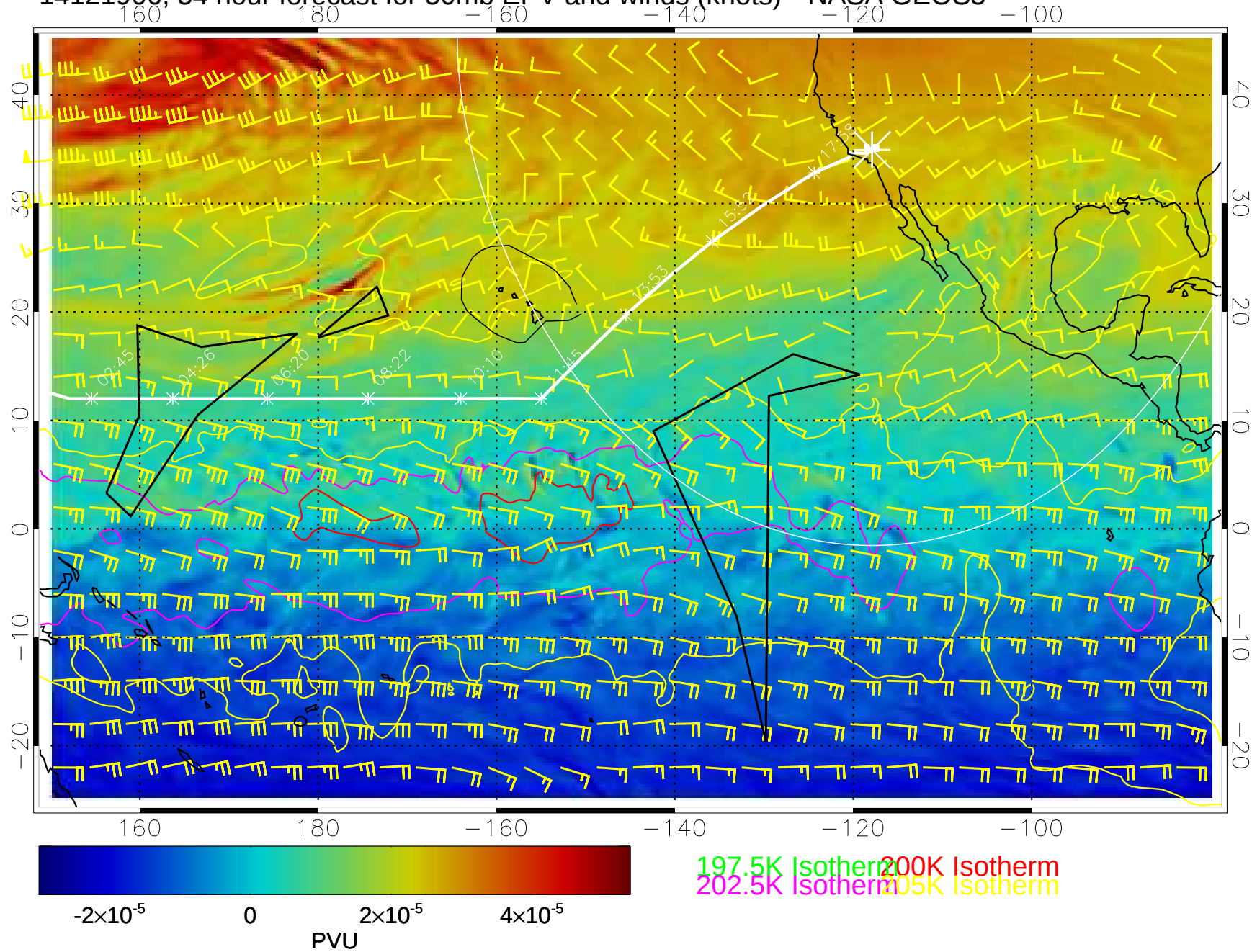
14121906, 54 hour forecast for 50mb EPV and winds (knots)-- NASA GEOS5
