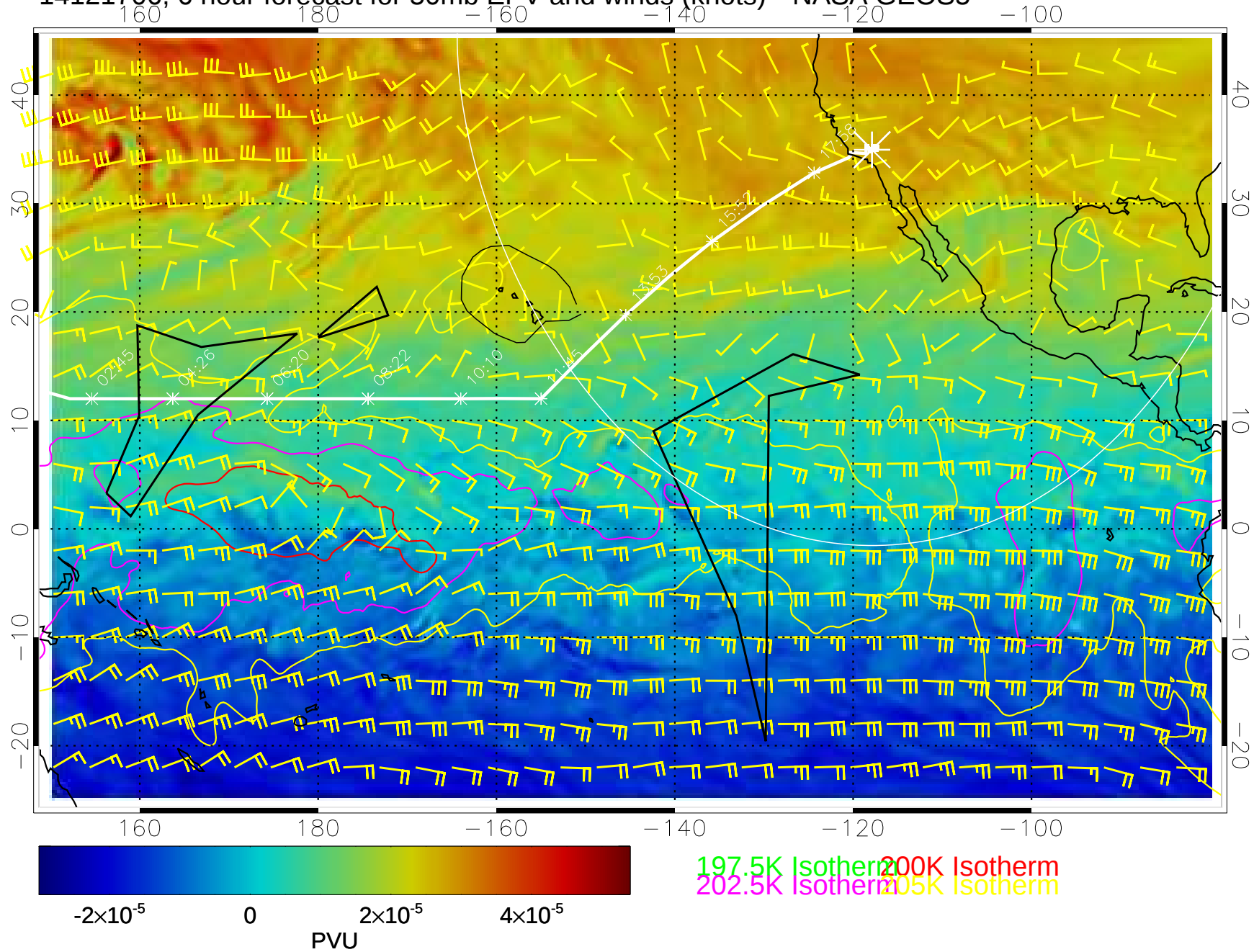
14121706, 6 hour forecast for 50mb EPV and winds (knots)-- NASA GEOS5
