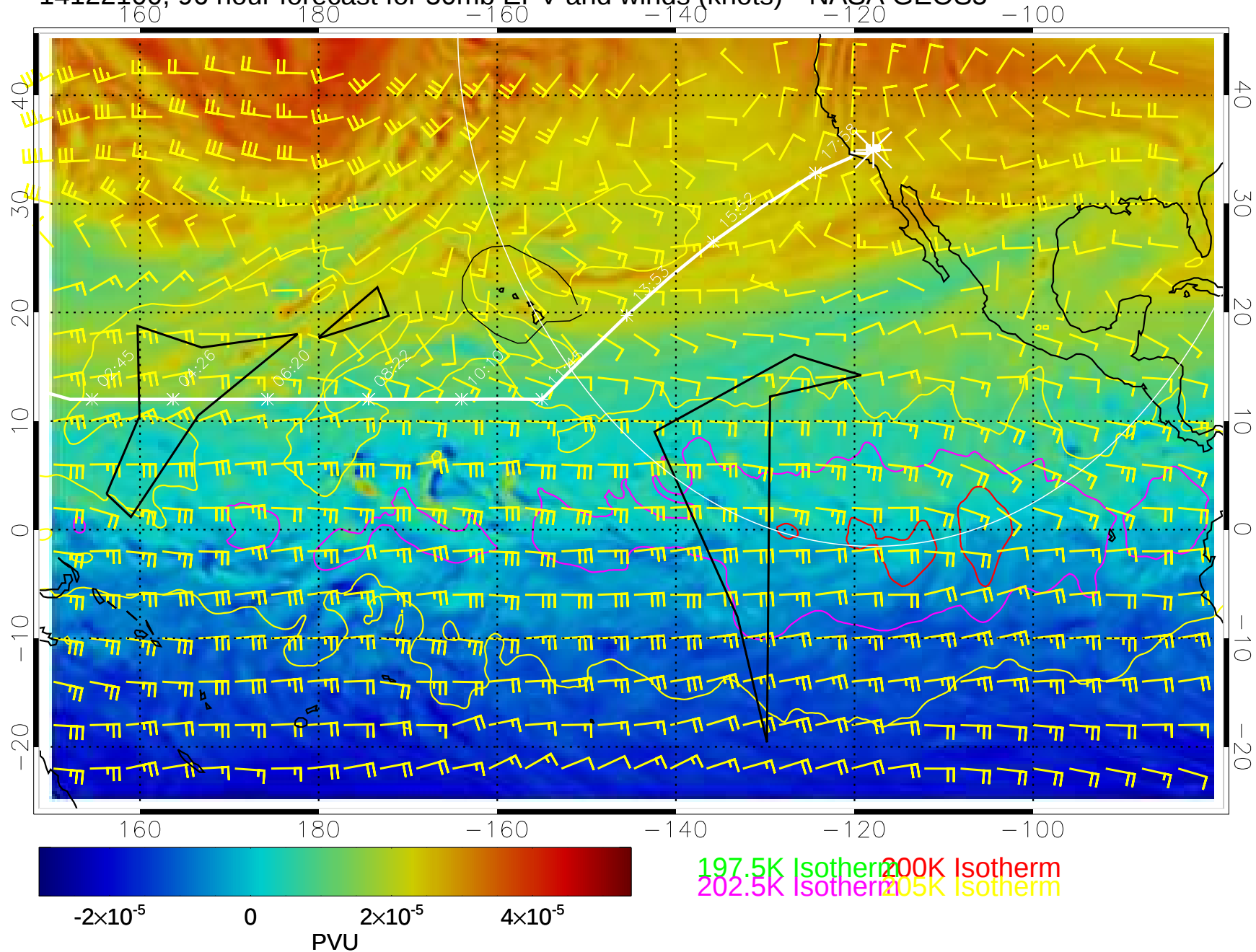
14122100, 96 hour forecast for 50mb EPV and winds (knots)-- NASA GEOS5
