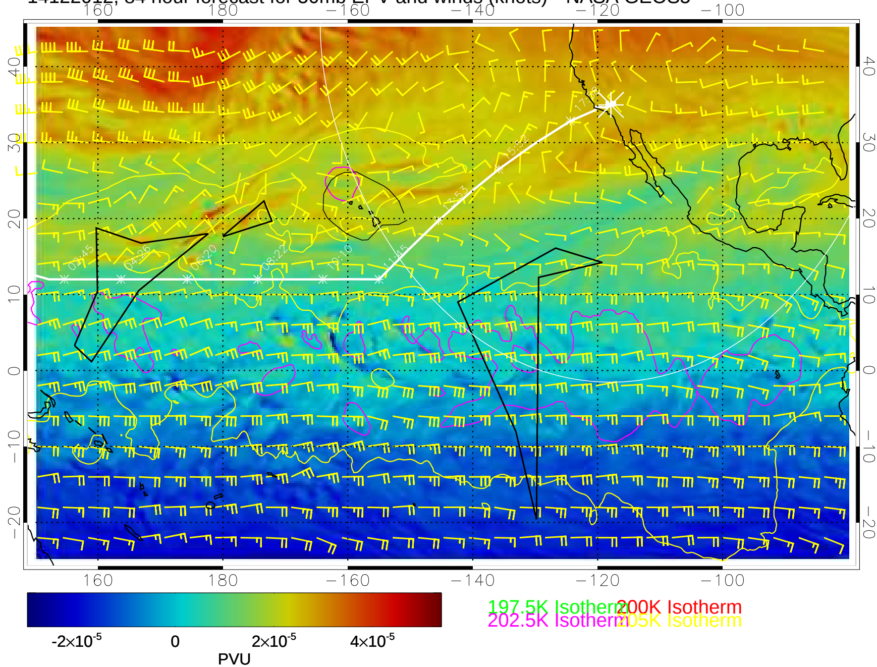
14122012, 84 hour forecast for 50mb EPV and winds (knots)-- NASA GEOS5
