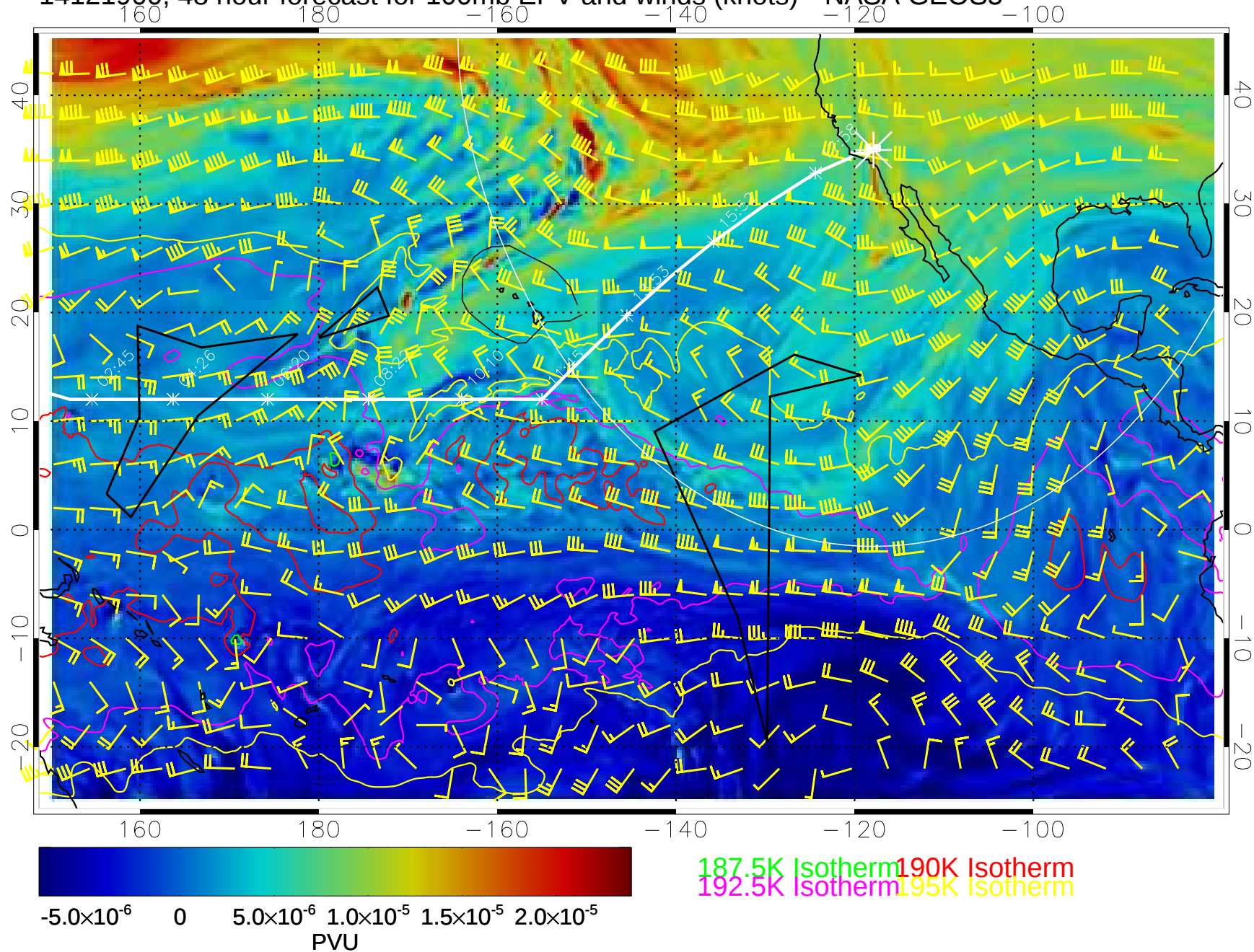
14121900, 48 hour forecast for 100mb EPV and winds (knots)-- NASA GEOS5
