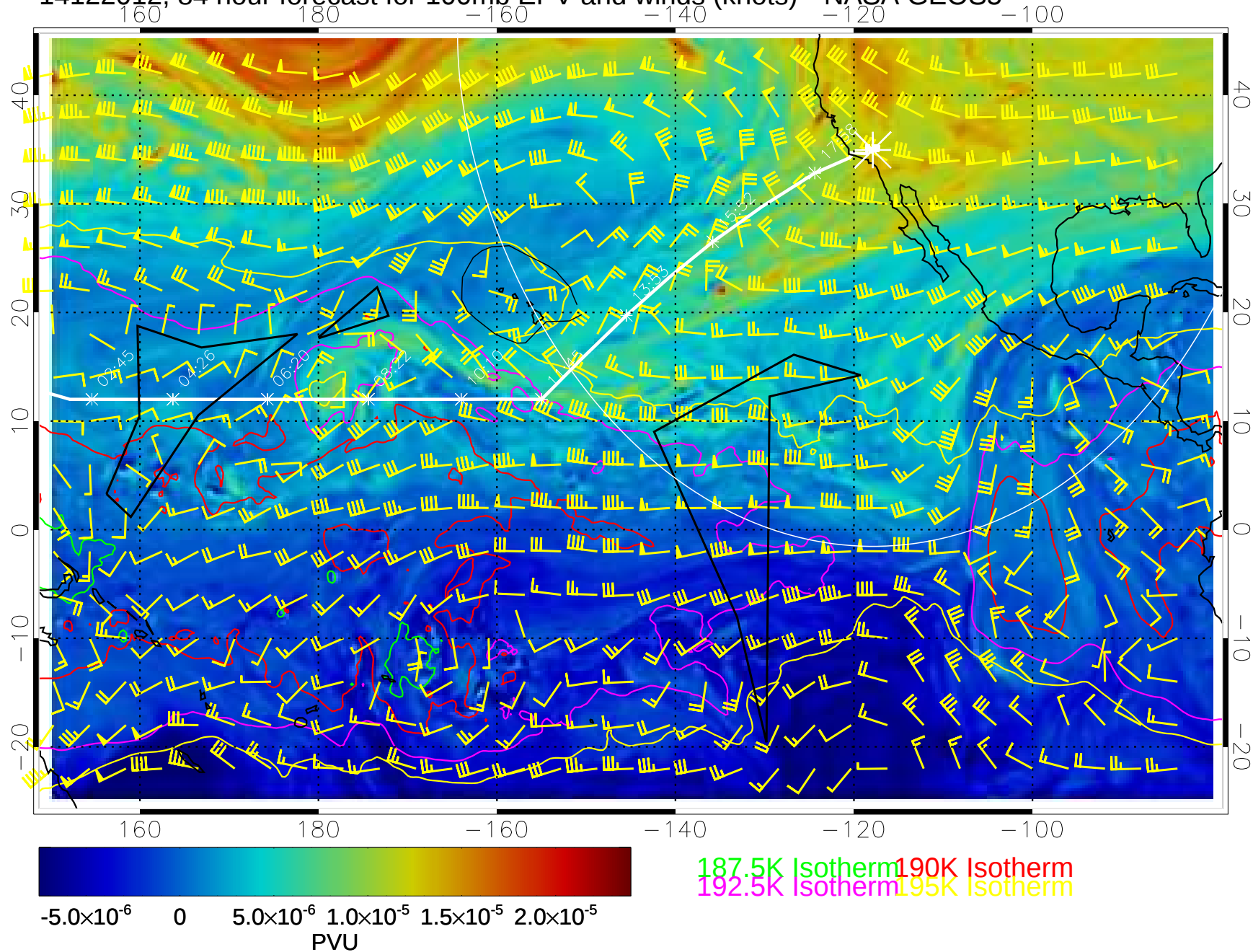
14122012, 84 hour forecast for 100mb EPV and winds (knots)-- NASA GEOS5
