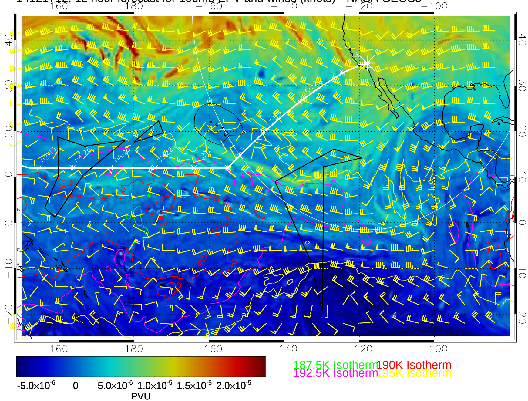
14121712, 12 hour forecast for 100mb EPV and winds (knots)-- NASA GEOS5
