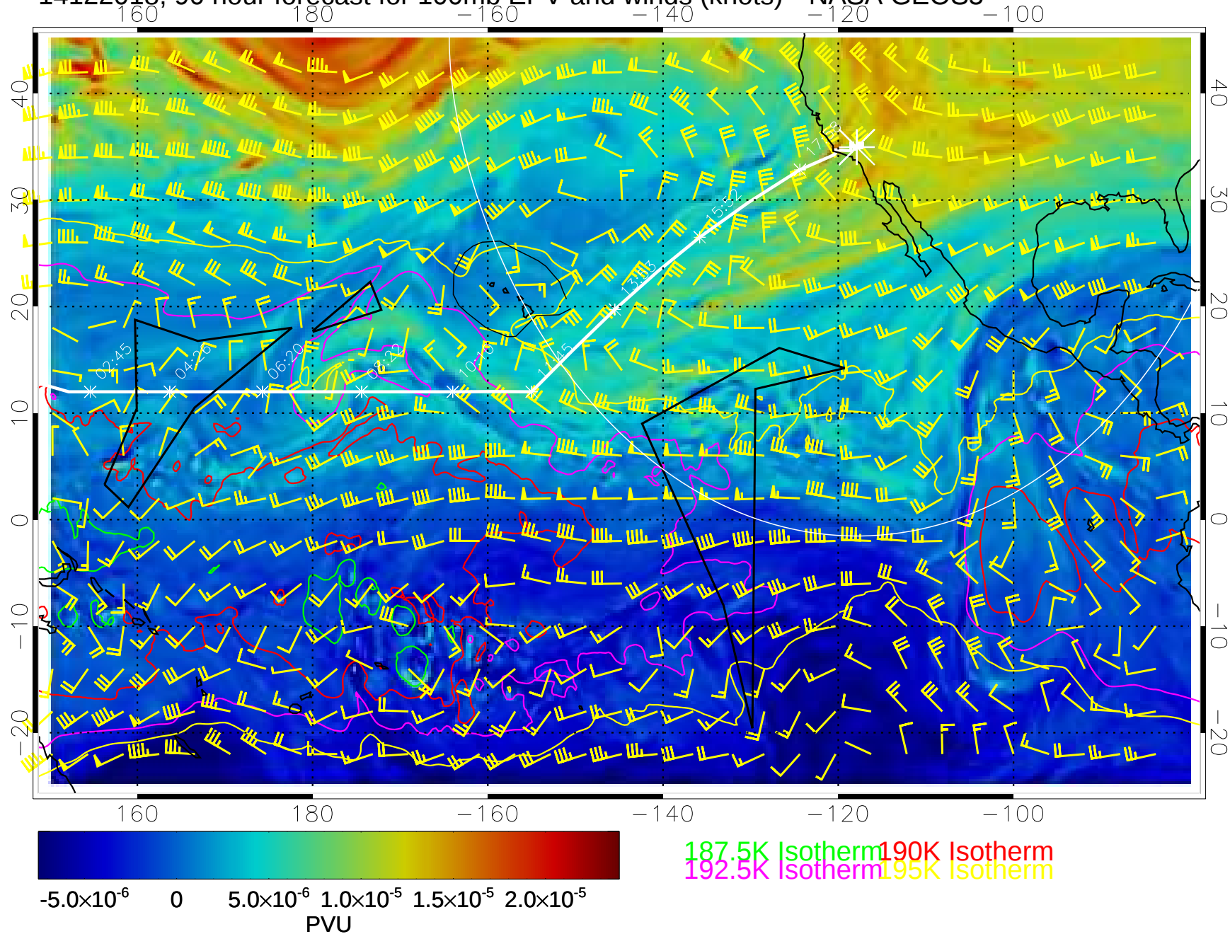
14122018, 90 hour forecast for 100mb EPV and winds (knots)-- NASA GEOS5
