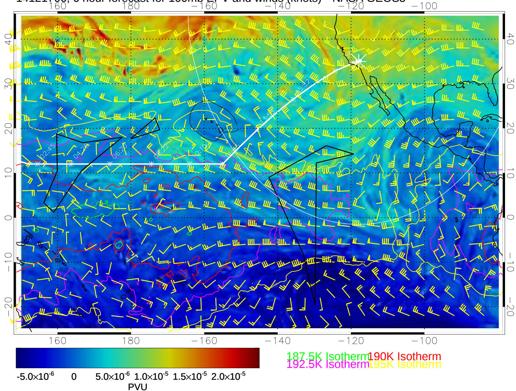
14121706, 6 hour forecast for 100mb EPV and winds (knots)-- NASA GEOS5
