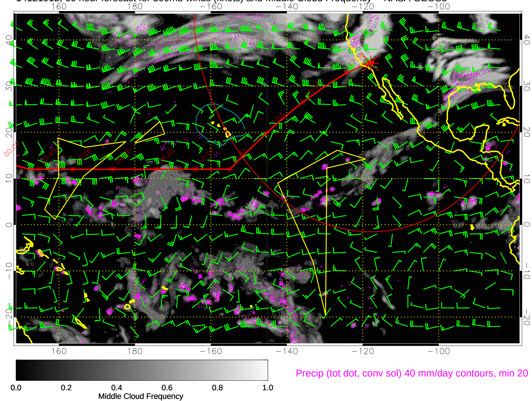
14121912, 60 hour forecast for 500mb winds (knots) and Middle Cloud Frequency -- NASA GEOS5
