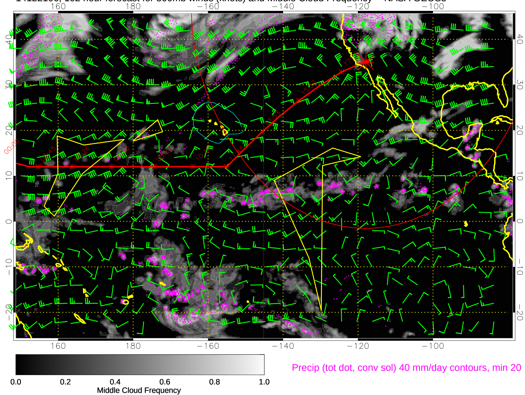
14122106, 102 hour forecast for 500mb winds (knots) and Middle Cloud Frequency -- NASA GEOS5
