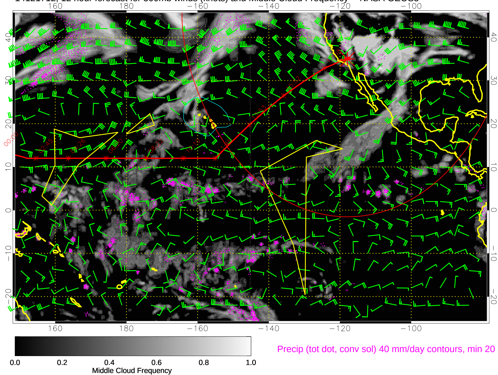
14121712, 12 hour forecast for 500mb winds (knots) and Middle Cloud Frequency -- NASA GEOS5
