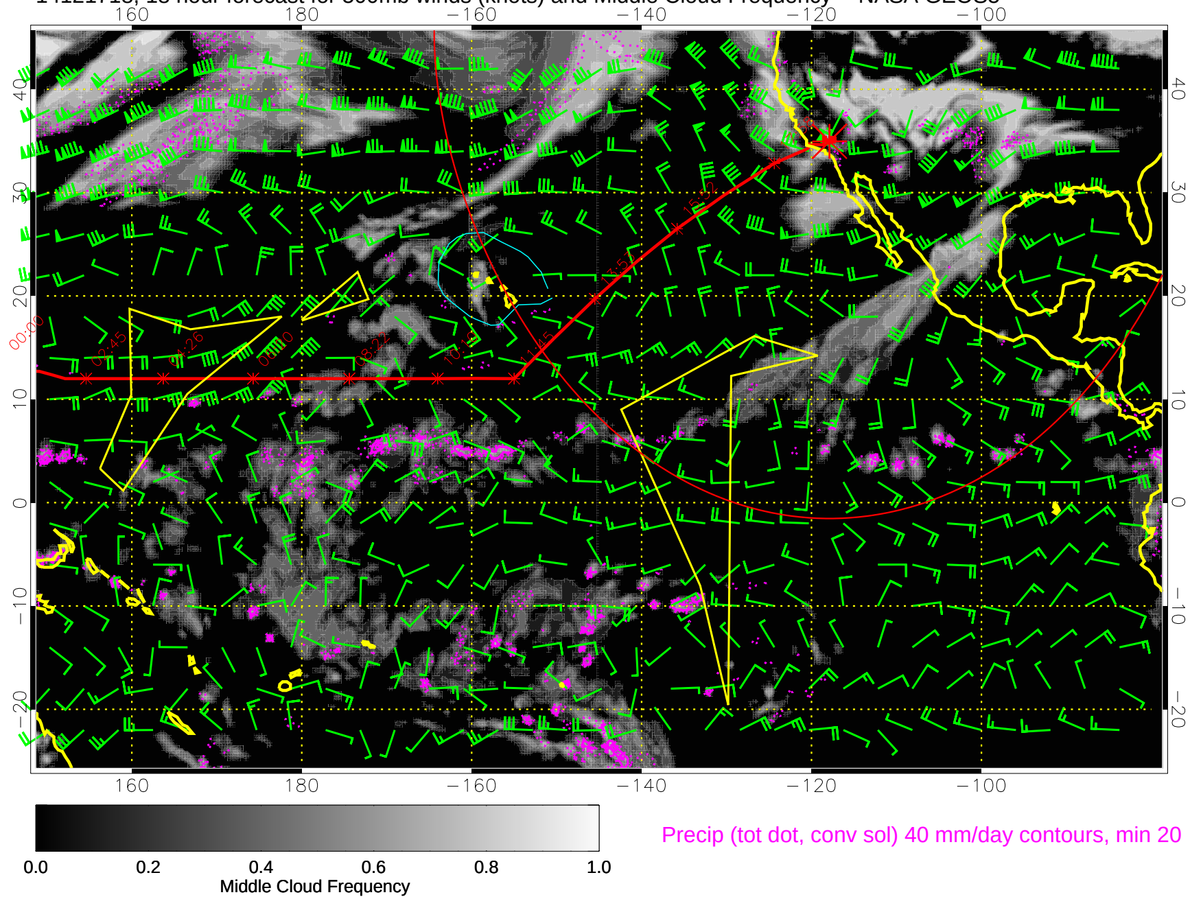
14121718, 18 hour forecast for 500mb winds (knots) and Middle Cloud Frequency -- NASA GEOS5
