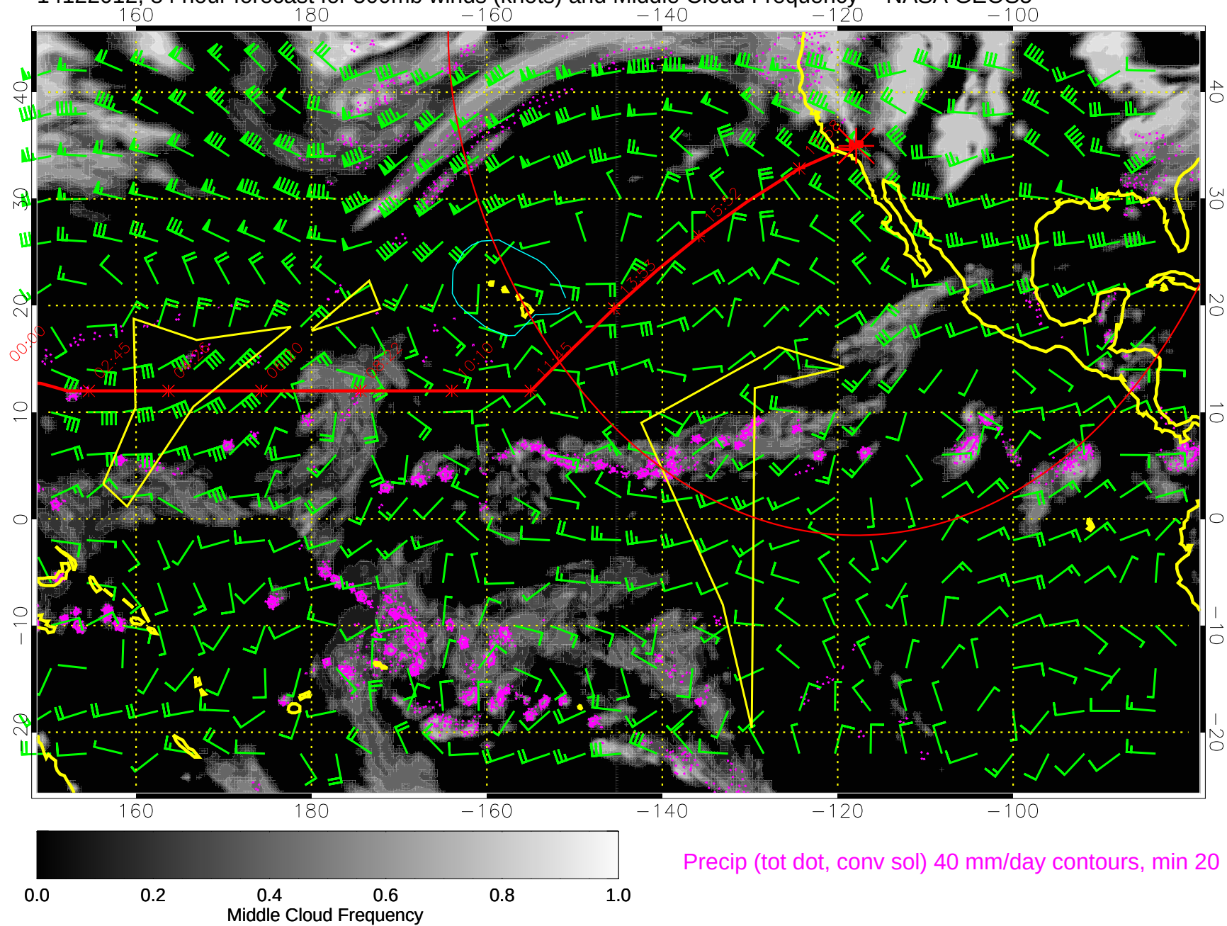
14122012, 84 hour forecast for 500mb winds (knots) and Middle Cloud Frequency -- NASA GEOS5
