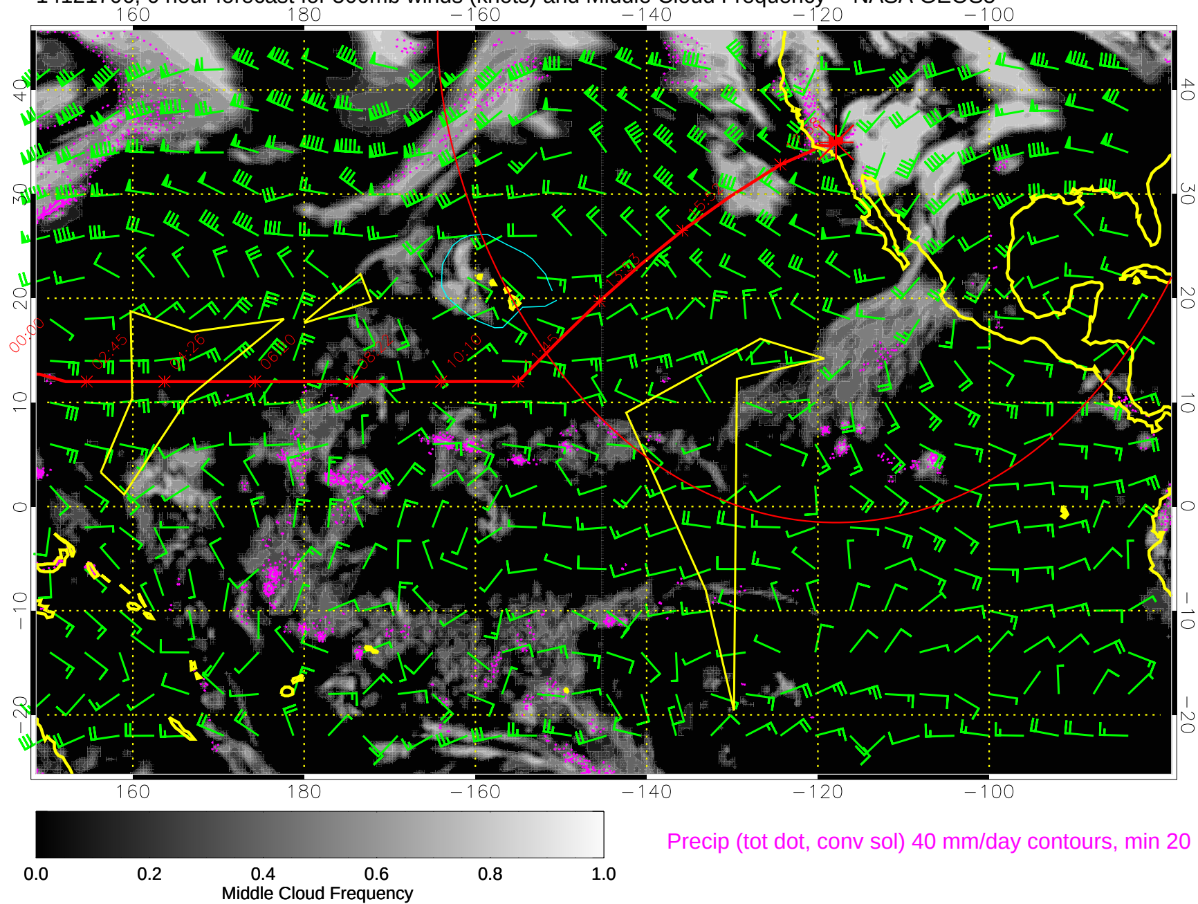
14121706, 6 hour forecast for 500mb winds (knots) and Middle Cloud Frequency -- NASA GEOS5
