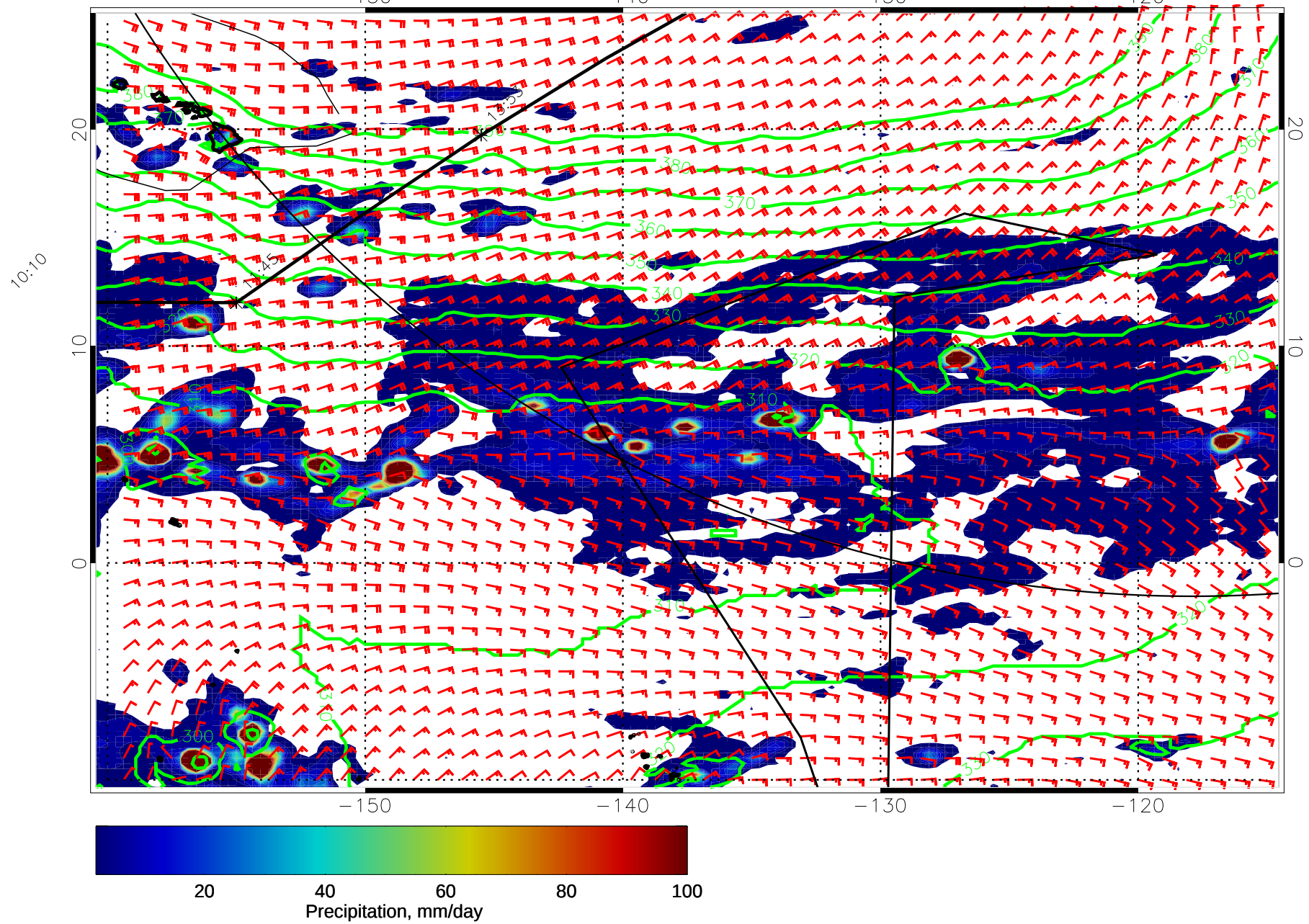
14121912, 108 hour forecast for 975mb Z, Precip., and Surface Winds (knots) -- NASA GEOS5
