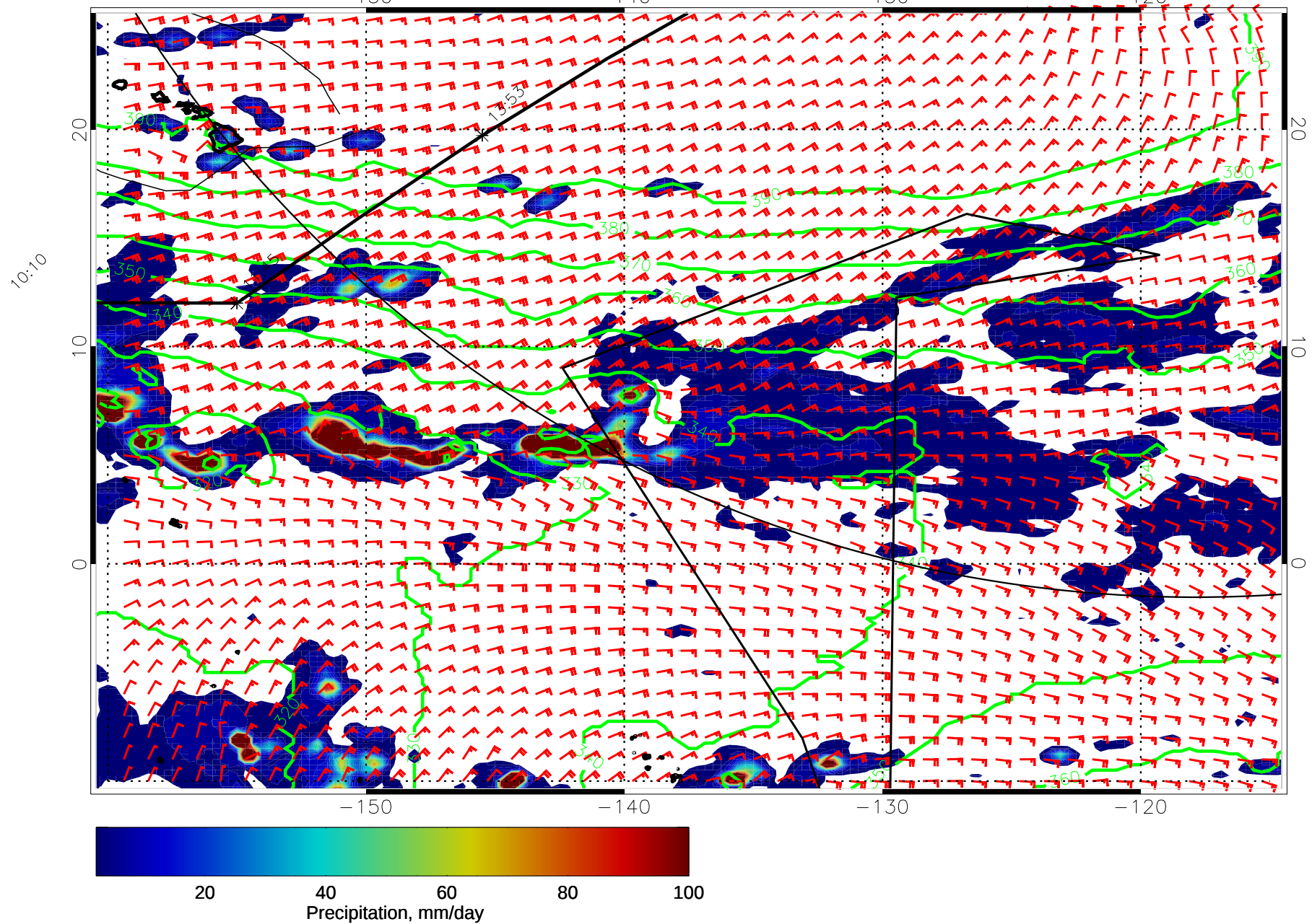
14121818, 90 hour forecast for 975mb Z, Precip., and Surface Winds (knots) -- NASA GEOS5
