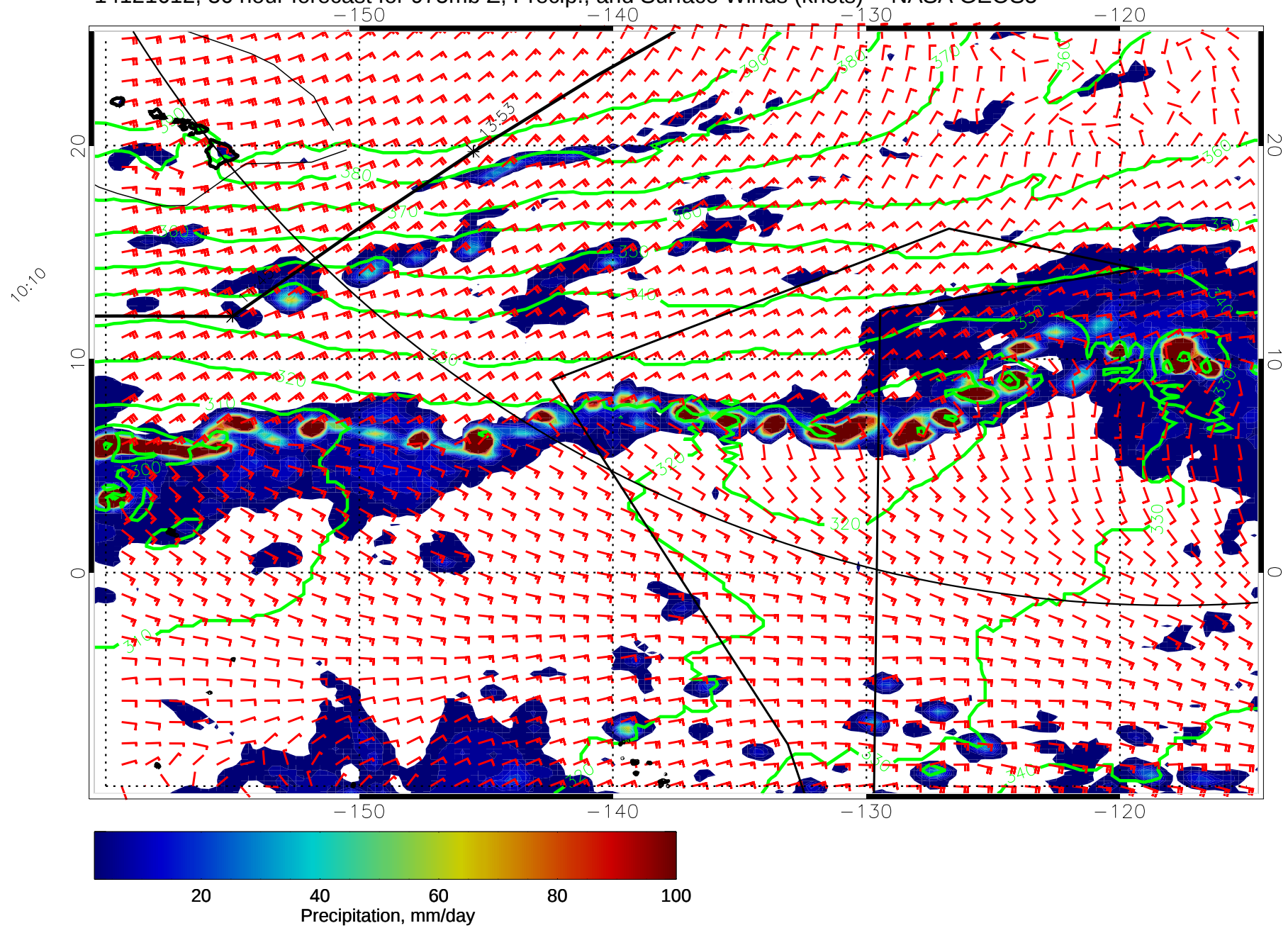
14121612, 36 hour forecast for 975mb Z, Precip., and Surface Winds (knots) -- NASA GEOS5
