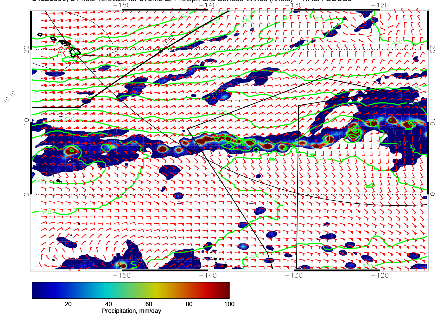
14121600, 24 hour forecast for 975mb Z, Precip., and Surface Winds (knots) -- NASA GEOS5
