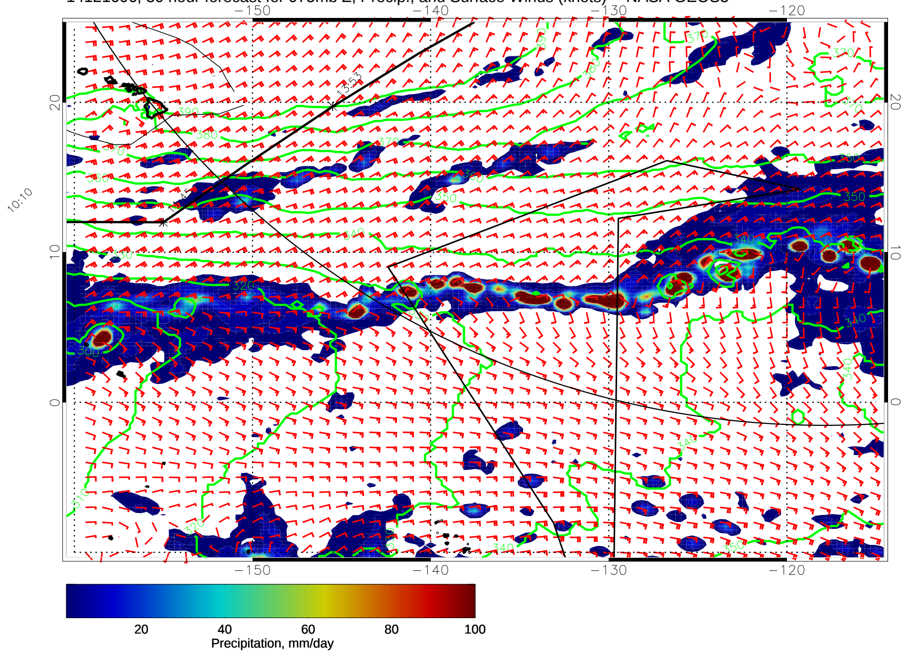
14121606, 30 hour forecast for 975mb Z, Precip., and Surface Winds (knots) -- NASA GEOS5
