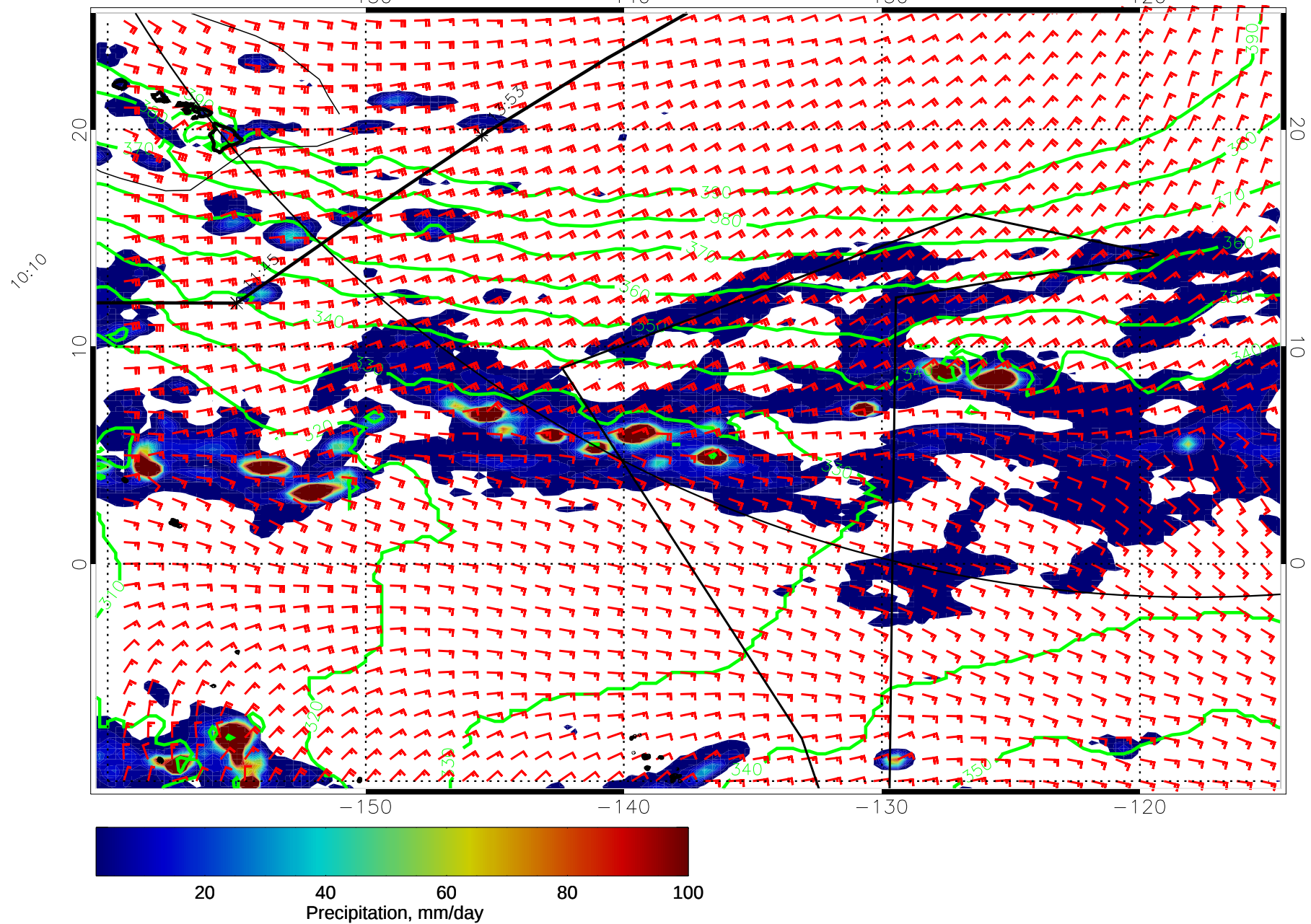
14121918, 114 hour forecast for 975mb Z, Precip., and Surface Winds (knots) -- NASA GEOS5
