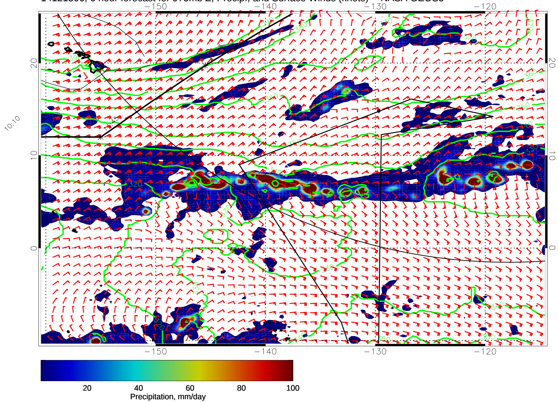
14121506, 6 hour forecast for 975mb Z, Precip., and Surface Winds (knots) -- NASA GEOS5
