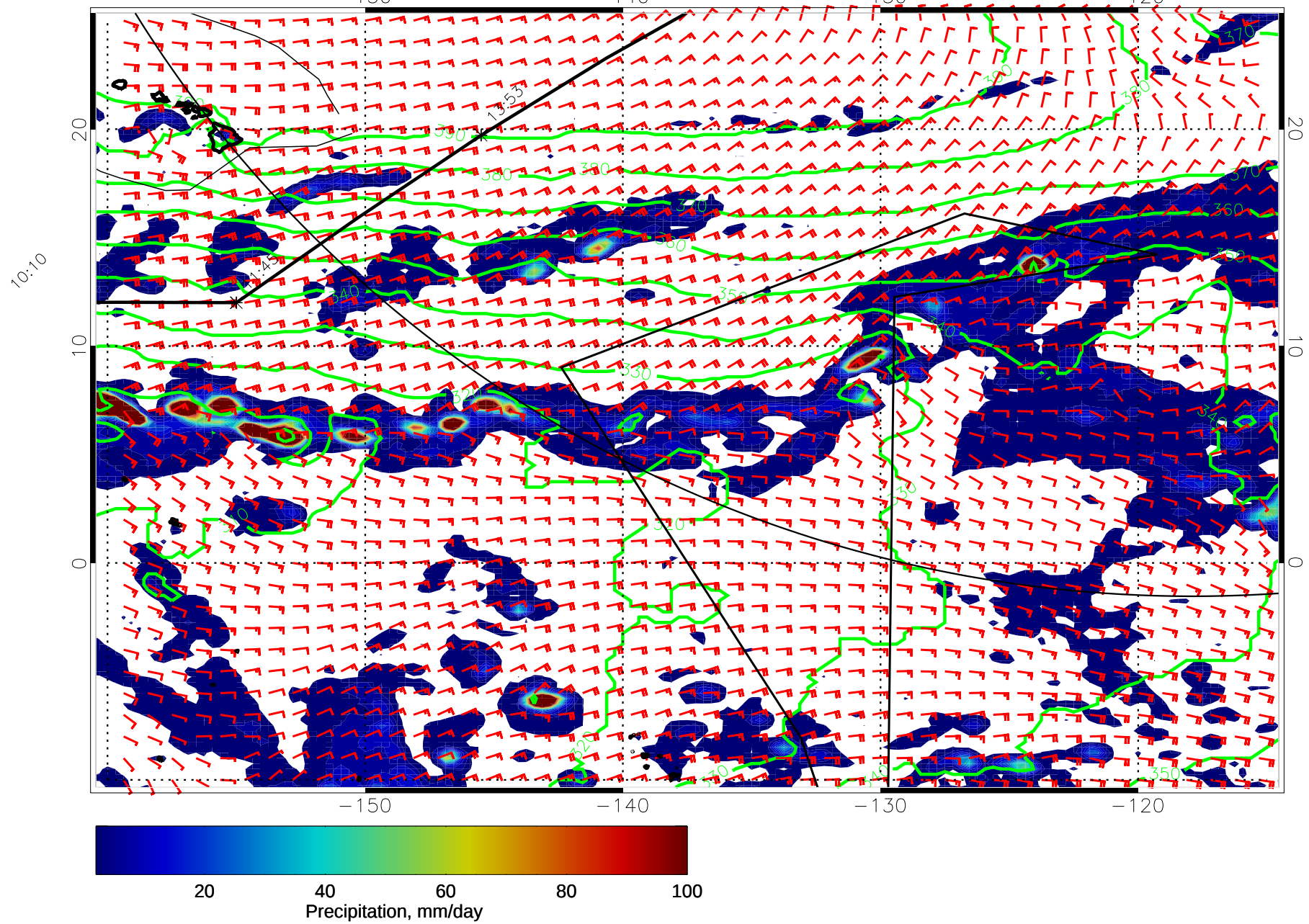
14121712, 60 hour forecast for 975mb Z, Precip., and Surface Winds (knots) -- NASA GEOS5
