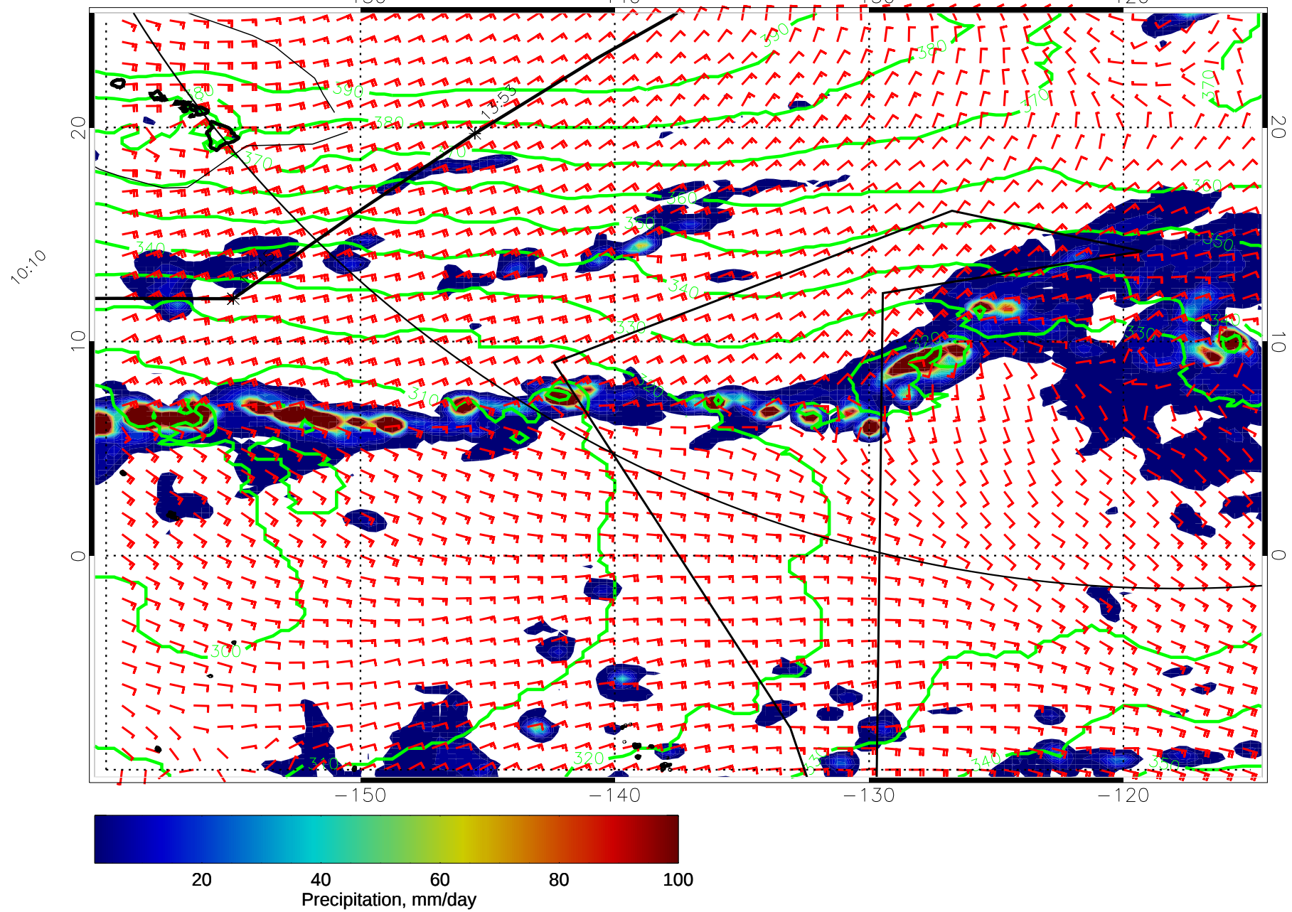
14121700, 48 hour forecast for 975mb Z, Precip., and Surface Winds (knots) -- NASA GEOS5
