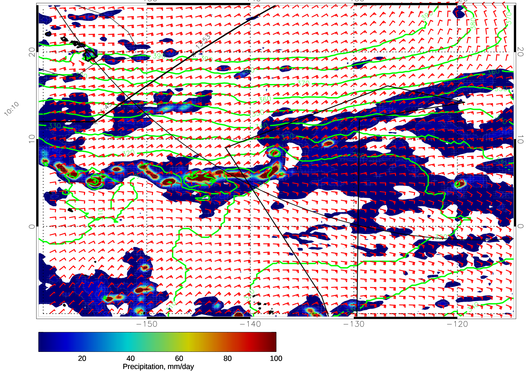
14121812, 84 hour forecast for 975mb Z, Precip., and Surface Winds (knots) -- NASA GEOS5
