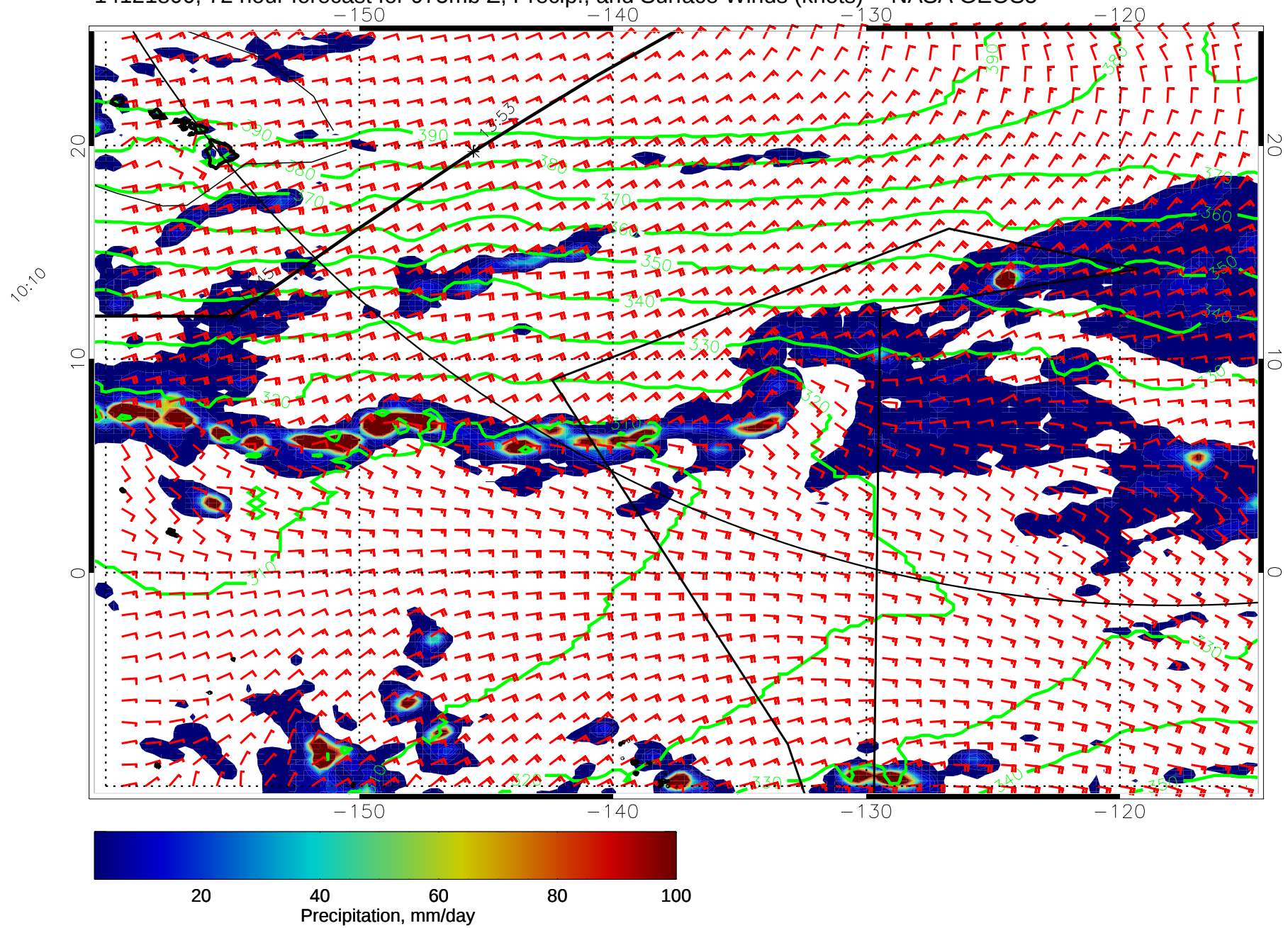
14121800, 72 hour forecast for 975mb Z, Precip., and Surface Winds (knots) -- NASA GEOS5
