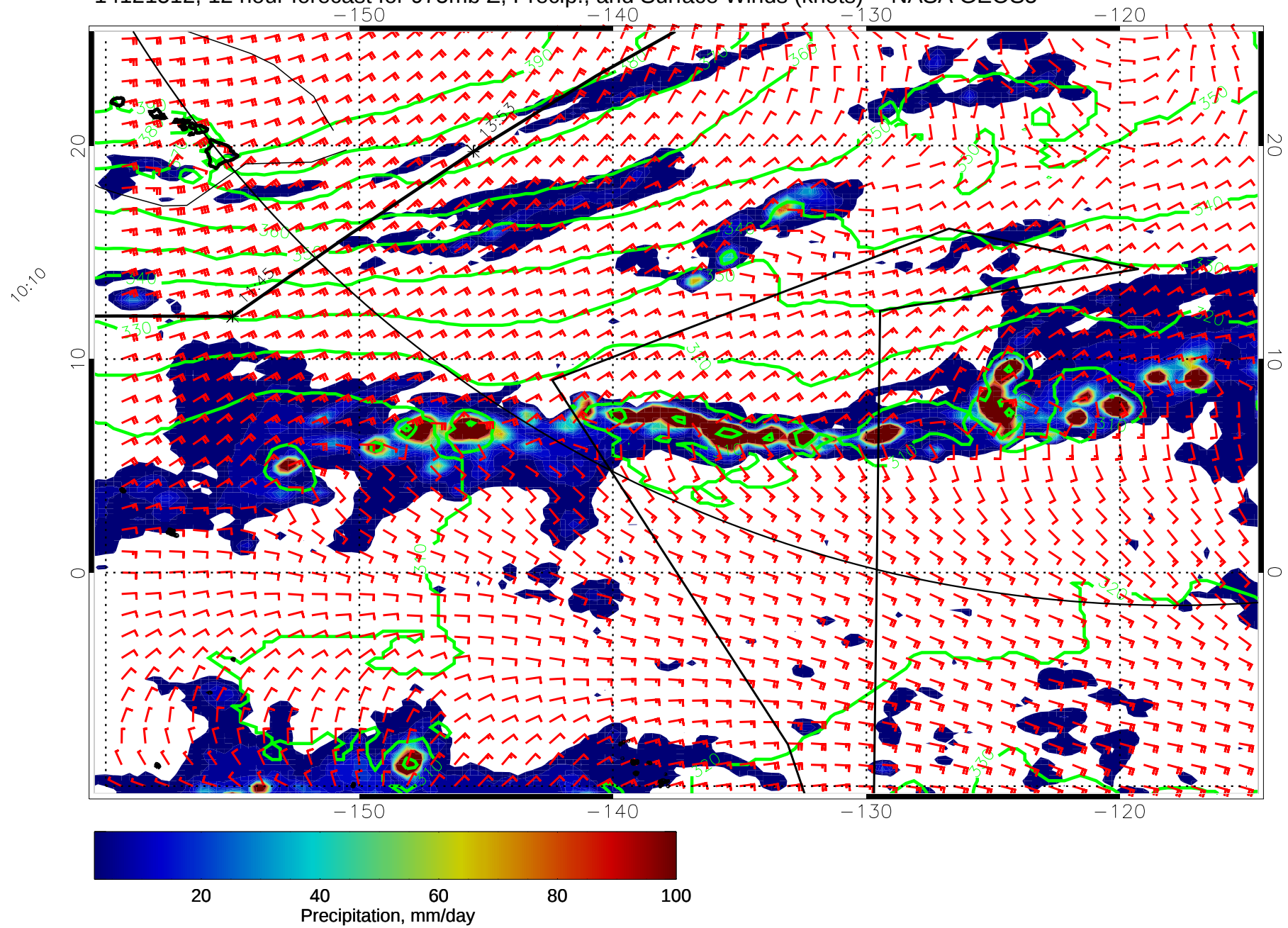
14121512, 12 hour forecast for 975mb Z, Precip., and Surface Winds (knots) -- NASA GEOS5
