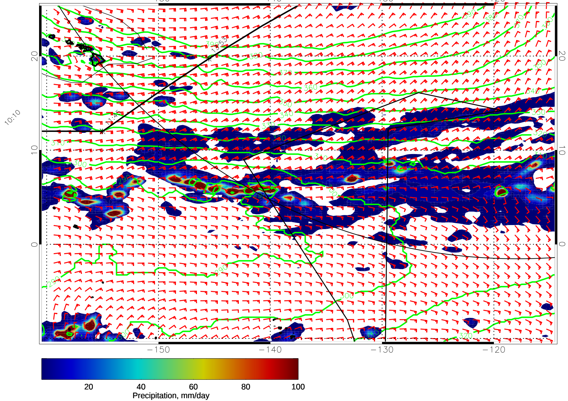
14122000, 120 hour forecast for 975mb Z, Precip., and Surface Winds (knots) -- NASA GEOS5
