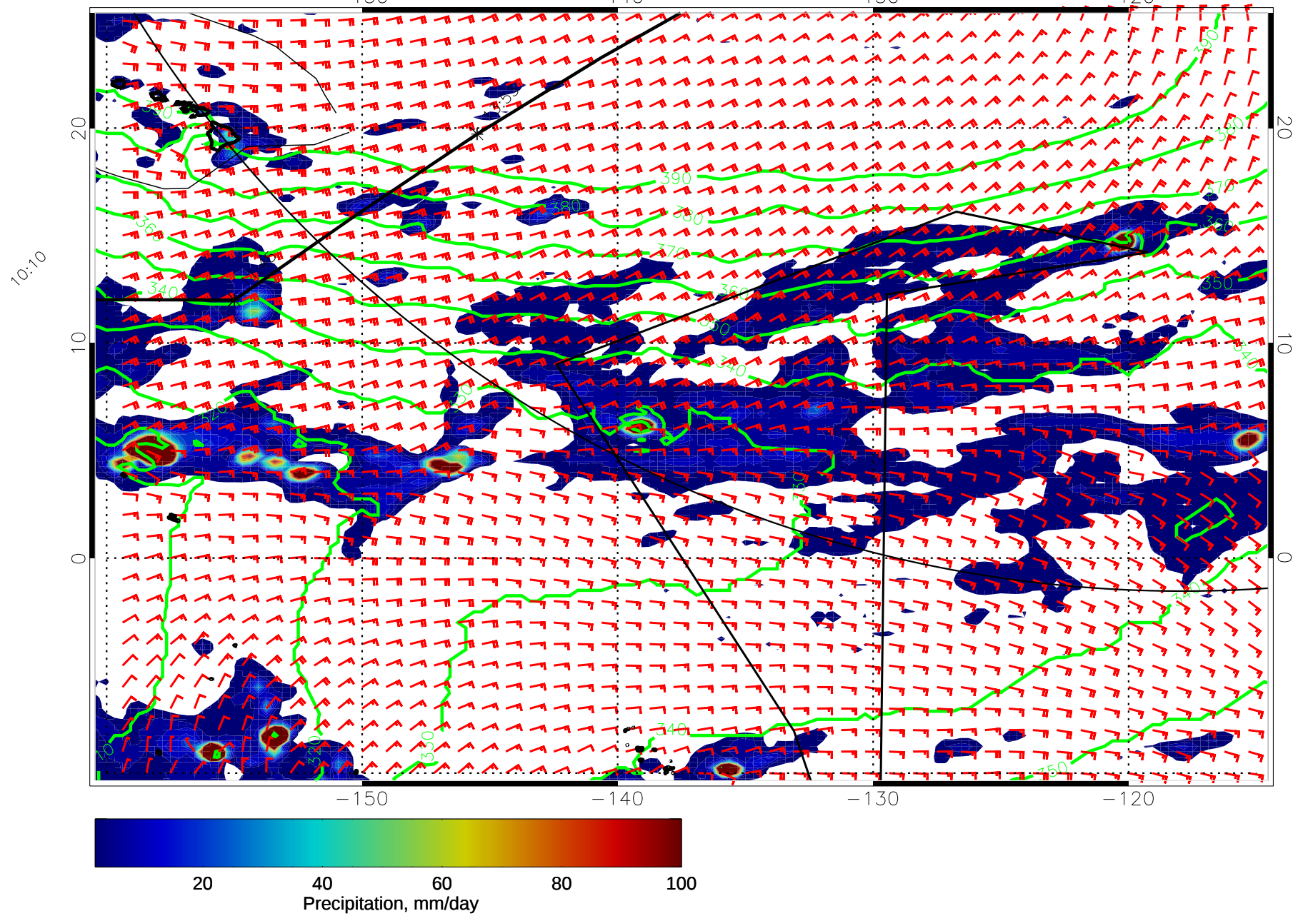
14121906, 102 hour forecast for 975mb Z, Precip., and Surface Winds (knots) -- NASA GEOS5
