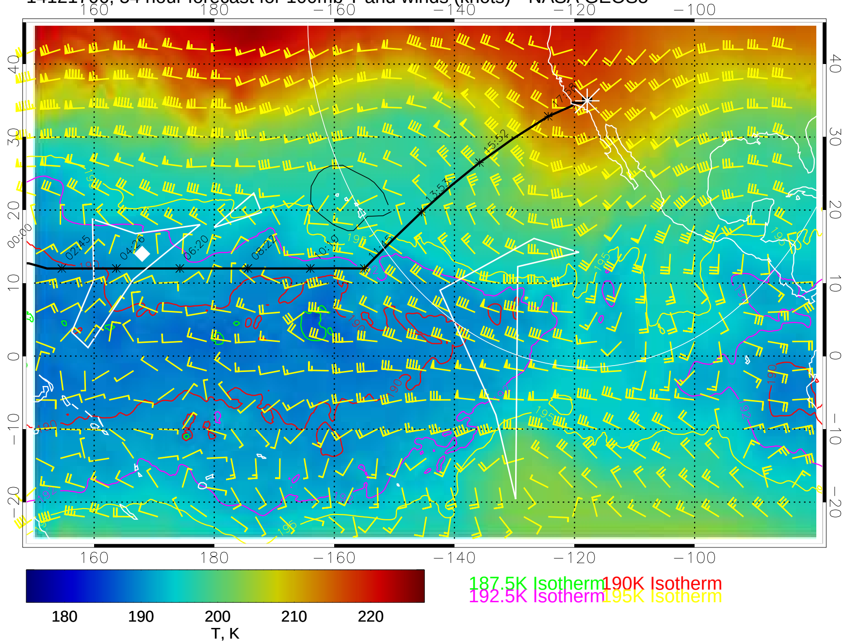
14121706, 54 hour forecast for 100mb T and winds (knots)-- NASA GEOS5
