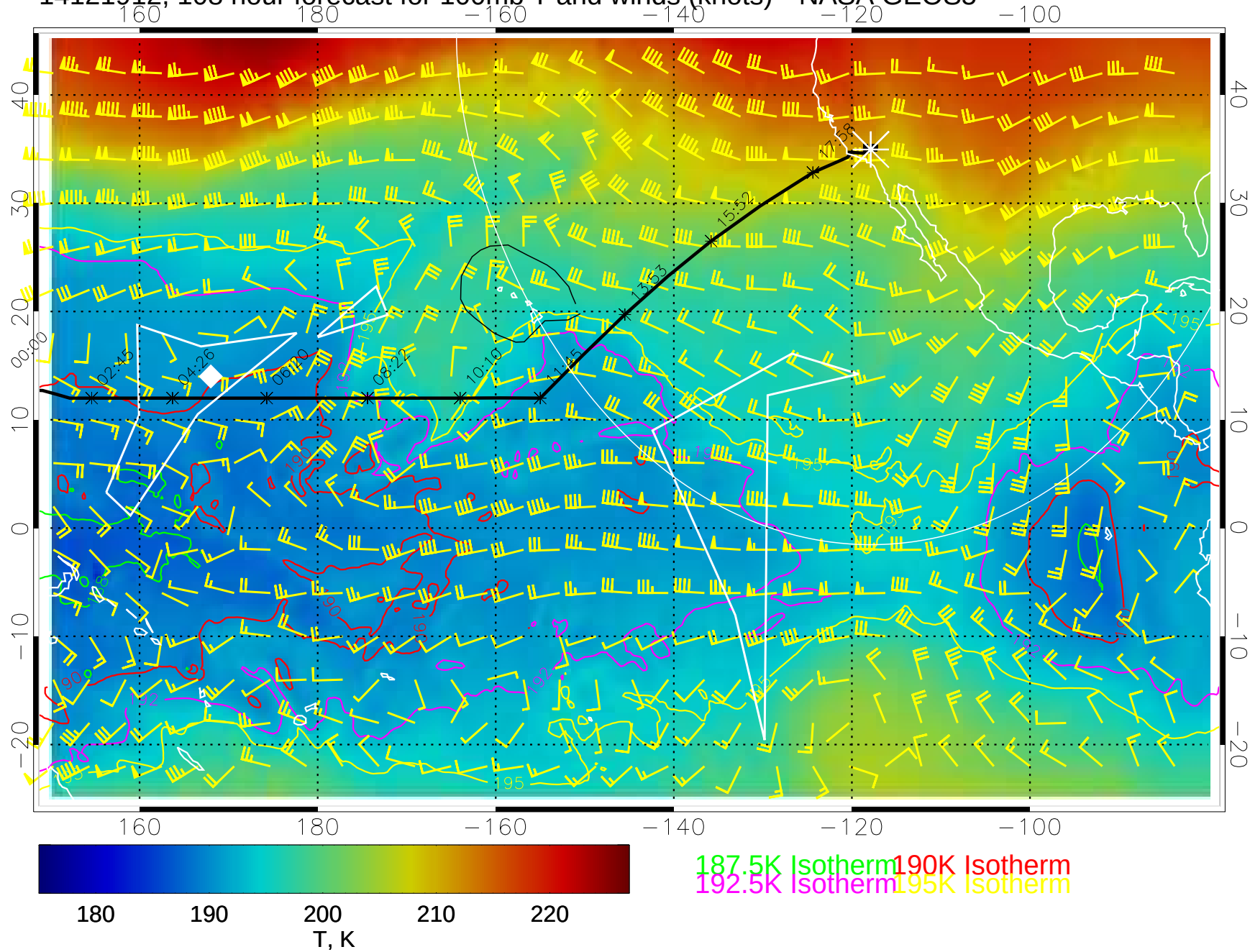
14121912, 108 hour forecast for 100mb T and winds (knots)-- NASA GEOS5
