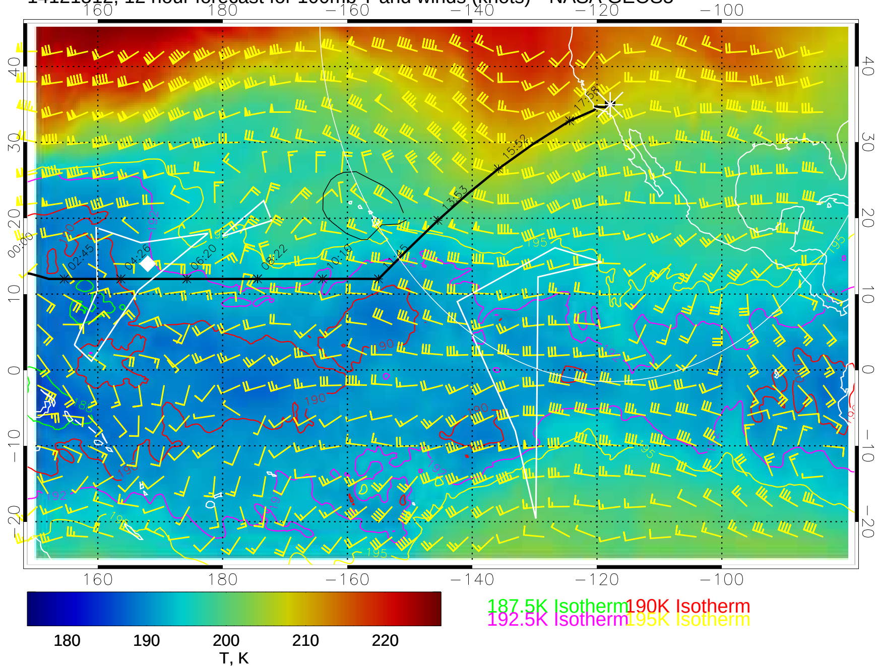
14121512, 12 hour forecast for 100mb T and winds (knots)-- NASA GEOS5
