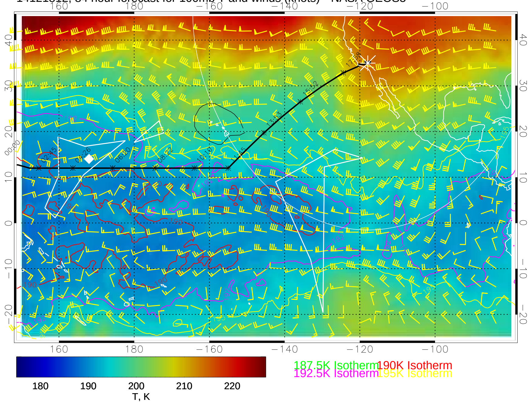
14121812, 84 hour forecast for 100mb T and winds (knots)-- NASA GEOS5
