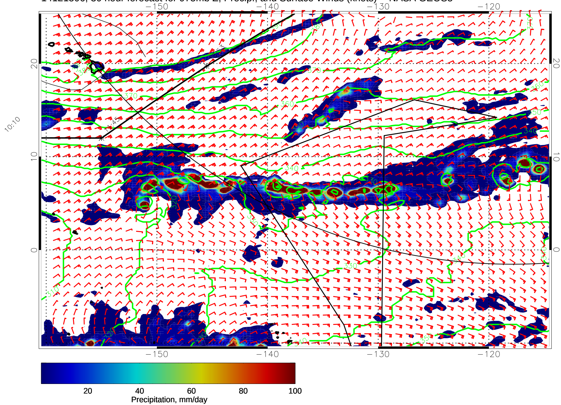
14121506, 30 hour forecast for 975mb Z, Precip., and Surface Winds (knots) -- NASA GEOS5
