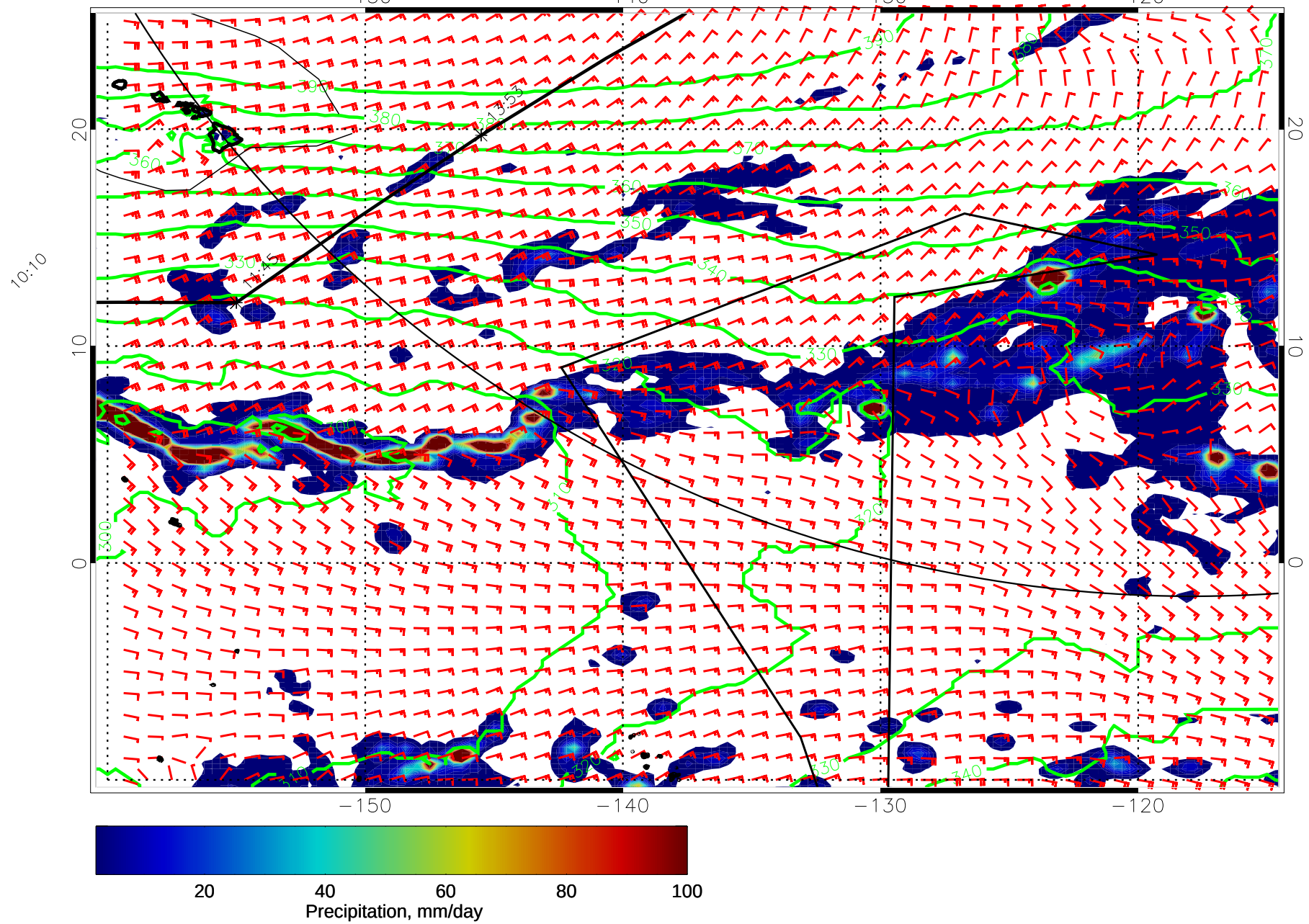
14121700, 72 hour forecast for 975mb Z, Precip., and Surface Winds (knots) -- NASA GEOS5
