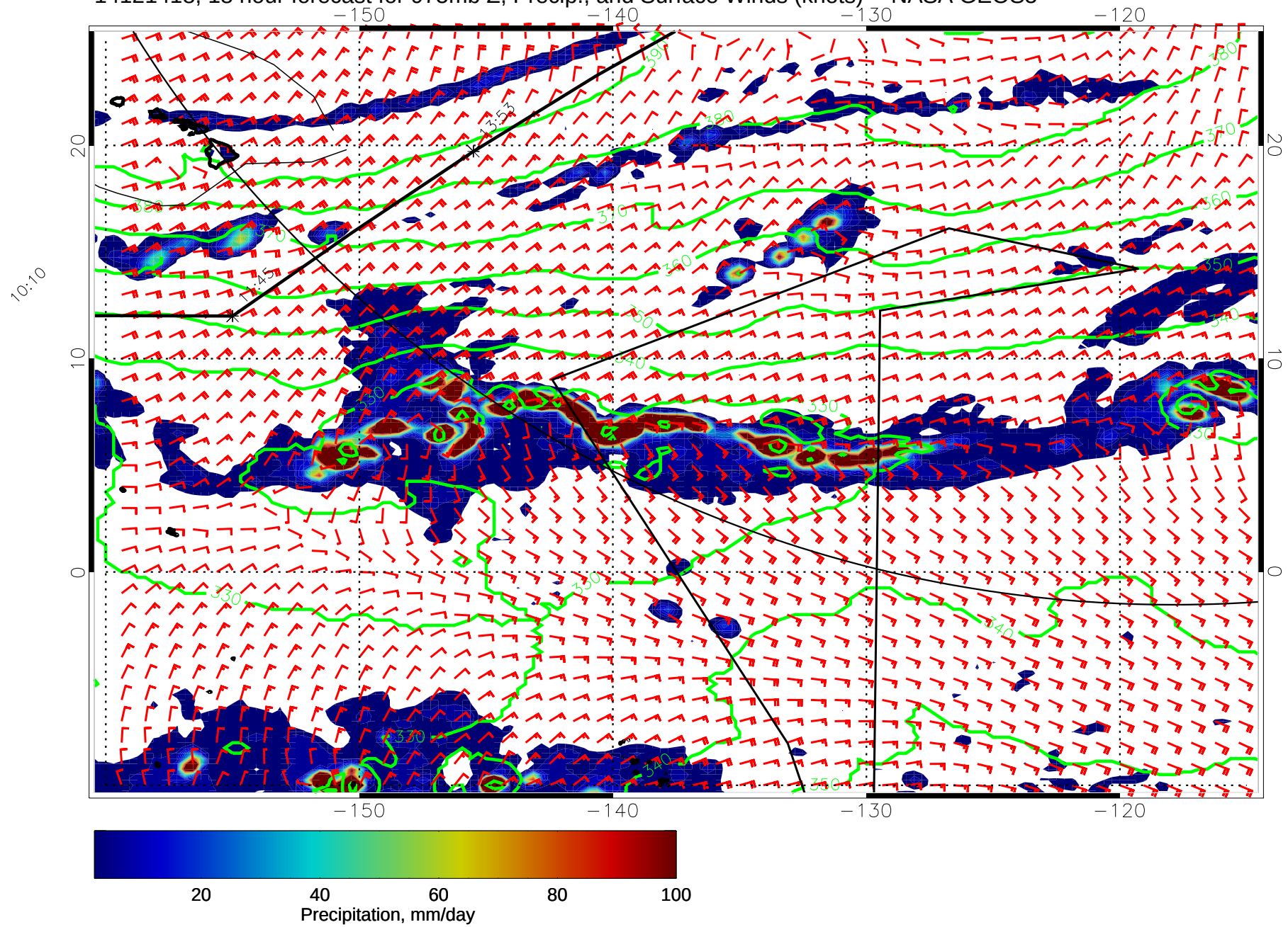
14121418, 18 hour forecast for 975mb Z, Precip., and Surface Winds (knots) -- NASA GEOS5
