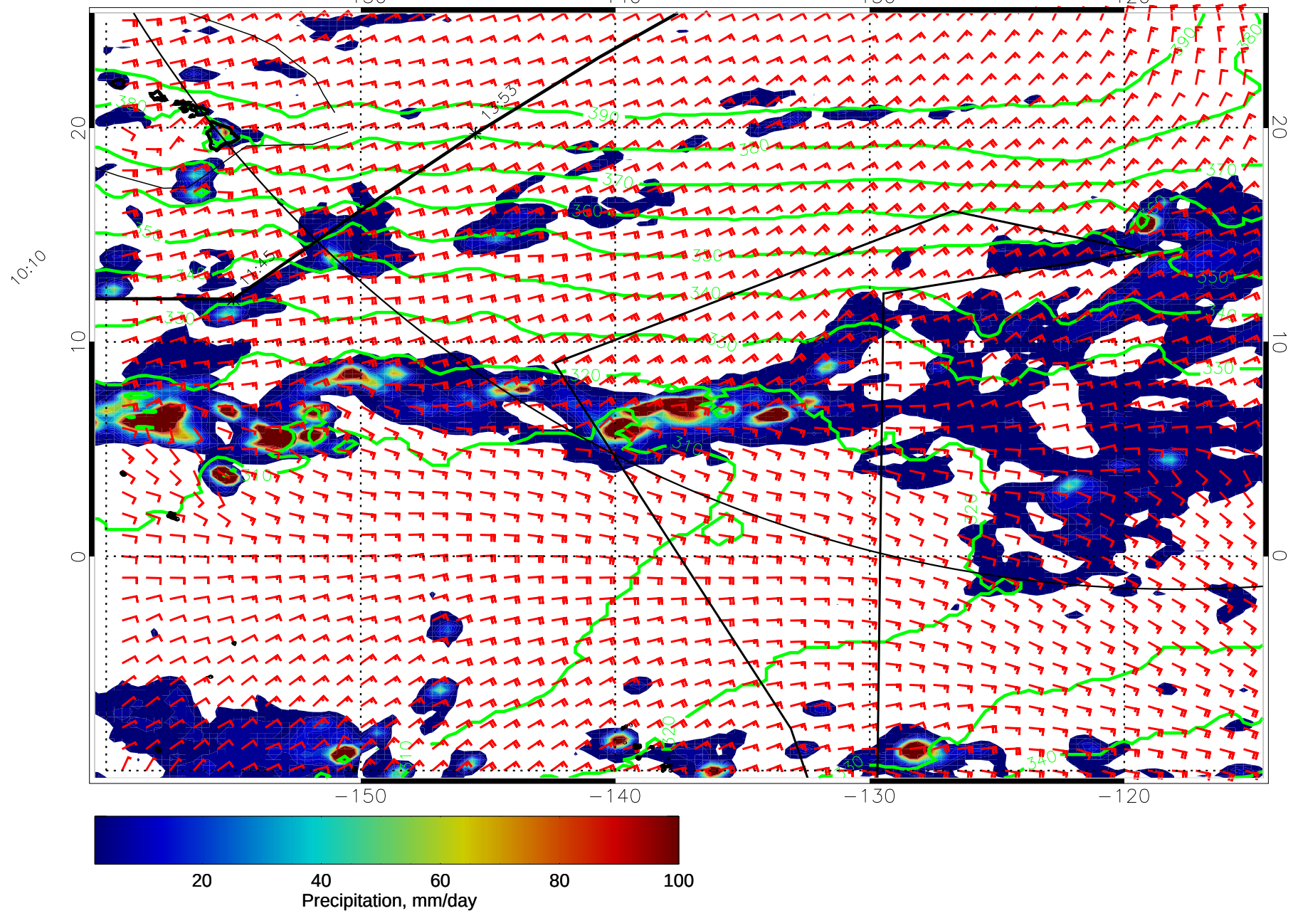
14121800, 96 hour forecast for 975mb Z, Precip., and Surface Winds (knots) -- NASA GEOS5
