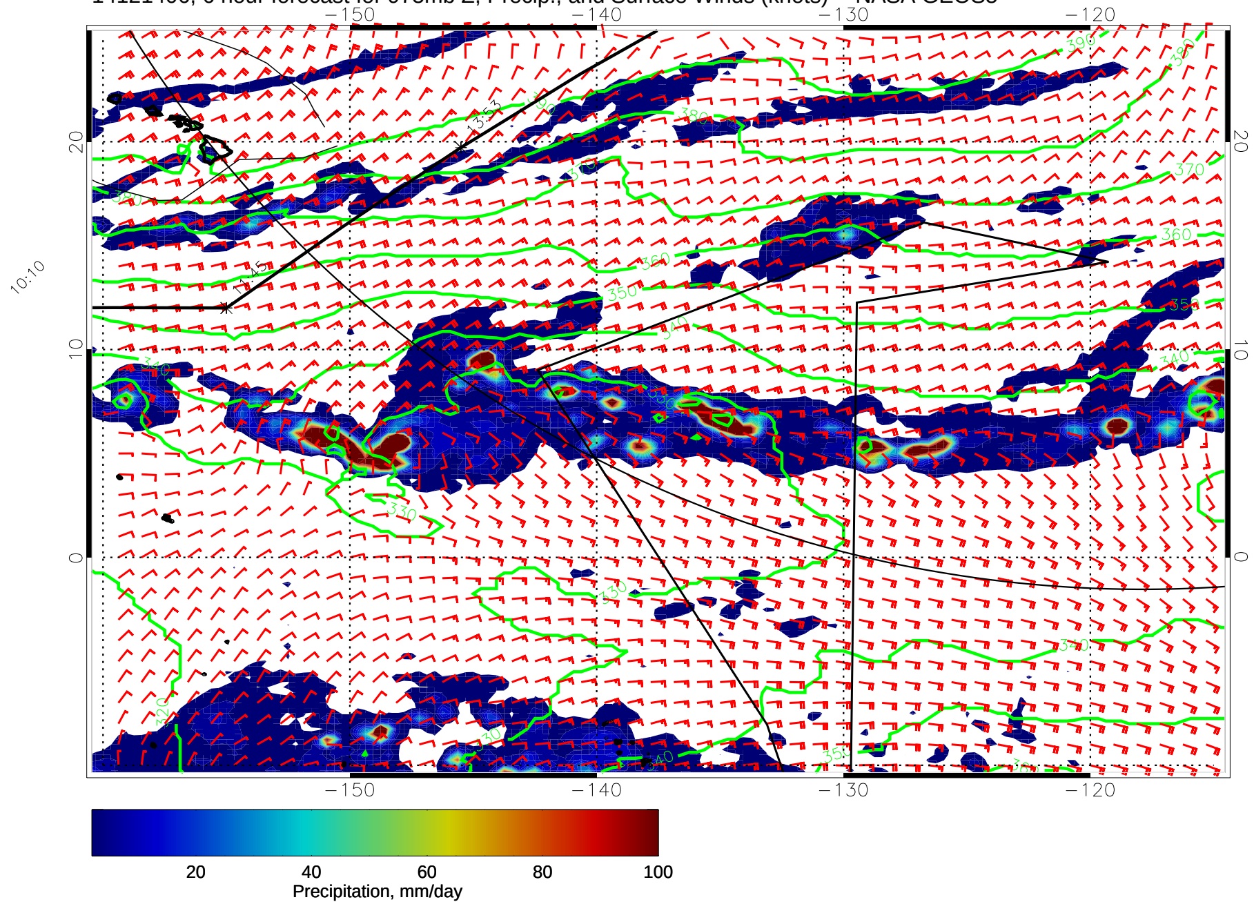
14121406, 6 hour forecast for 975mb Z, Precip., and Surface Winds (knots) -- NASA GEOS5
