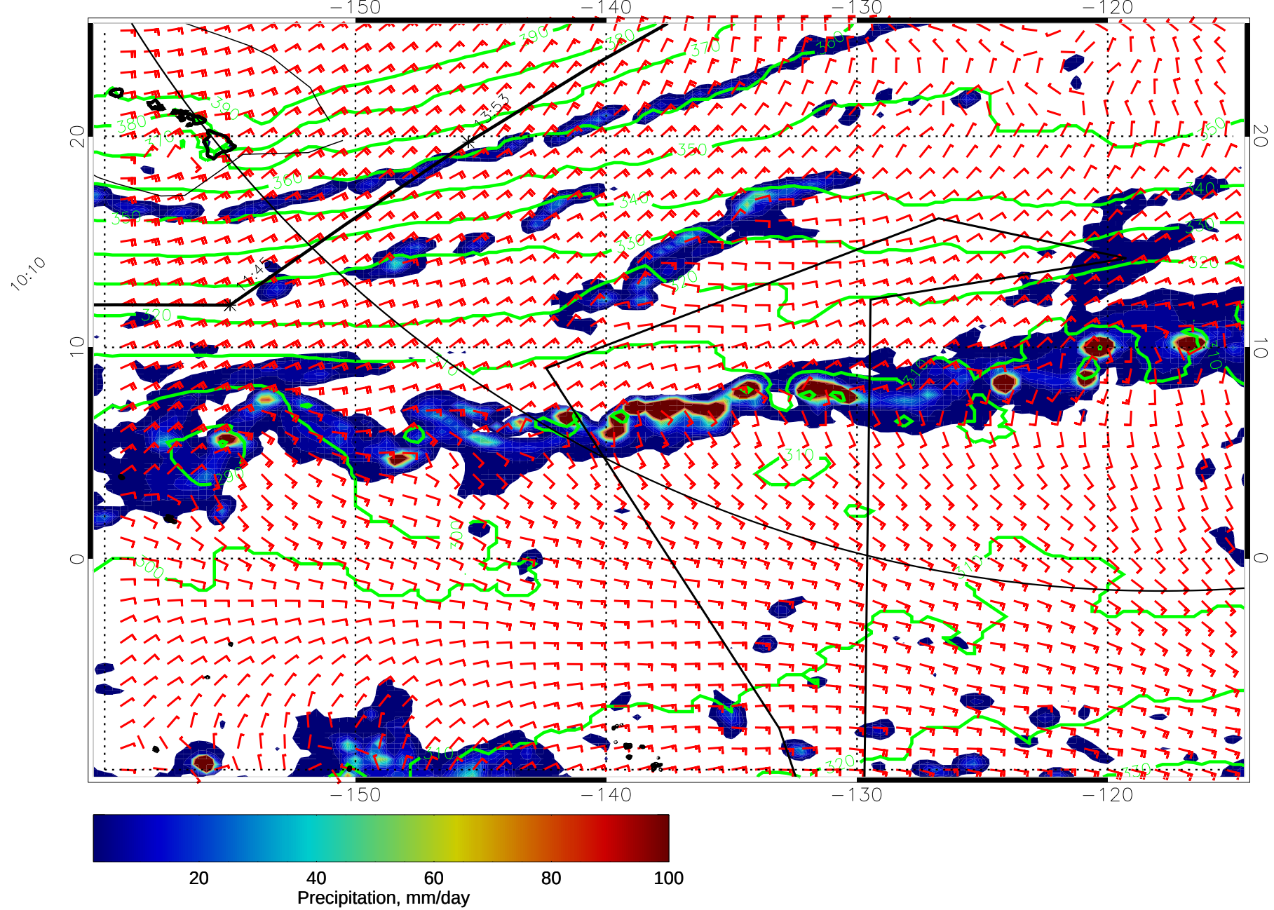
14121600, 48 hour forecast for 975mb Z, Precip., and Surface Winds (knots) -- NASA GEOS5
