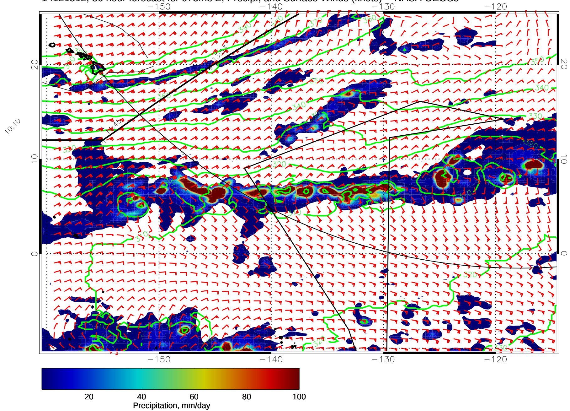
14121512, 36 hour forecast for 975mb Z, Precip., and Surface Winds (knots) -- NASA GEOS5
