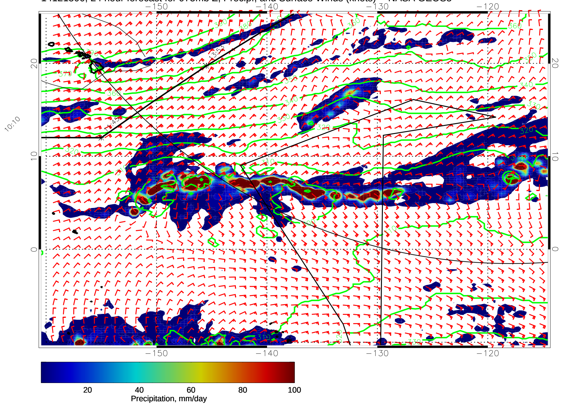
14121500, 24 hour forecast for 975mb Z, Precip., and Surface Winds (knots) -- NASA GEOS5
