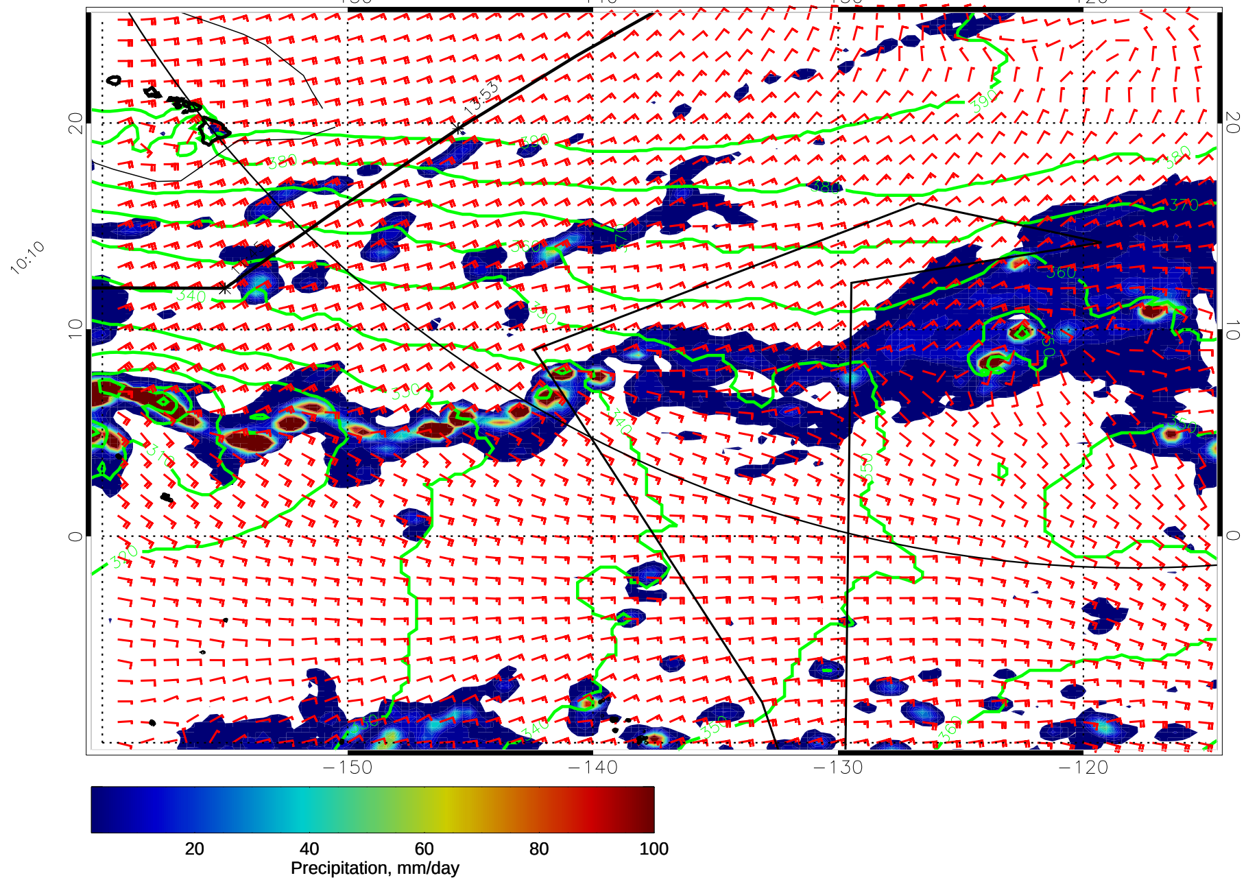
14121618, 66 hour forecast for 975mb Z, Precip., and Surface Winds (knots) -- NASA GEOS5
