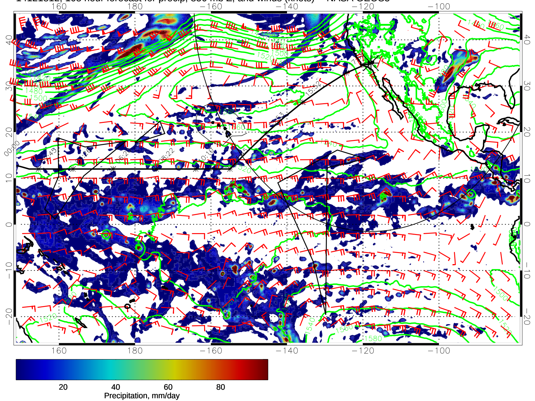
14121812, 108 hour forecast for precip, 850 mb Z, and winds (knots) -- NASA GEOS5
