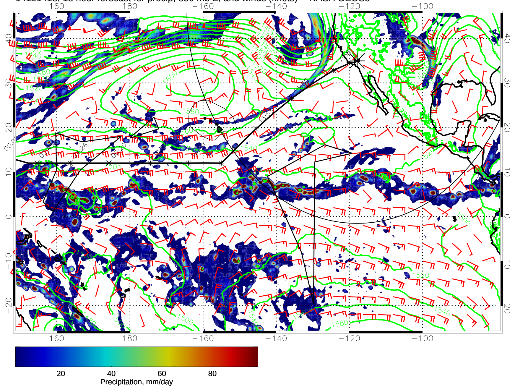
14121418, 18 hour forecast for precip, 850 mb Z, and winds (knots) -- NASA GEOS5
