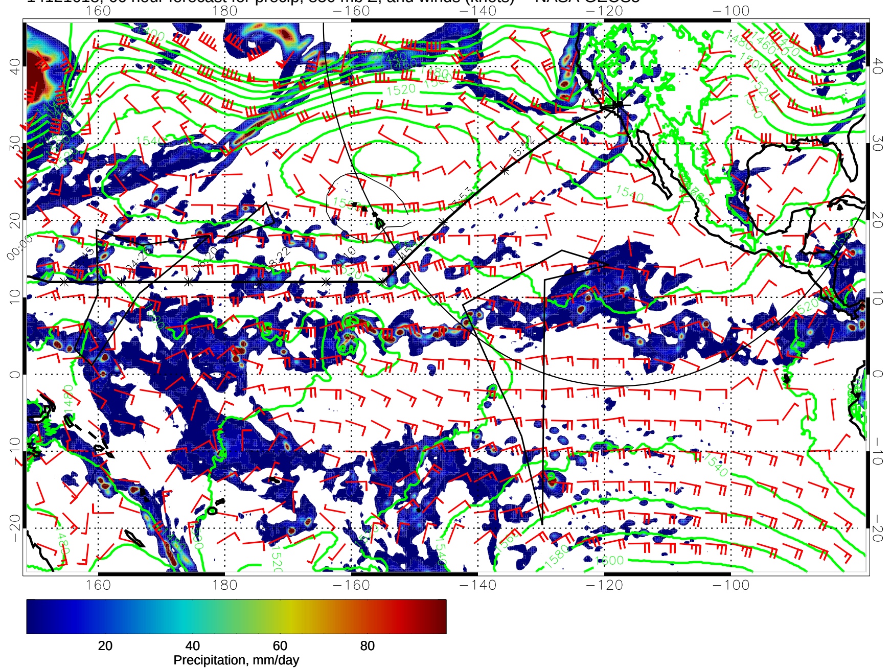
14121618, 66 hour forecast for precip, 850 mb Z, and winds (knots) -- NASA GEOS5
