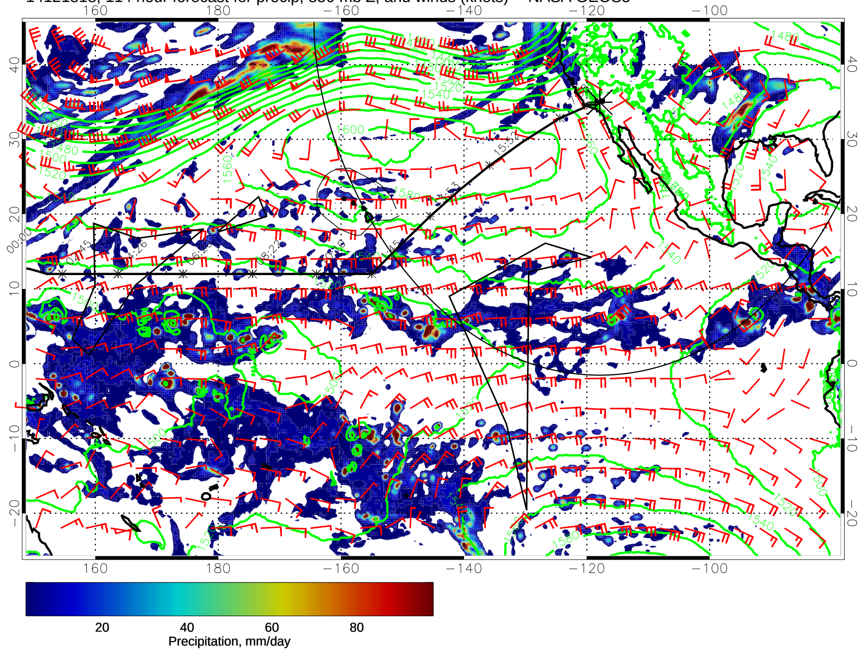
14121818, 114 hour forecast for precip, 850 mb Z, and winds (knots) -- NASA GEOS5
