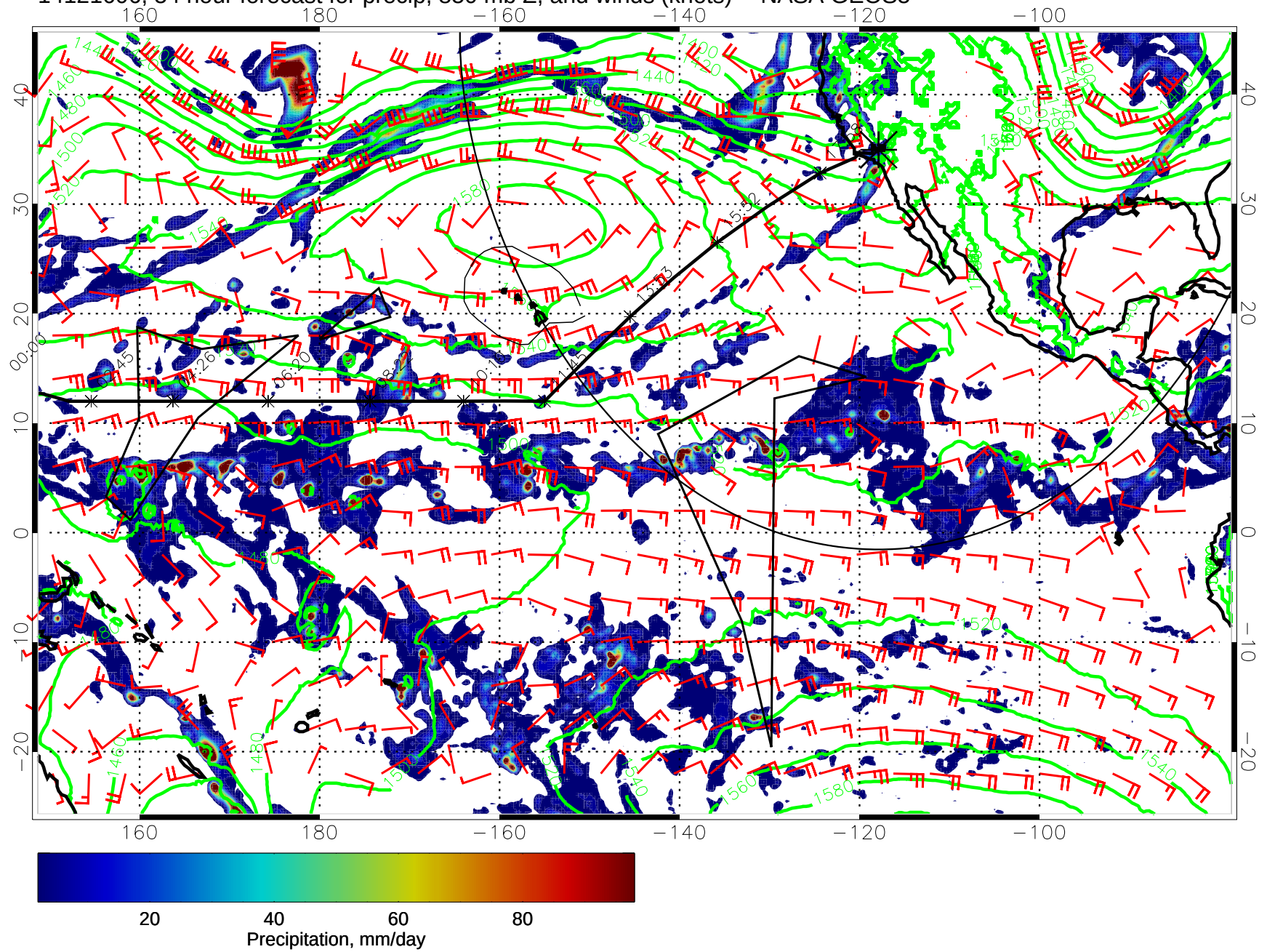
14121606, 54 hour forecast for precip, 850 mb Z, and winds (knots) -- NASA GEOS5
