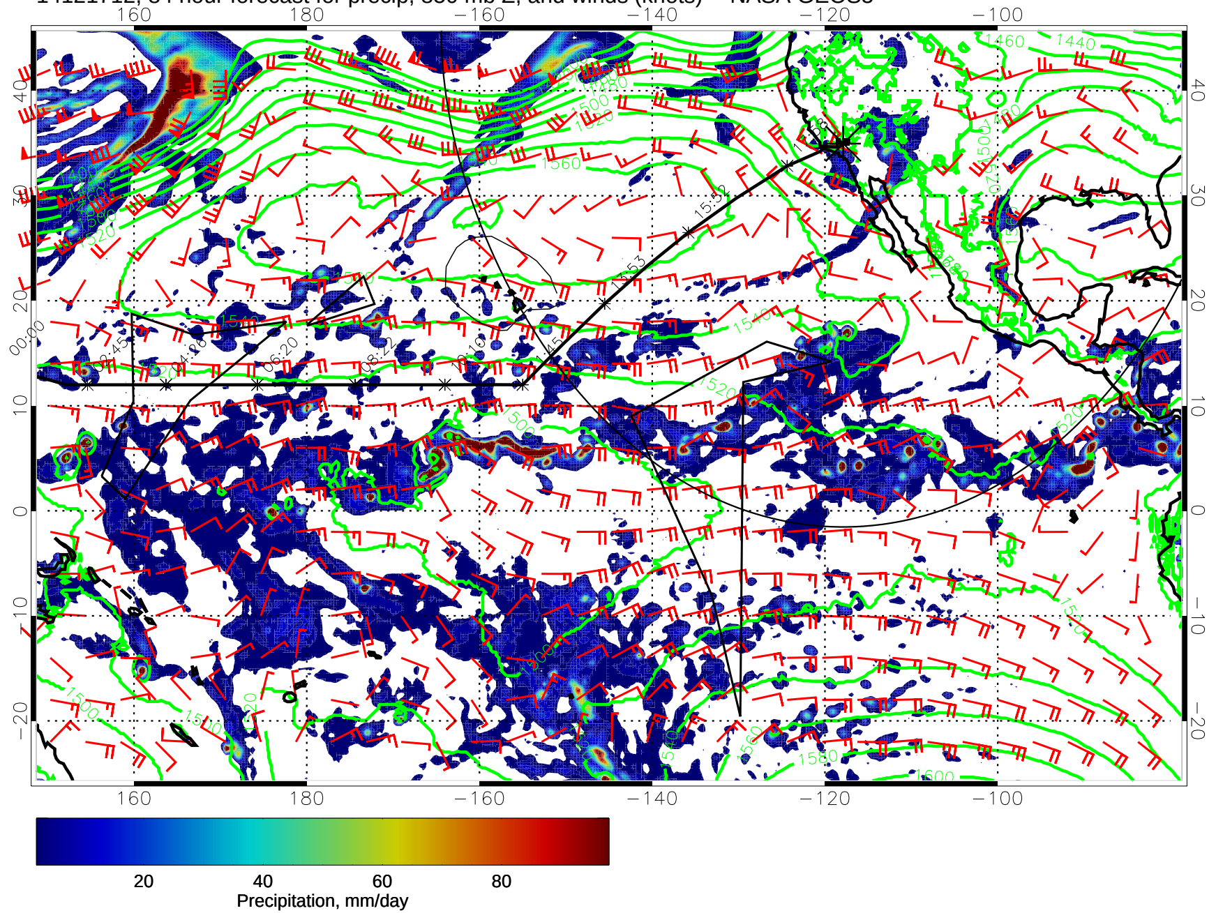
14121712, 84 hour forecast for precip, 850 mb Z, and winds (knots) -- NASA GEOS5
