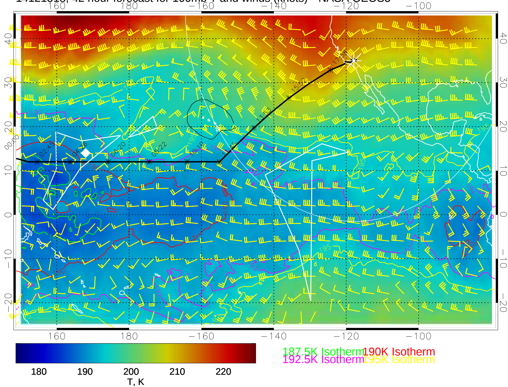
14121518, 42 hour forecast for 100mb T and winds (knots)-- NASA GEOS5
