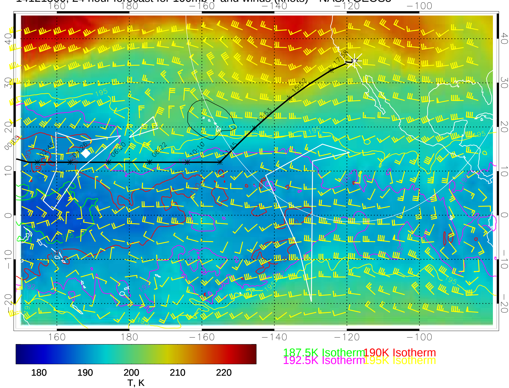
14121500, 24 hour forecast for 100mb T and winds (knots)-- NASA GEOS5
