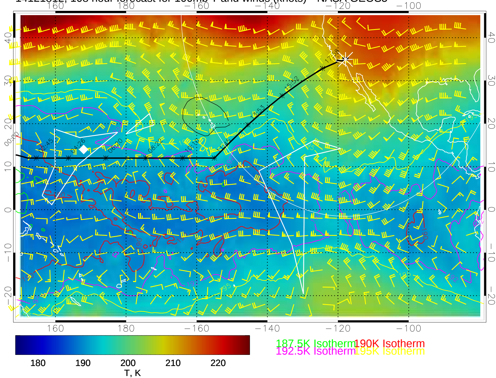
14121812, 108 hour forecast for 100mb T and winds (knots)-- NASA GEOS5
