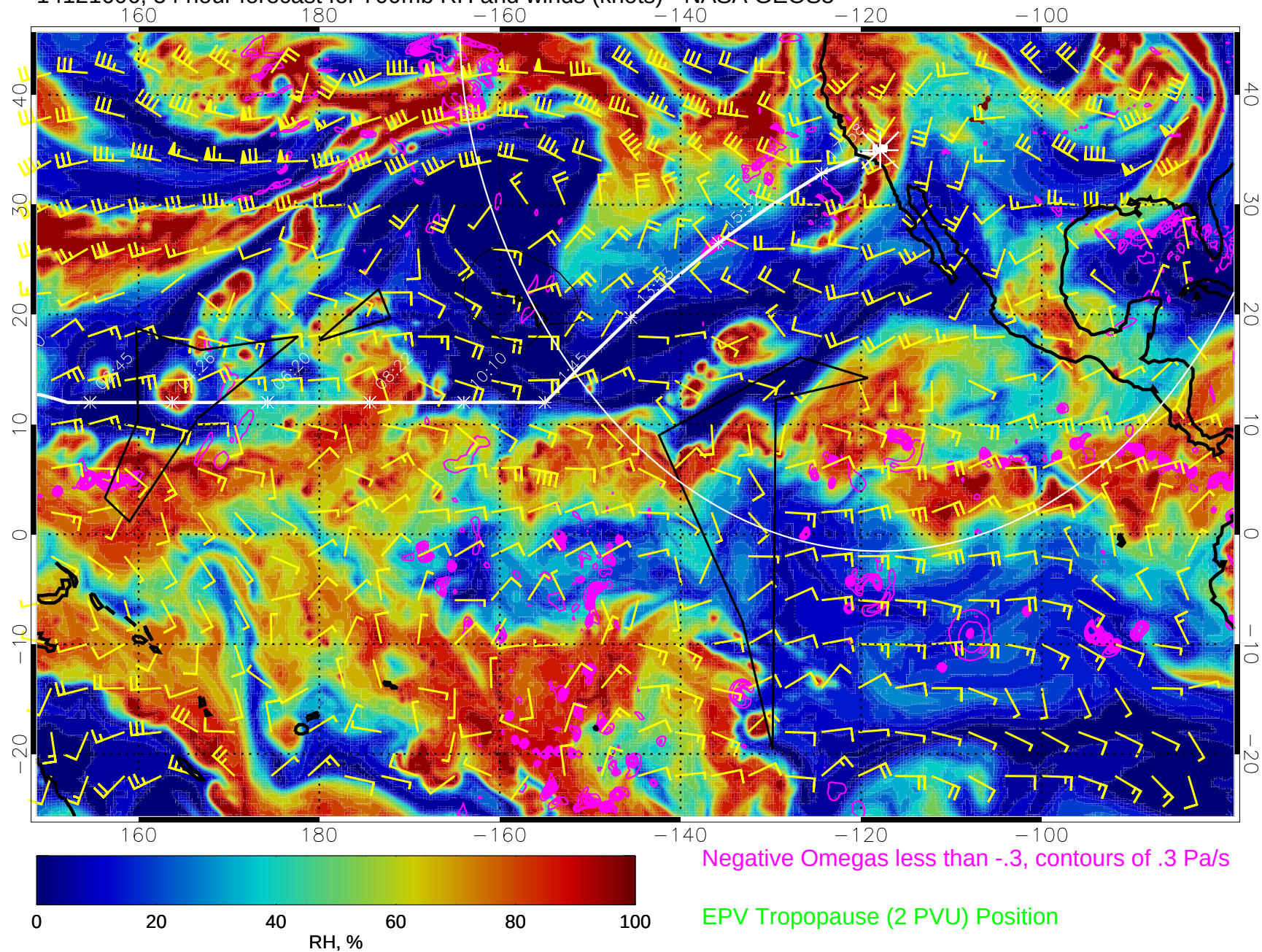
14121606, 54 hour forecast for 700mb RH and winds (knots) - NASA GEOS5
