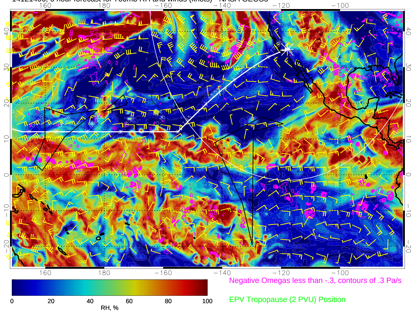
14121406, 6 hour forecast for 700mb RH and winds (knots) - NASA GEOS5
