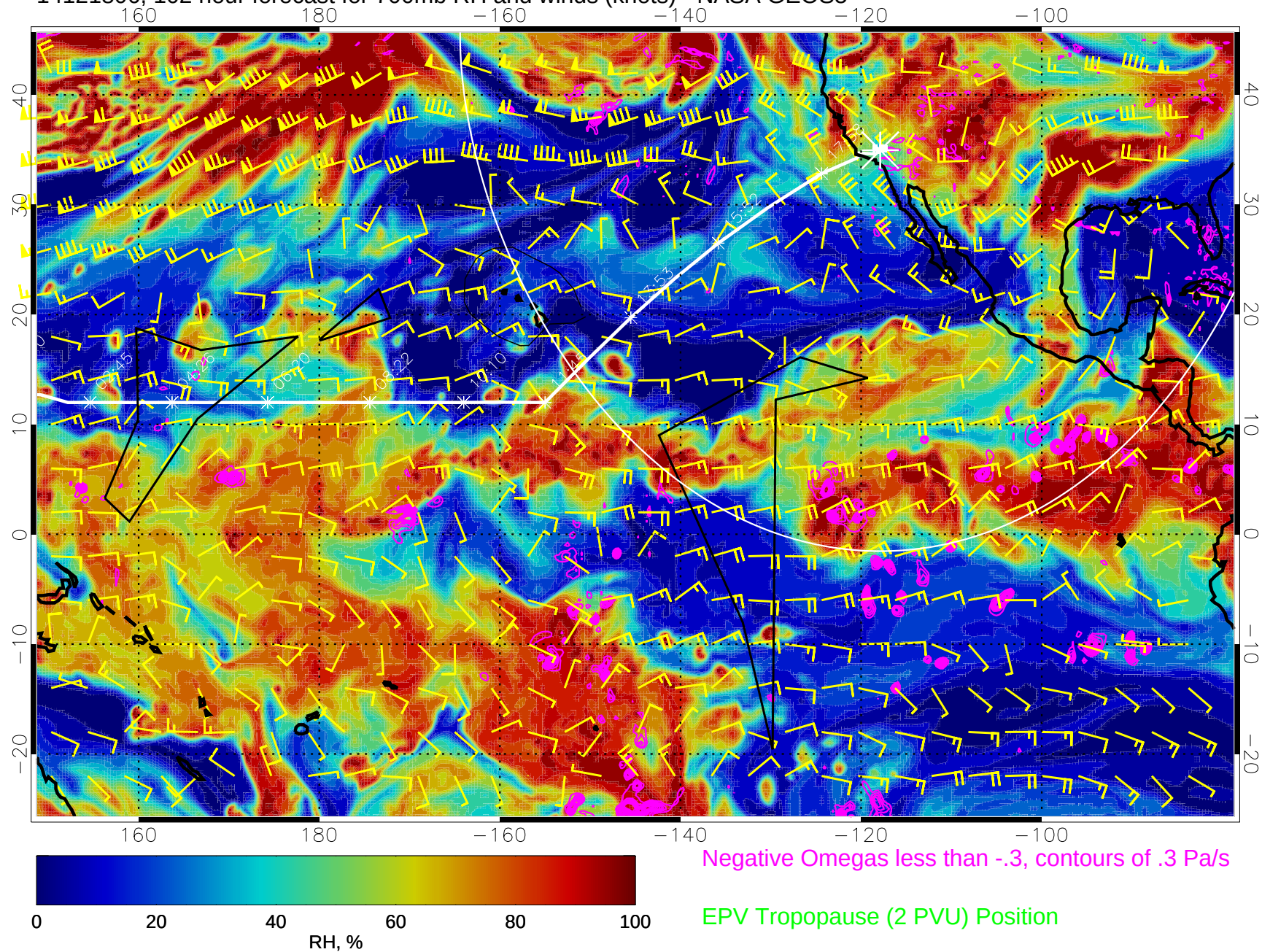
14121806, 102 hour forecast for 700mb RH and winds (knots) - NASA GEOS5
