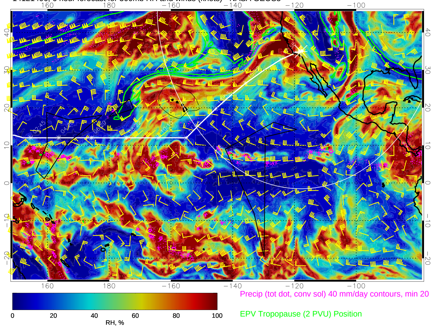
14121406, 6 hour forecast for 300mb RH and winds (knots) - NASA GEOS5
