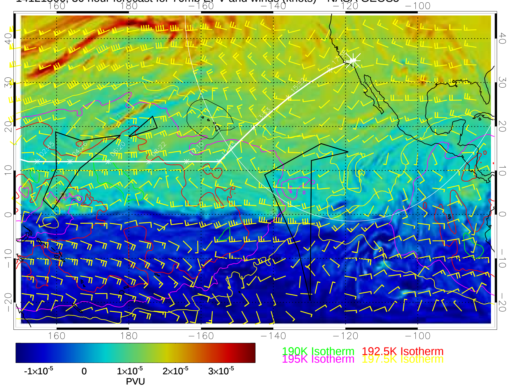
14121506, 30 hour forecast for 70mb EPV and winds (knots)-- NASA GEOS5
