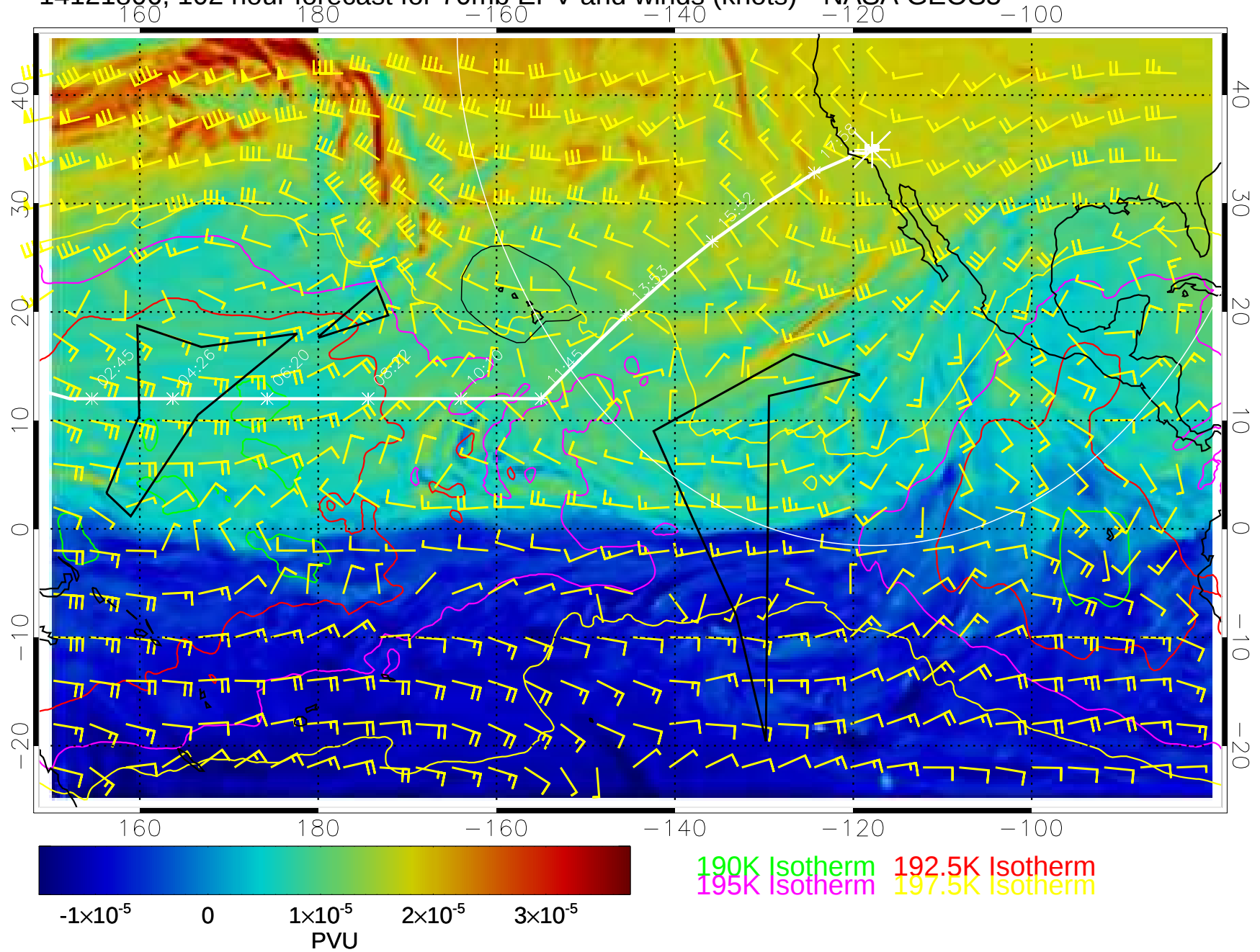
14121806, 102 hour forecast for 70mb EPV and winds (knots)-- NASA GEOS5
