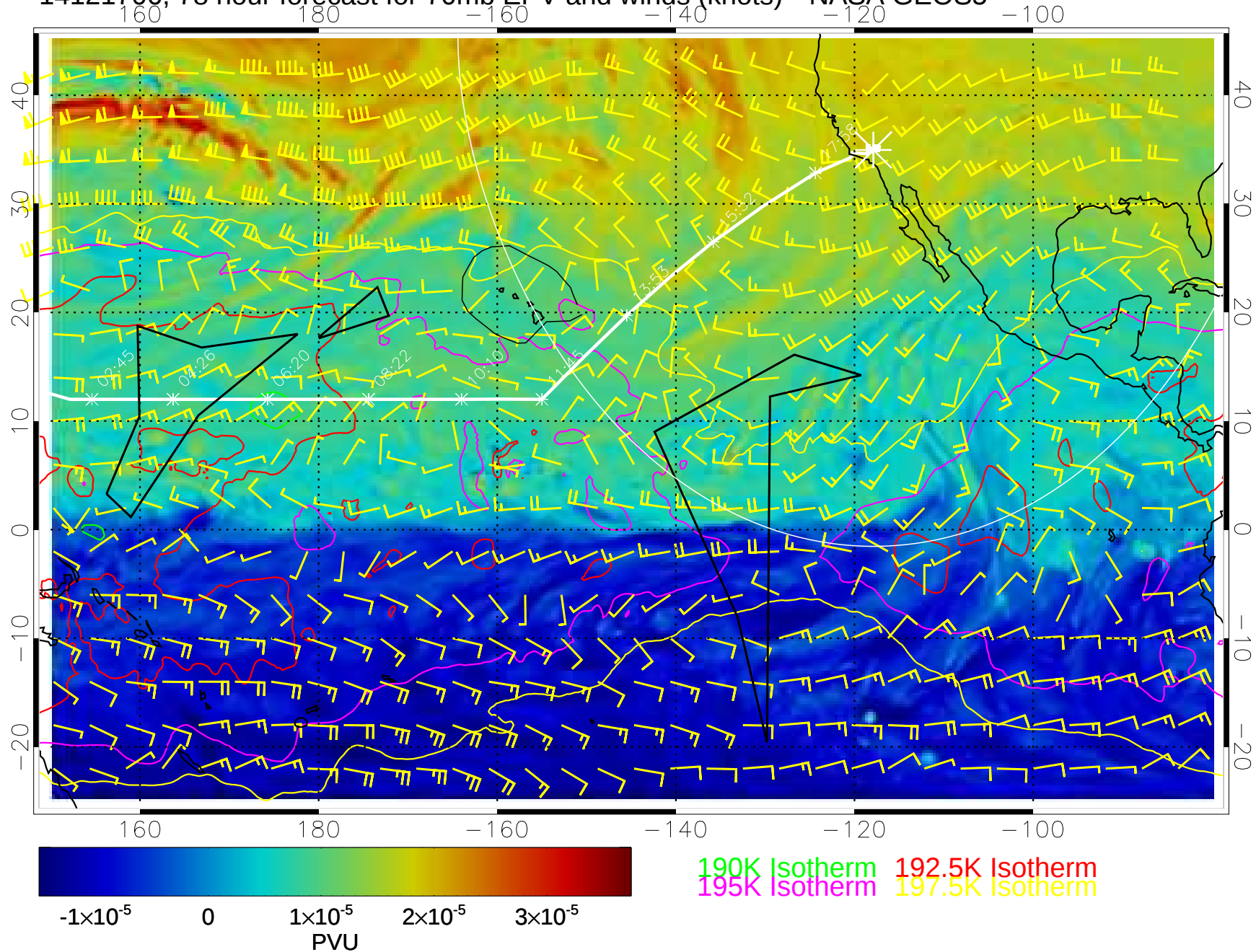
14121706, 78 hour forecast for 70mb EPV and winds (knots)-- NASA GEOS5
