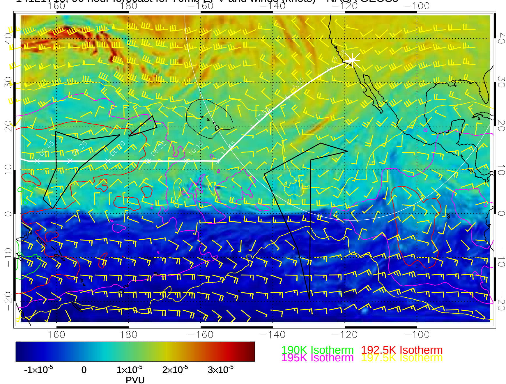
14121718, 90 hour forecast for 70mb EPV and winds (knots)-- NASA GEOS5
