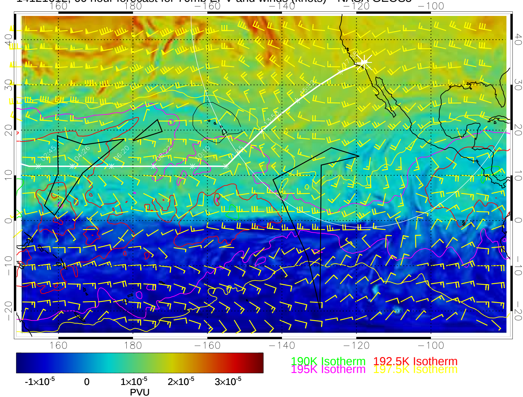
14121612, 60 hour forecast for 70mb EPV and winds (knots)-- NASA GEOS5
