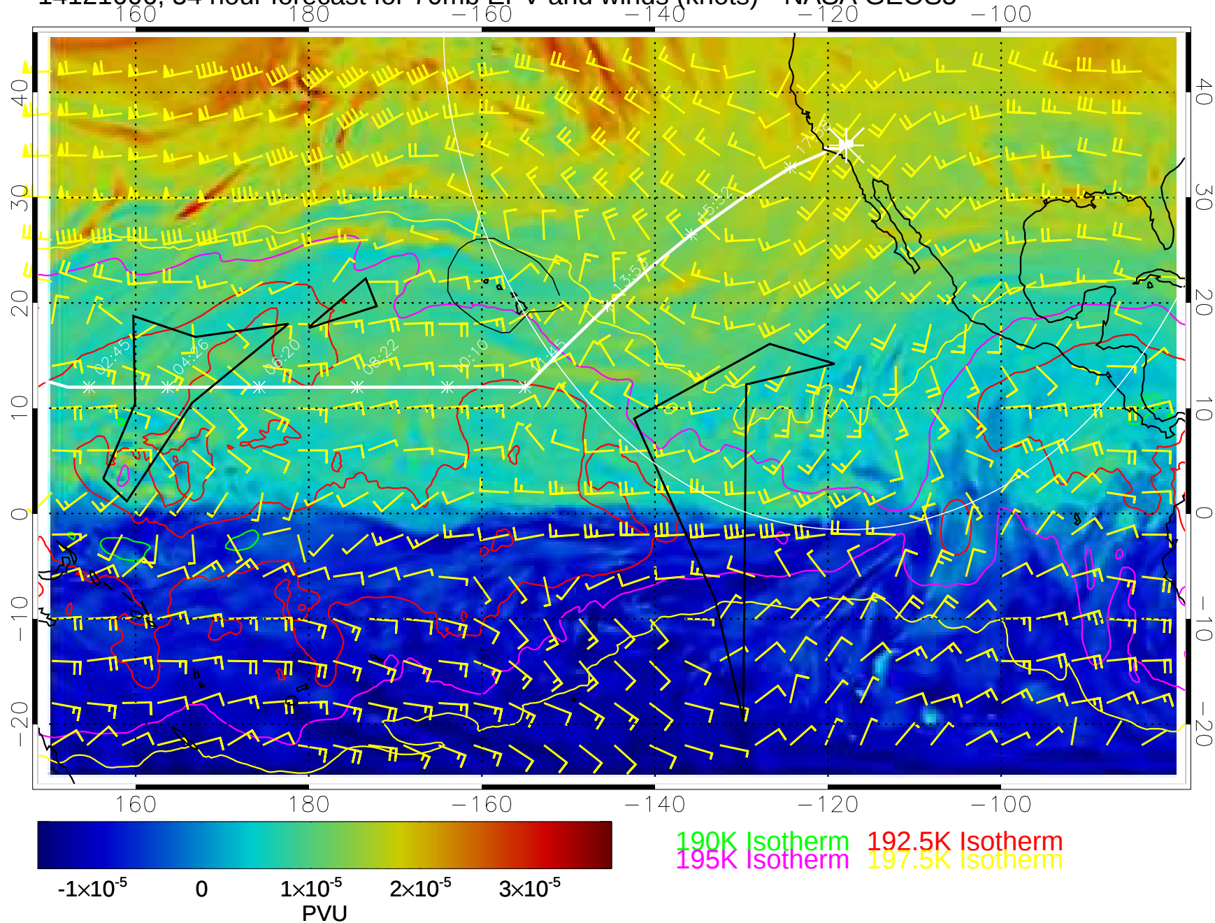
14121606, 54 hour forecast for 70mb EPV and winds (knots)-- NASA GEOS5
