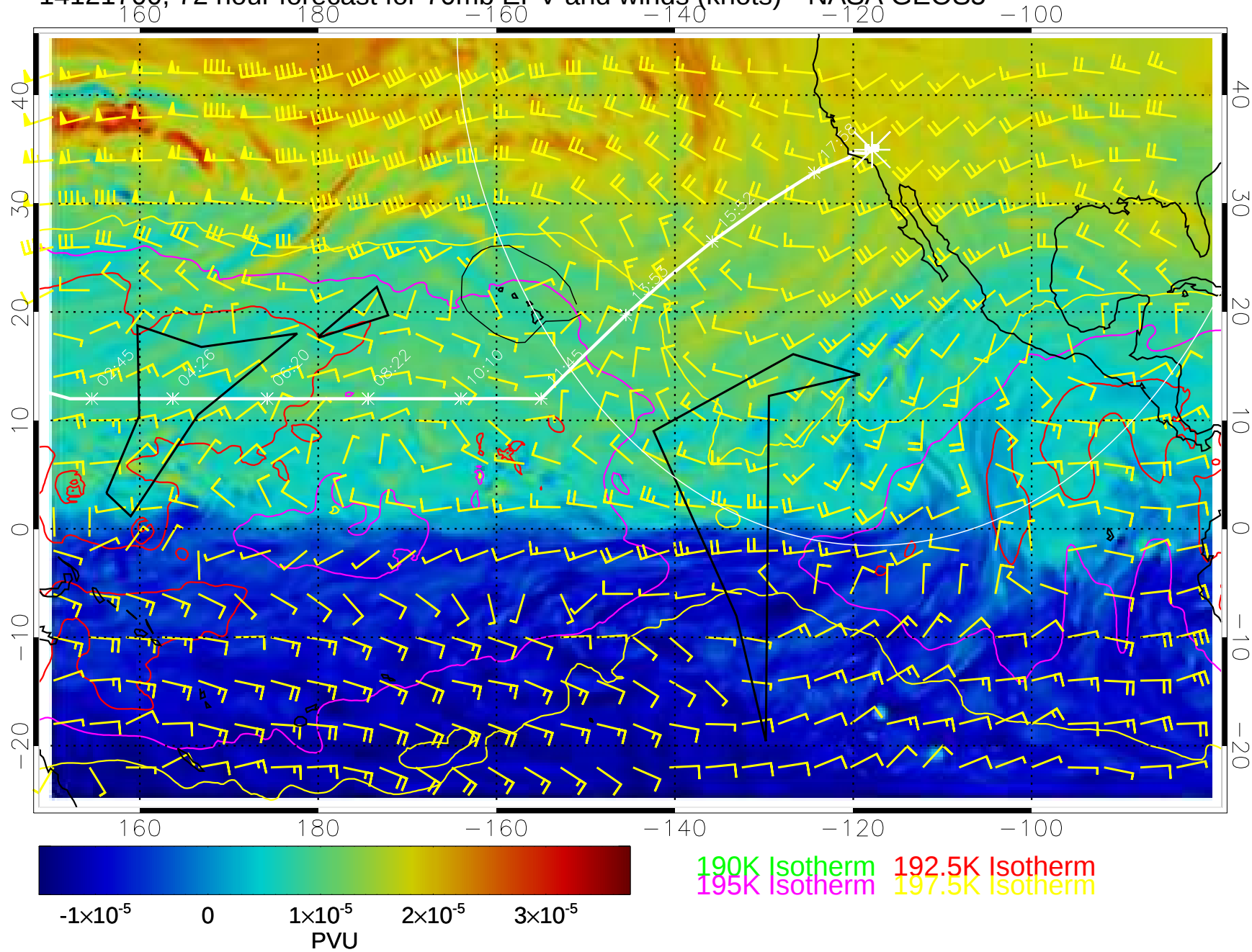
14121700, 72 hour forecast for 70mb EPV and winds (knots)-- NASA GEOS5
