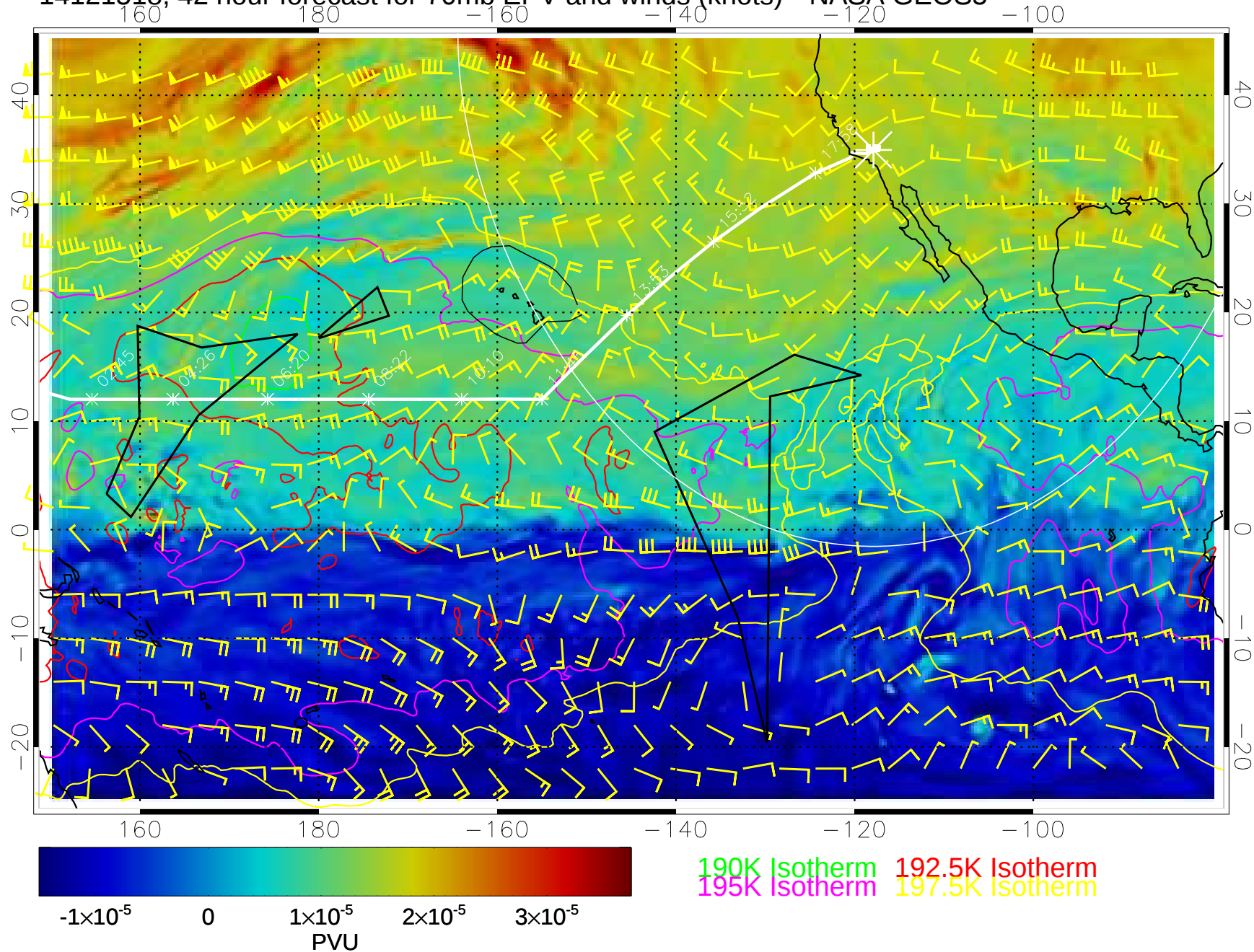
14121518, 42 hour forecast for 70mb EPV and winds (knots)-- NASA GEOS5
