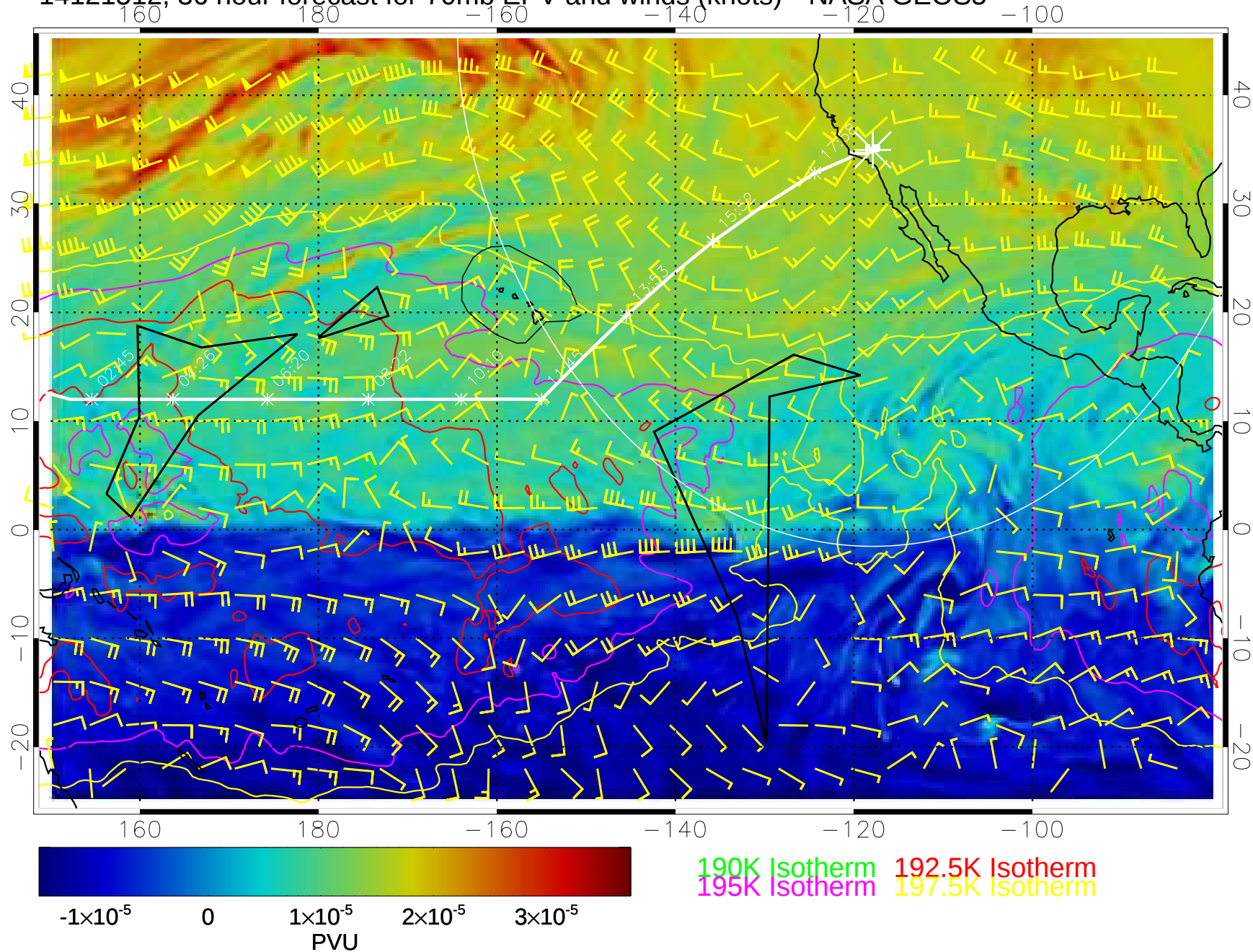
14121512, 36 hour forecast for 70mb EPV and winds (knots)-- NASA GEOS5
