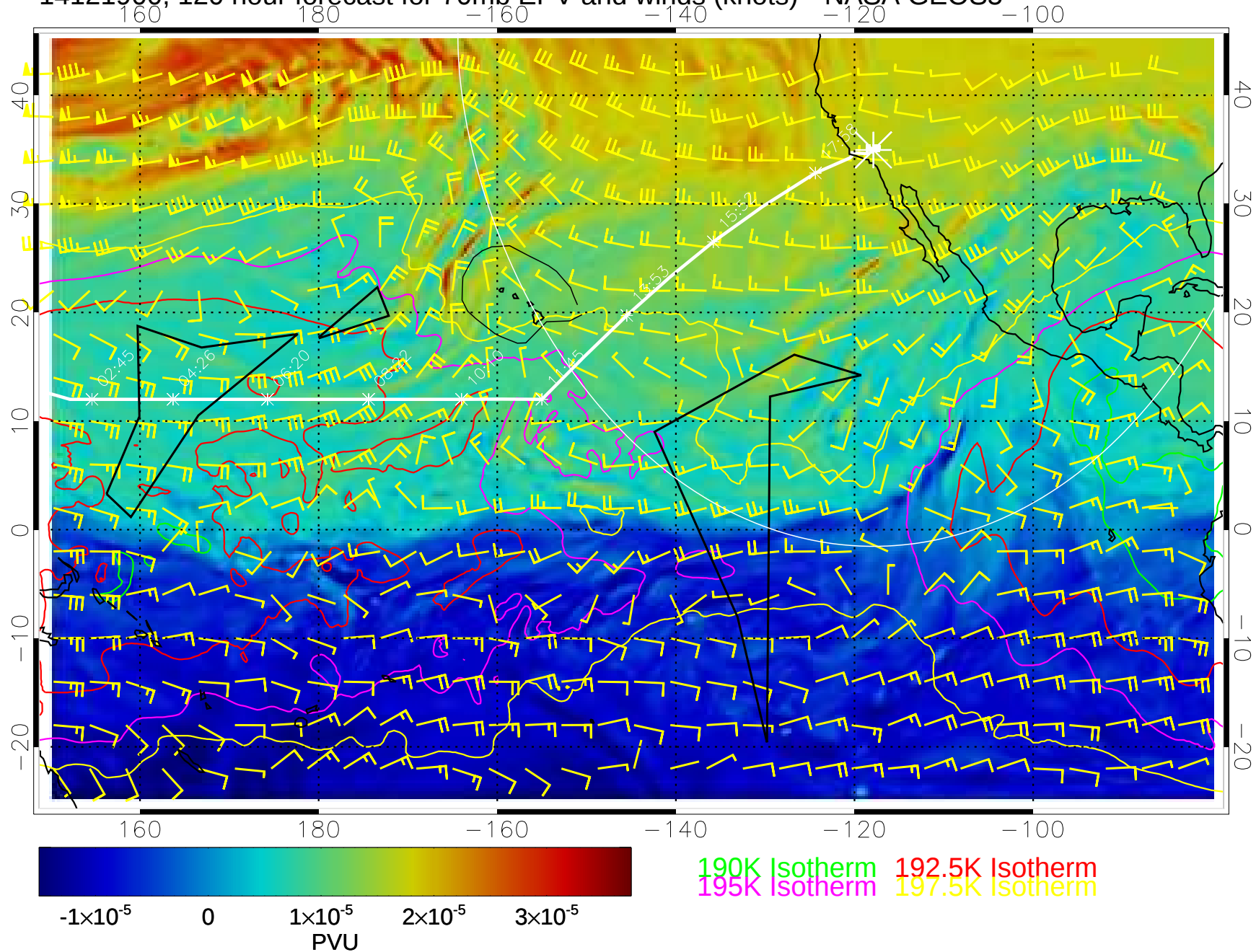
14121900, 120 hour forecast for 70mb EPV and winds (knots)-- NASA GEOS5
