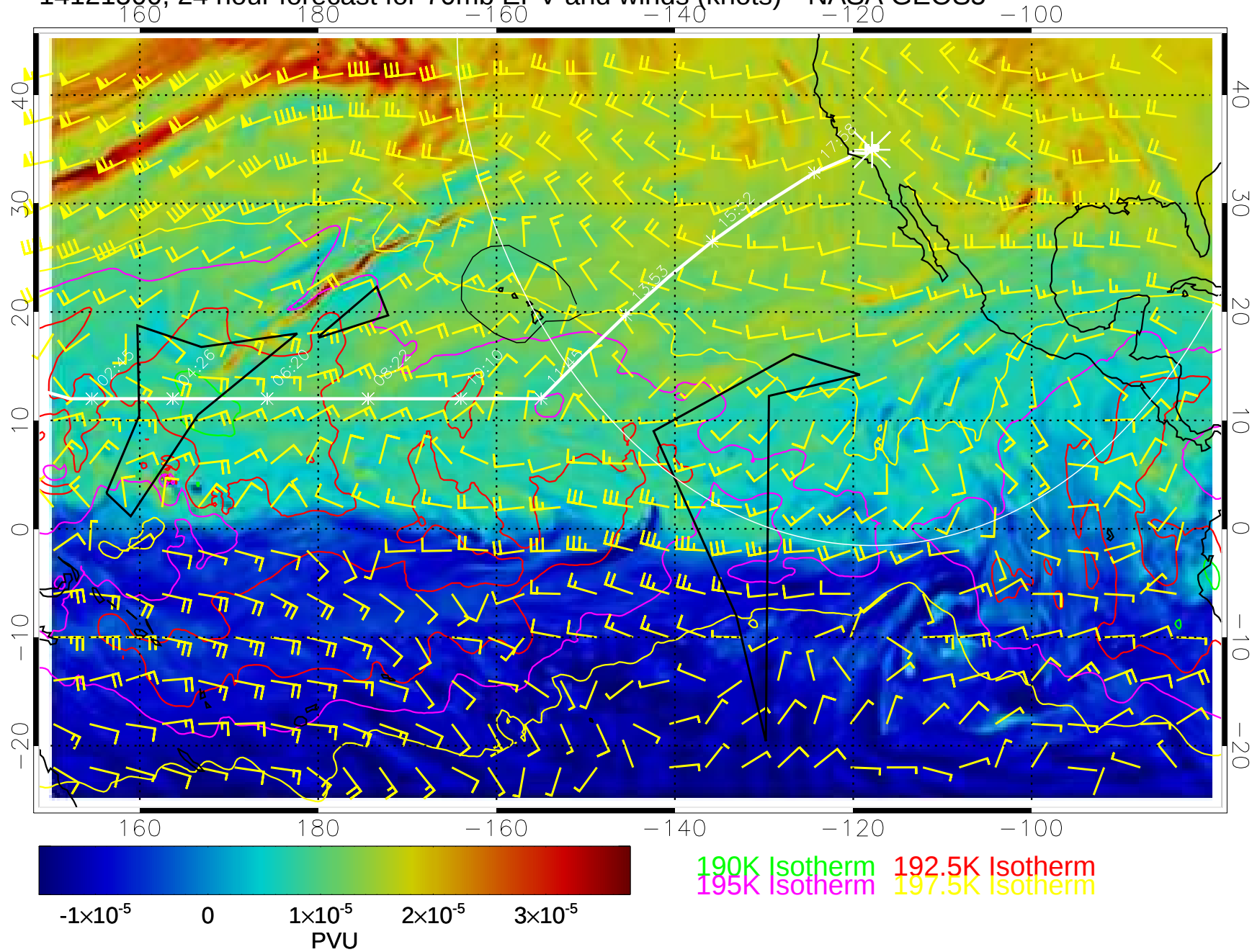
14121500, 24 hour forecast for 70mb EPV and winds (knots)-- NASA GEOS5
