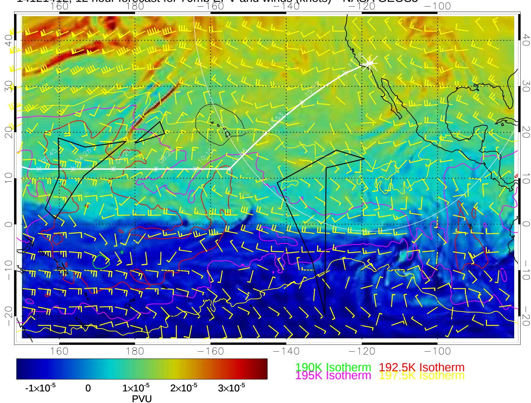
14121412, 12 hour forecast for 70mb EPV and winds (knots)-- NASA GEOS5
