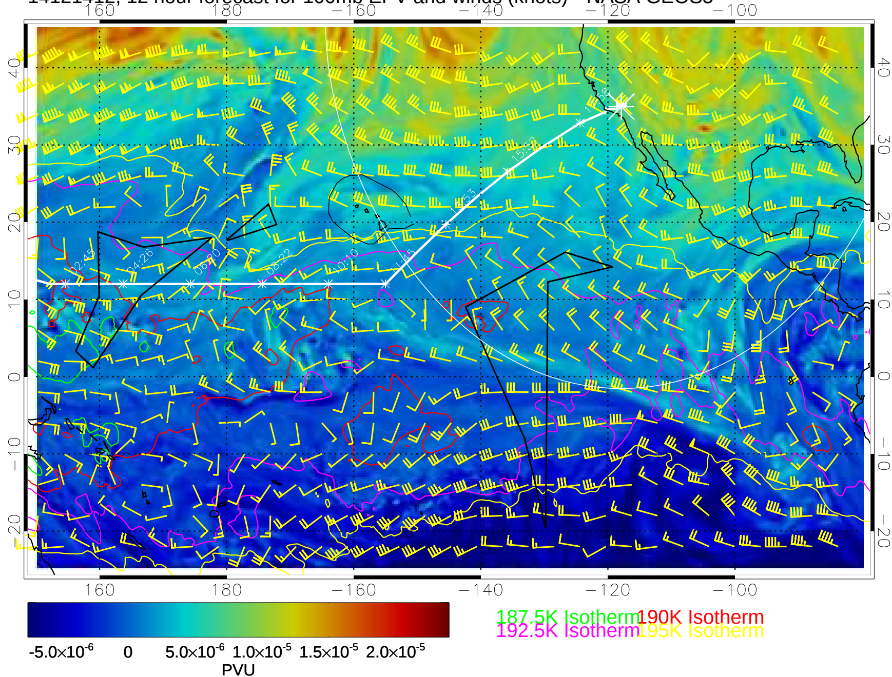
14121412, 12 hour forecast for 100mb EPV and winds (knots)-- NASA GEOS5
