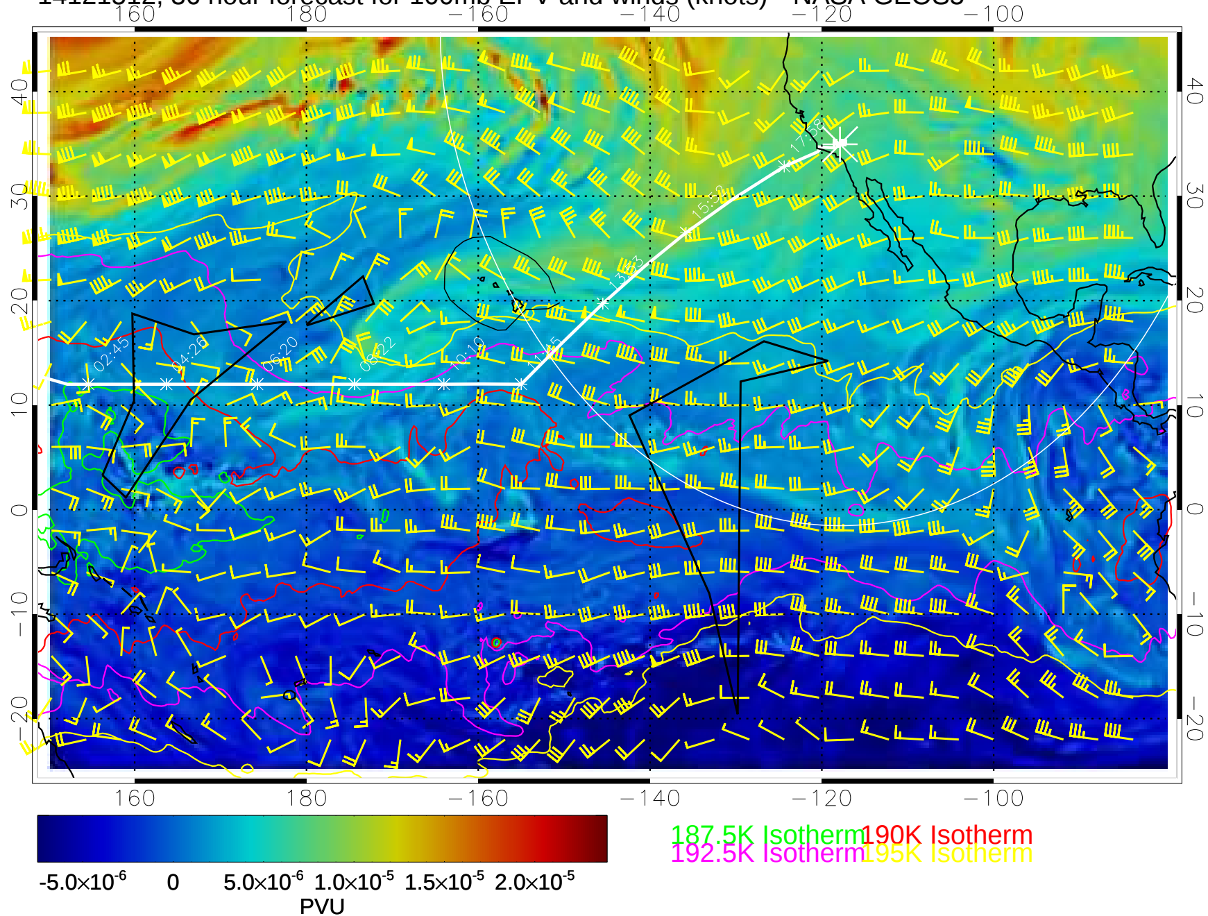
14121512, 36 hour forecast for 100mb EPV and winds (knots)-- NASA GEOS5
