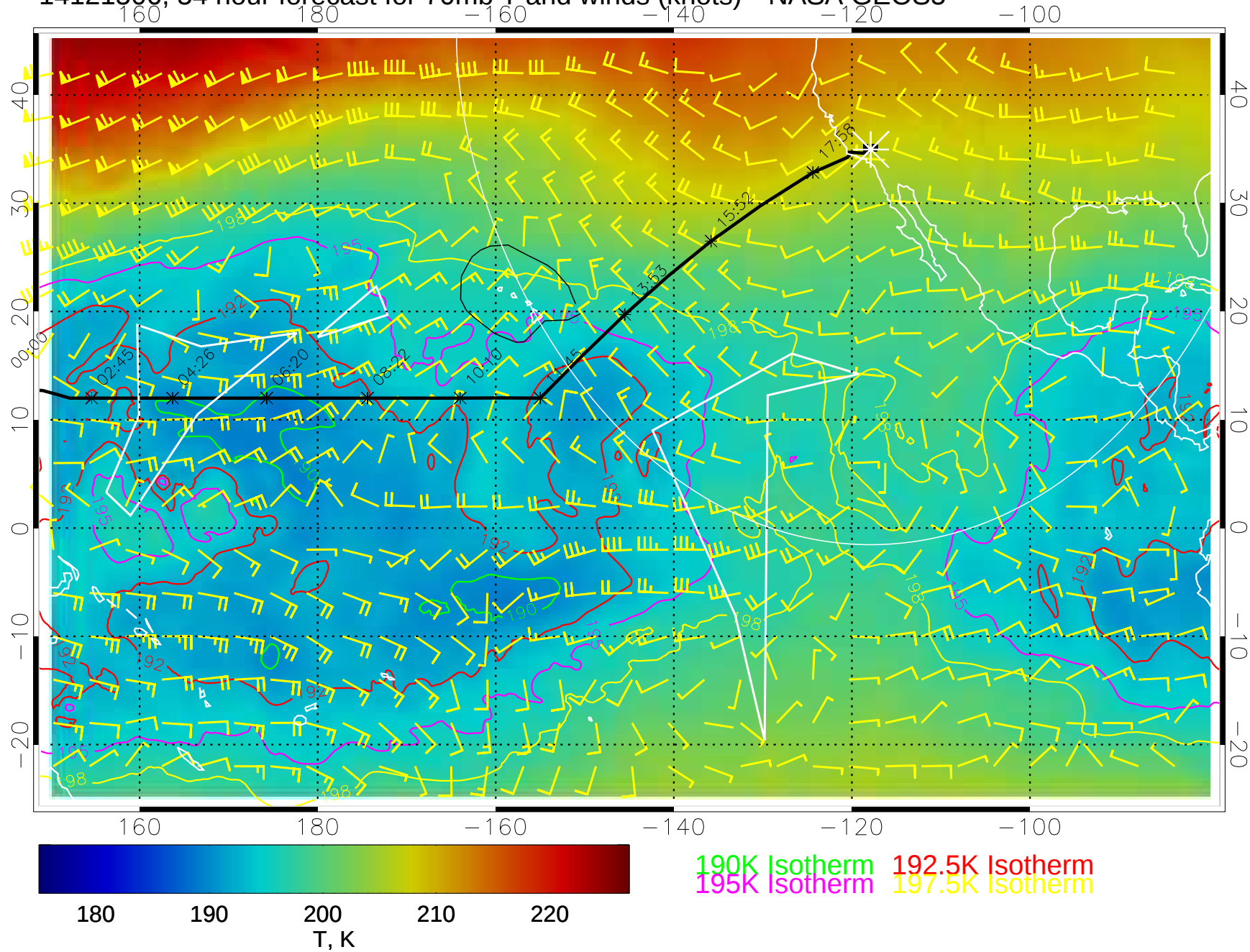
14121506, 54 hour forecast for 70mb T and winds (knots)-- NASA GEOS5
