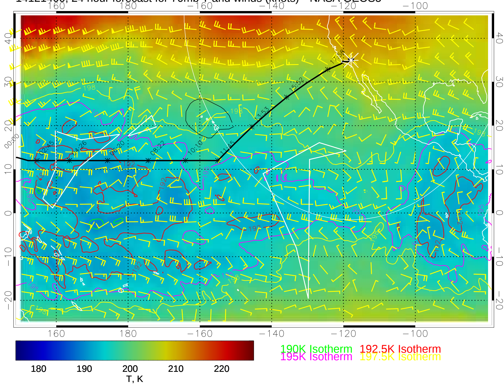
14121400, 24 hour forecast for 70mb T and winds (knots)-- NASA GEOS5
