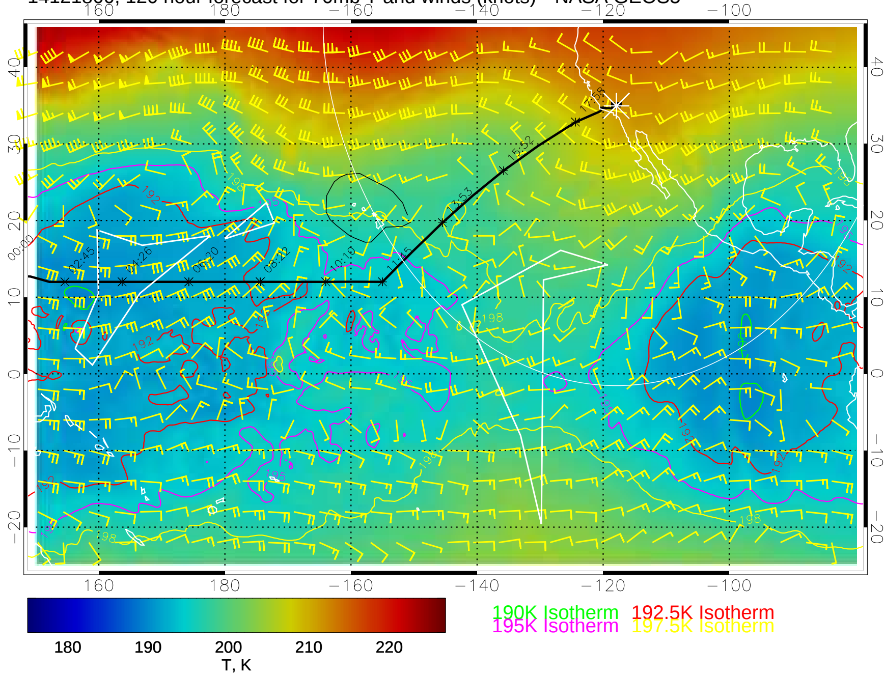
14121800, 120 hour forecast for 70mb T and winds (knots)-- NASA GEOS5
