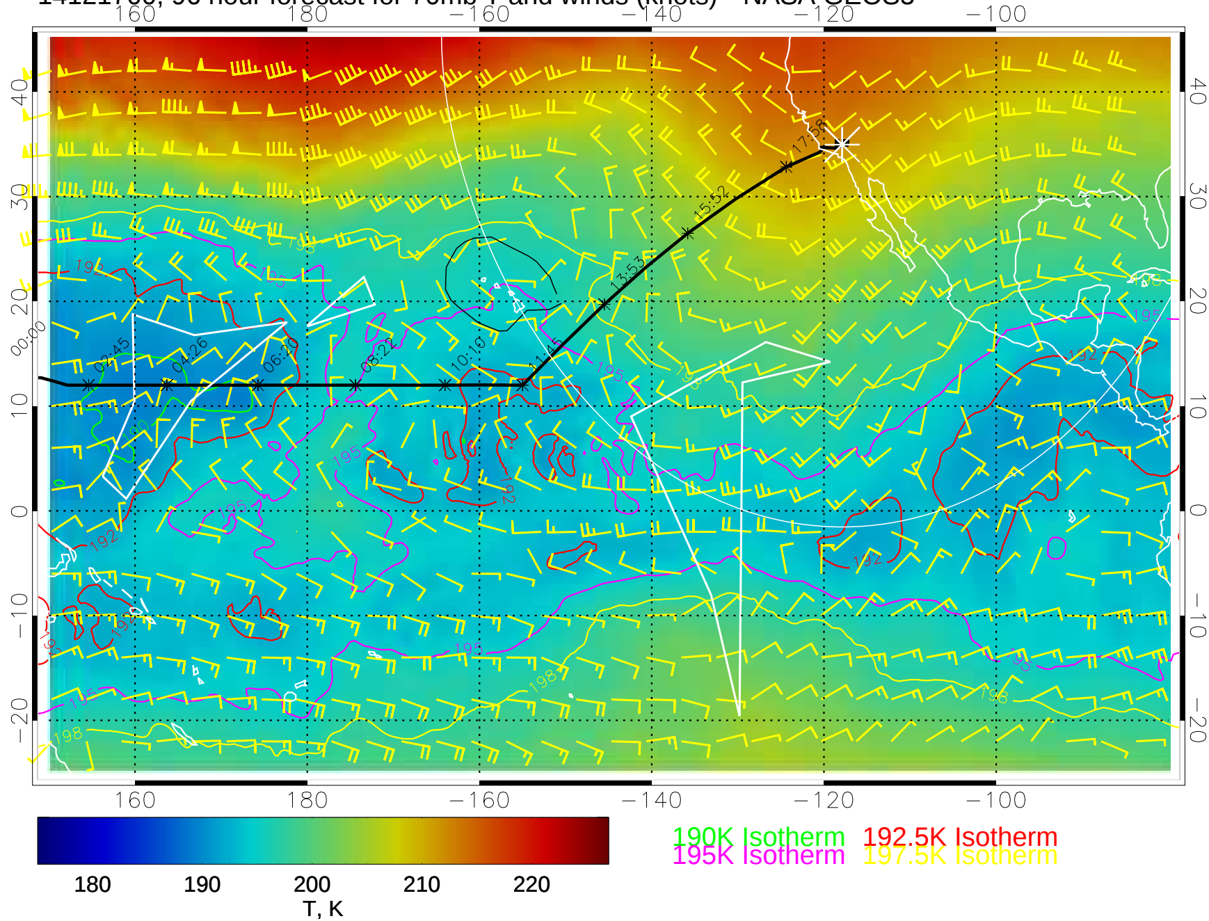
14121700, 96 hour forecast for 70mb T and winds (knots)-- NASA GEOS5
