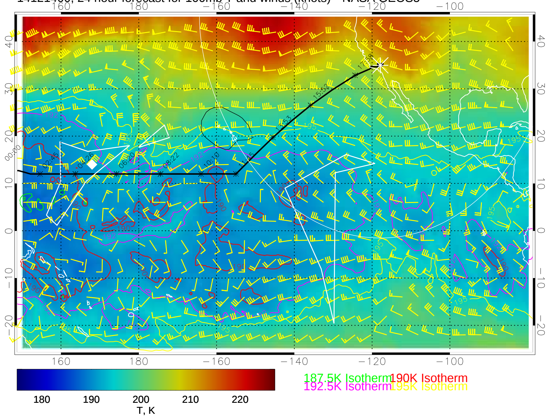
14121400, 24 hour forecast for 100mb T and winds (knots)-- NASA GEOS5
