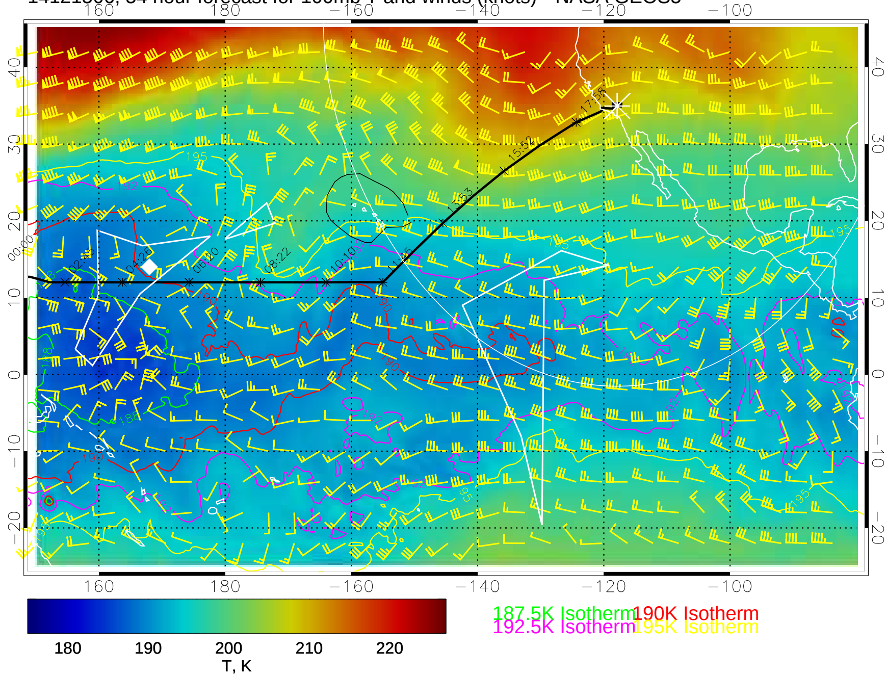
14121506, 54 hour forecast for 100mb T and winds (knots)-- NASA GEOS5
