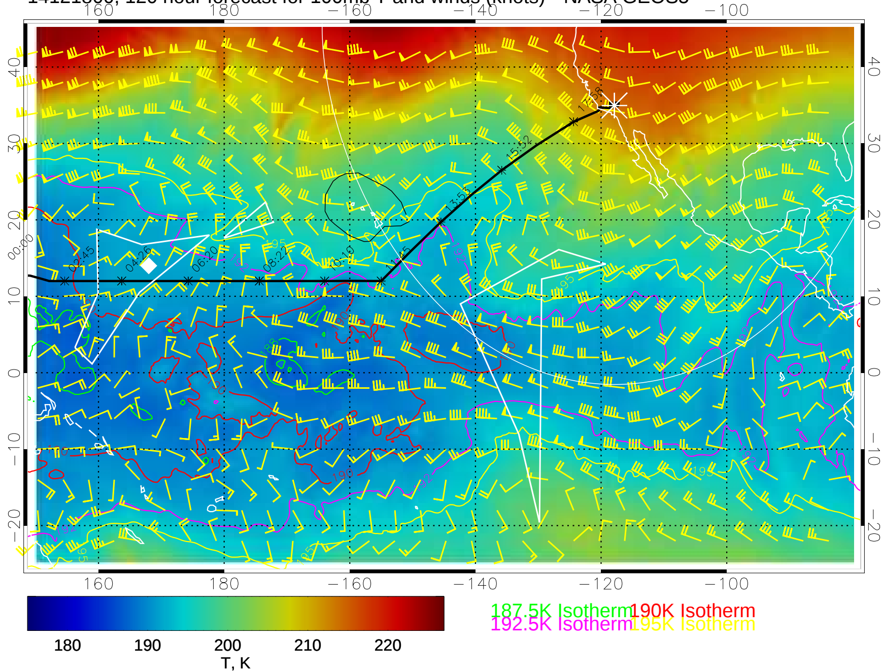
14121800, 120 hour forecast for 100mb T and winds (knots)-- NASA GEOS5
