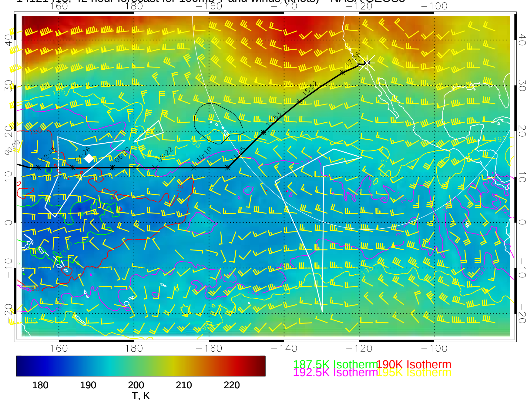
14121418, 42 hour forecast for 100mb T and winds (knots)-- NASA GEOS5
