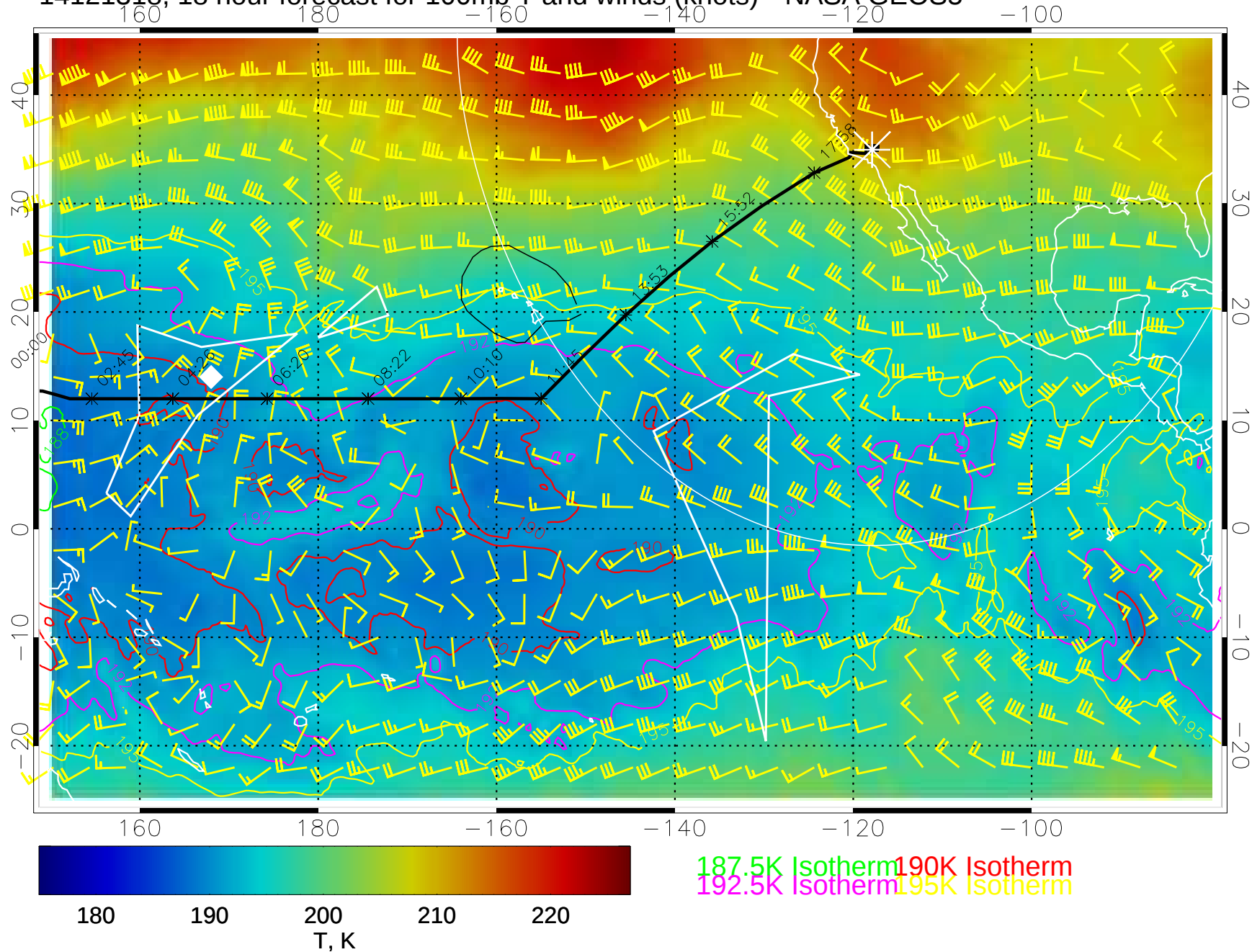
14121318, 18 hour forecast for 100mb T and winds (knots)-- NASA GEOS5
