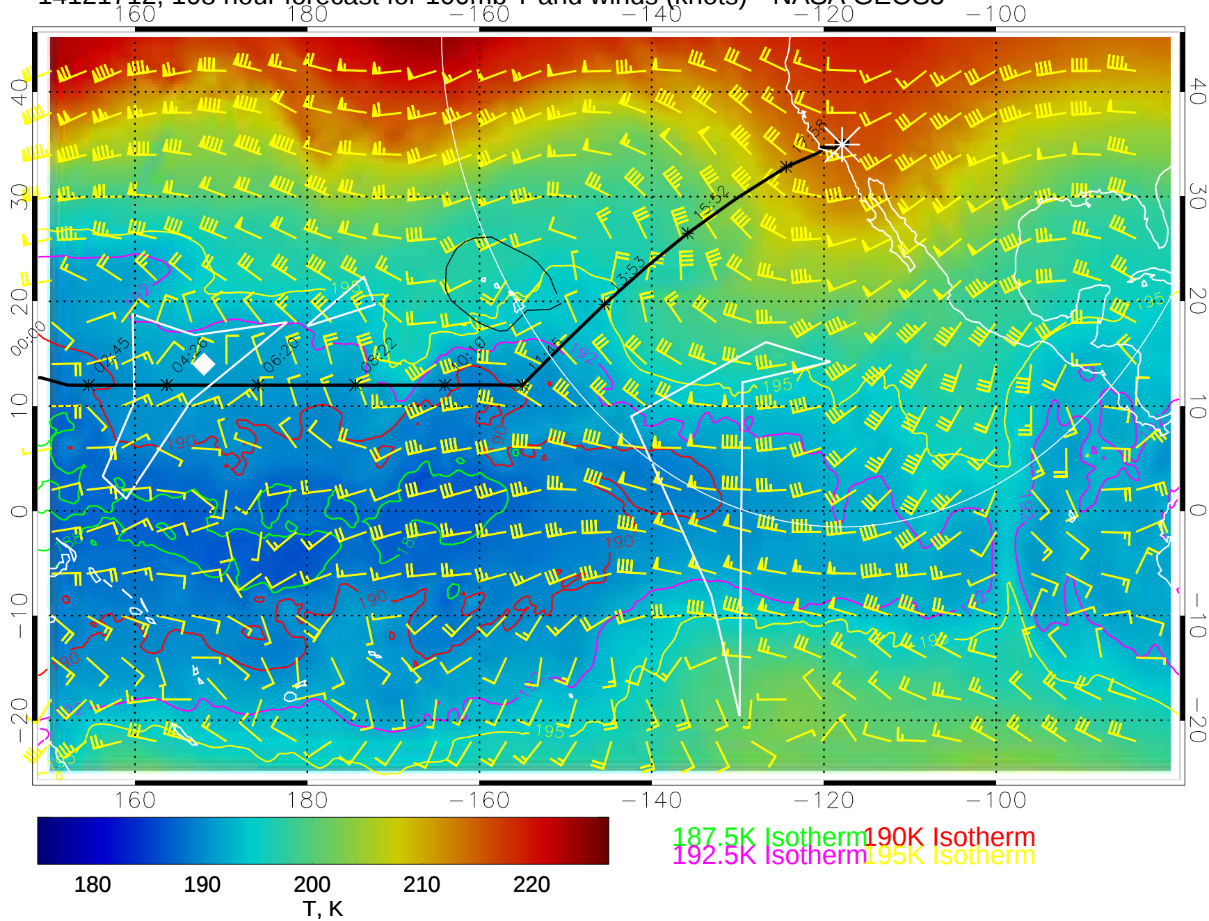
14121712, 108 hour forecast for 100mb T and winds (knots)-- NASA GEOS5
