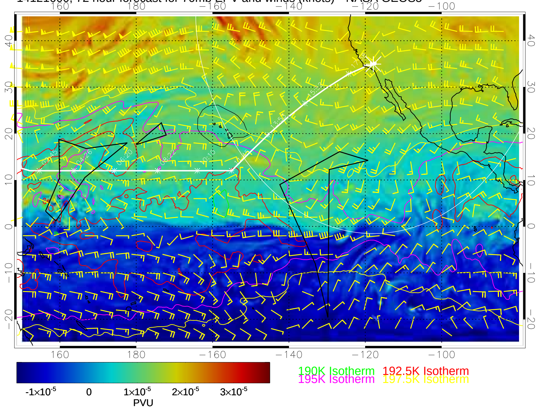
14121600, 72 hour forecast for 70mb EPV and winds (knots)-- NASA GEOS5
