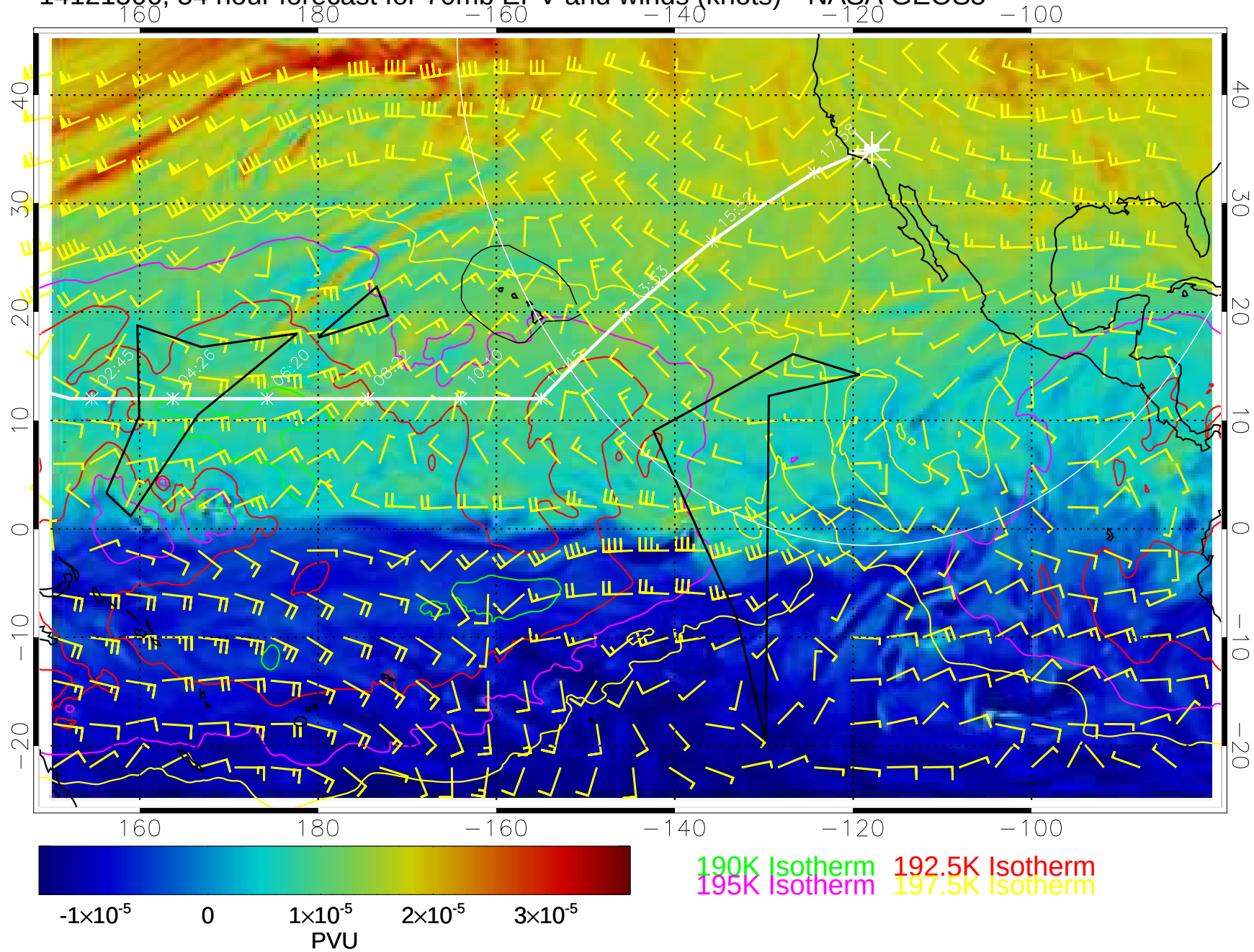
14121506, 54 hour forecast for 70mb EPV and winds (knots)-- NASA GEOS5
