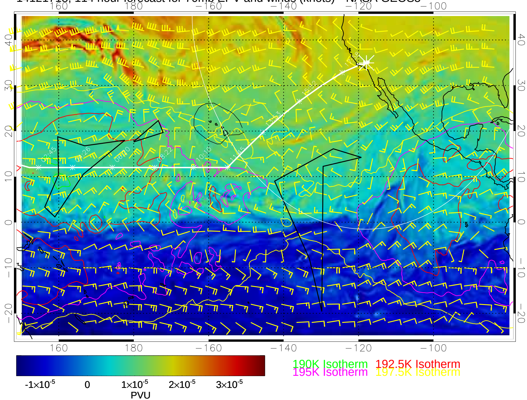
14121718, 114 hour forecast for 70mb EPV and winds (knots)-- NASA GEOS5
