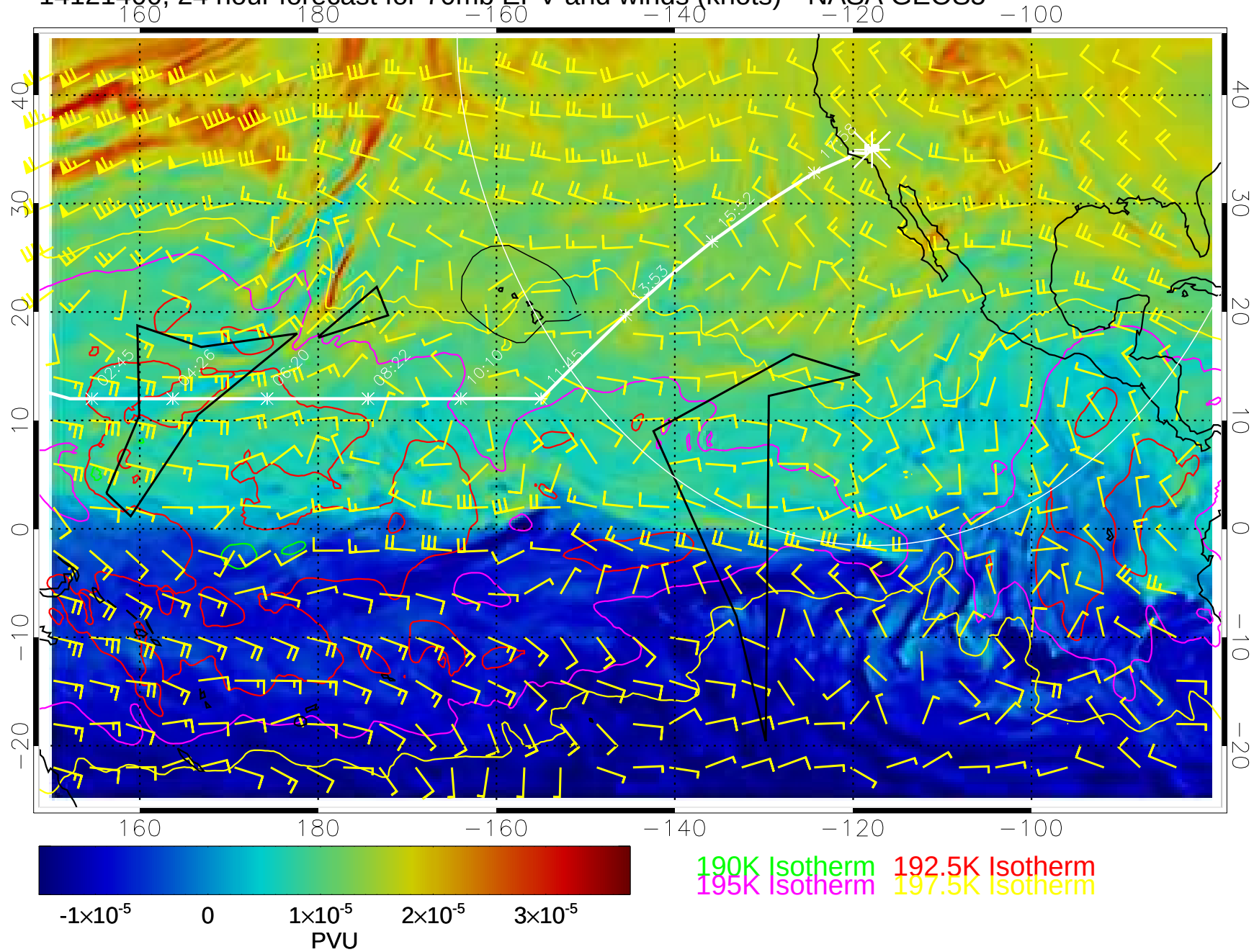
14121400, 24 hour forecast for 70mb EPV and winds (knots)-- NASA GEOS5
