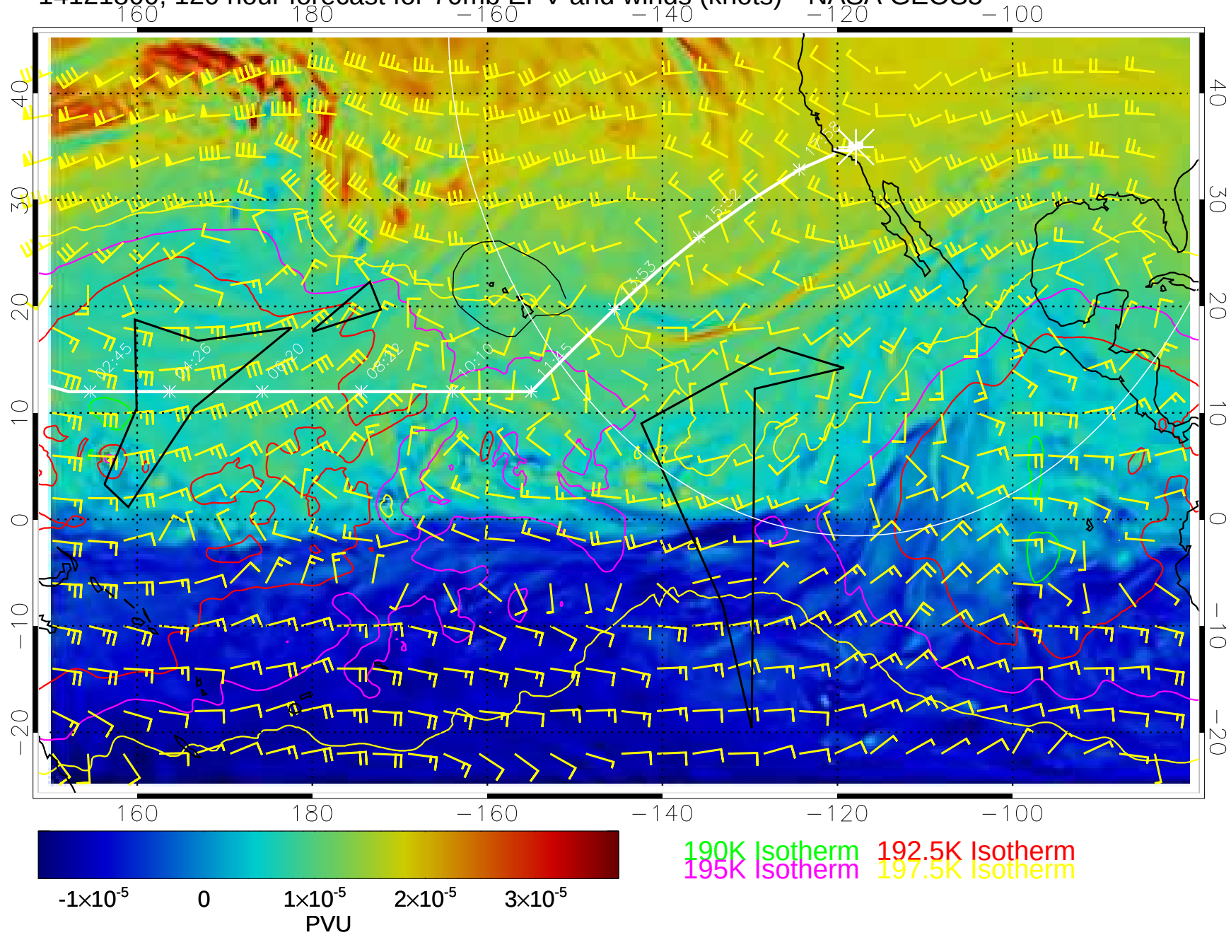
14121800, 120 hour forecast for 70mb EPV and winds (knots)-- NASA GEOS5
