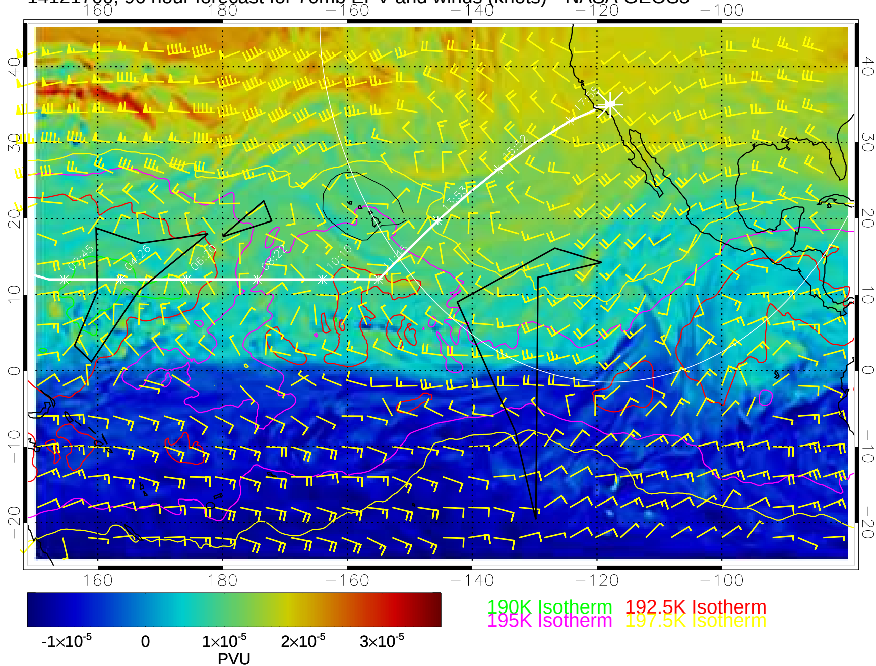
14121700, 96 hour forecast for 70mb EPV and winds (knots)-- NASA GEOS5
