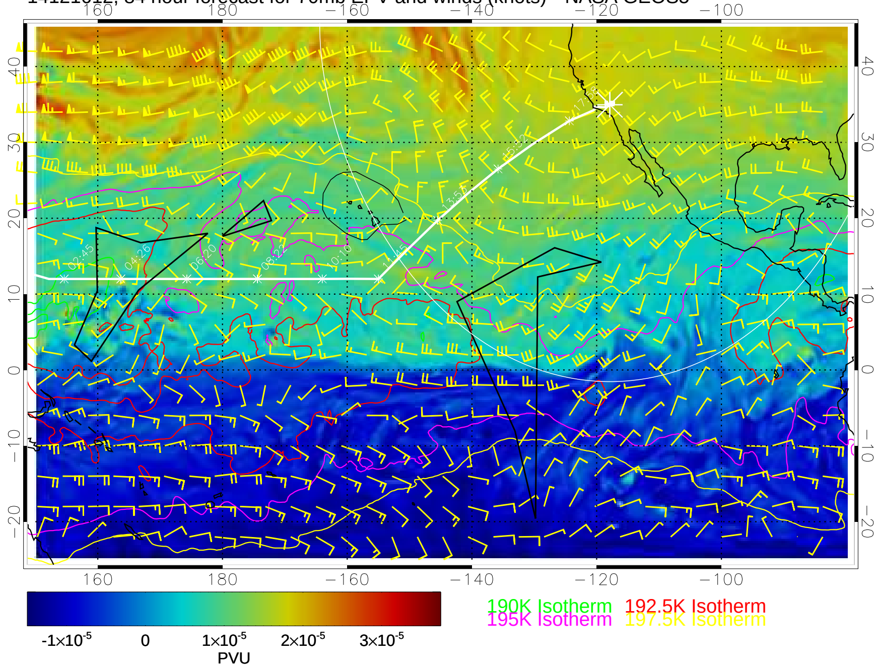
14121612, 84 hour forecast for 70mb EPV and winds (knots)-- NASA GEOS5
