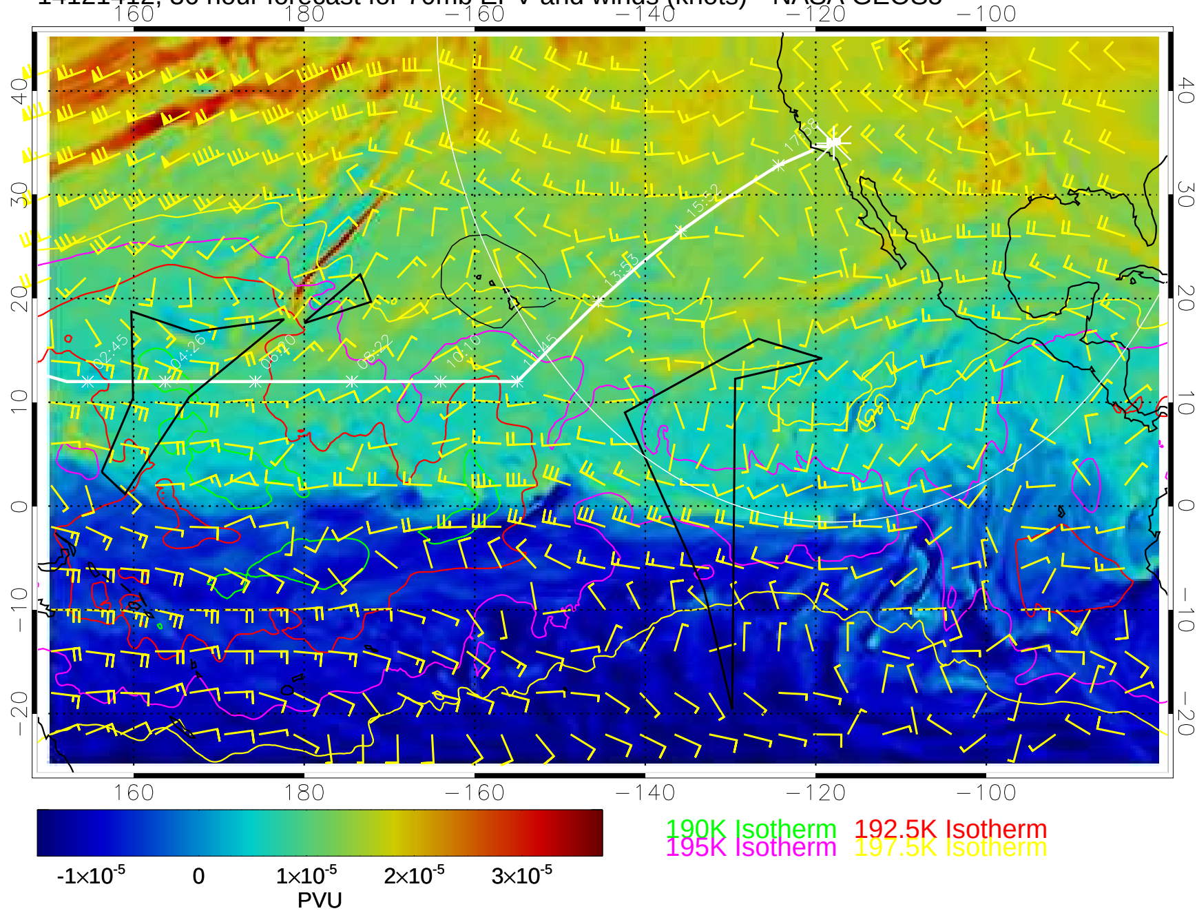
14121412, 36 hour forecast for 70mb EPV and winds (knots)-- NASA GEOS5
