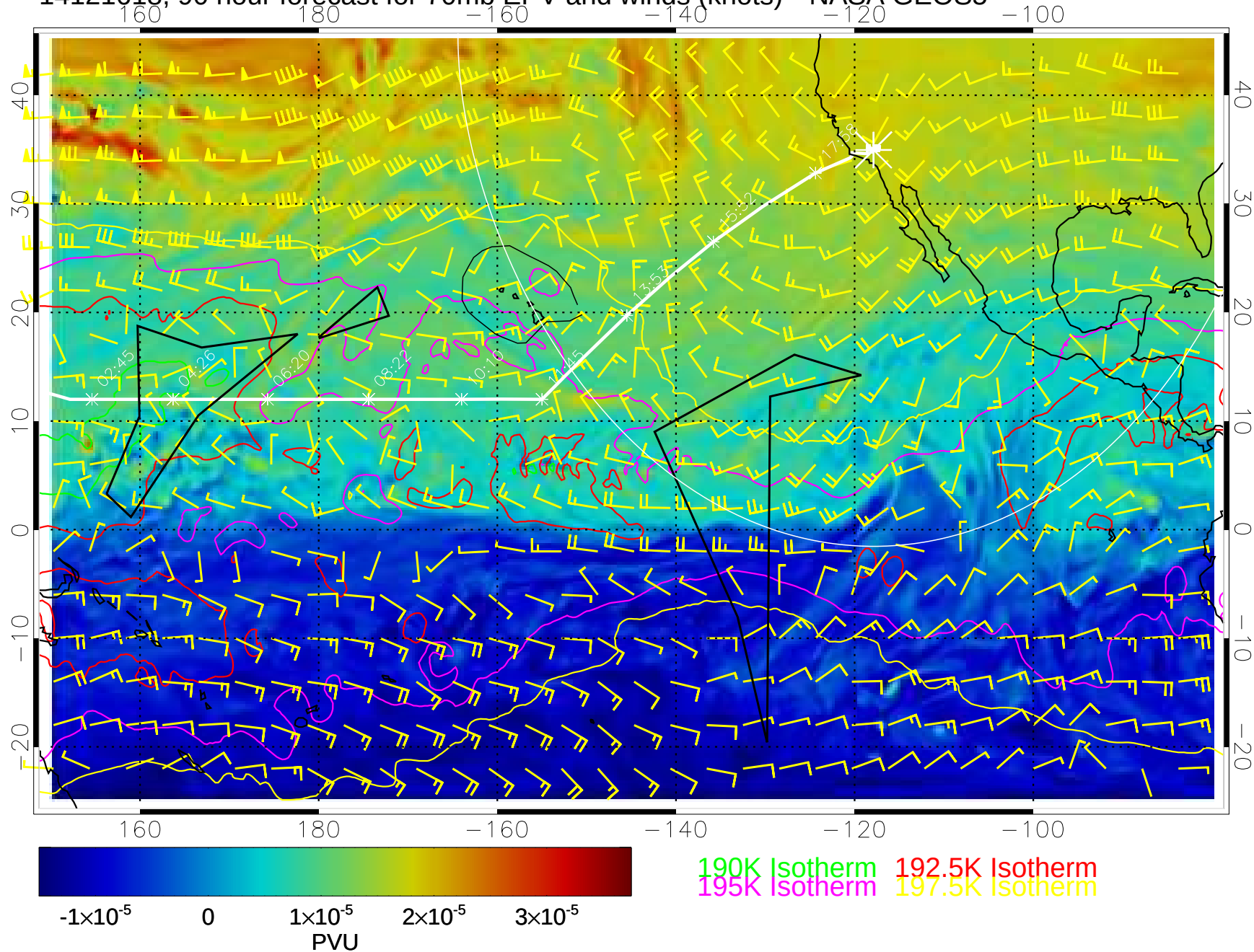
14121618, 90 hour forecast for 70mb EPV and winds (knots)-- NASA GEOS5
