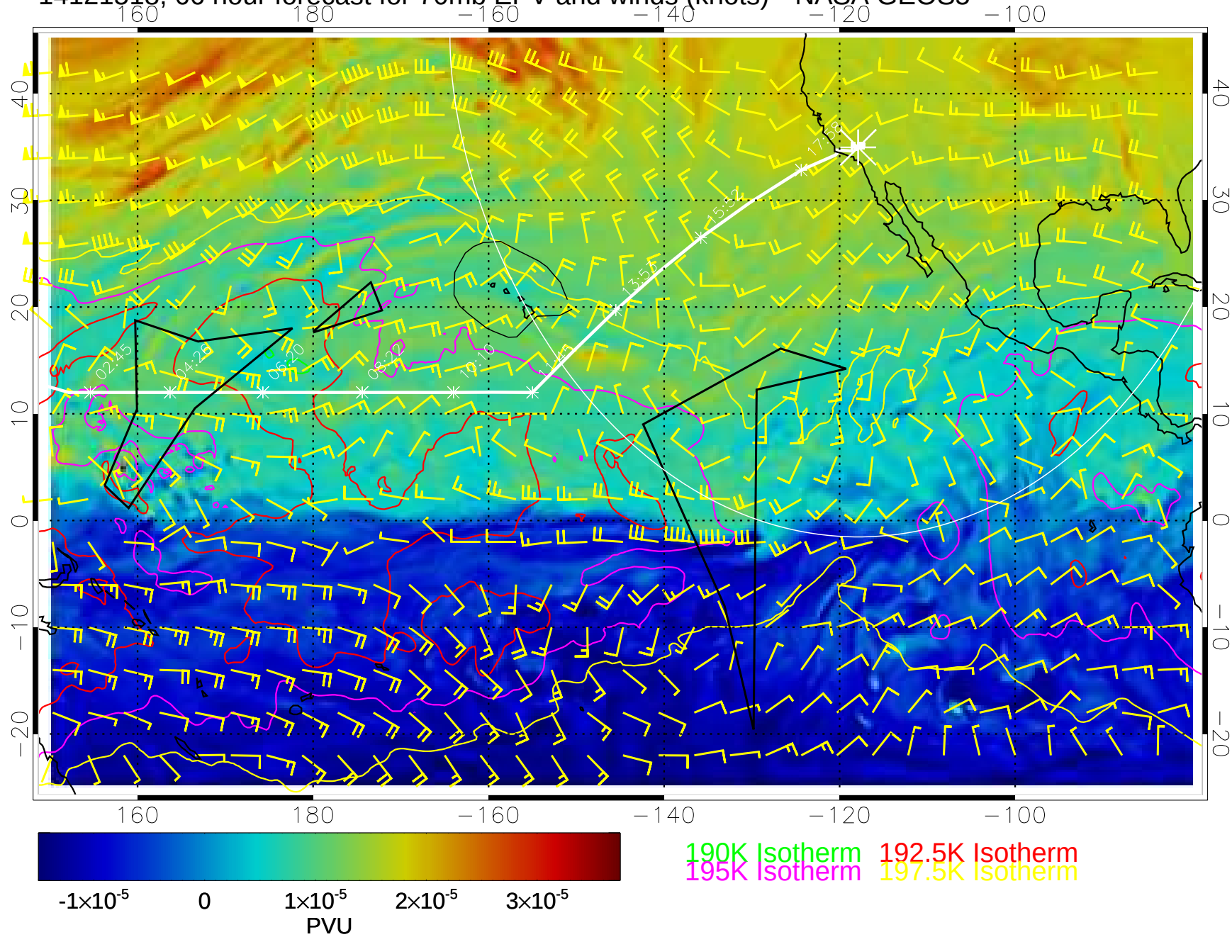
14121518, 66 hour forecast for 70mb EPV and winds (knots)-- NASA GEOS5
