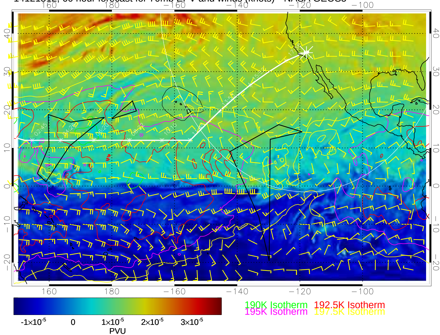
14121512, 60 hour forecast for 70mb EPV and winds (knots)-- NASA GEOS5
