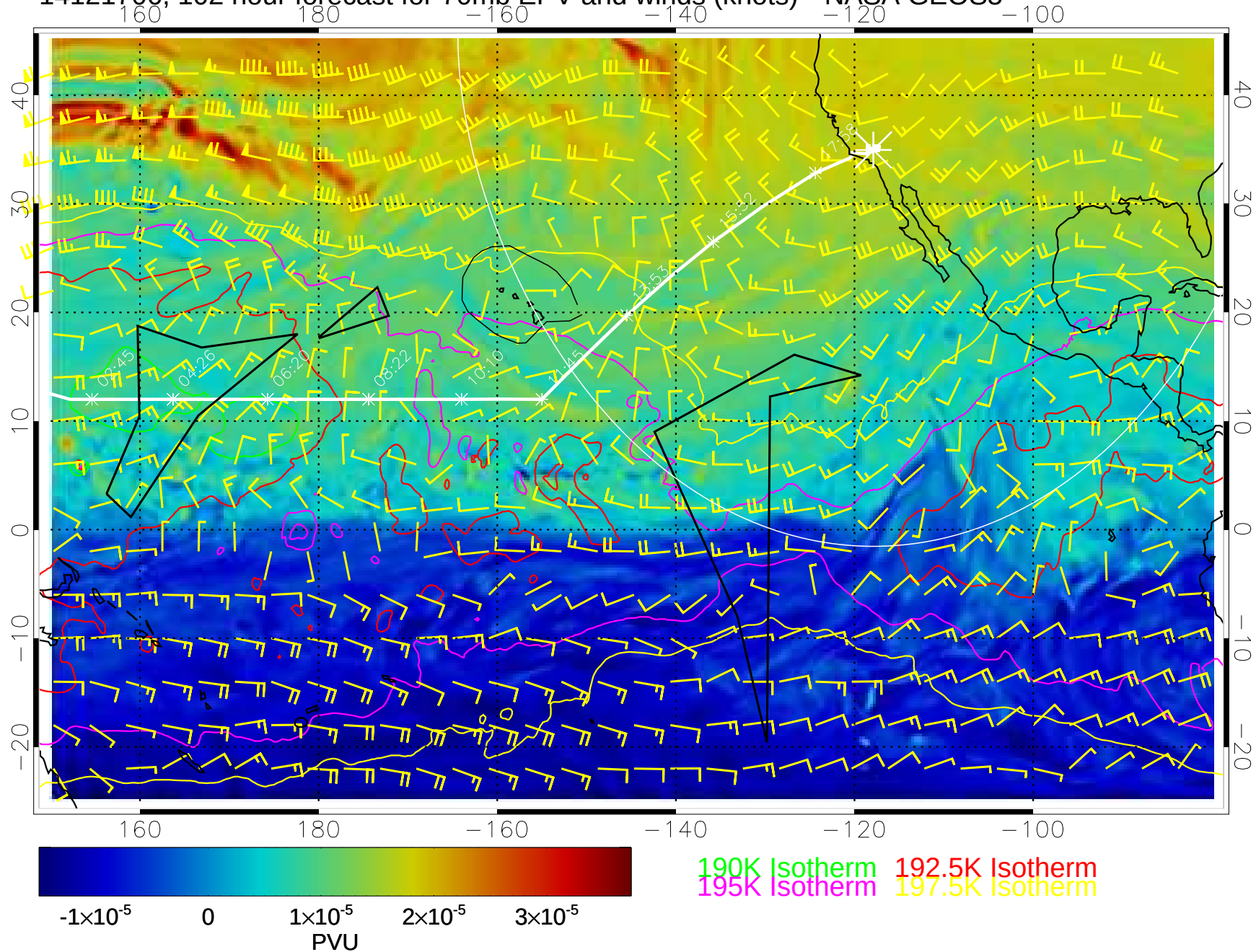
14121706, 102 hour forecast for 70mb EPV and winds (knots)-- NASA GEOS5
