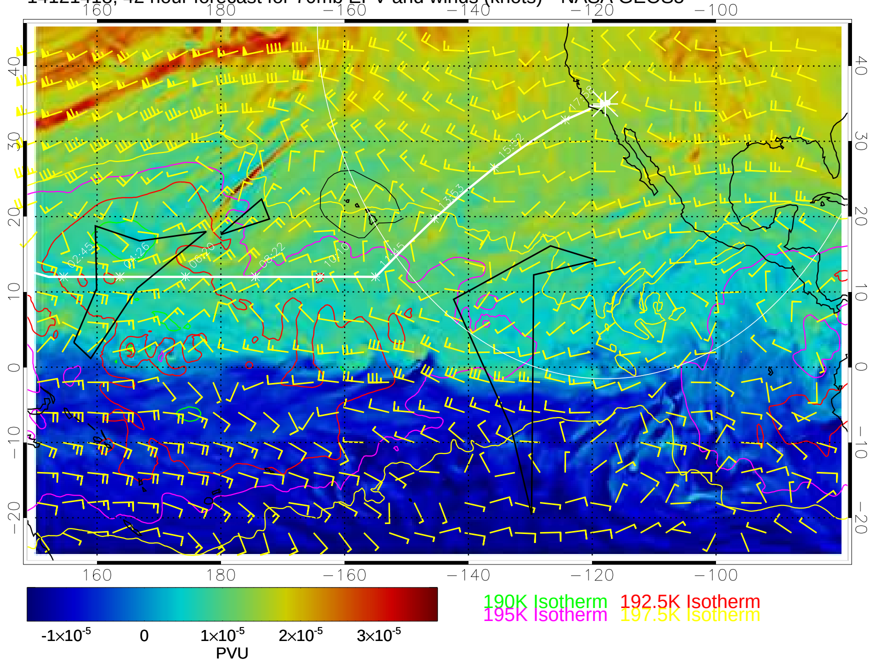
14121418, 42 hour forecast for 70mb EPV and winds (knots)-- NASA GEOS5
