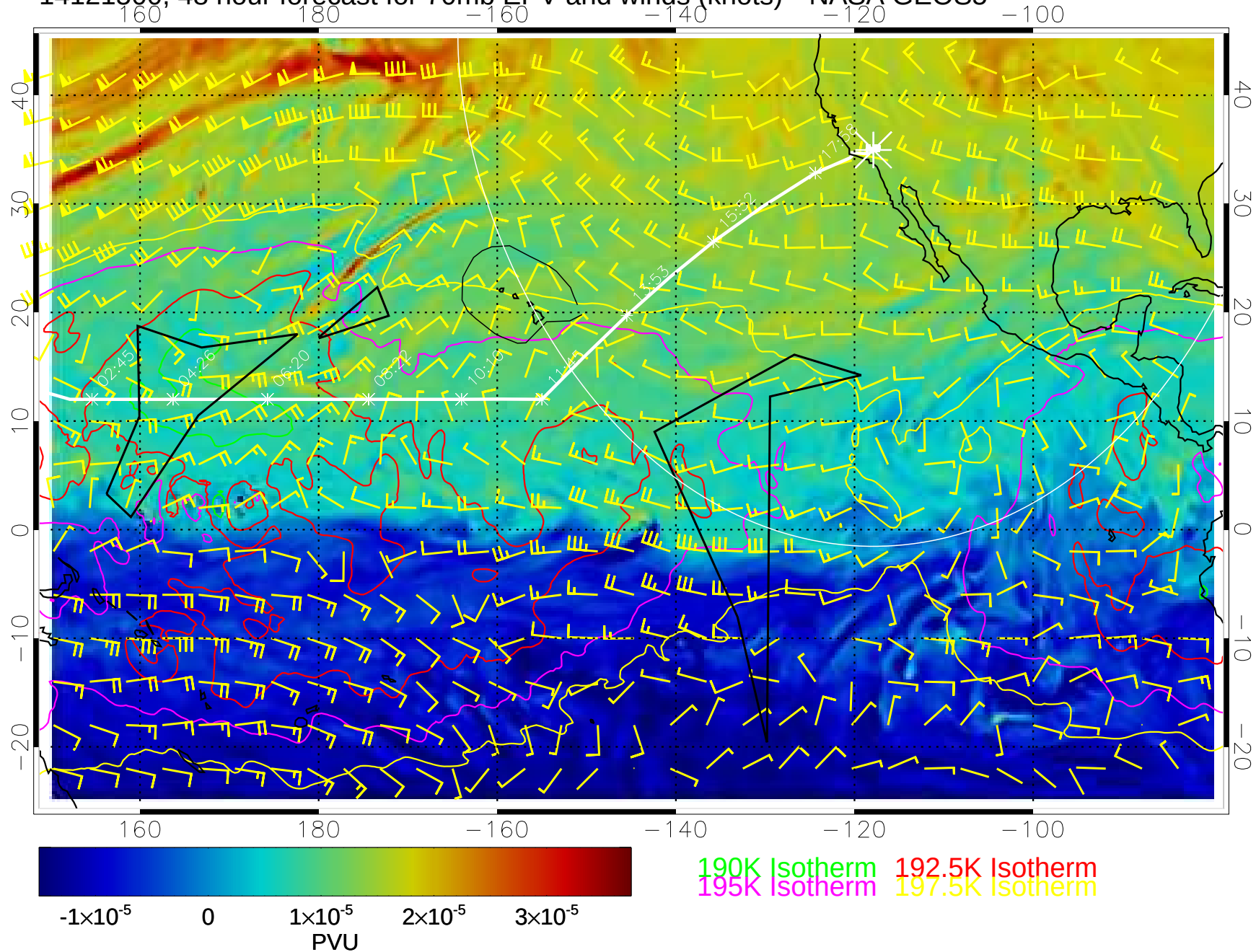
14121500, 48 hour forecast for 70mb EPV and winds (knots)-- NASA GEOS5
