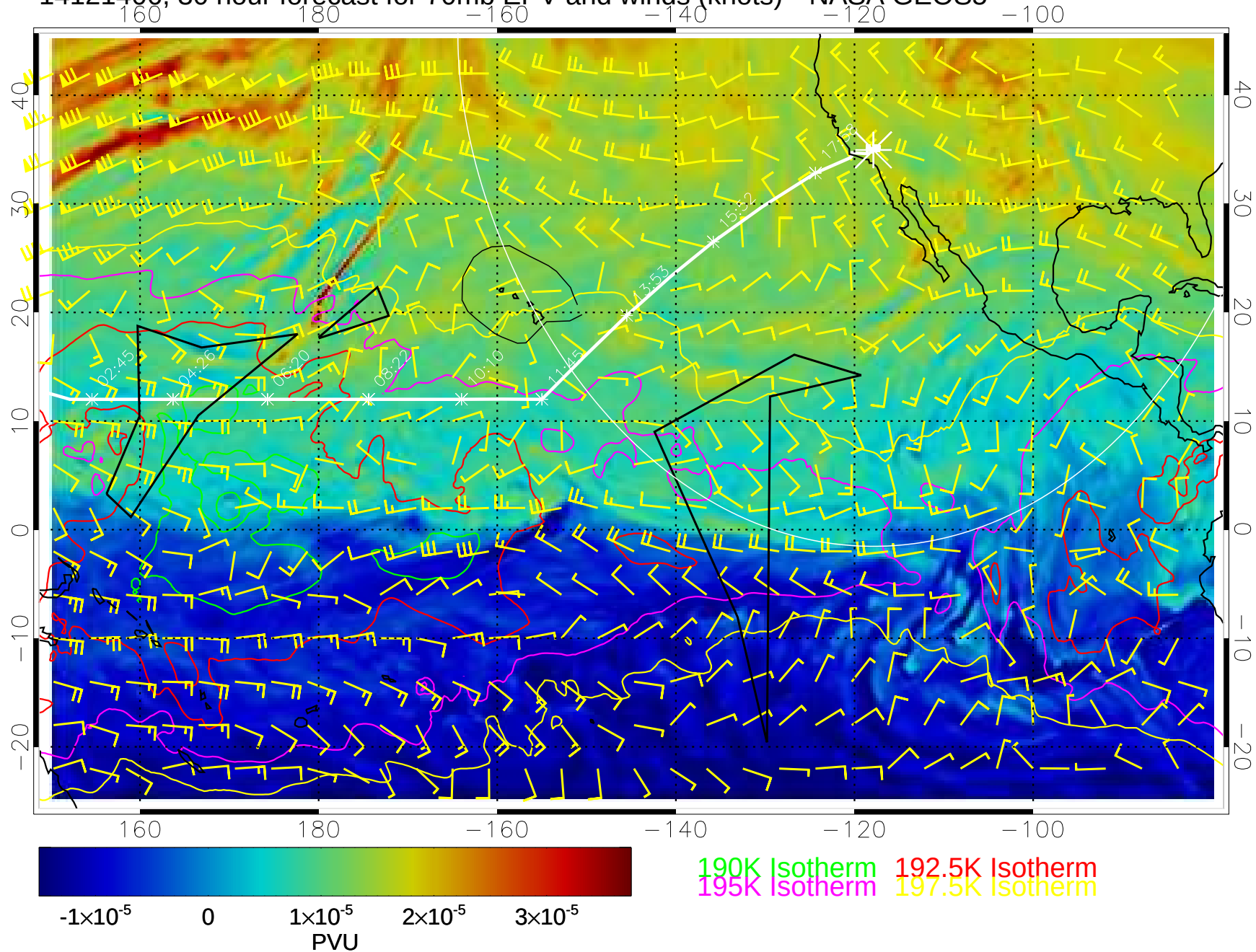
14121406, 30 hour forecast for 70mb EPV and winds (knots)-- NASA GEOS5
