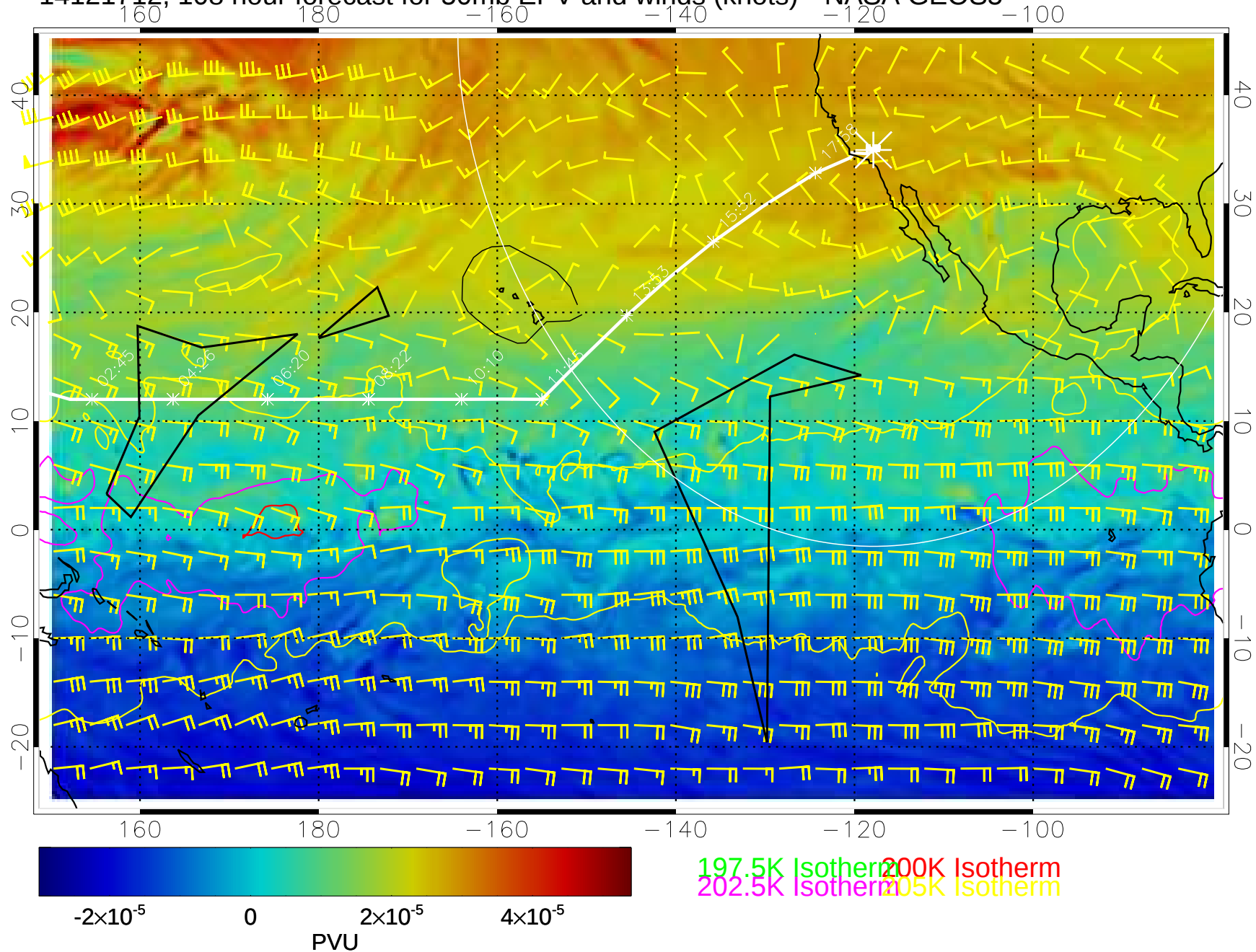
14121712, 108 hour forecast for 50mb EPV and winds (knots)-- NASA GEOS5
