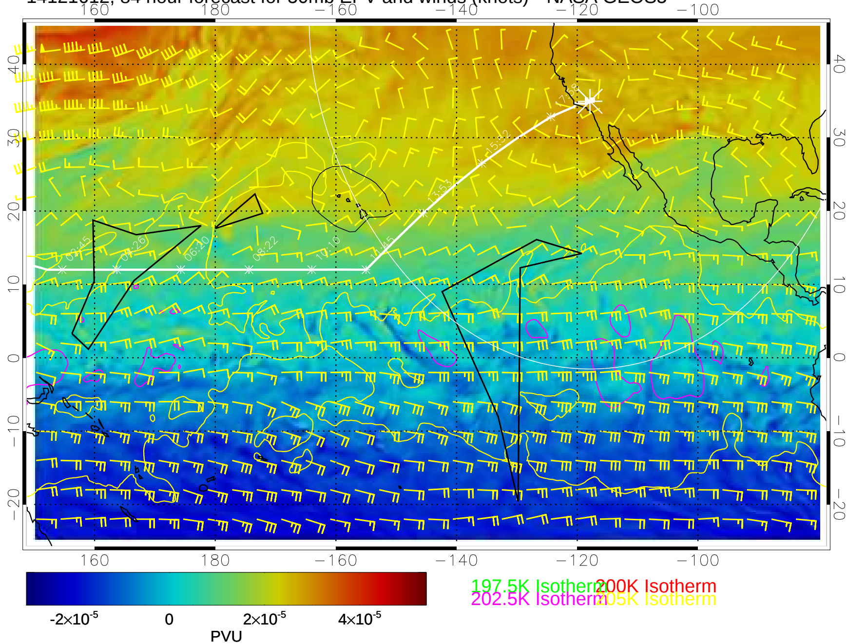
14121612, 84 hour forecast for 50mb EPV and winds (knots)-- NASA GEOS5
