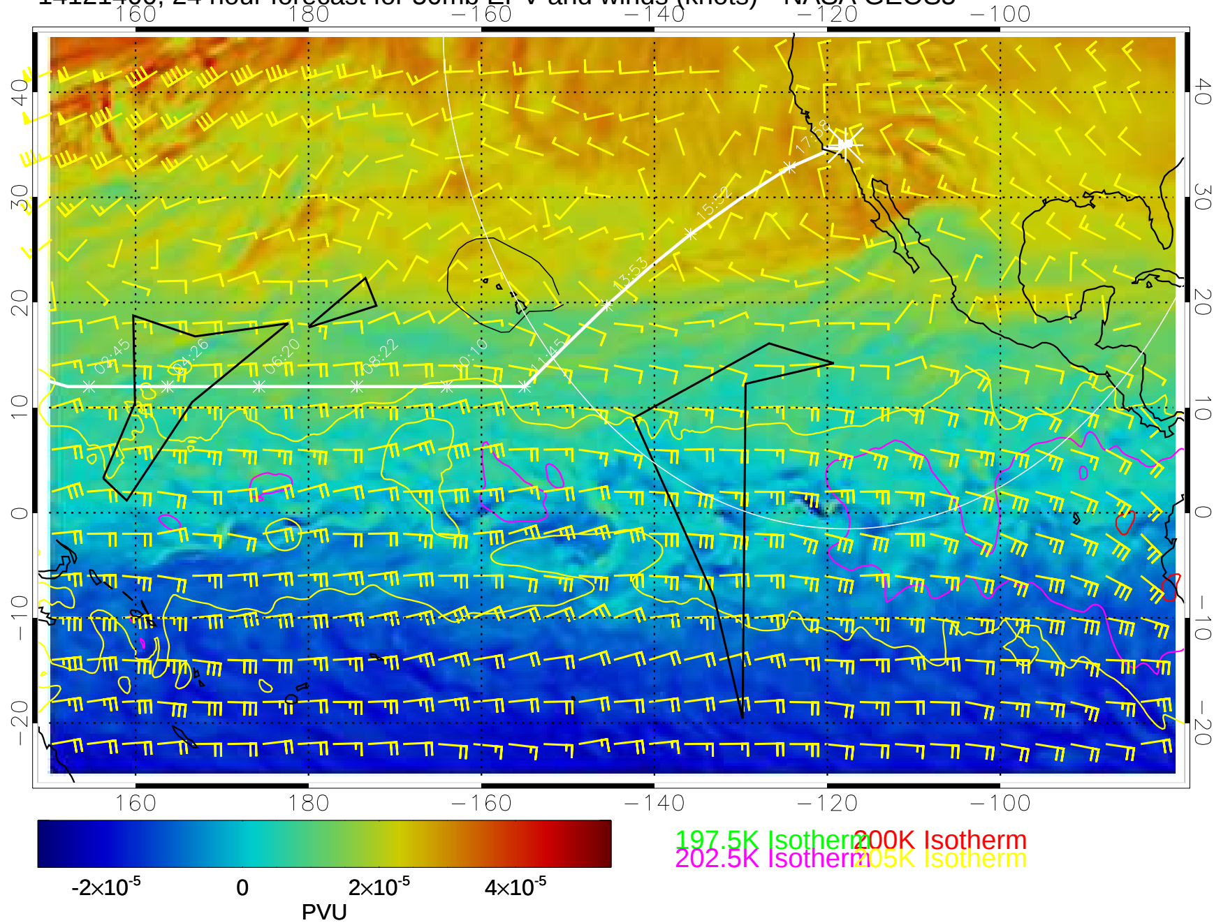
14121400, 24 hour forecast for 50mb EPV and winds (knots)-- NASA GEOS5
