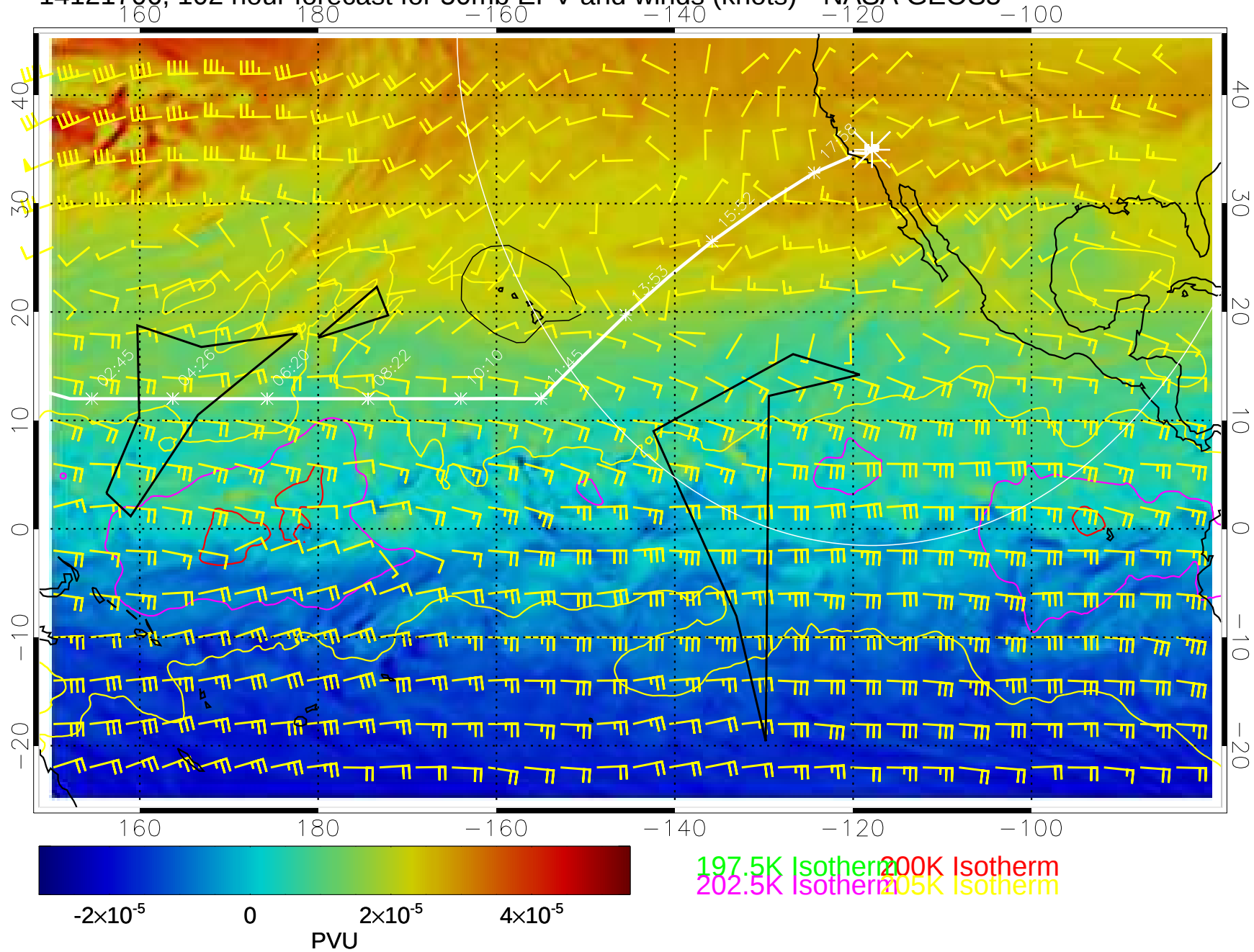
14121706, 102 hour forecast for 50mb EPV and winds (knots)-- NASA GEOS5
