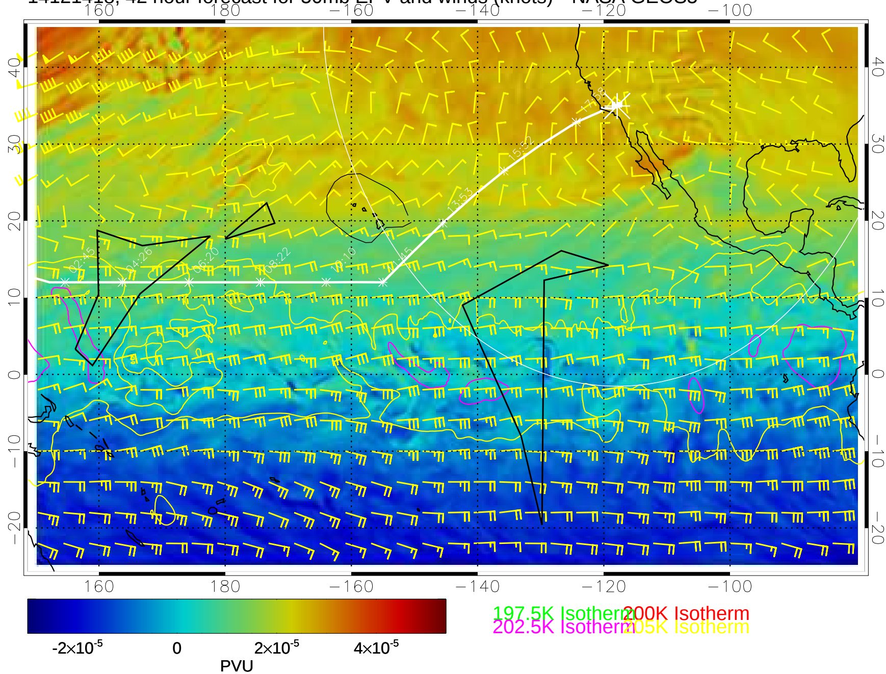
14121418, 42 hour forecast for 50mb EPV and winds (knots)-- NASA GEOS5
