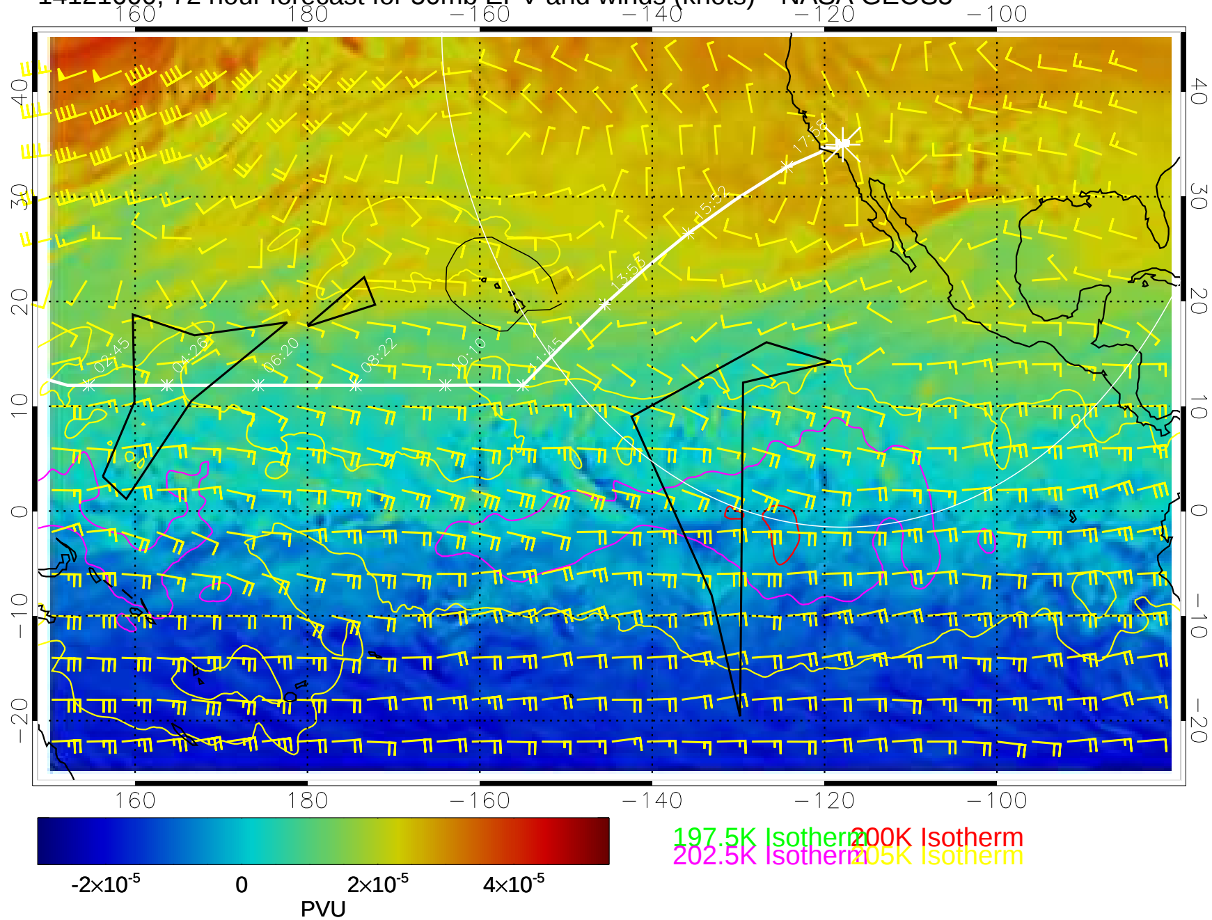
14121600, 72 hour forecast for 50mb EPV and winds (knots)-- NASA GEOS5
