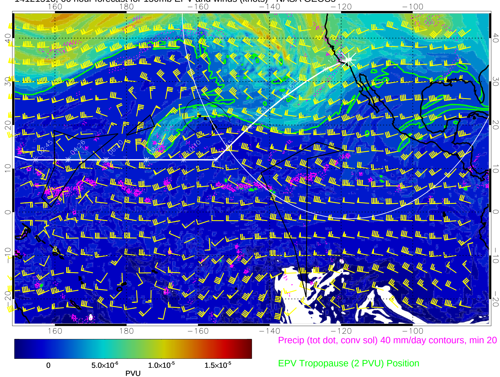
14121518, 66 hour forecast for 150mb EPV and winds (knots) - NASA GEOS5
