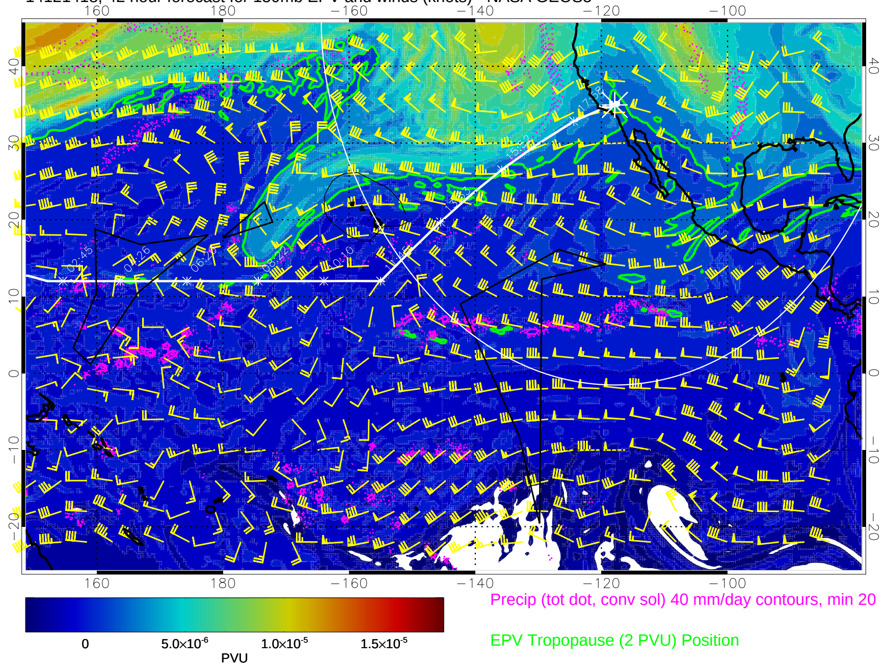
14121418, 42 hour forecast for 150mb EPV and winds (knots) - NASA GEOS5
