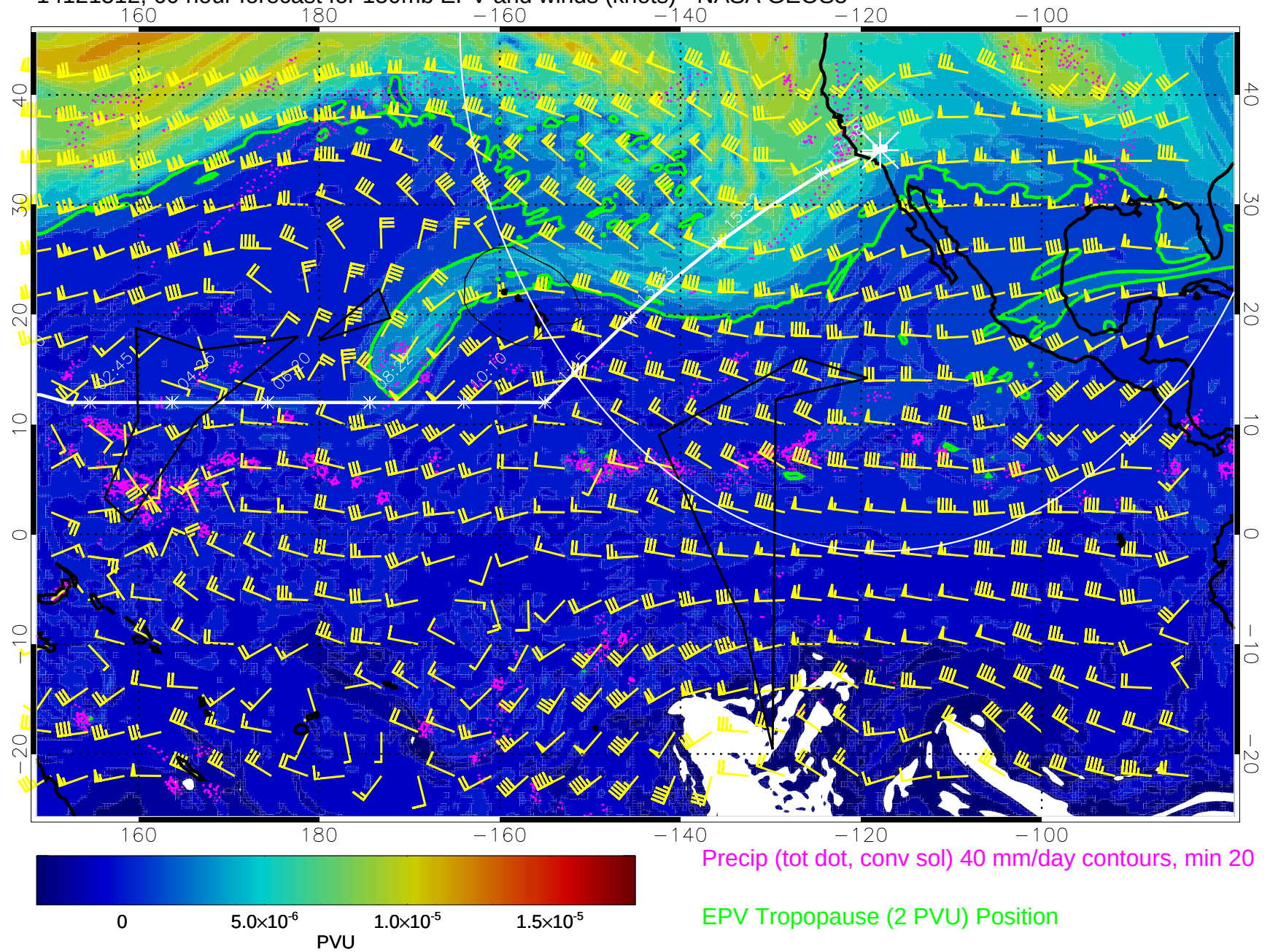
14121512, 60 hour forecast for 150mb EPV and winds (knots) - NASA GEOS5
