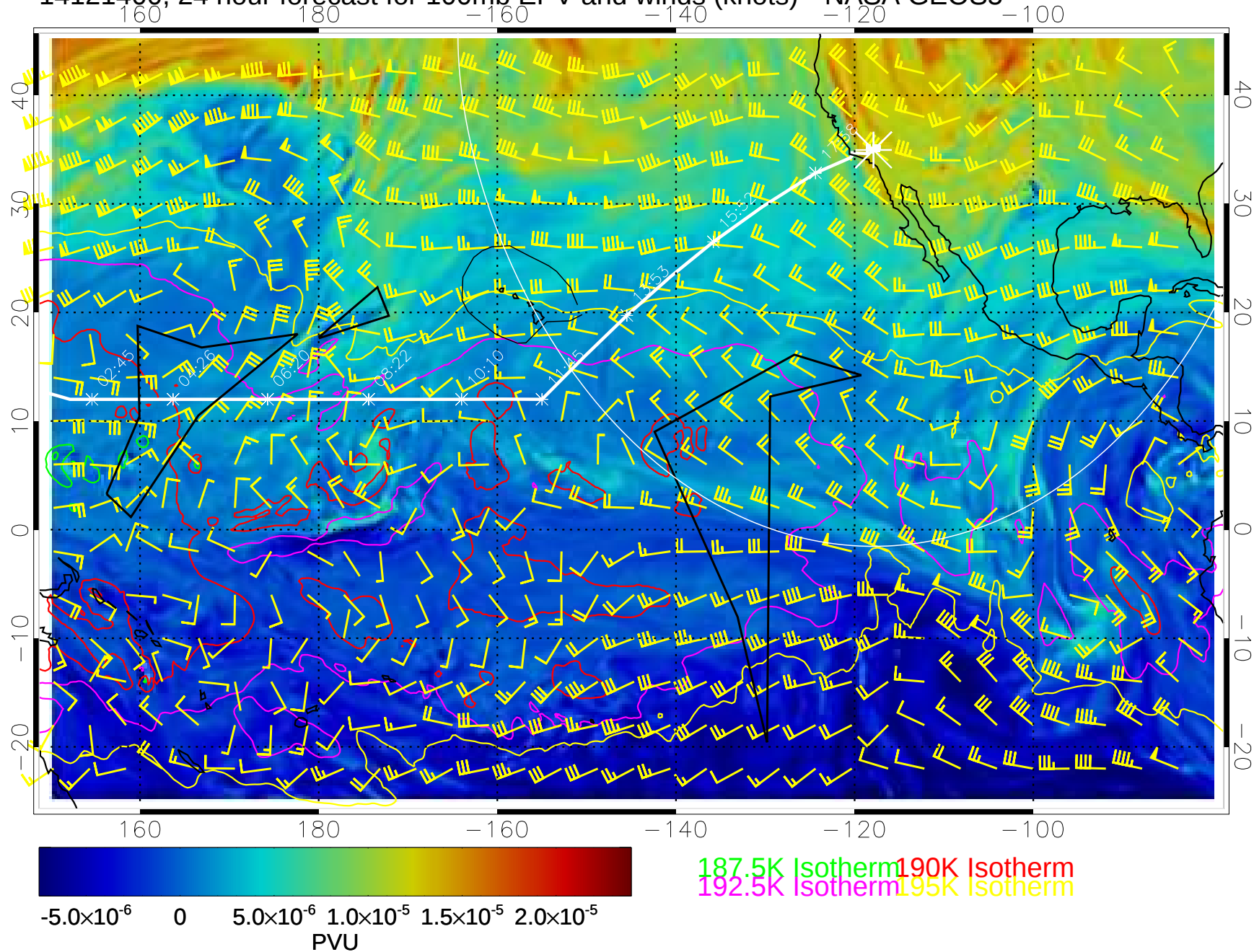
14121400, 24 hour forecast for 100mb EPV and winds (knots)-- NASA GEOS5
