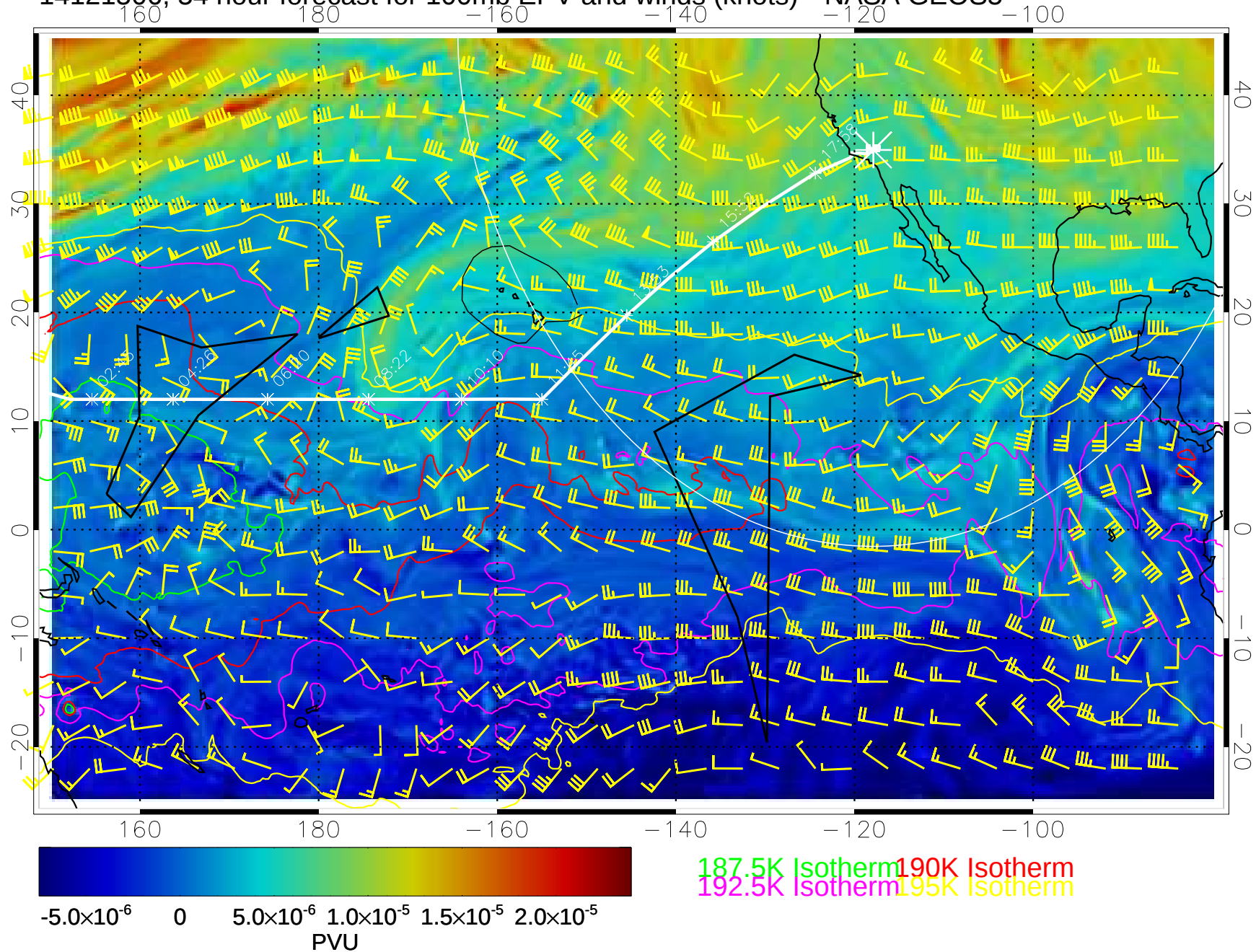
14121506, 54 hour forecast for 100mb EPV and winds (knots)-- NASA GEOS5
