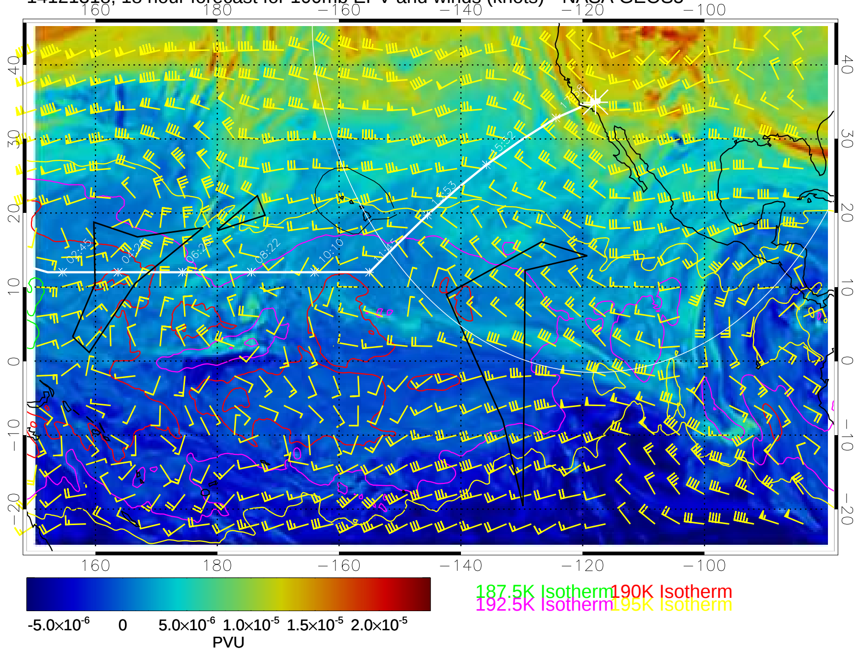
14121318, 18 hour forecast for 100mb EPV and winds (knots)-- NASA GEOS5
