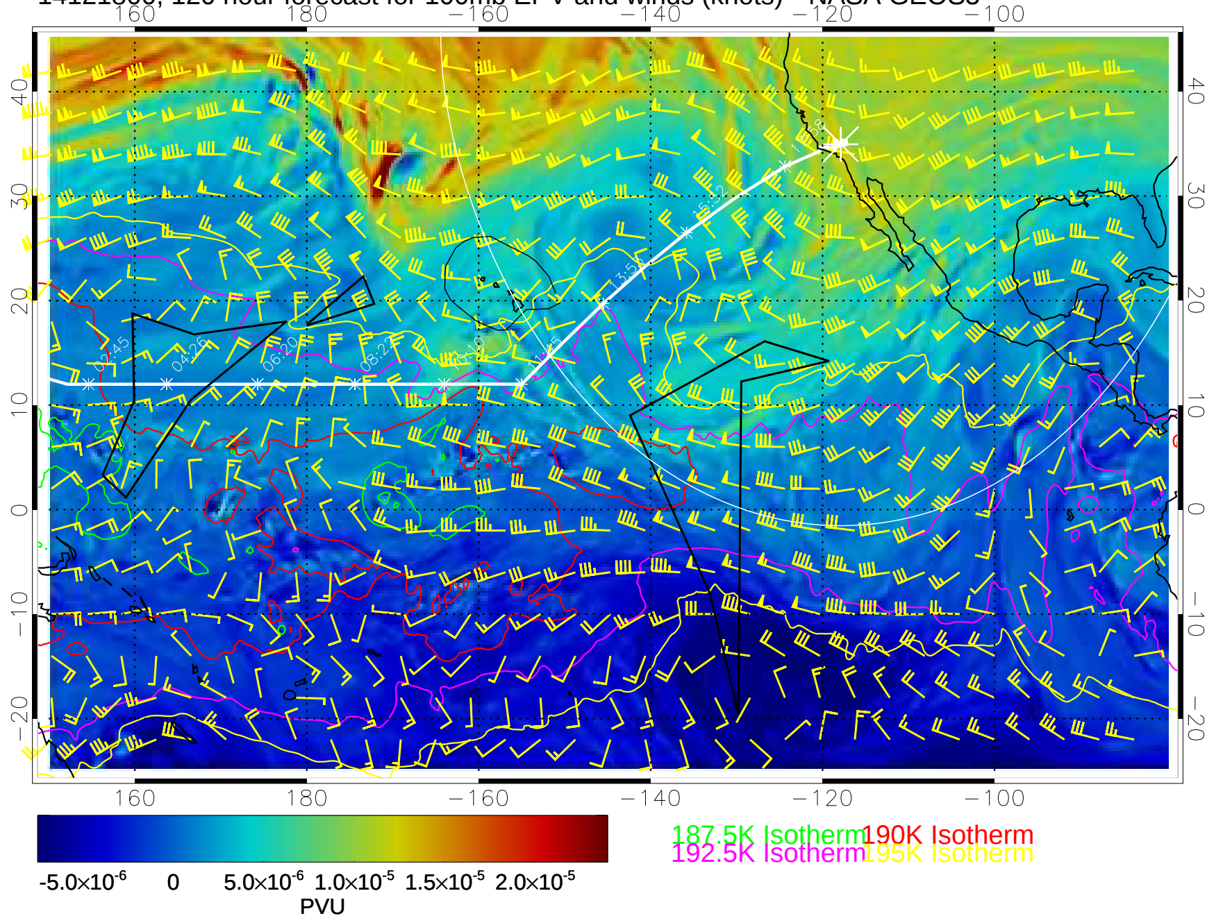
14121800, 120 hour forecast for 100mb EPV and winds (knots)-- NASA GEOS5
