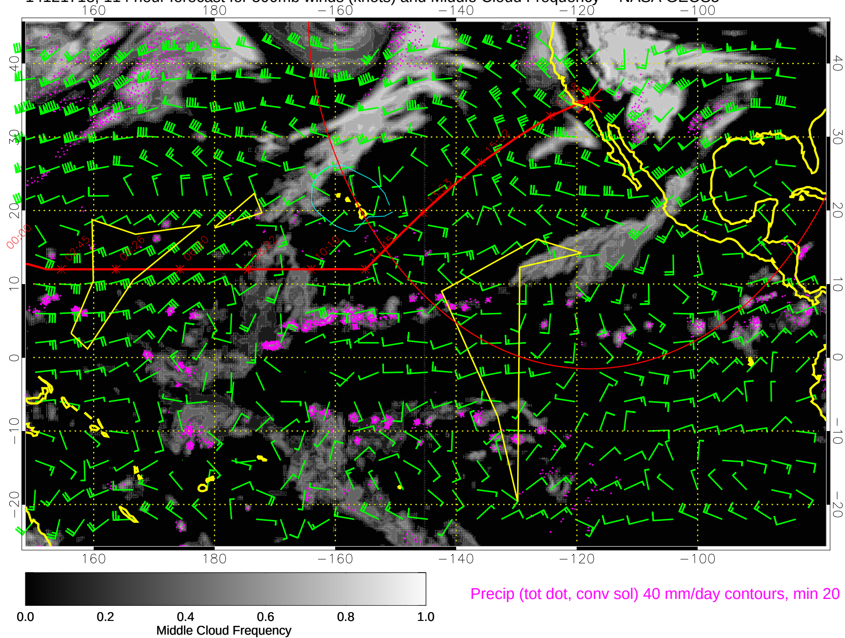
14121718, 114 hour forecast for 500mb winds (knots) and Middle Cloud Frequency -- NASA GEOS5
