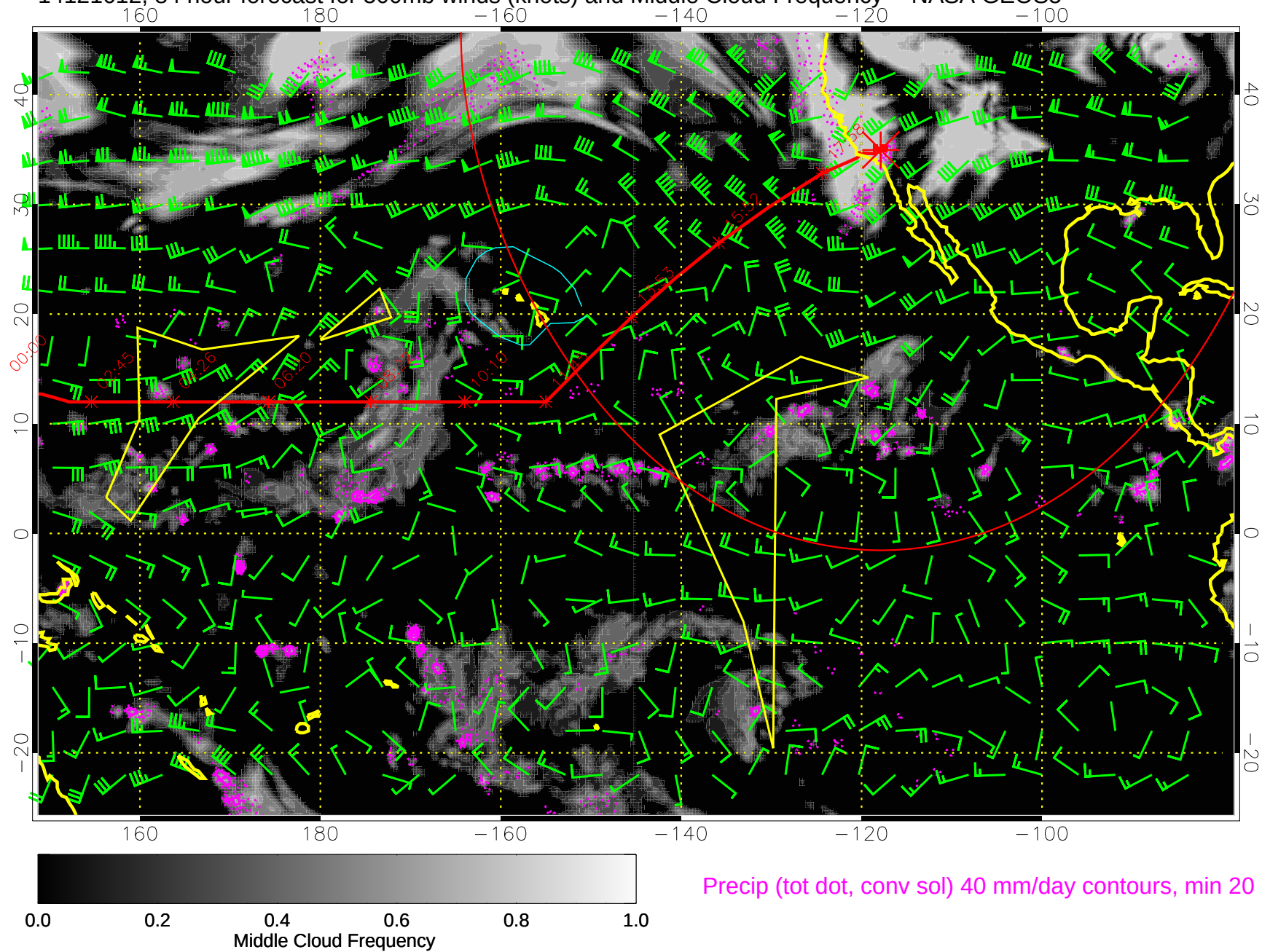
14121612, 84 hour forecast for 500mb winds (knots) and Middle Cloud Frequency -- NASA GEOS5
