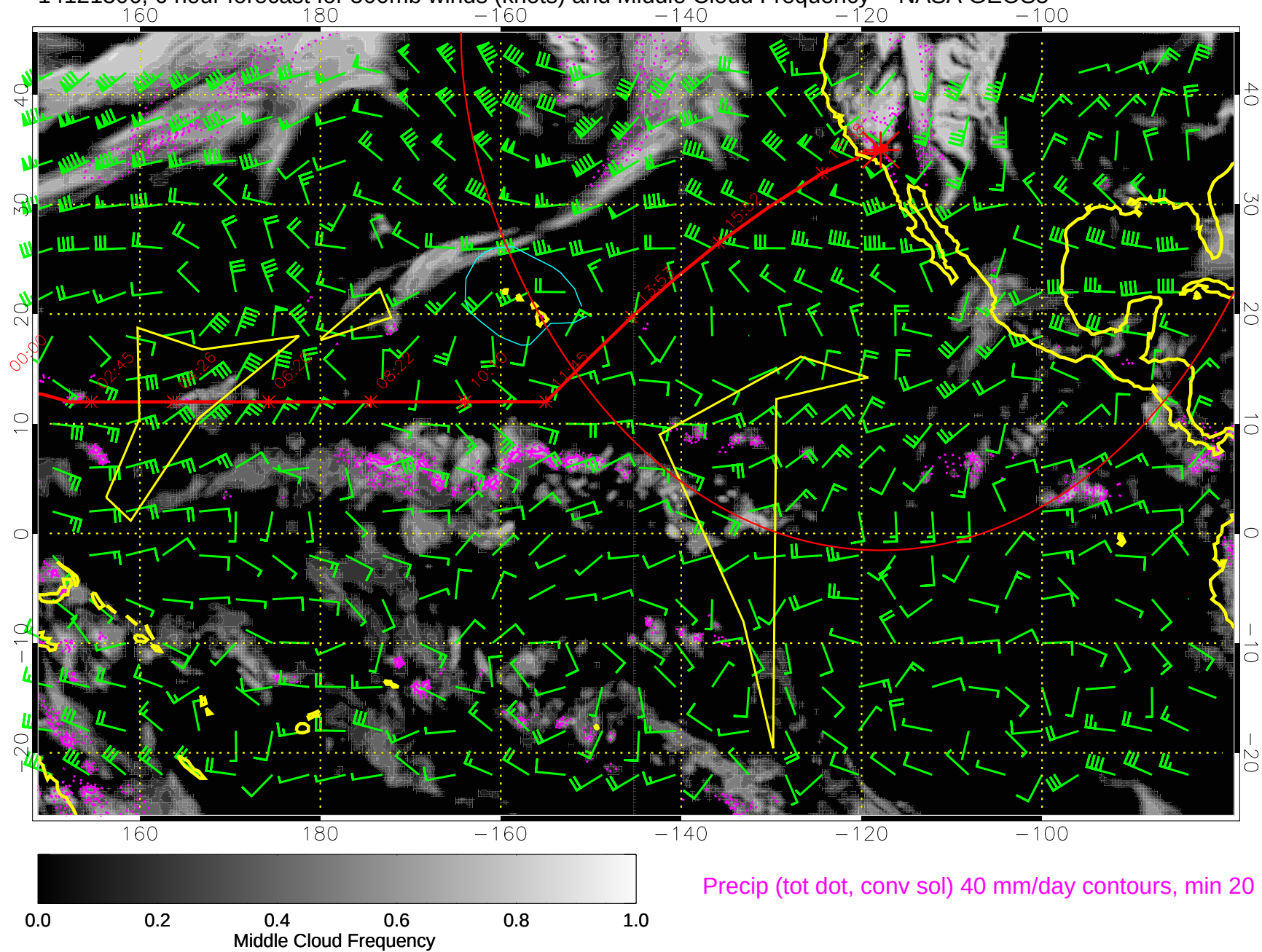
14121306, 6 hour forecast for 500mb winds (knots) and Middle Cloud Frequency -- NASA GEOS5
