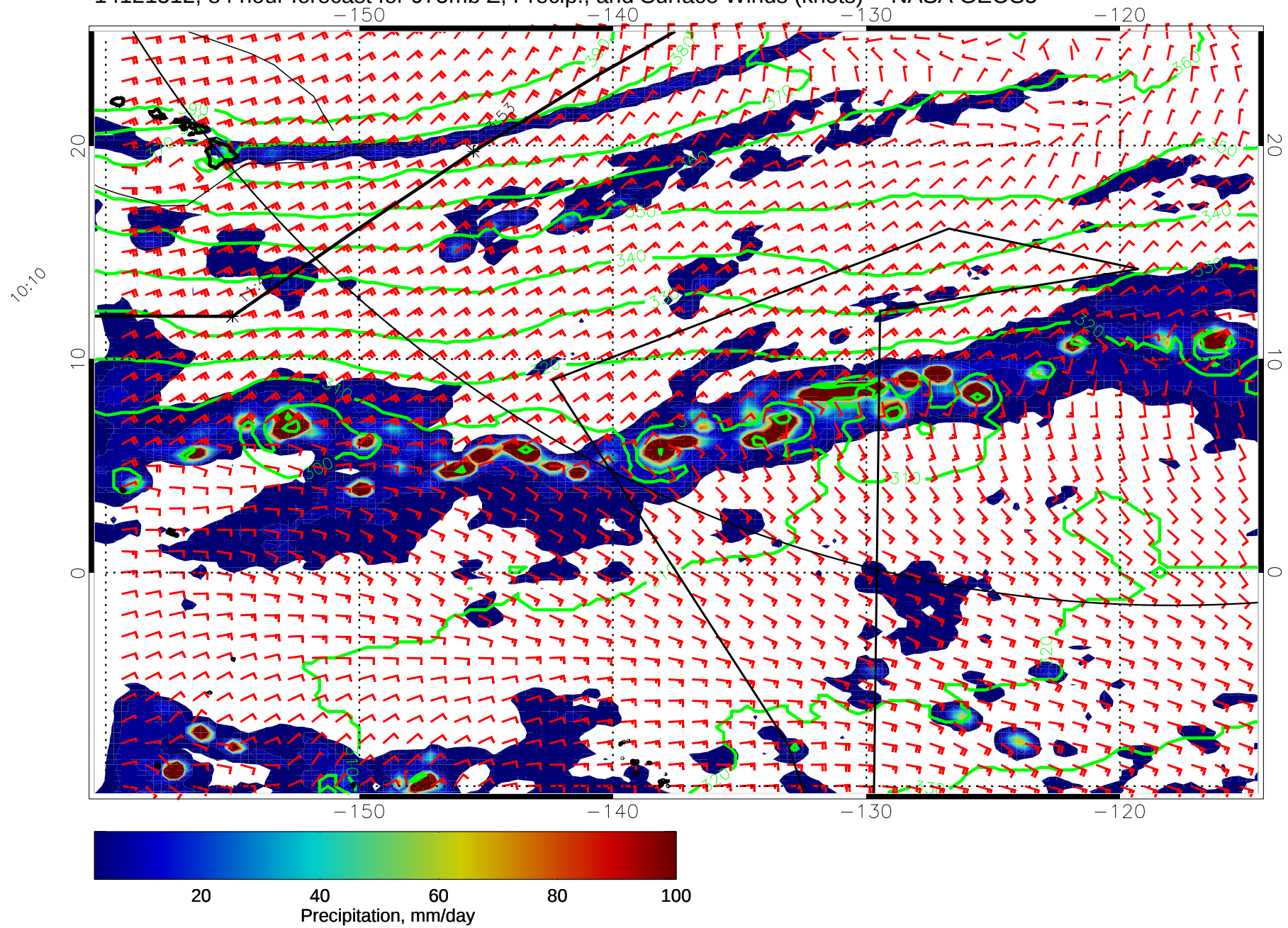
14121512, 84 hour forecast for 975mb Z, Precip., and Surface Winds (knots) -- NASA GEOS5
