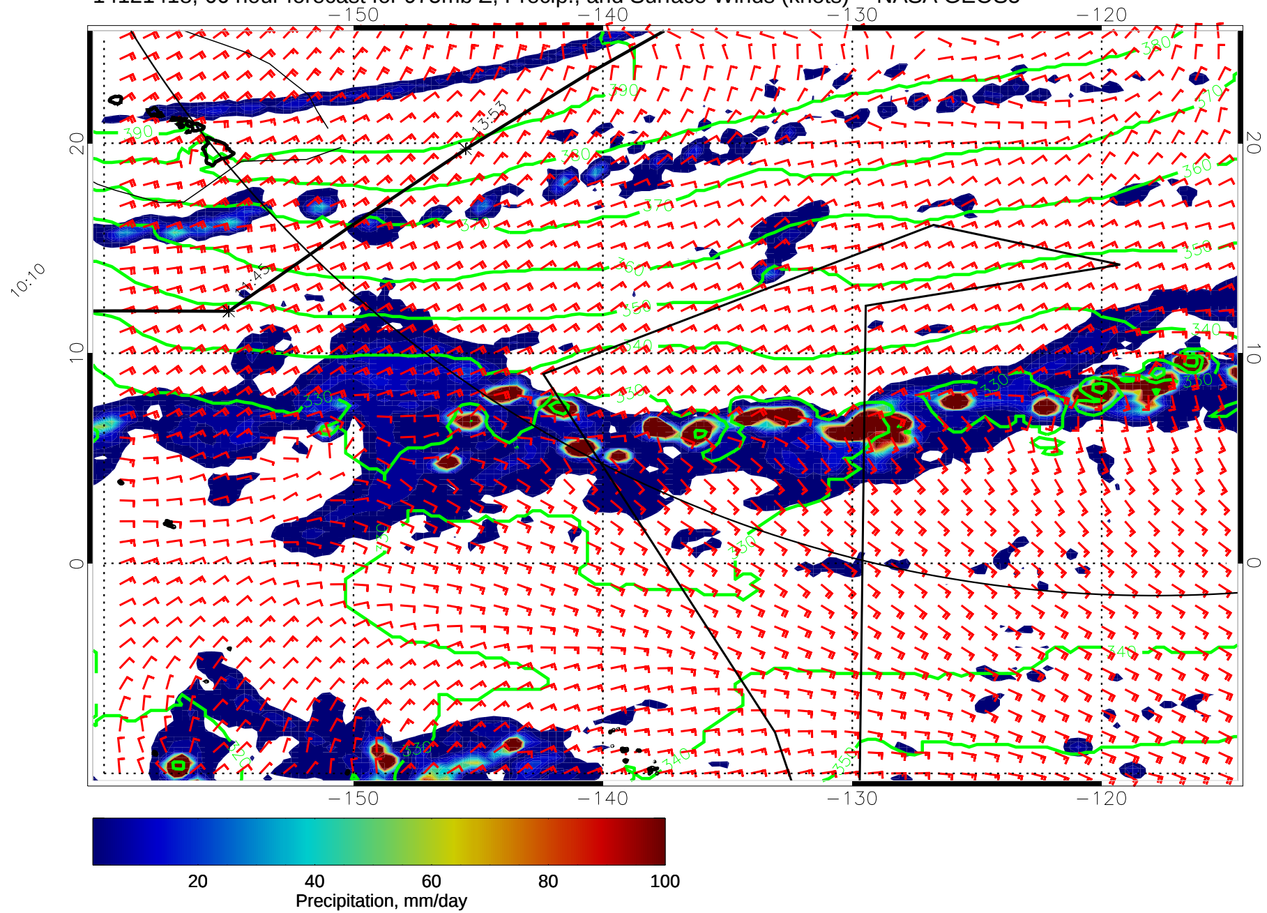
14121418, 66 hour forecast for 975mb Z, Precip., and Surface Winds (knots) -- NASA GEOS5
