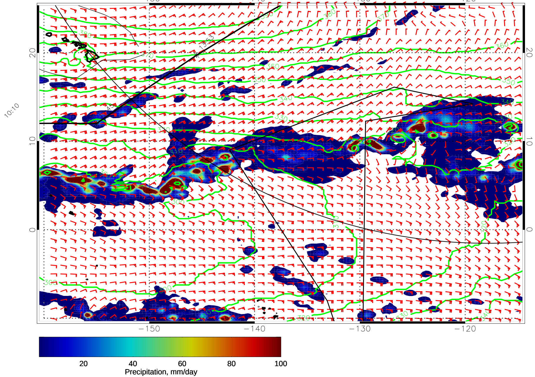
14121700, 120 hour forecast for 975mb Z, Precip., and Surface Winds (knots) -- NASA GEOS5
