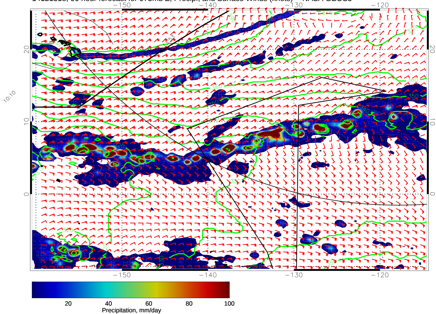
14121518, 90 hour forecast for 975mb Z, Precip., and Surface Winds (knots) -- NASA GEOS5
