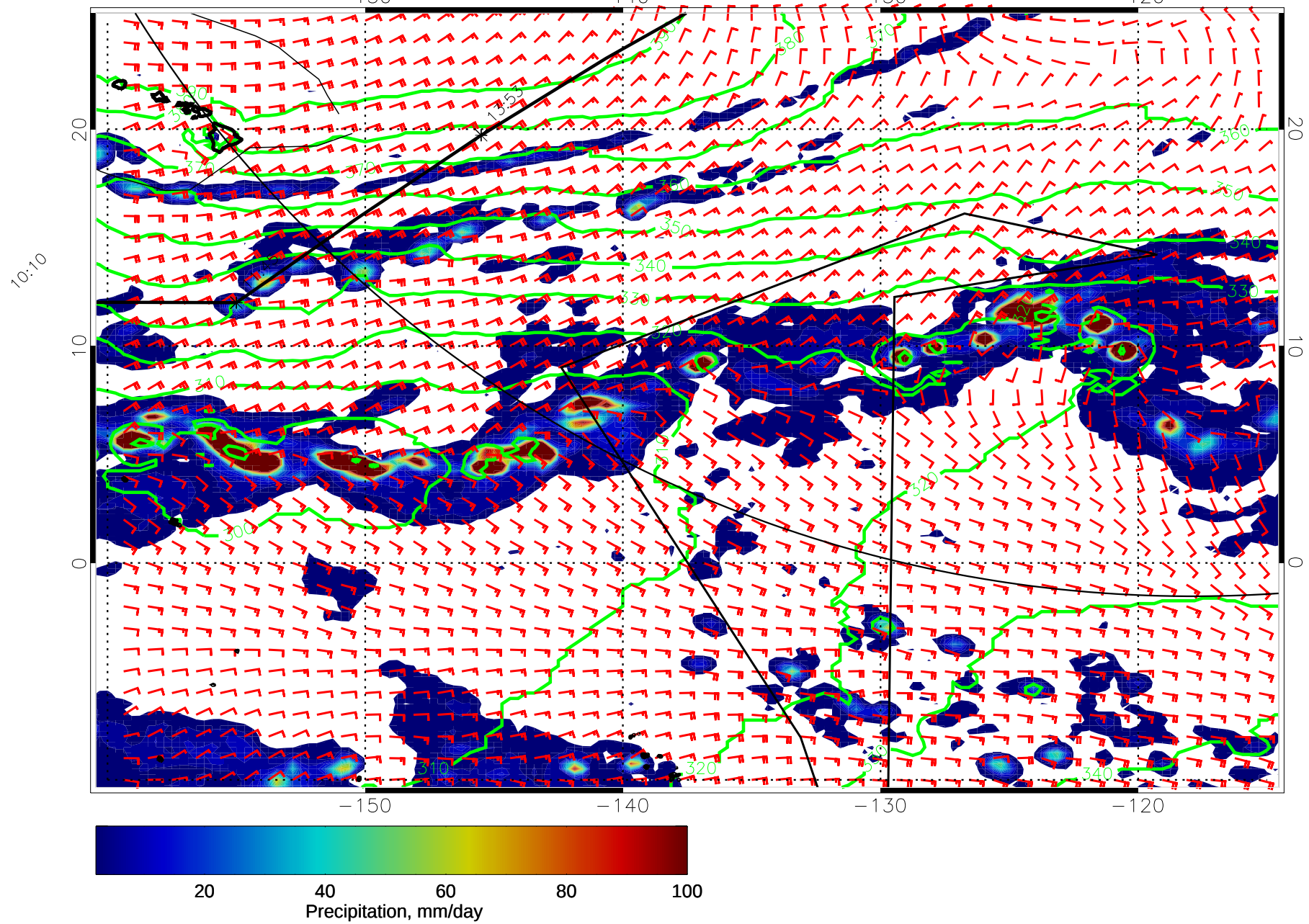
14121612, 108 hour forecast for 975mb Z, Precip., and Surface Winds (knots) -- NASA GEOS5
