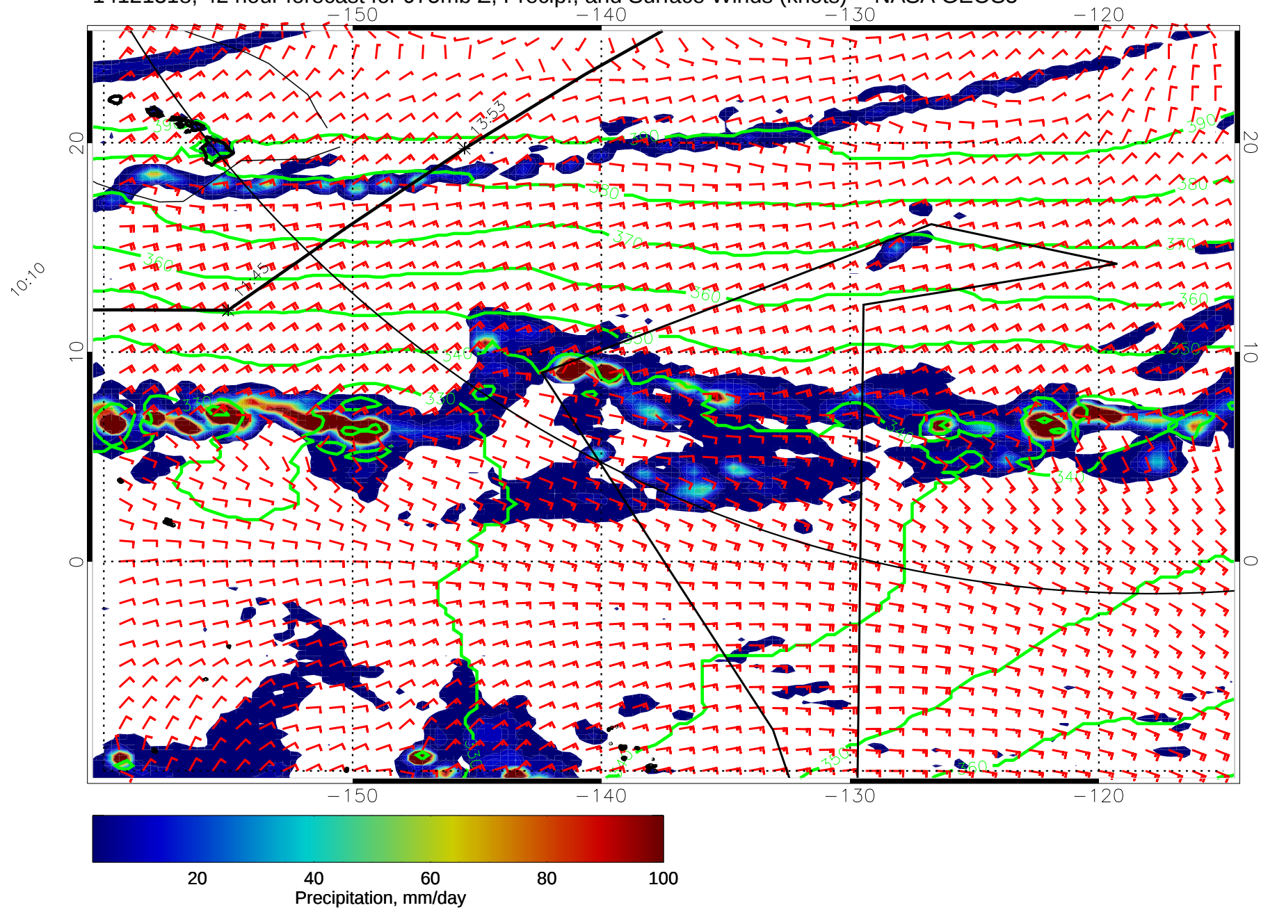
14121318, 42 hour forecast for 975mb Z, Precip., and Surface Winds (knots) -- NASA GEOS5
