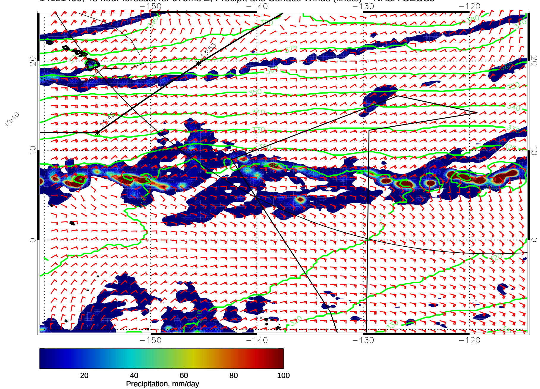
14121400, 48 hour forecast for 975mb Z, Precip., and Surface Winds (knots) -- NASA GEOS5
