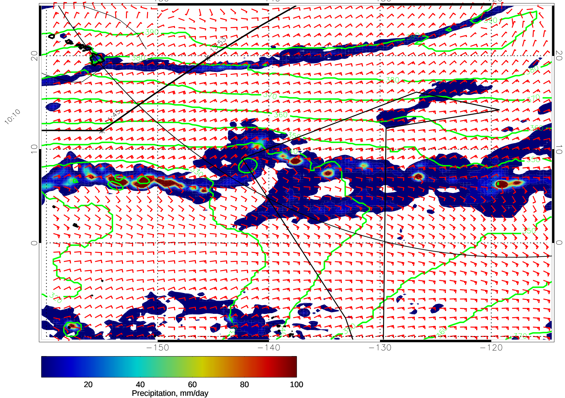
14121306, 30 hour forecast for 975mb Z, Precip., and Surface Winds (knots) -- NASA GEOS5
