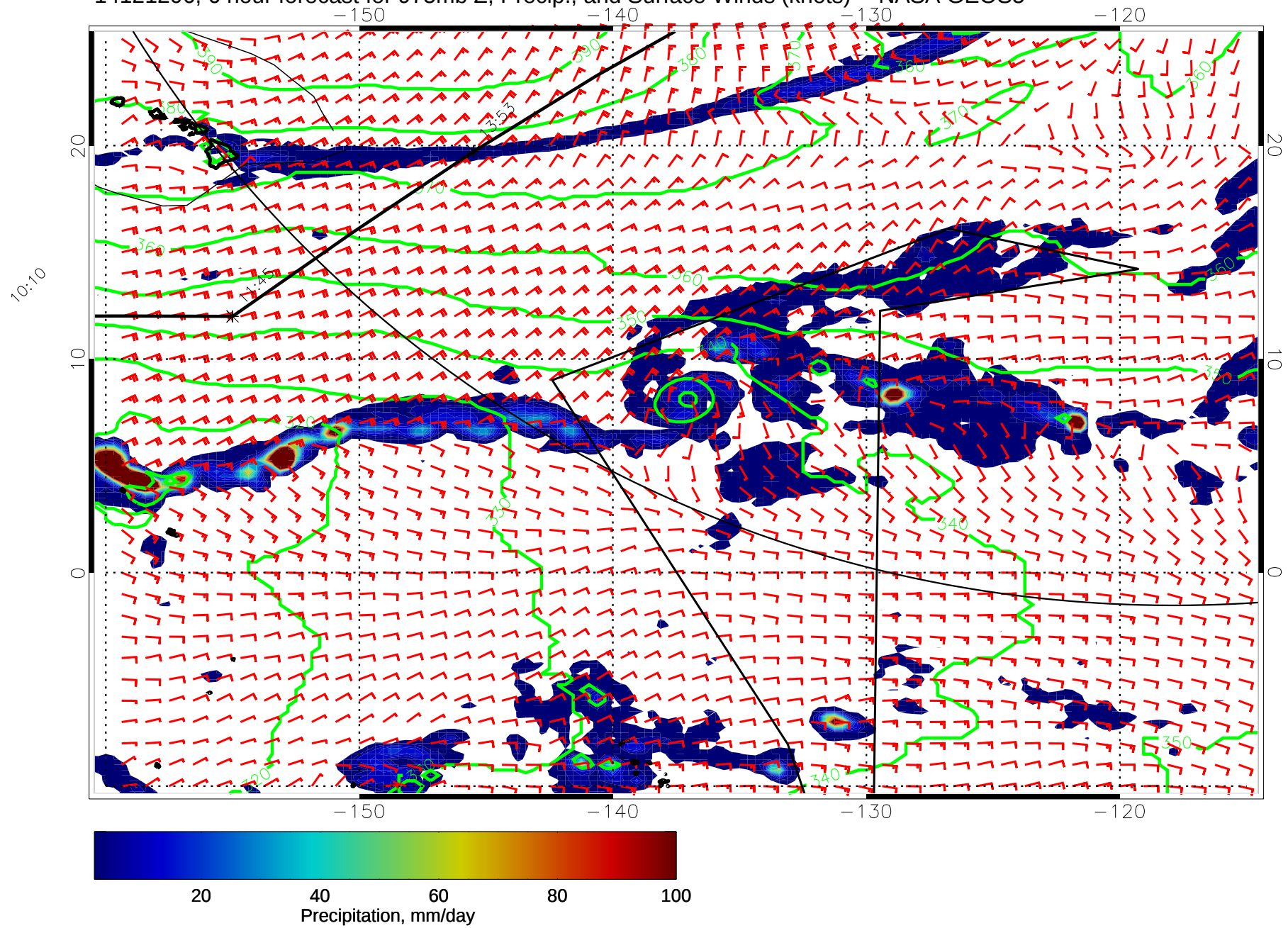
14121206, 6 hour forecast for 975mb Z, Precip., and Surface Winds (knots) -- NASA GEOS5
