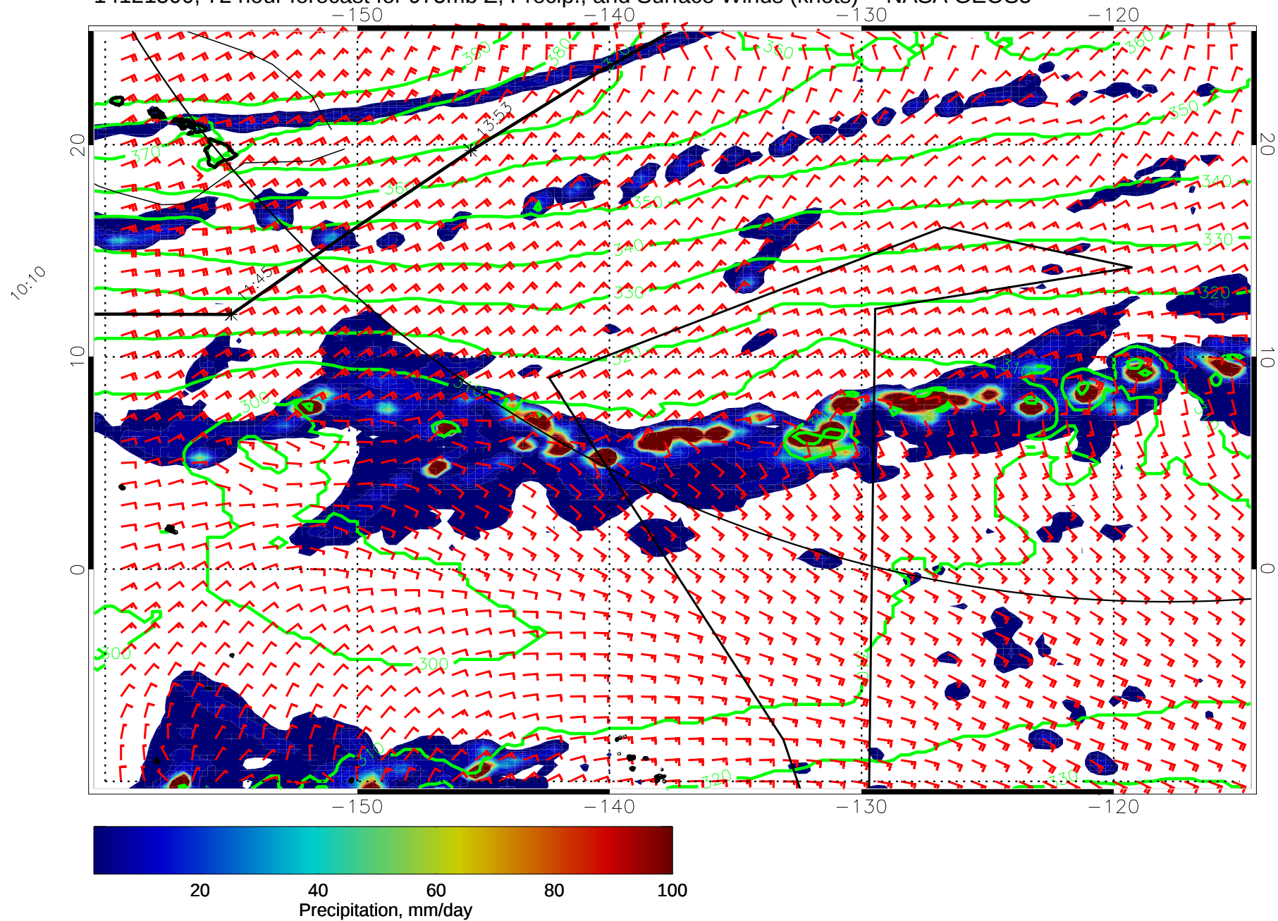
14121500, 72 hour forecast for 975mb Z, Precip., and Surface Winds (knots) -- NASA GEOS5
