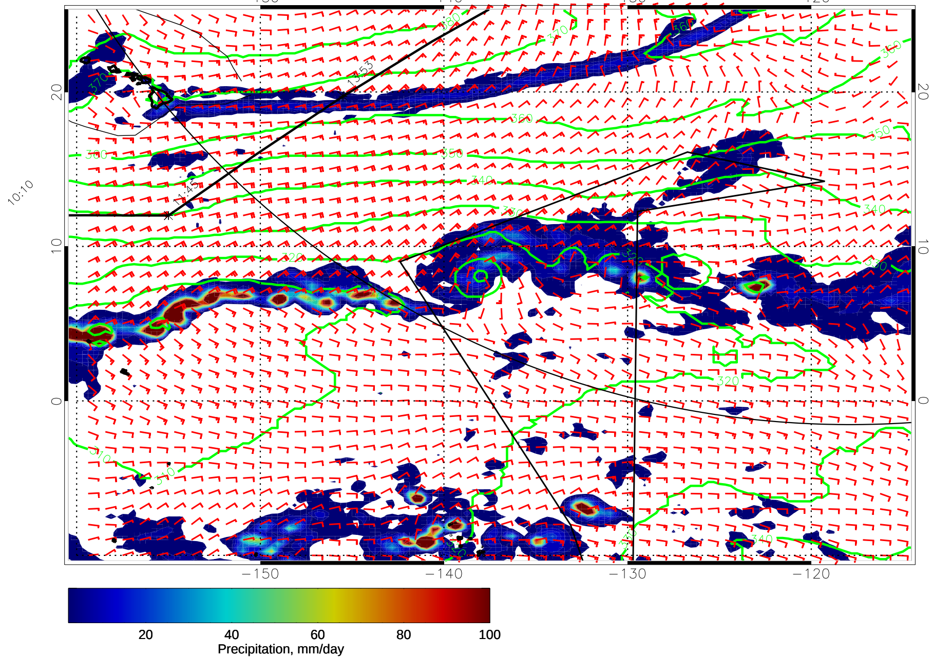
14121212, 12 hour forecast for 975mb Z, Precip., and Surface Winds (knots) -- NASA GEOS5
