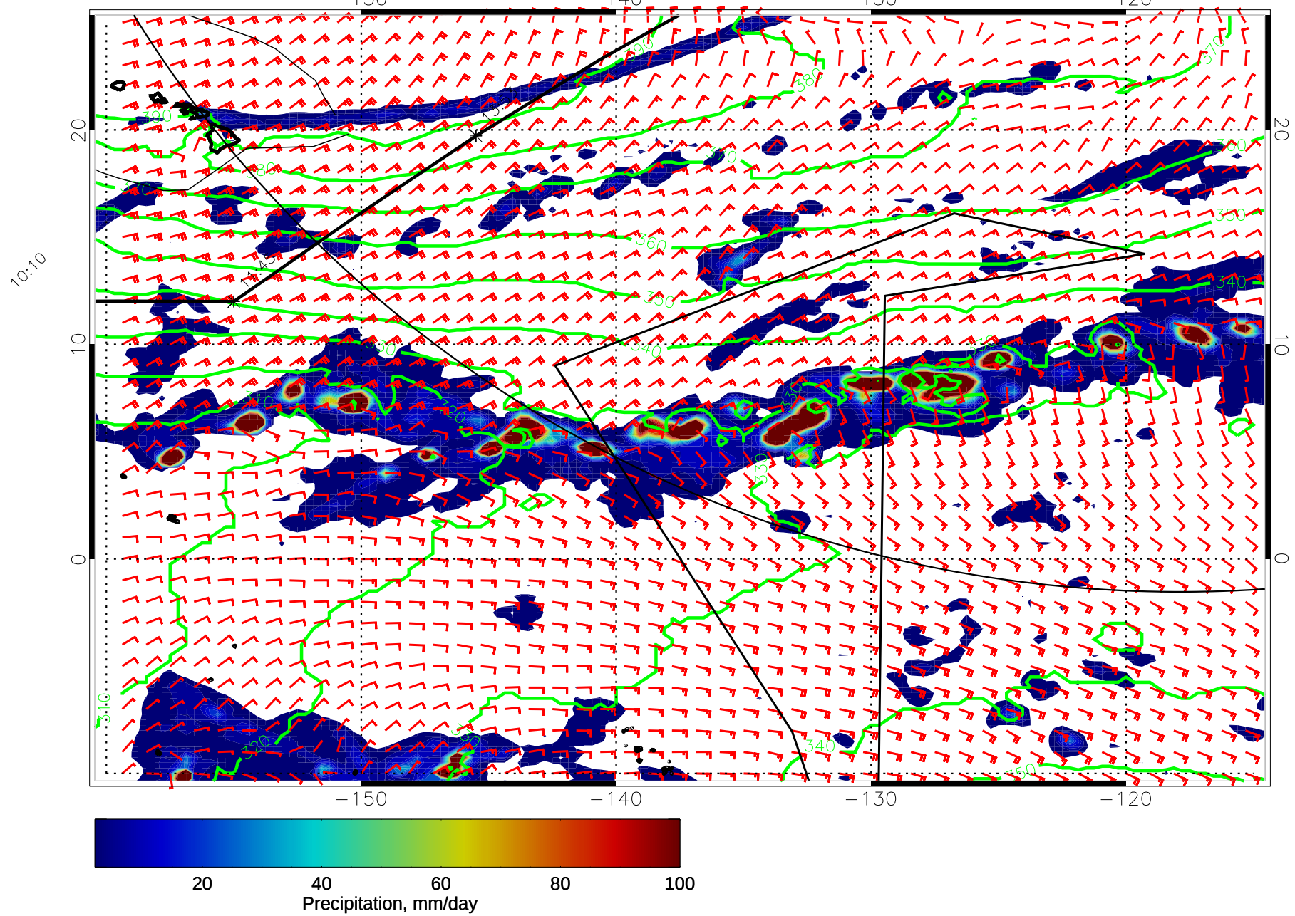
14121506, 78 hour forecast for 975mb Z, Precip., and Surface Winds (knots) -- NASA GEOS5
