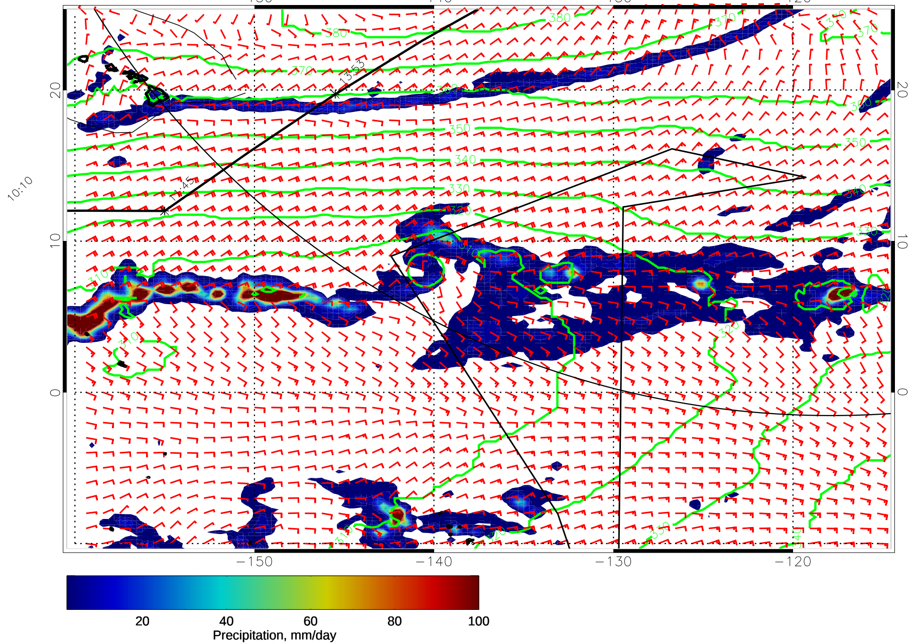
14121300, 24 hour forecast for 975mb Z, Precip., and Surface Winds (knots) -- NASA GEOS5
