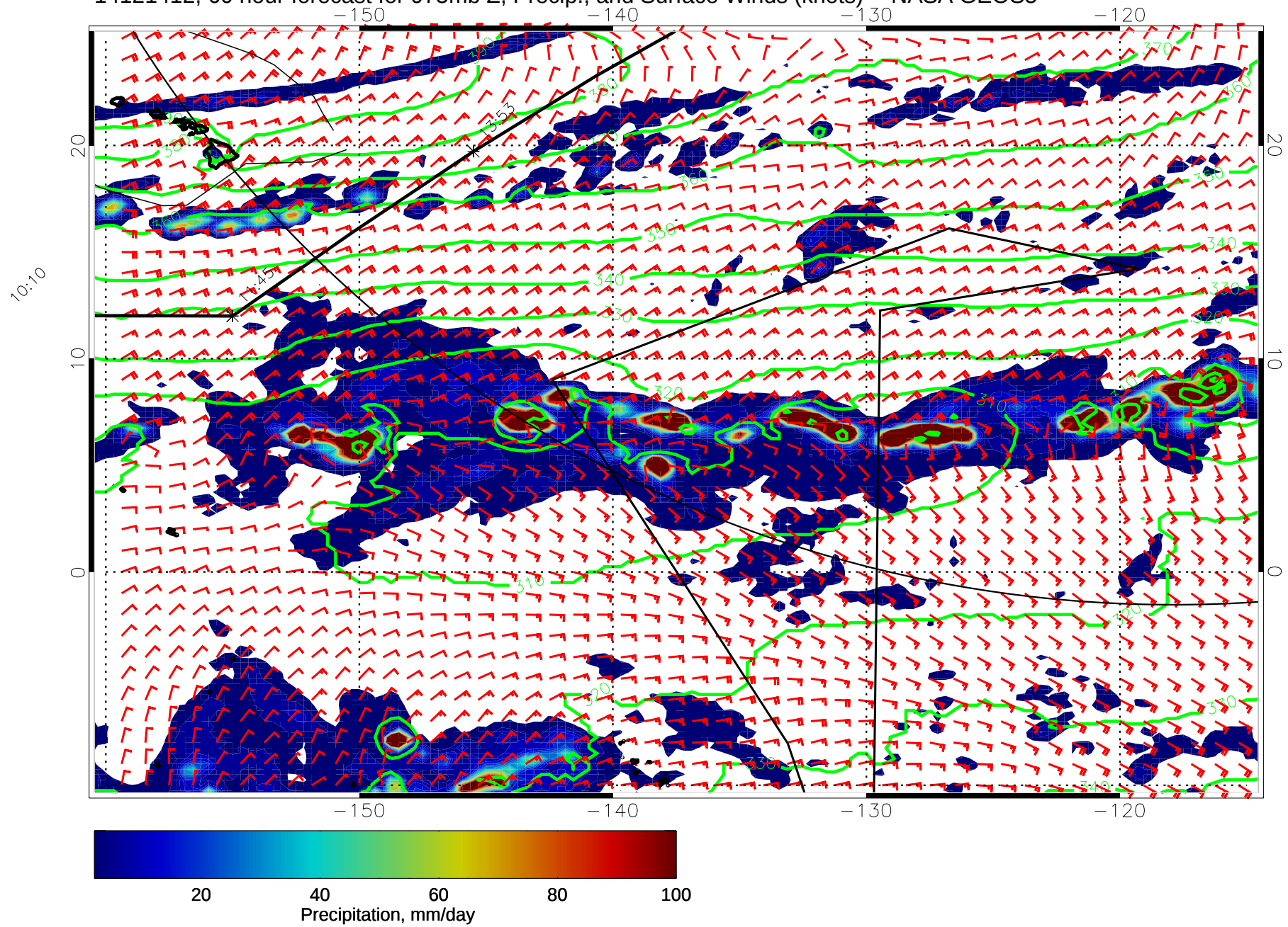
14121412, 60 hour forecast for 975mb Z, Precip., and Surface Winds (knots) -- NASA GEOS5
