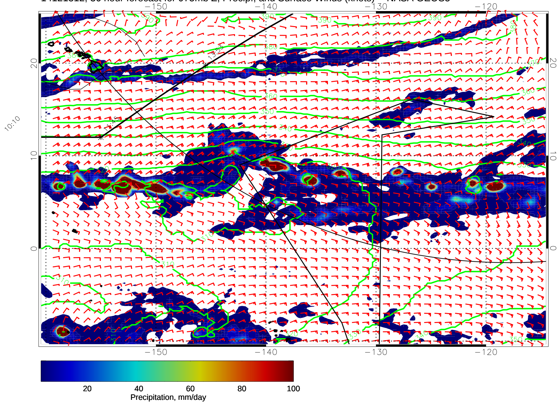
14121312, 36 hour forecast for 975mb Z, Precip., and Surface Winds (knots) -- NASA GEOS5
