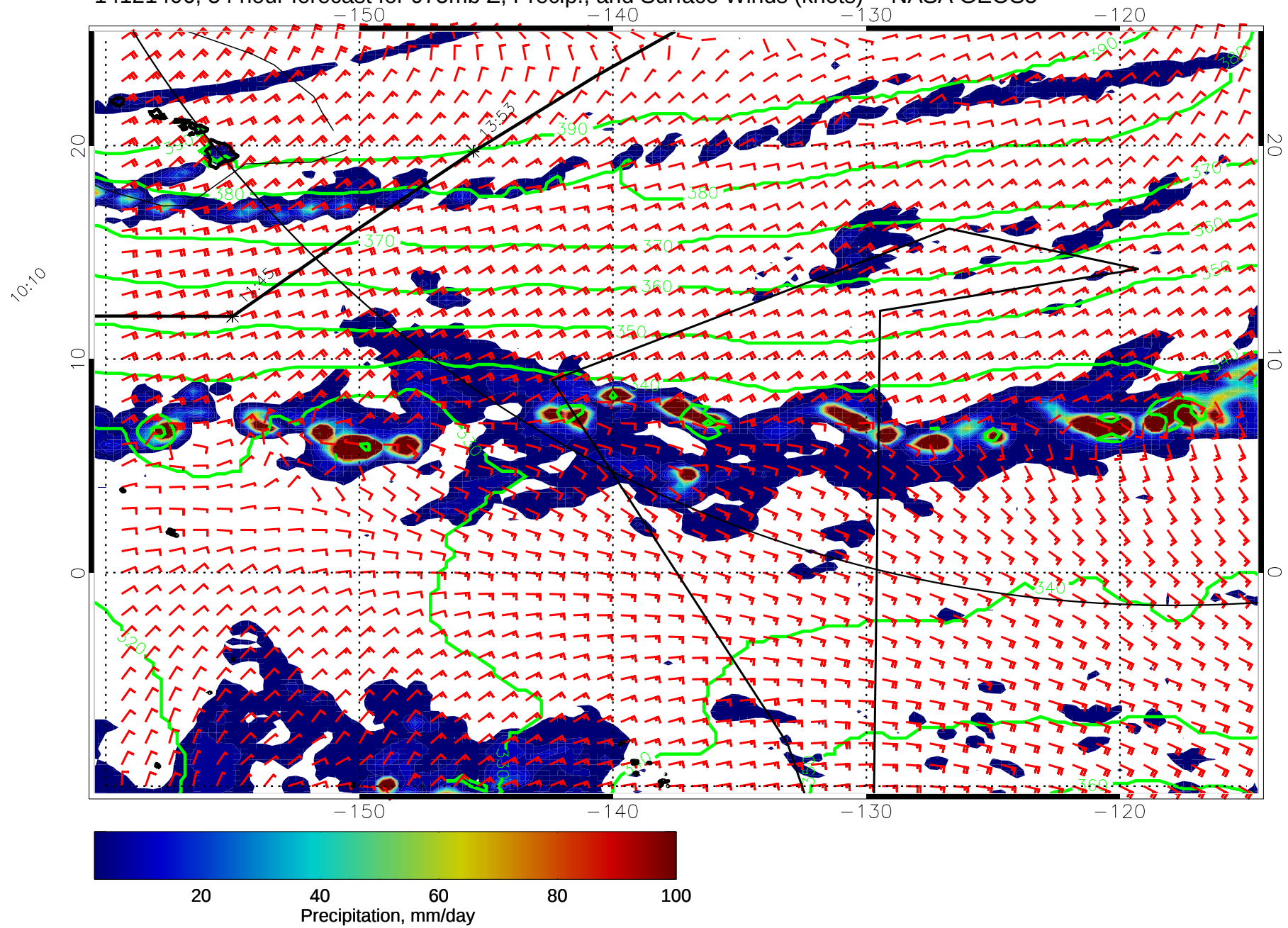
14121406, 54 hour forecast for 975mb Z, Precip., and Surface Winds (knots) -- NASA GEOS5
