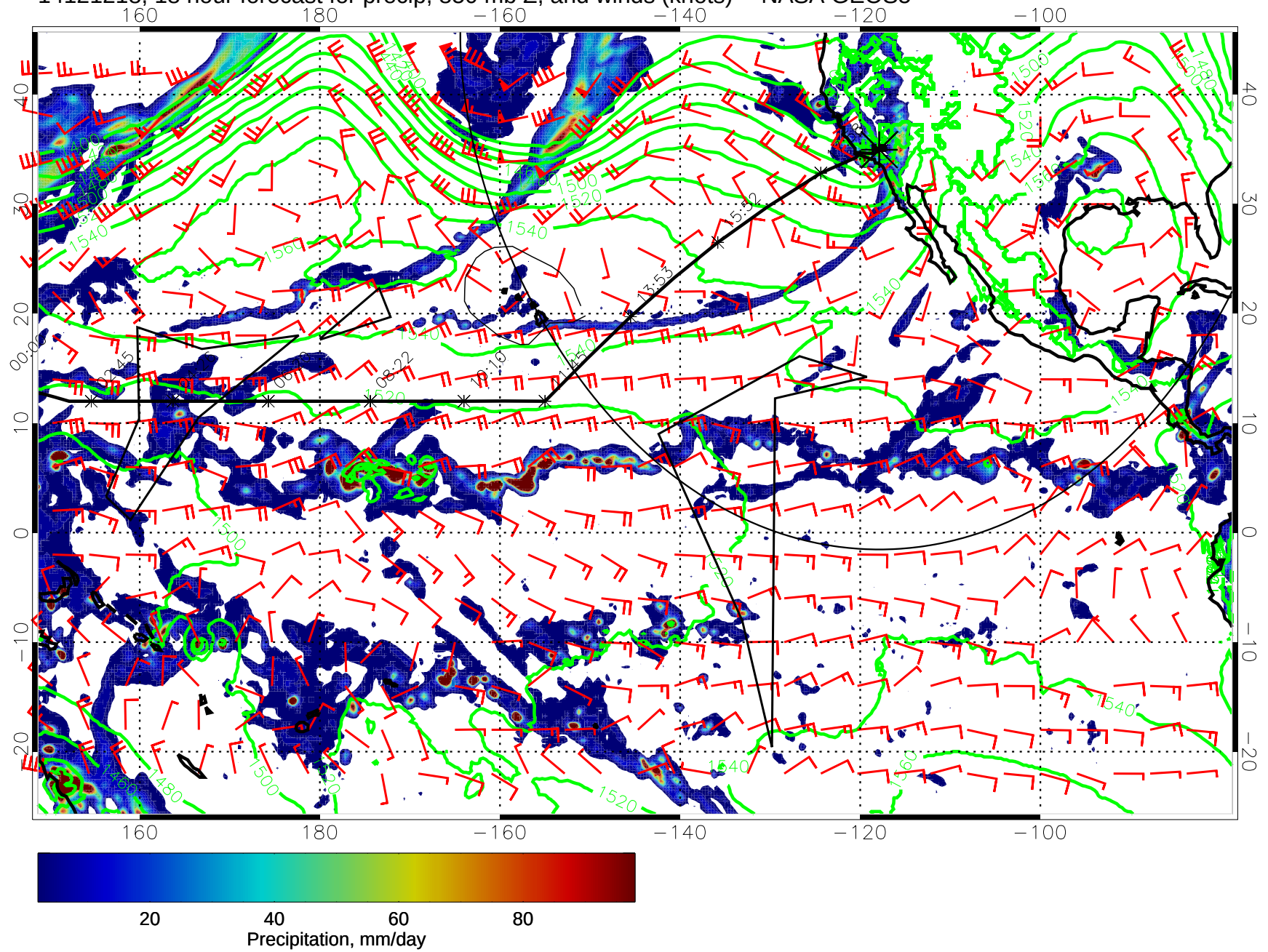
14121218, 18 hour forecast for precip, 850 mb Z, and winds (knots) -- NASA GEOS5
