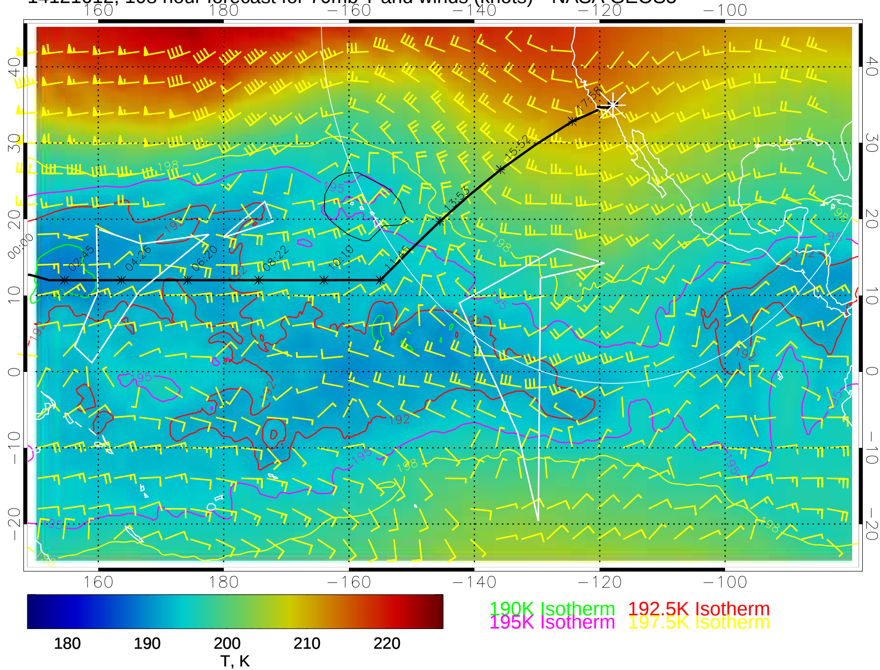
14121612, 108 hour forecast for 70mb T and winds (knots)-- NASA GEOS5
