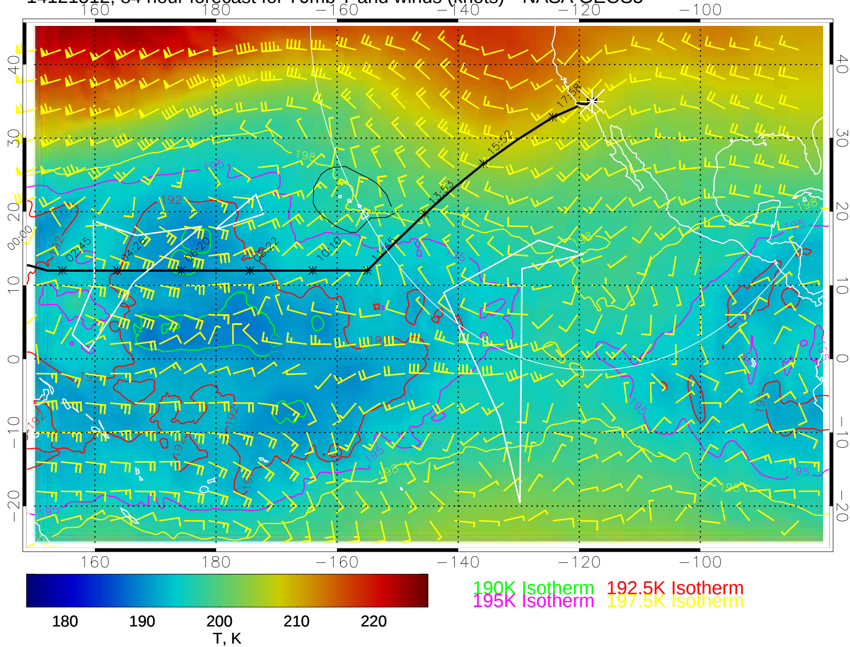
14121512, 84 hour forecast for 70mb T and winds (knots)-- NASA GEOS5
