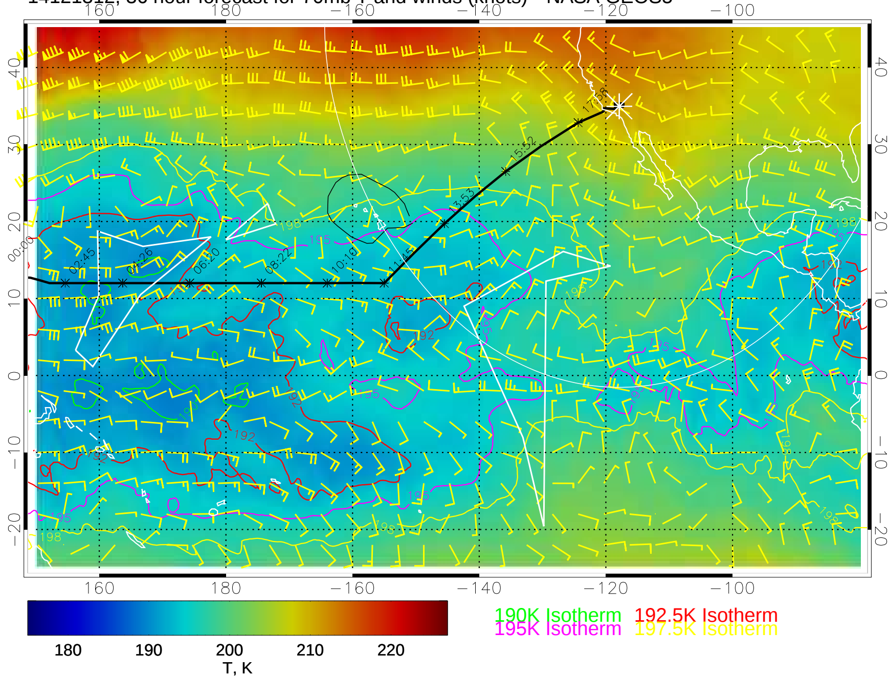
14121312, 36 hour forecast for 70mb T and winds (knots)-- NASA GEOS5
