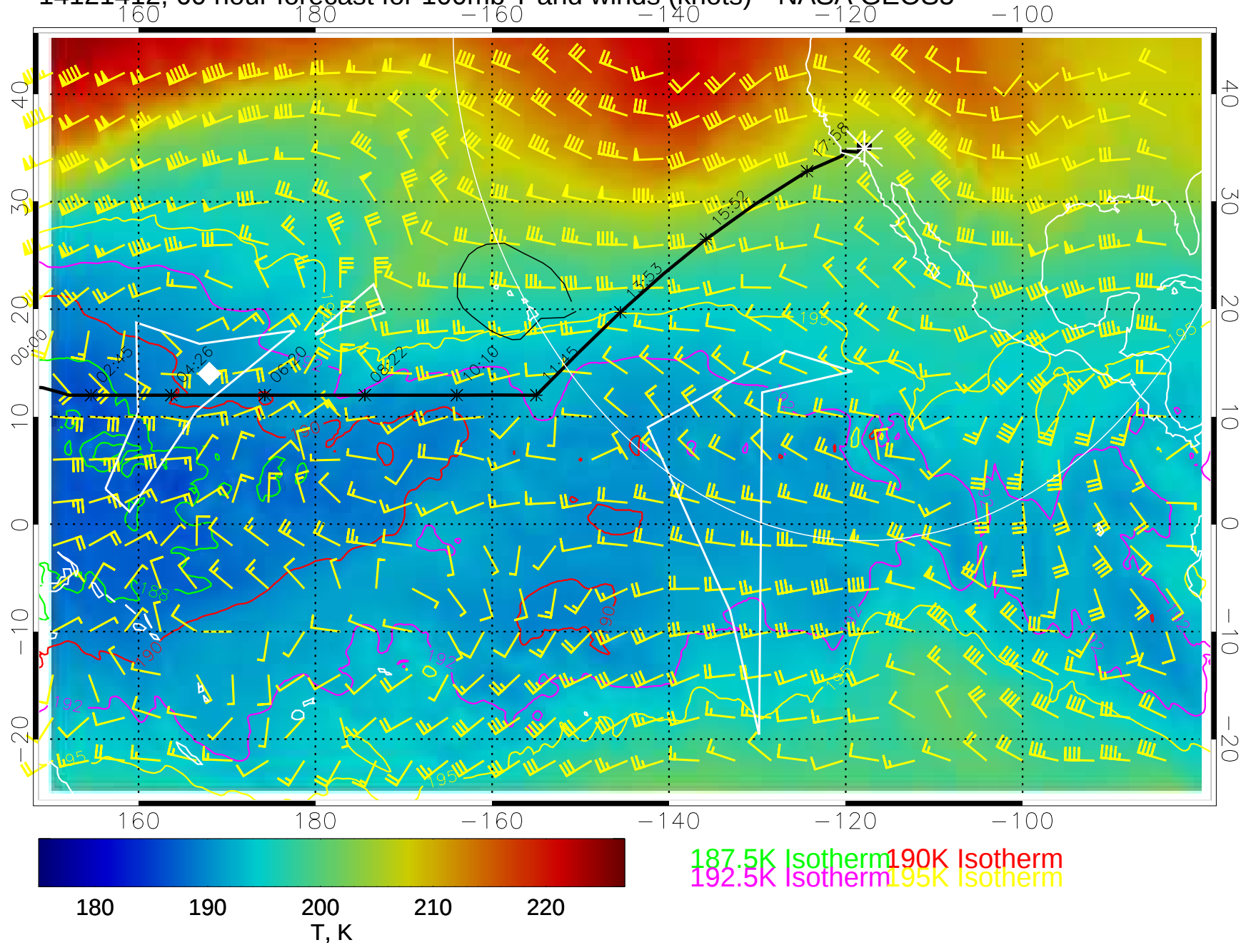
14121412, 60 hour forecast for 100mb T and winds (knots)-- NASA GEOS5
