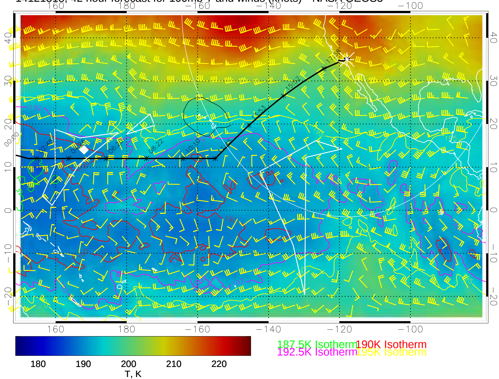
14121318, 42 hour forecast for 100mb T and winds (knots)-- NASA GEOS5
