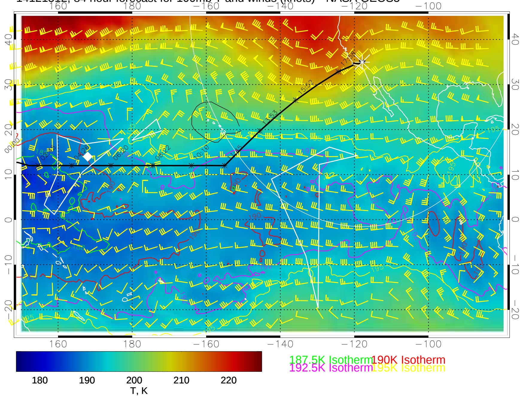
14121512, 84 hour forecast for 100mb T and winds (knots)-- NASA GEOS5
