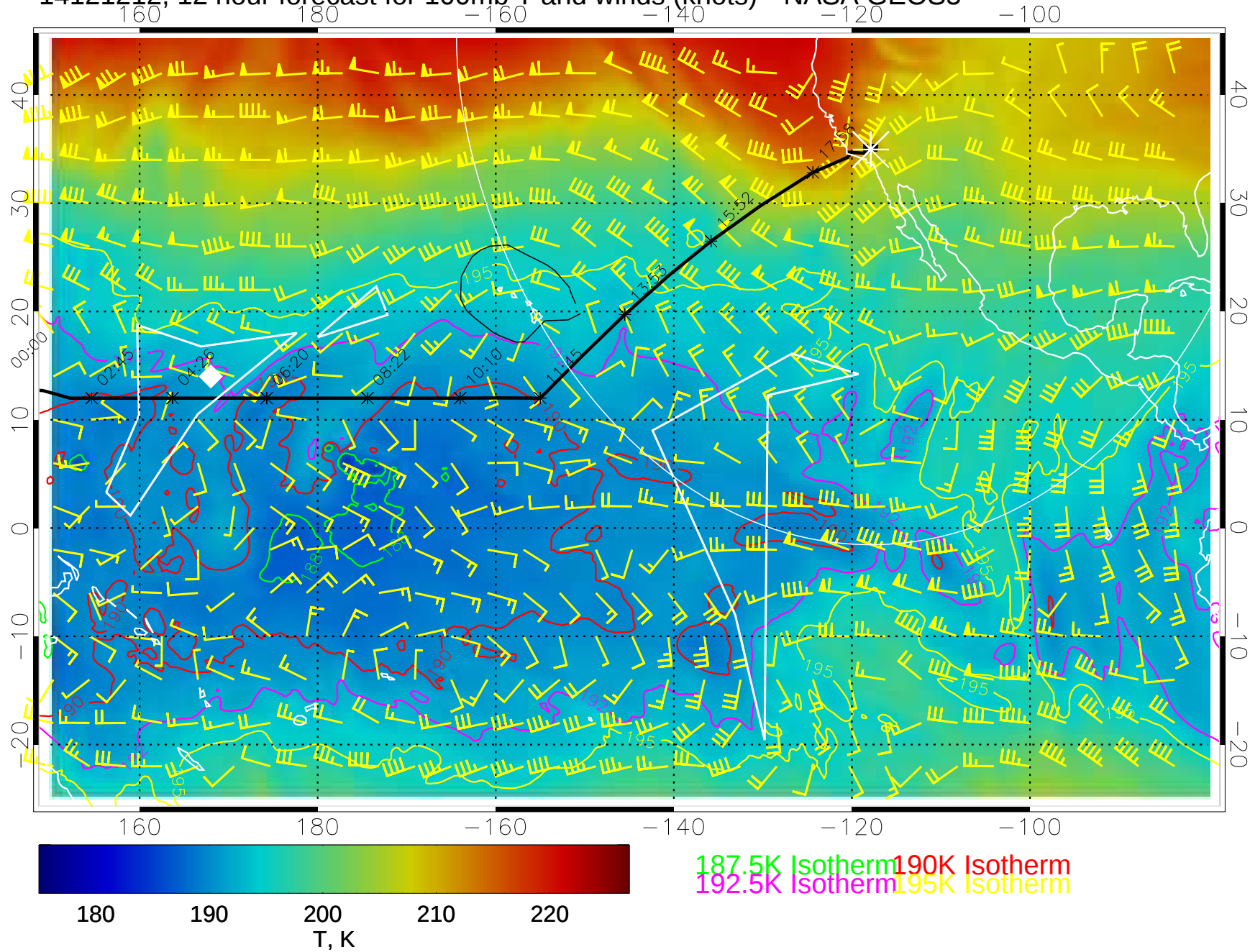
14121212, 12 hour forecast for 100mb T and winds (knots)-- NASA GEOS5
