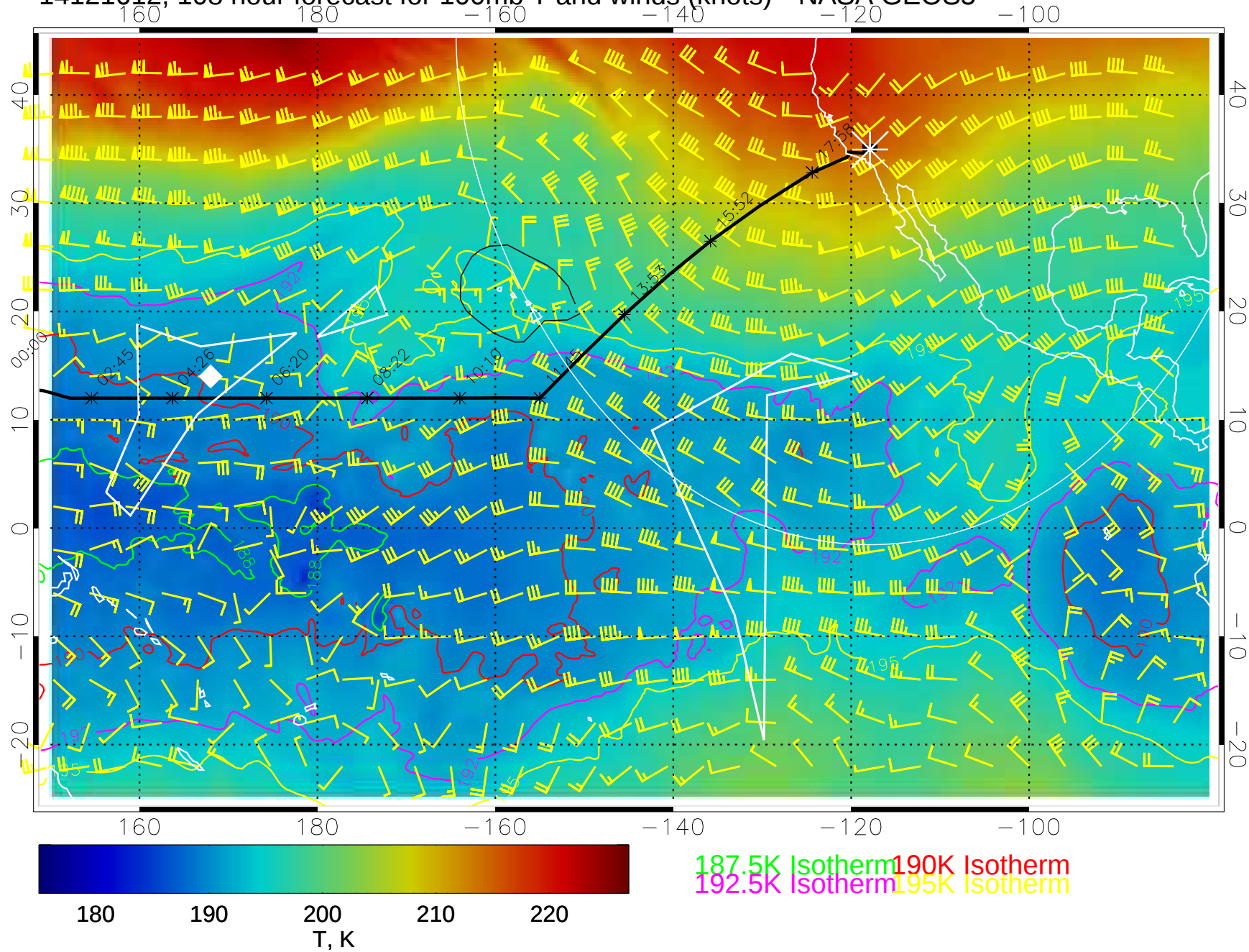
14121612, 108 hour forecast for 100mb T and winds (knots)-- NASA GEOS5
