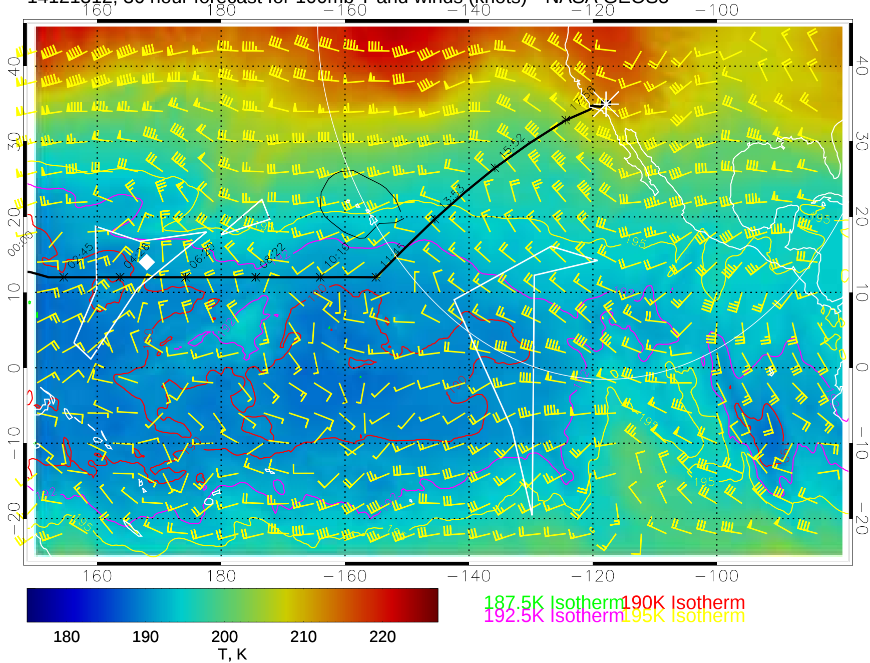
14121312, 36 hour forecast for 100mb T and winds (knots)-- NASA GEOS5
