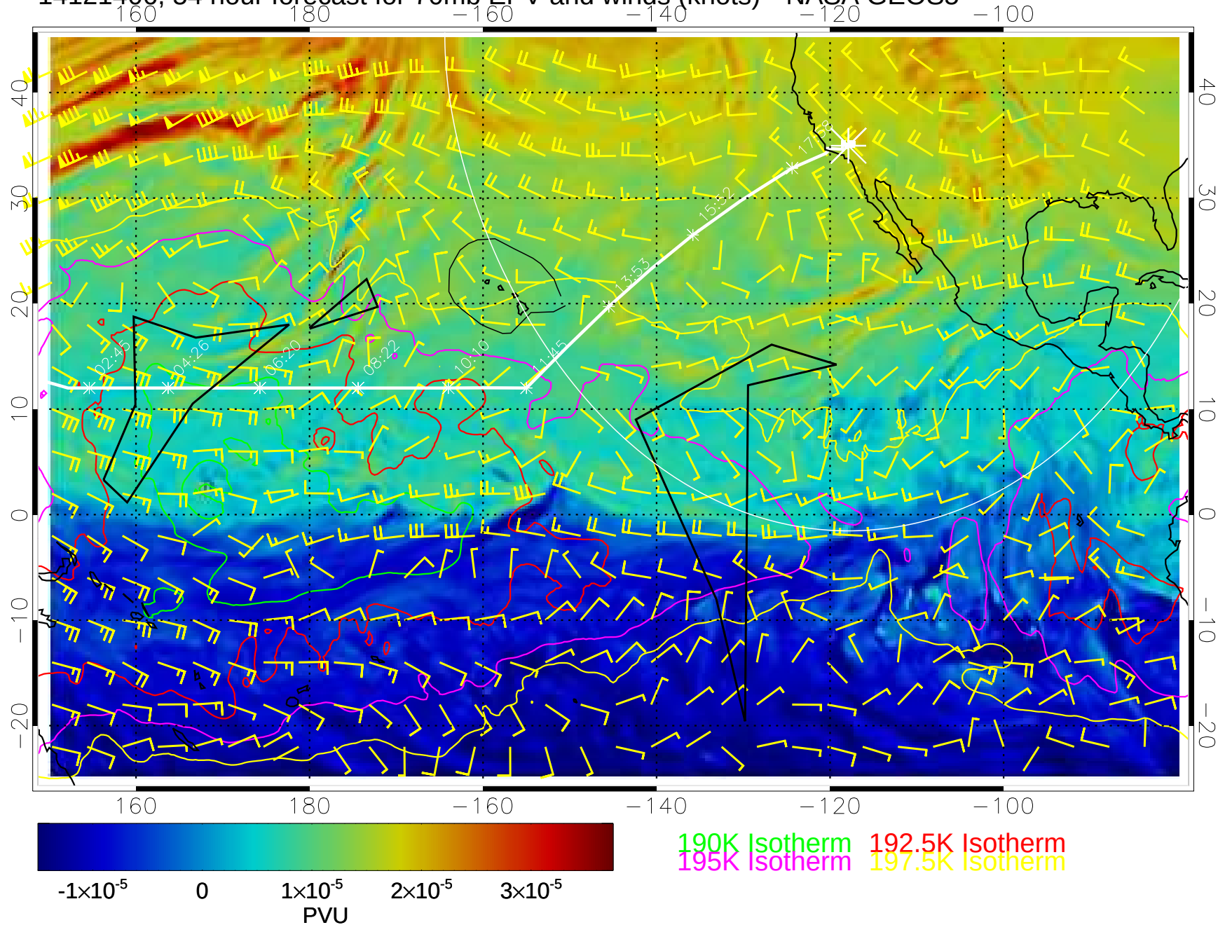
14121406, 54 hour forecast for 70mb EPV and winds (knots)-- NASA GEOS5
