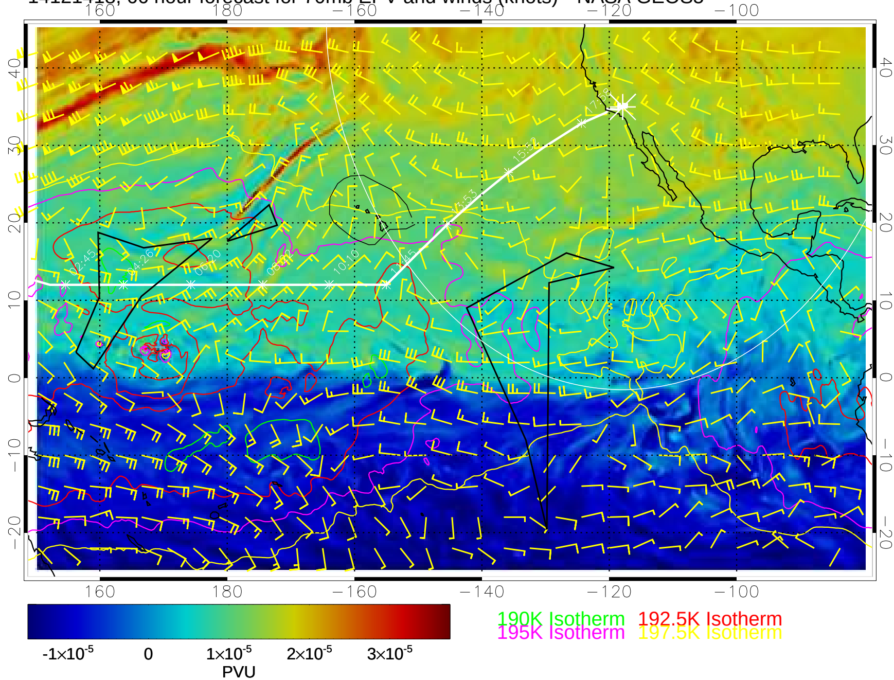
14121418, 66 hour forecast for 70mb EPV and winds (knots)-- NASA GEOS5
