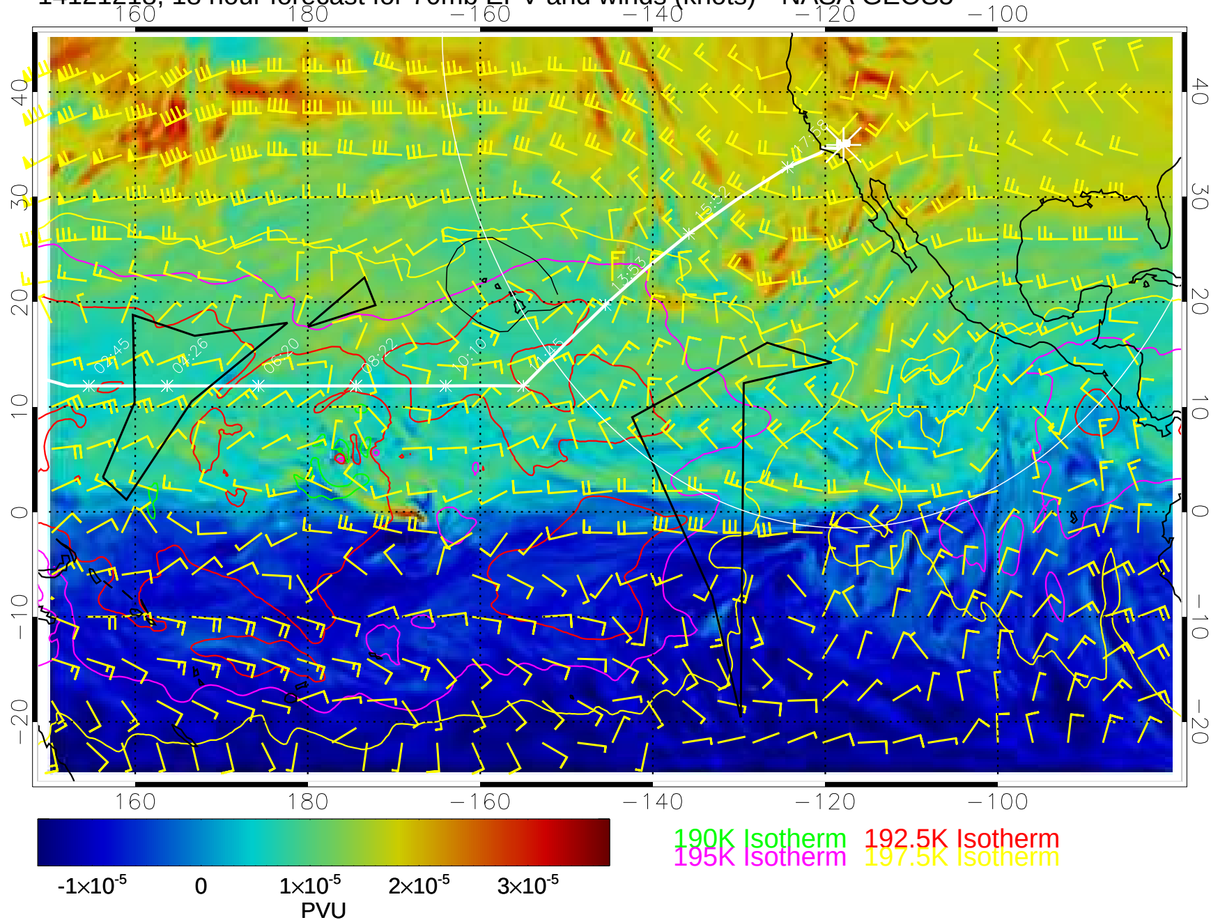
14121218, 18 hour forecast for 70mb EPV and winds (knots)-- NASA GEOS5
