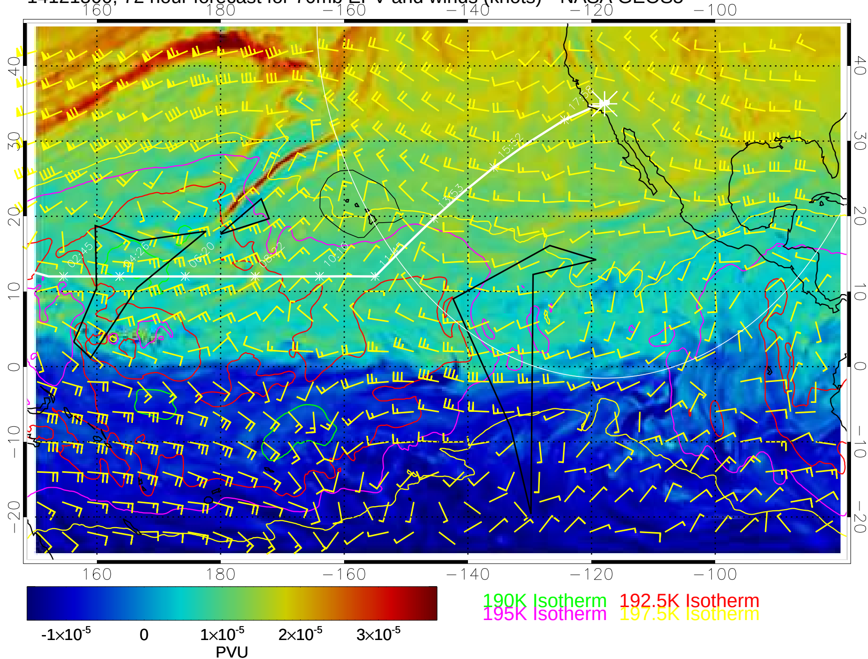
14121500, 72 hour forecast for 70mb EPV and winds (knots)-- NASA GEOS5
