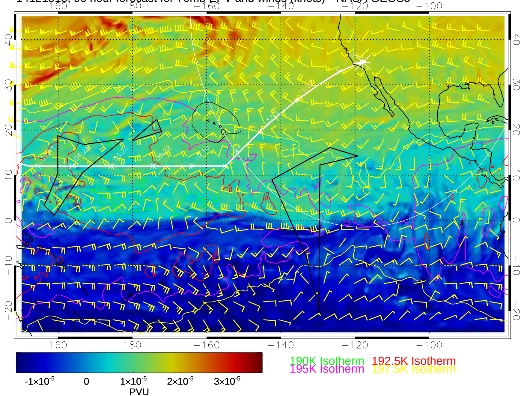
14121518, 90 hour forecast for 70mb EPV and winds (knots)-- NASA GEOS5
