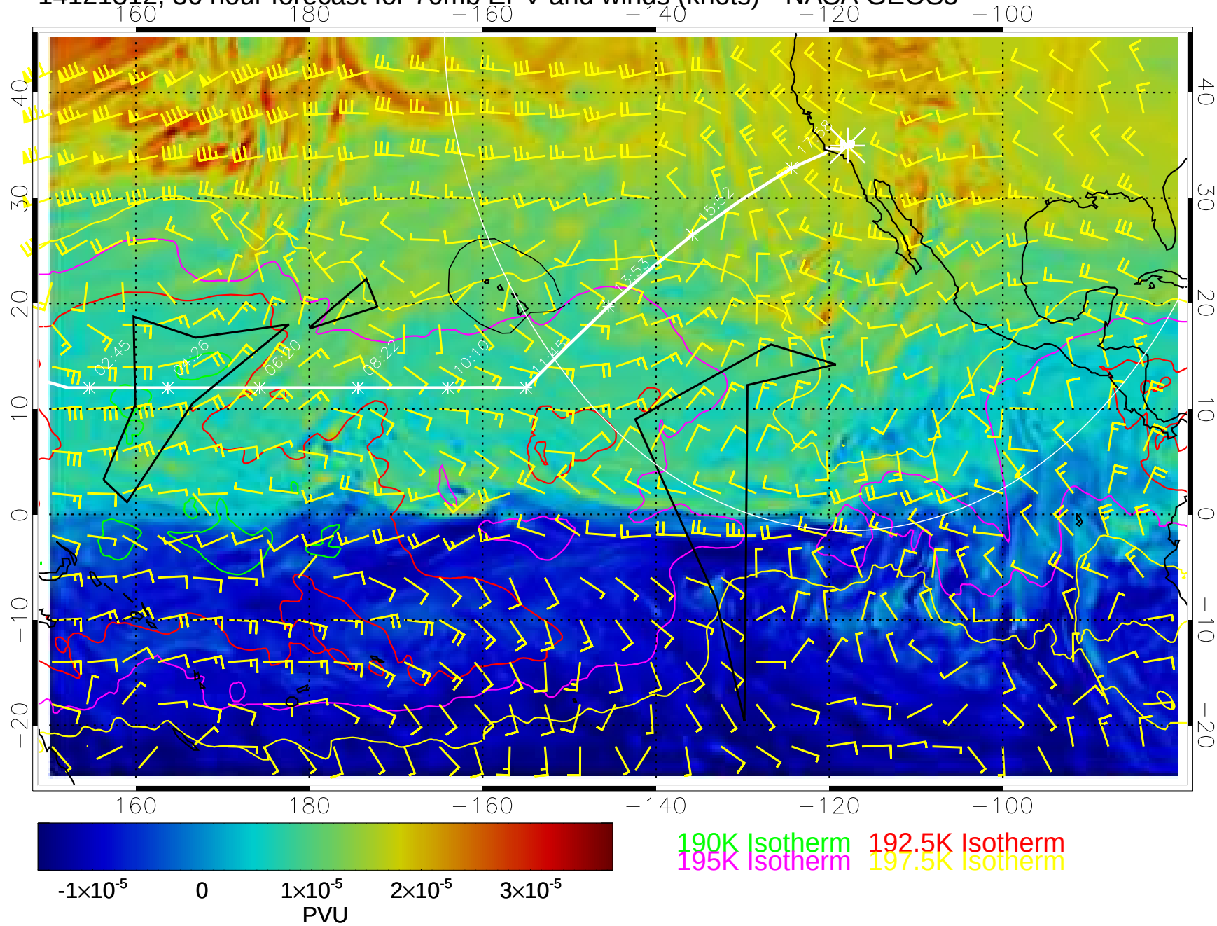
14121312, 36 hour forecast for 70mb EPV and winds (knots)-- NASA GEOS5
