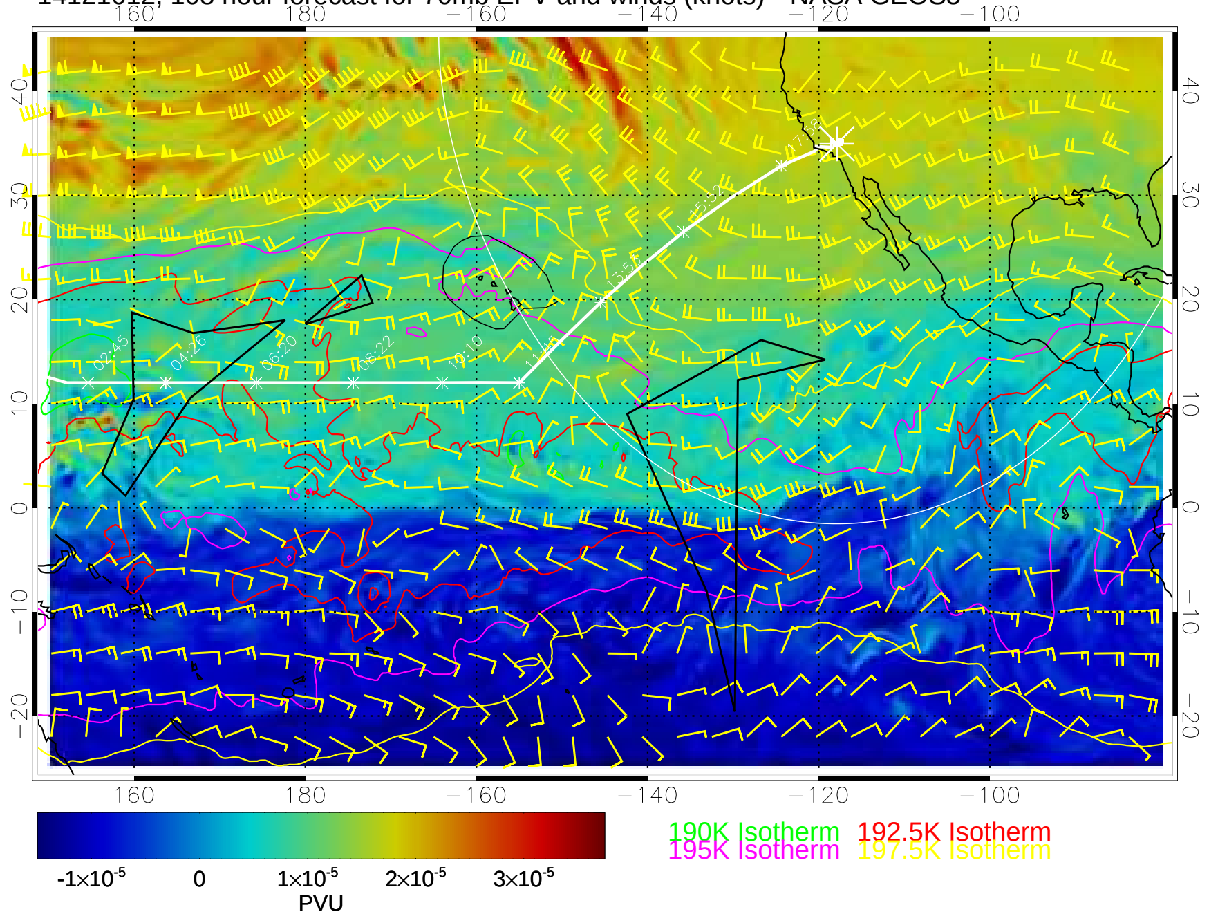
14121612, 108 hour forecast for 70mb EPV and winds (knots)-- NASA GEOS5
