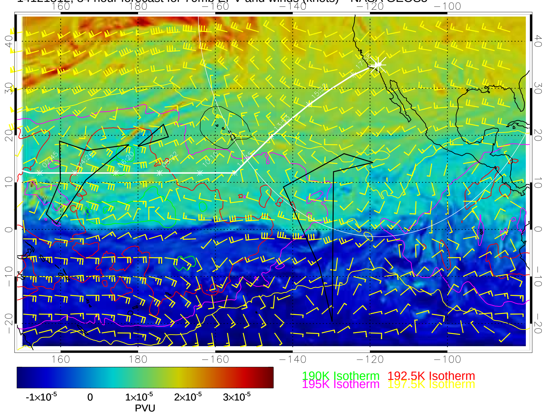
14121512, 84 hour forecast for 70mb EPV and winds (knots)-- NASA GEOS5
