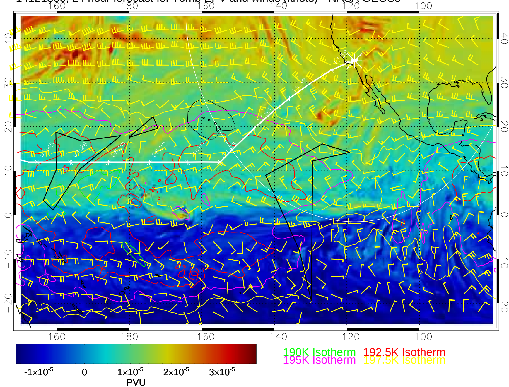
14121300, 24 hour forecast for 70mb EPV and winds (knots)-- NASA GEOS5
