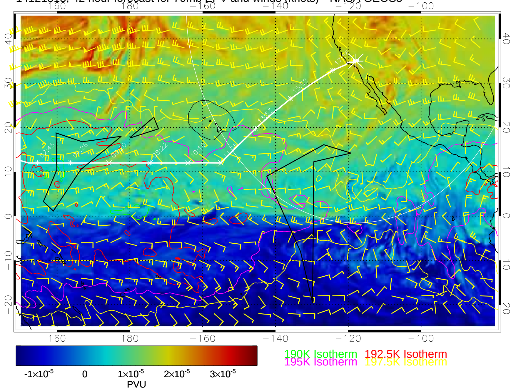
14121318, 42 hour forecast for 70mb EPV and winds (knots)-- NASA GEOS5
