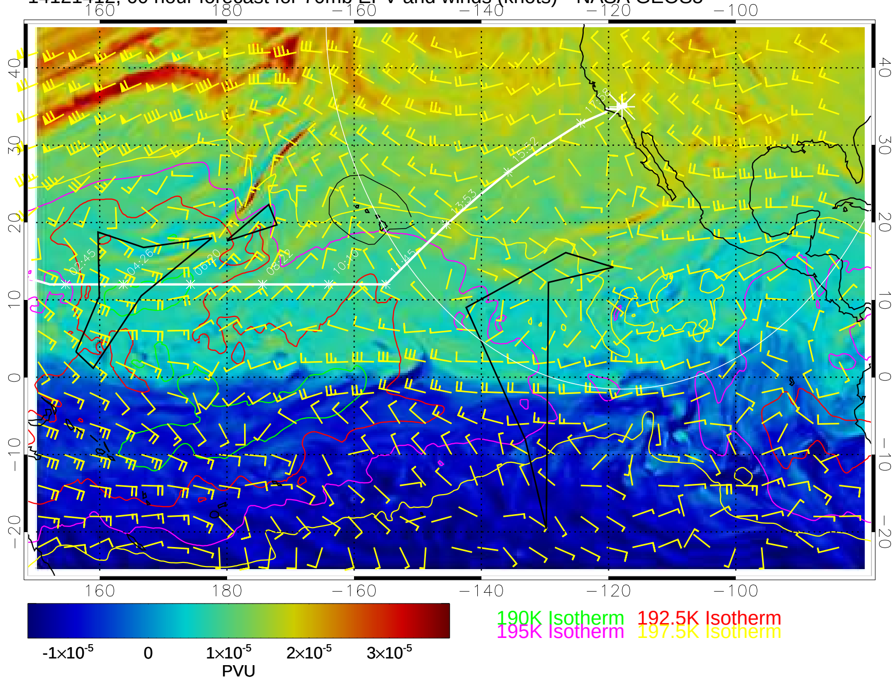
14121412, 60 hour forecast for 70mb EPV and winds (knots)-- NASA GEOS5
