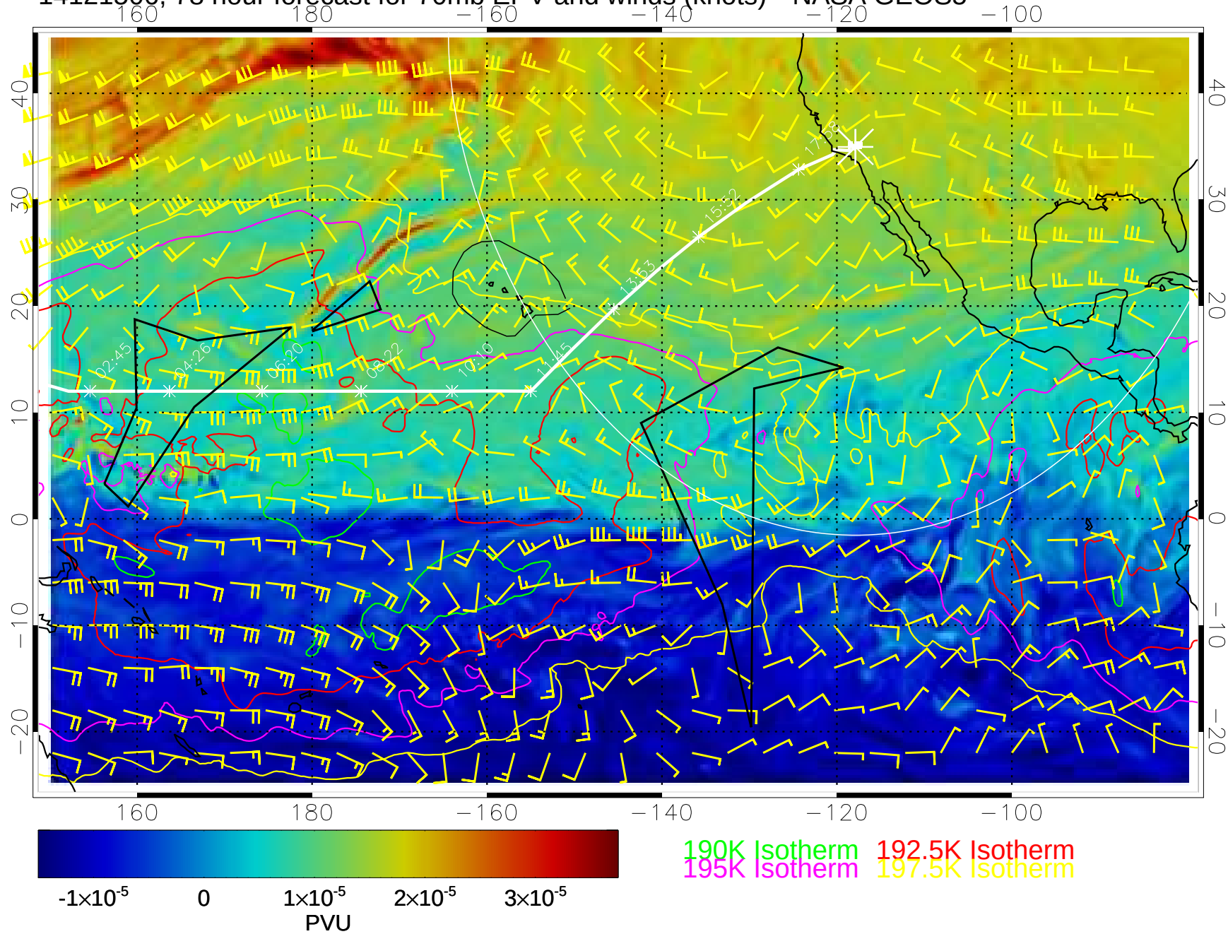
14121506, 78 hour forecast for 70mb EPV and winds (knots)-- NASA GEOS5
