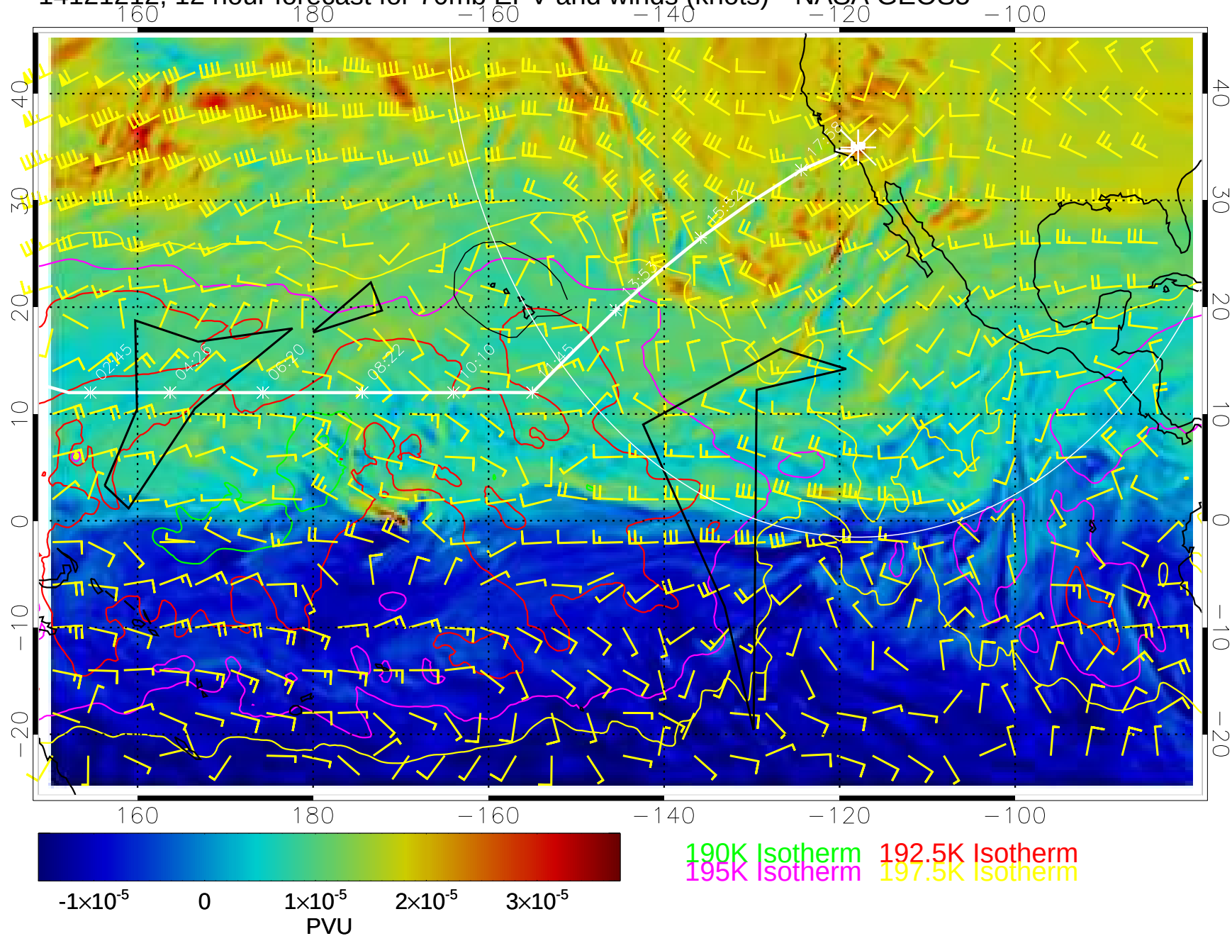
14121212, 12 hour forecast for 70mb EPV and winds (knots)-- NASA GEOS5
