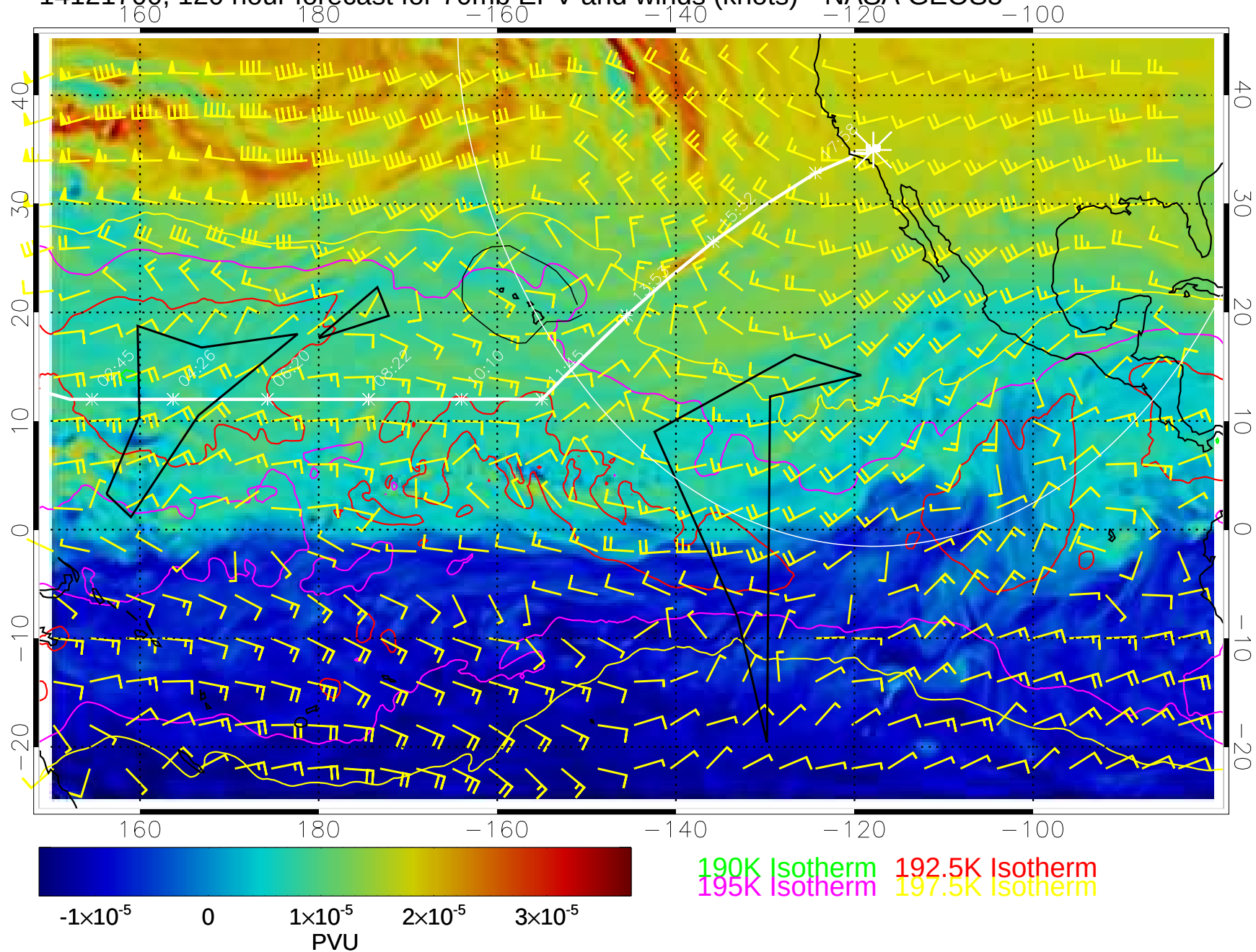
14121700, 120 hour forecast for 70mb EPV and winds (knots)-- NASA GEOS5
