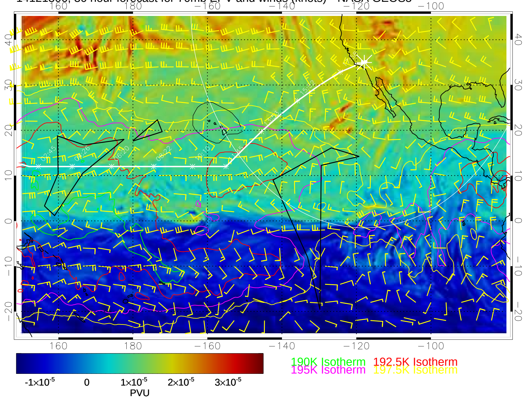
14121306, 30 hour forecast for 70mb EPV and winds (knots)-- NASA GEOS5
