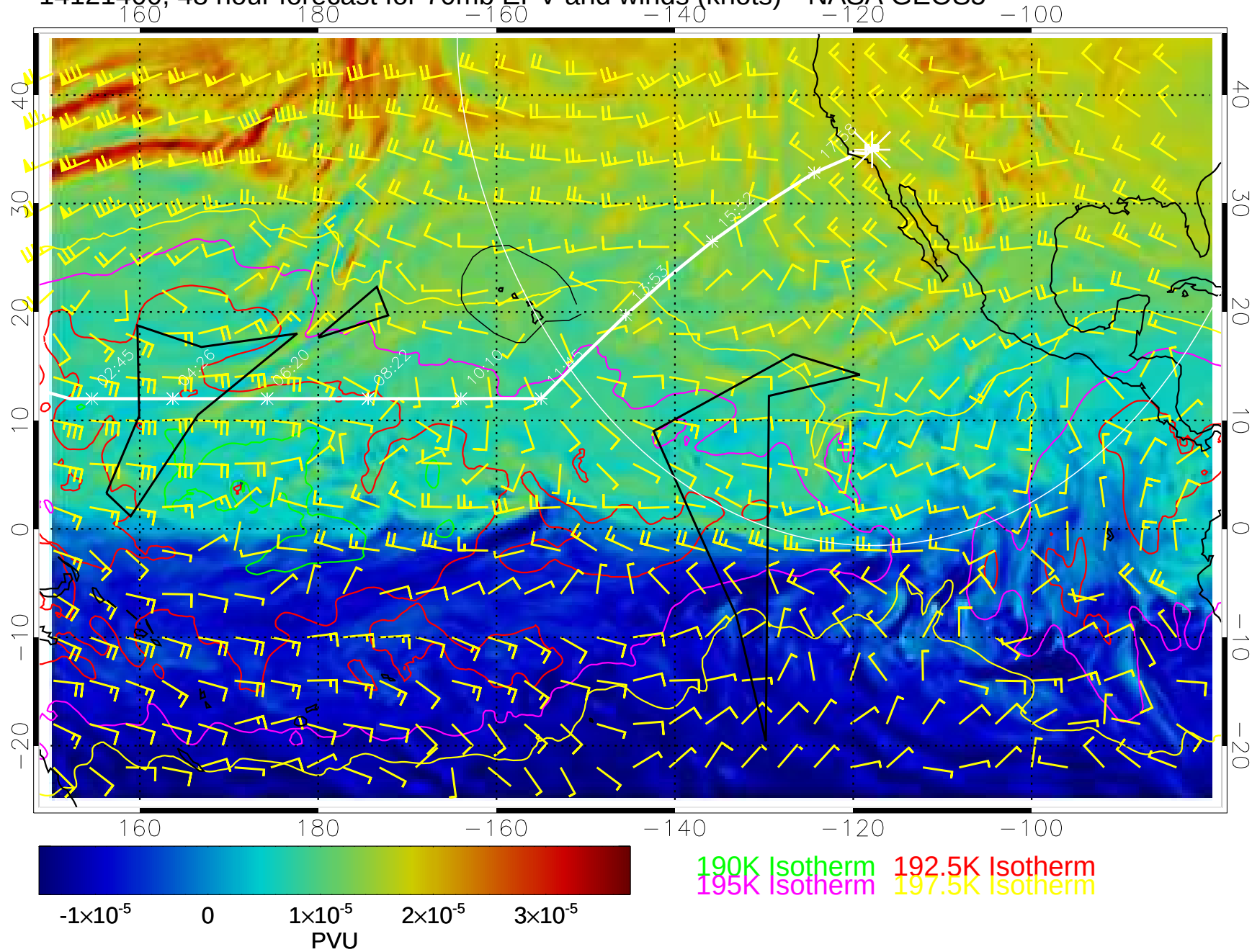
14121400, 48 hour forecast for 70mb EPV and winds (knots)-- NASA GEOS5
