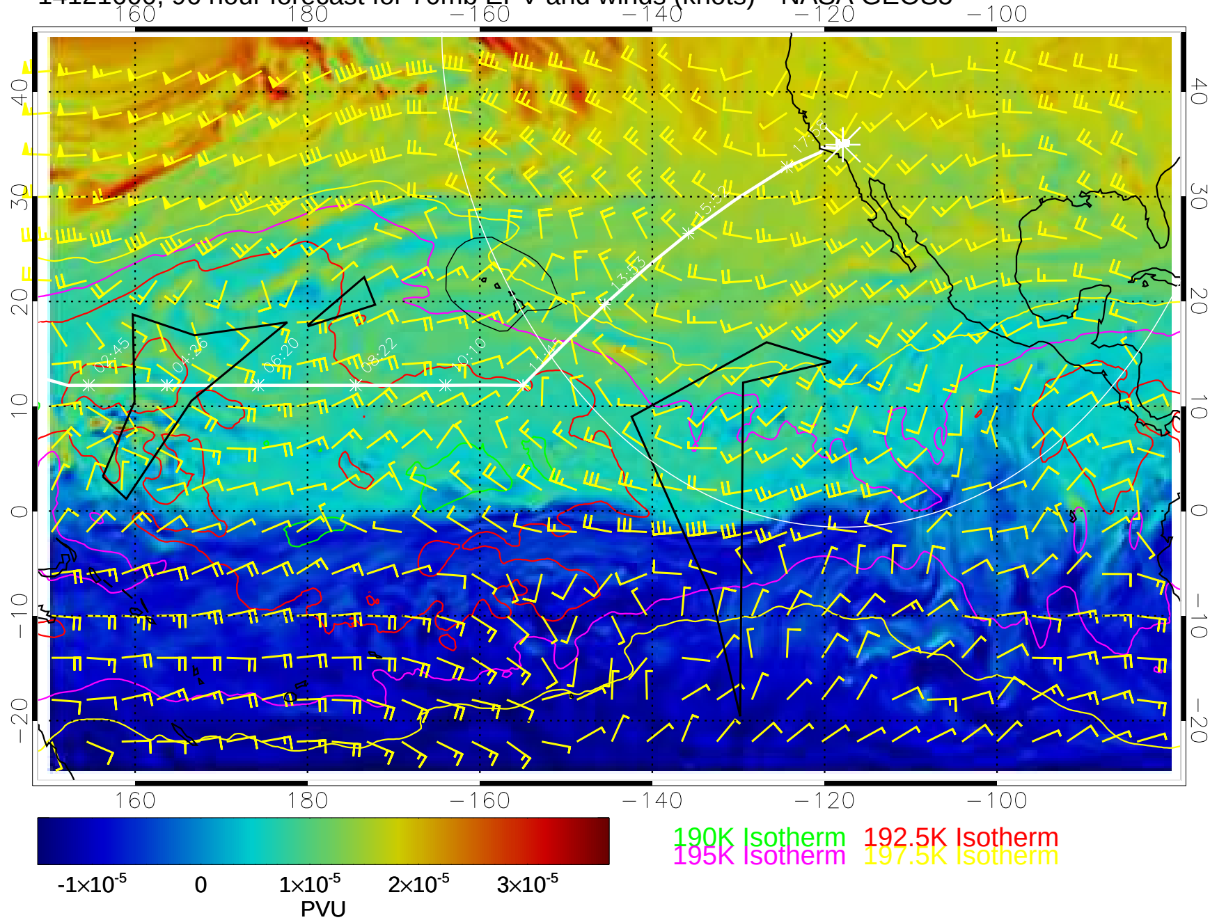
14121600, 96 hour forecast for 70mb EPV and winds (knots)-- NASA GEOS5
