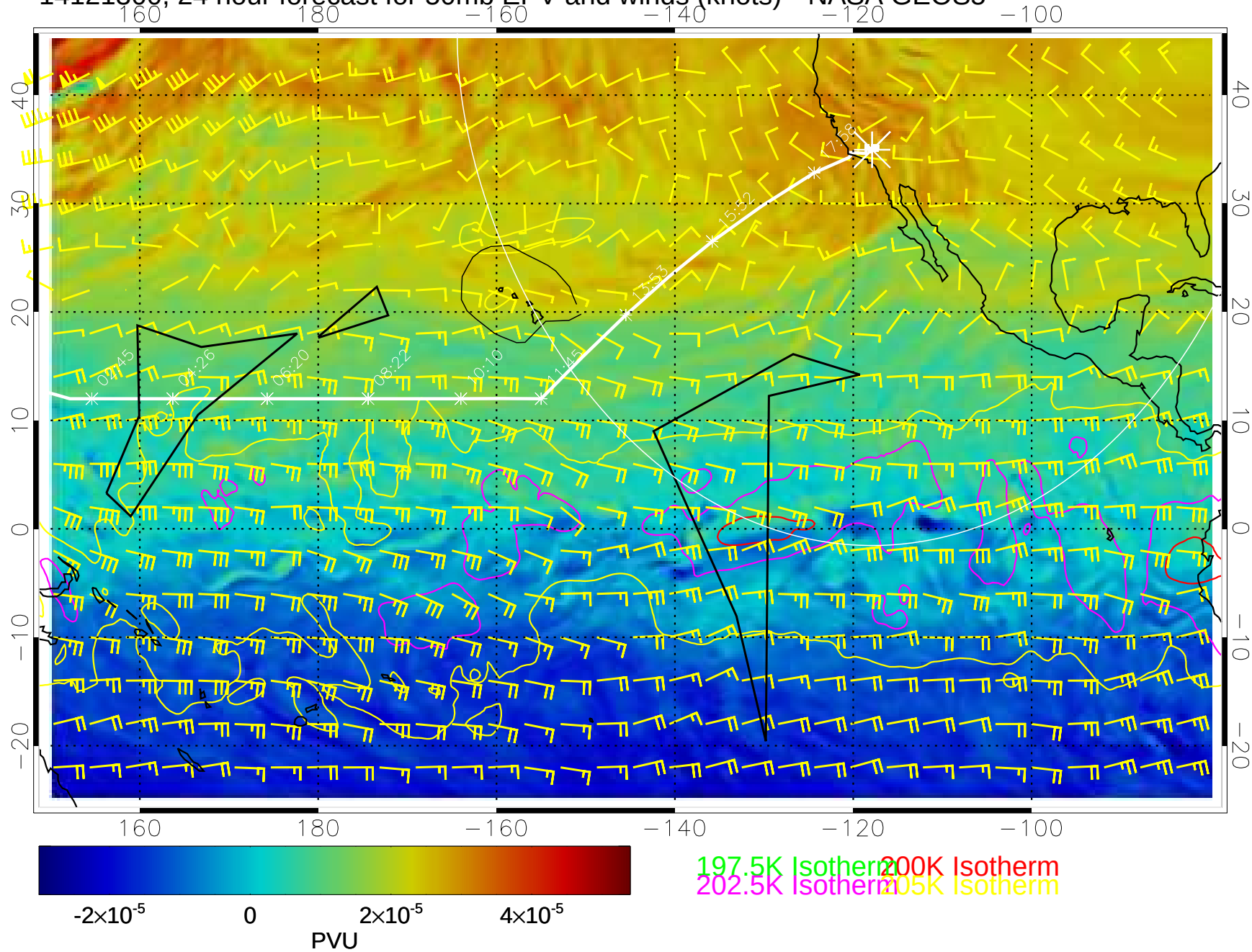
14121300, 24 hour forecast for 50mb EPV and winds (knots)-- NASA GEOS5
