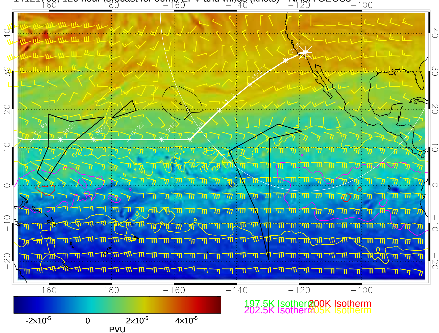
14121700, 120 hour forecast for 50mb EPV and winds (knots)-- NASA GEOS5
