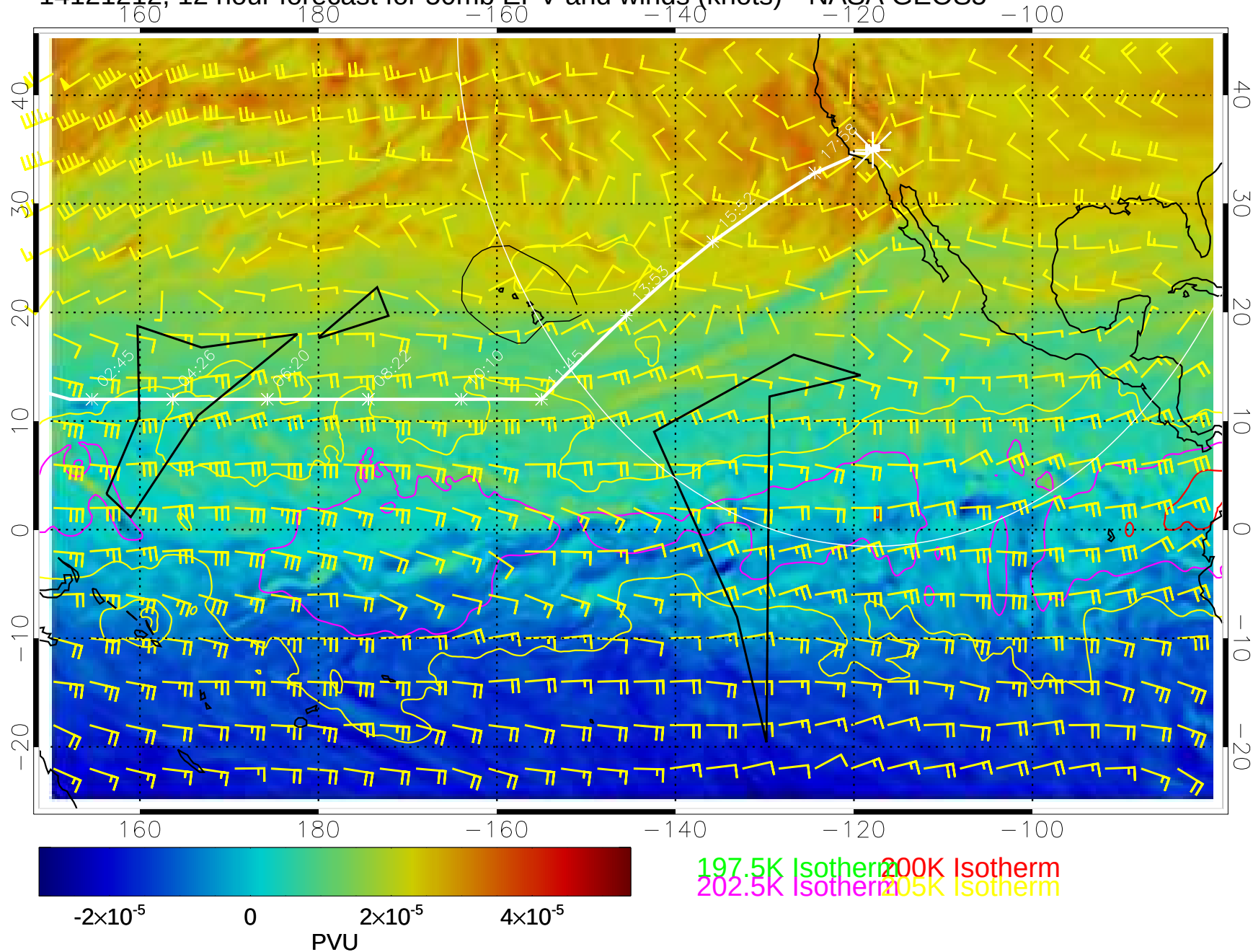
14121212, 12 hour forecast for 50mb EPV and winds (knots)-- NASA GEOS5
