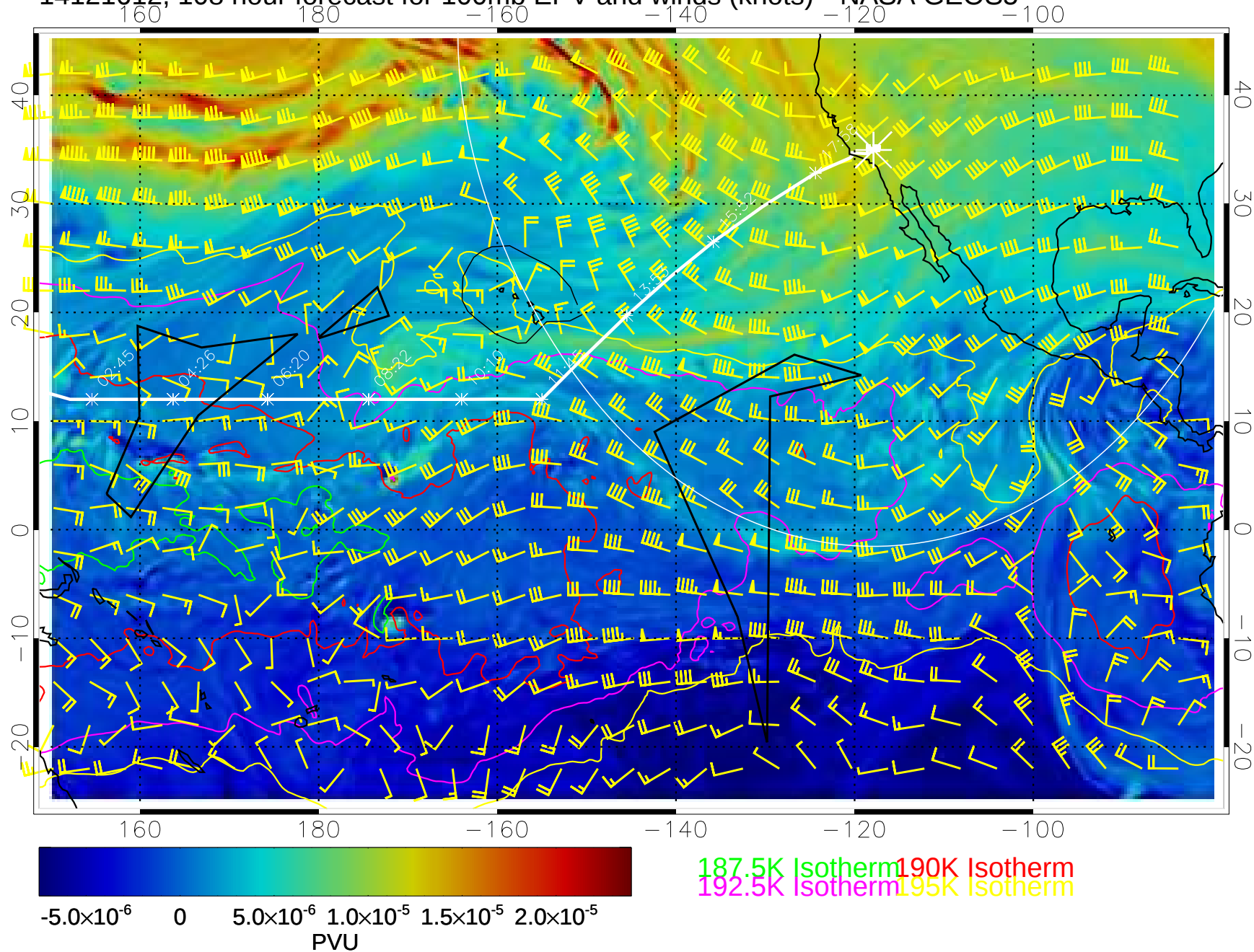
14121612, 108 hour forecast for 100mb EPV and winds (knots)-- NASA GEOS5
