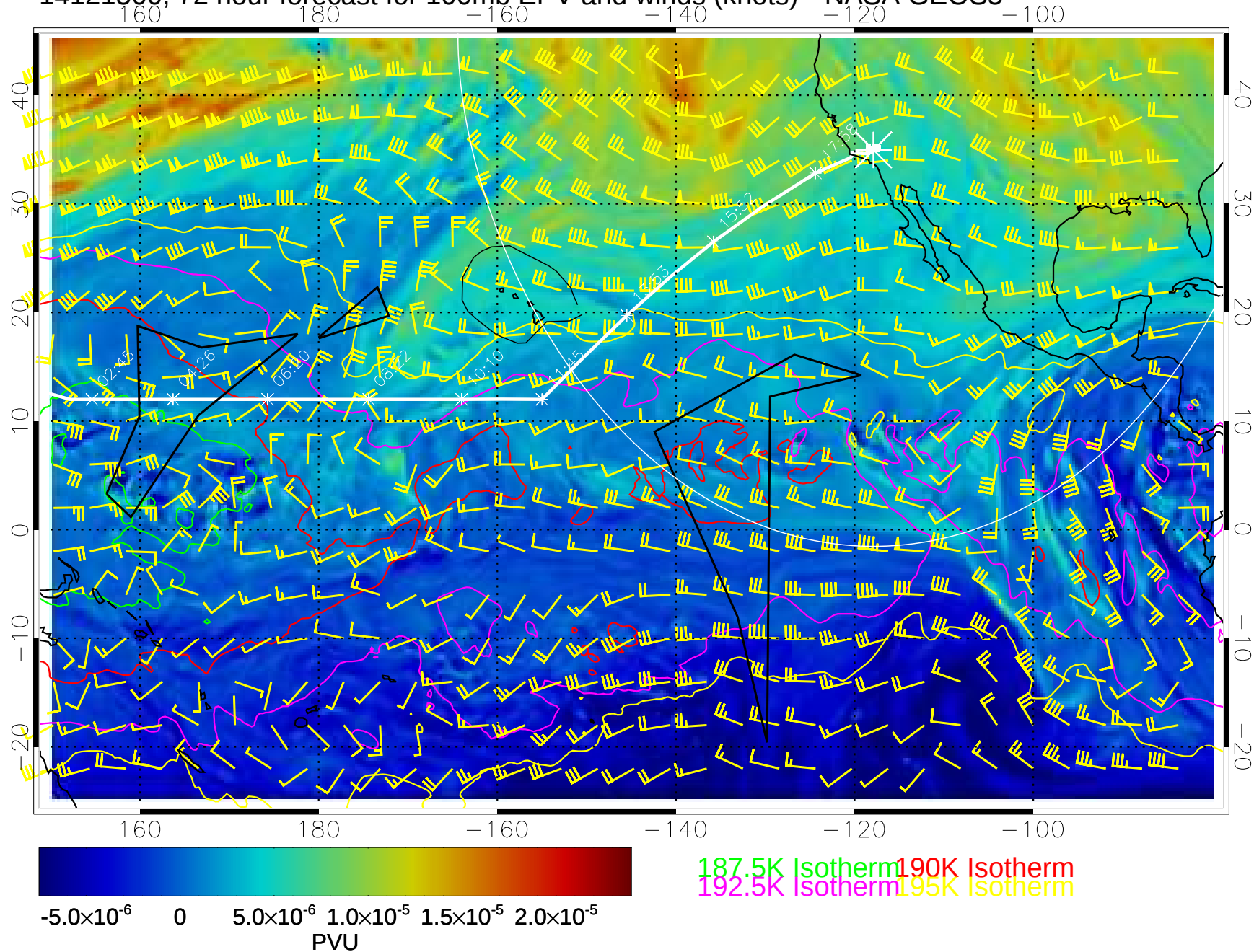
14121500, 72 hour forecast for 100mb EPV and winds (knots)-- NASA GEOS5
