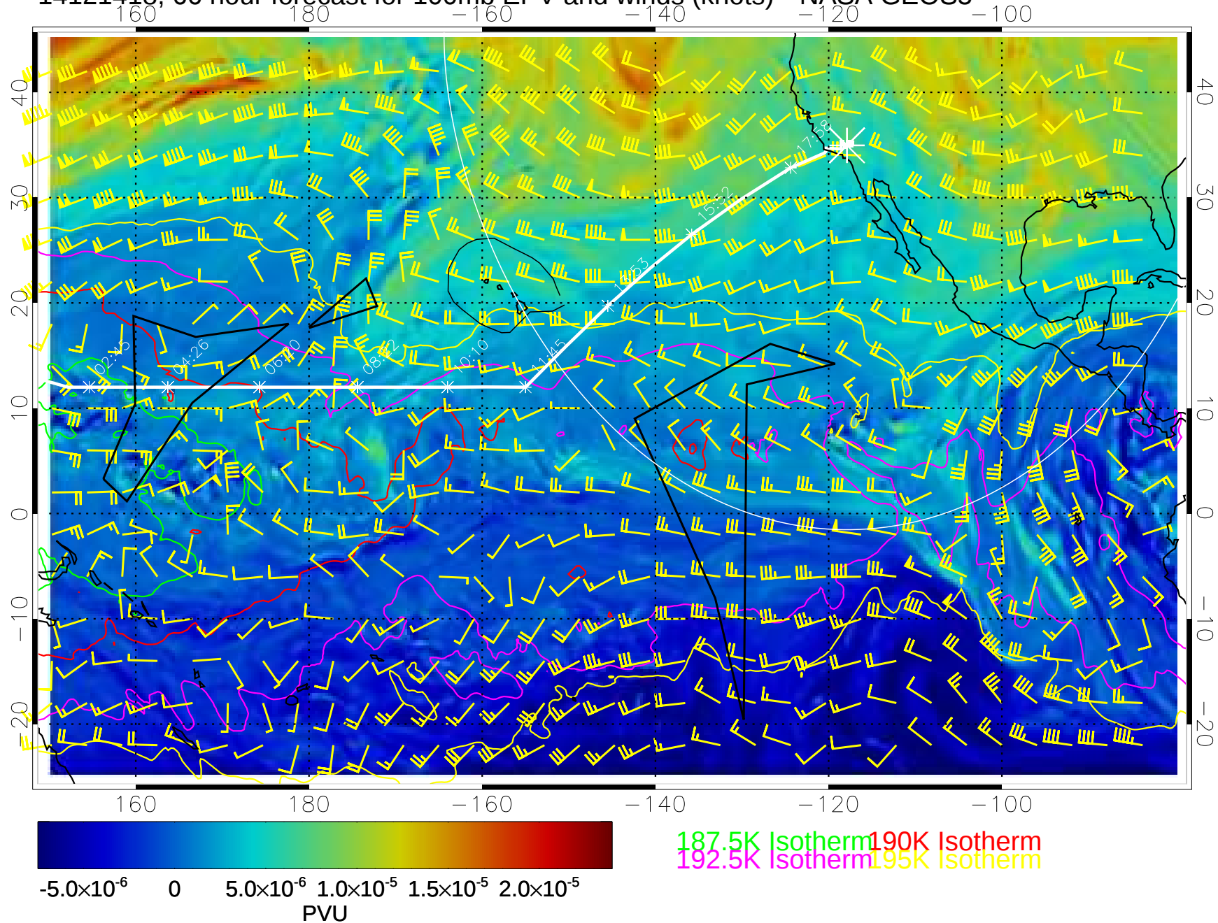
14121418, 66 hour forecast for 100mb EPV and winds (knots)-- NASA GEOS5
