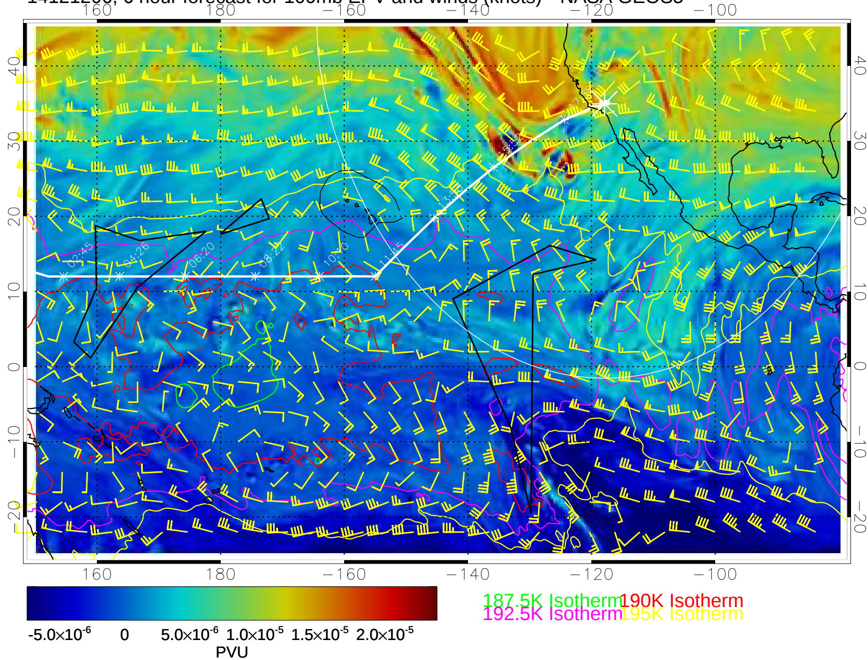
14121206, 6 hour forecast for 100mb EPV and winds (knots)-- NASA GEOS5
