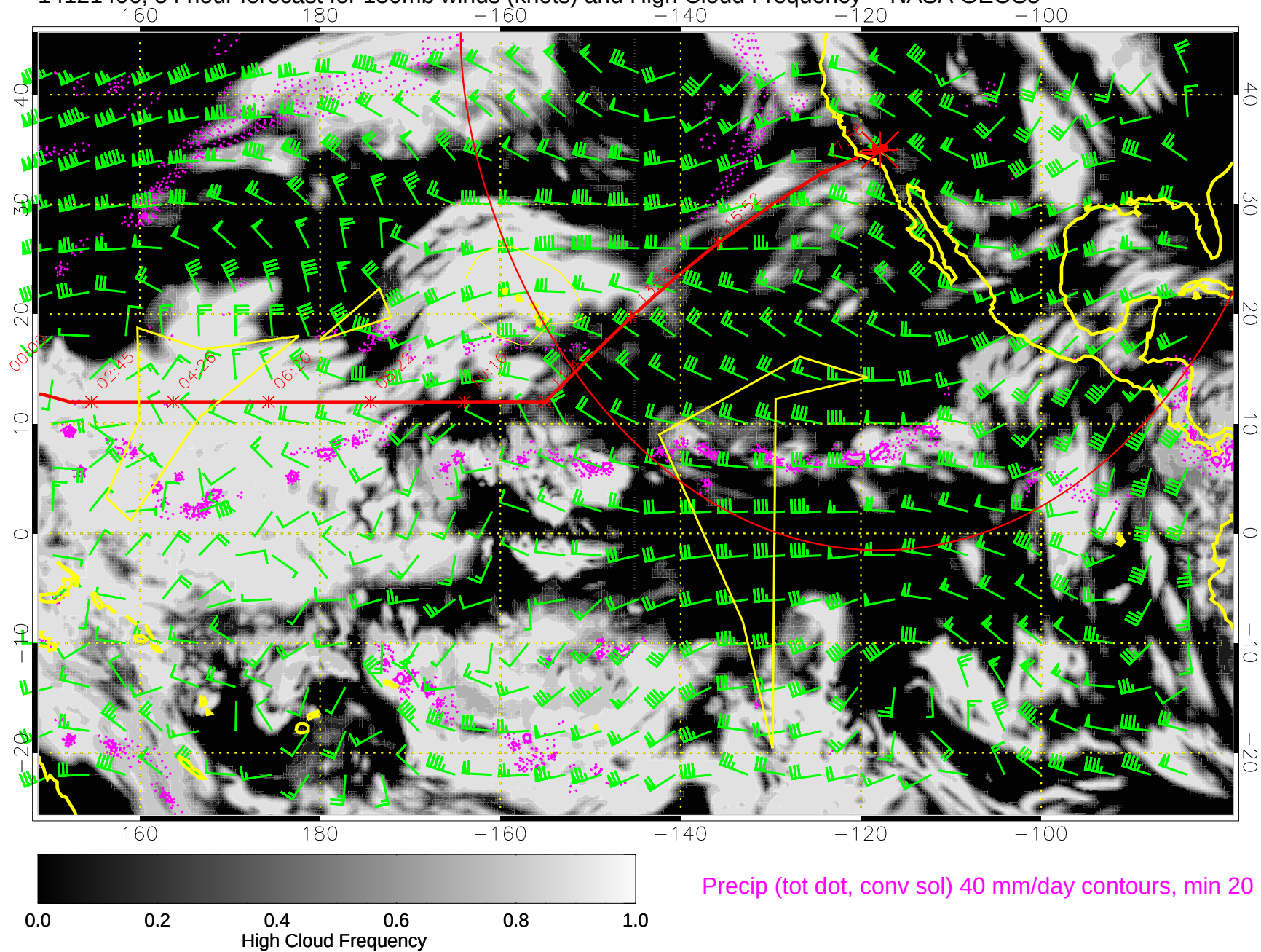
14121406, 54 hour forecast for 150mb winds (knots) and High Cloud Frequency -- NASA GEOS5
