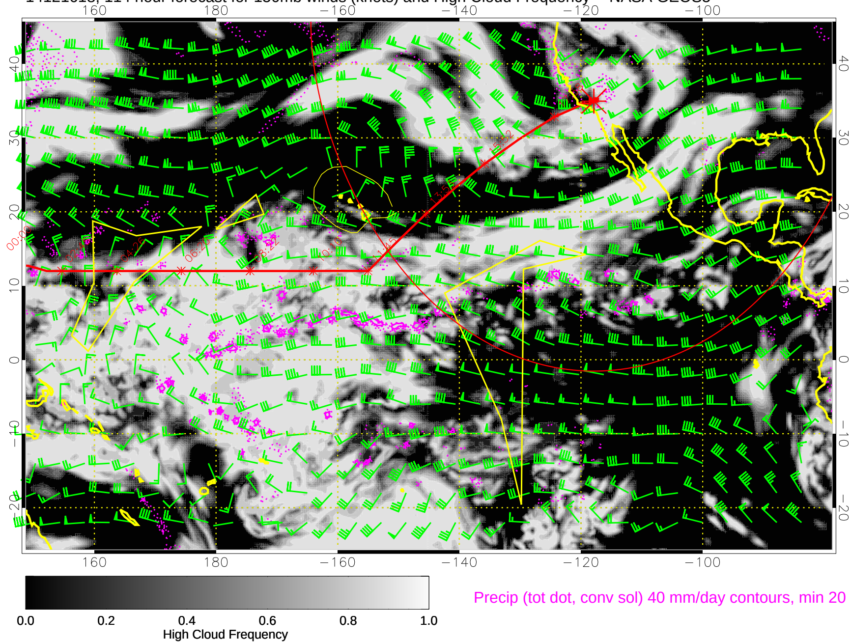
14121618, 114 hour forecast for 150mb winds (knots) and High Cloud Frequency -- NASA GEOS5
