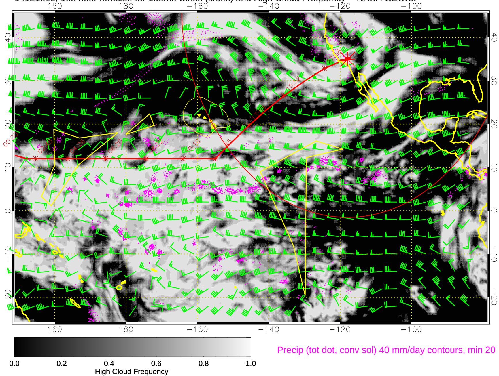
14121612, 108 hour forecast for 150mb winds (knots) and High Cloud Frequency -- NASA GEOS5
