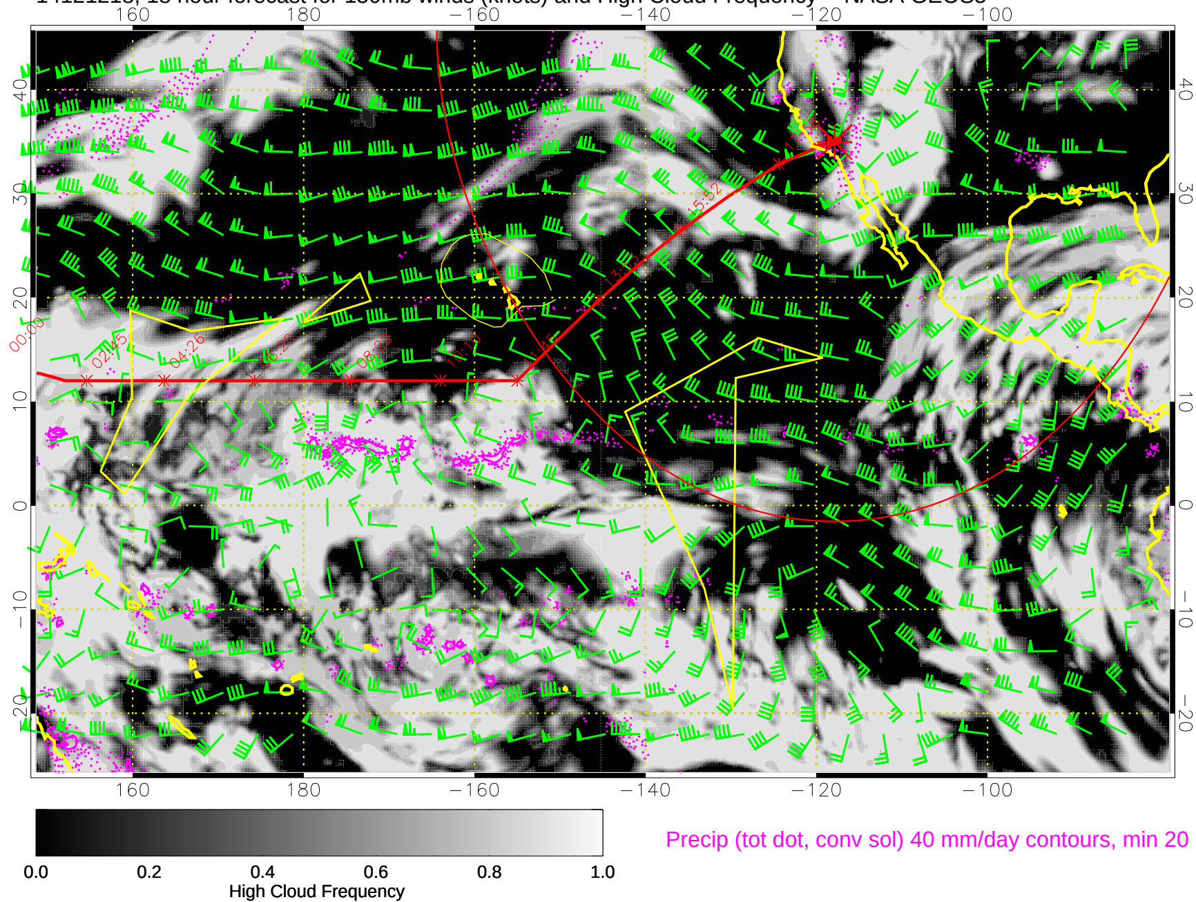
14121218, 18 hour forecast for 150mb winds (knots) and High Cloud Frequency -- NASA GEOS5
