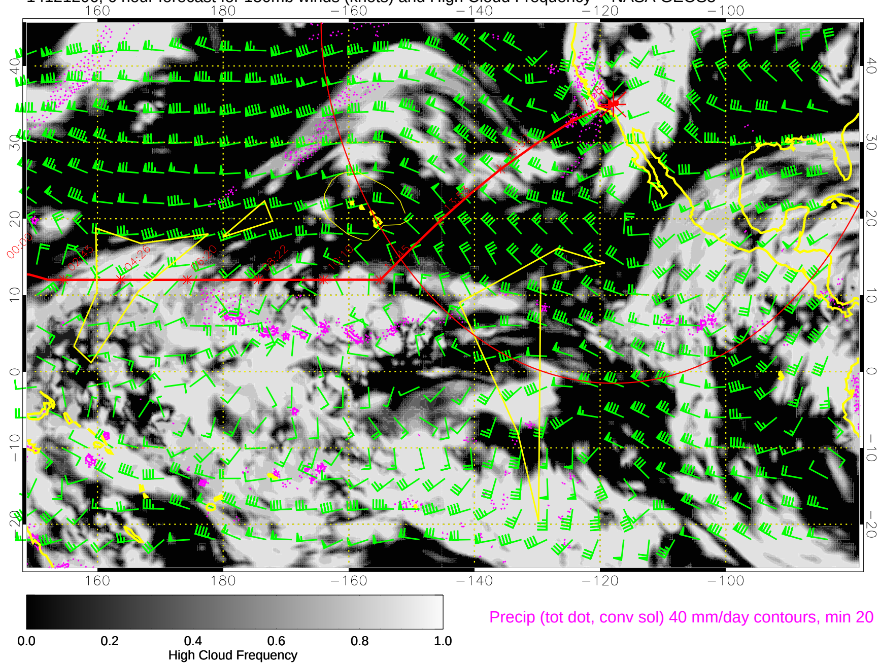
14121206, 6 hour forecast for 150mb winds (knots) and High Cloud Frequency -- NASA GEOS5
