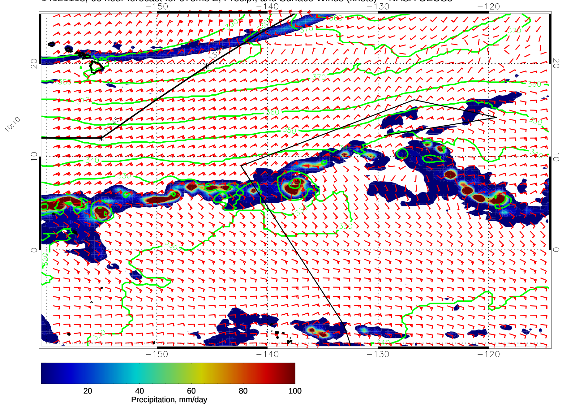
14121118, 66 hour forecast for 975mb Z, Precip., and Surface Winds (knots) -- NASA GEOS5
