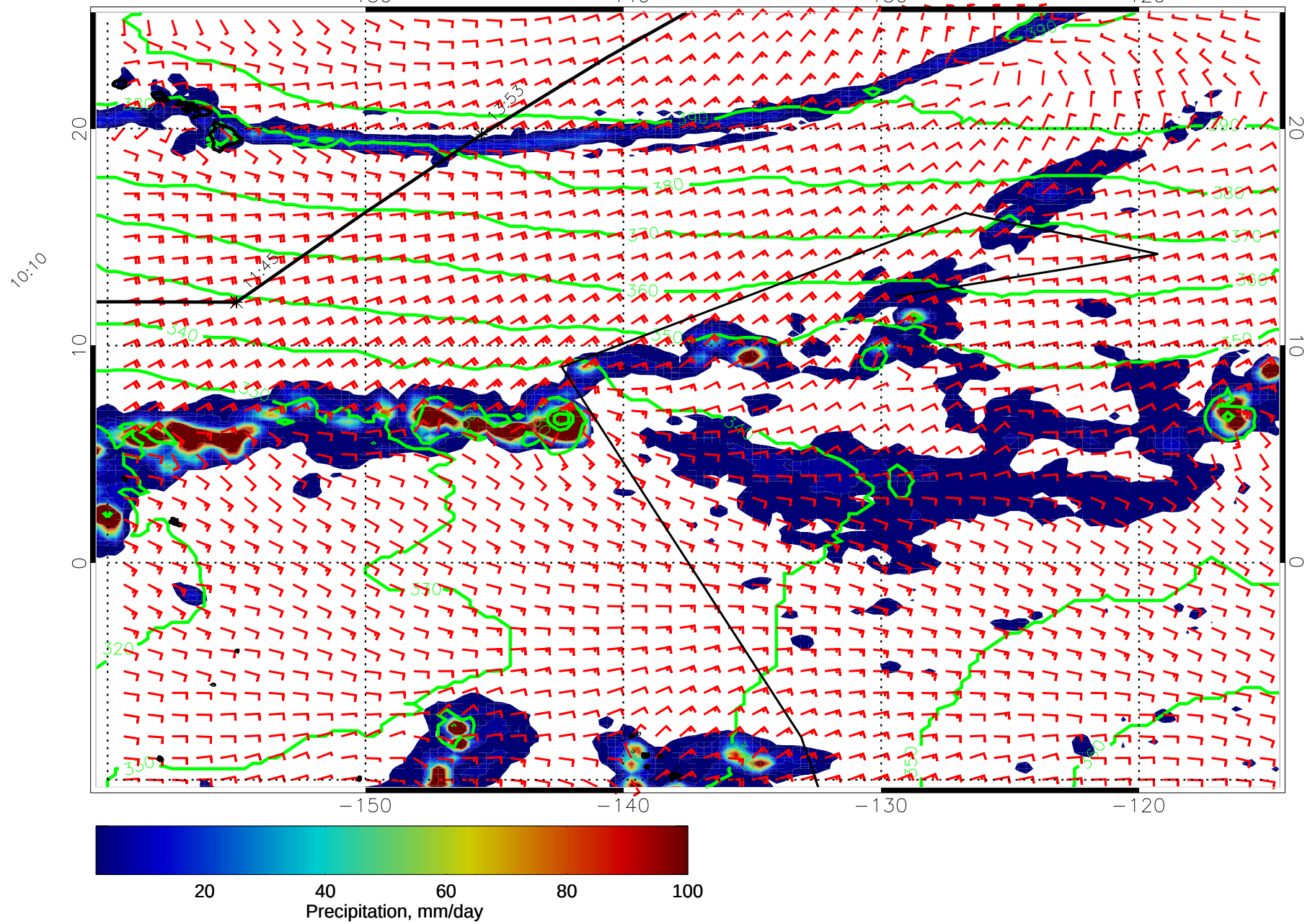
14121218, 90 hour forecast for 975mb Z, Precip., and Surface Winds (knots) -- NASA GEOS5
