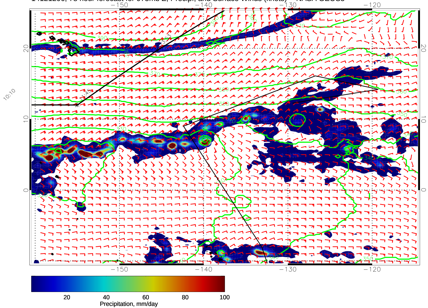
14121206, 78 hour forecast for 975mb Z, Precip., and Surface Winds (knots) -- NASA GEOS5
