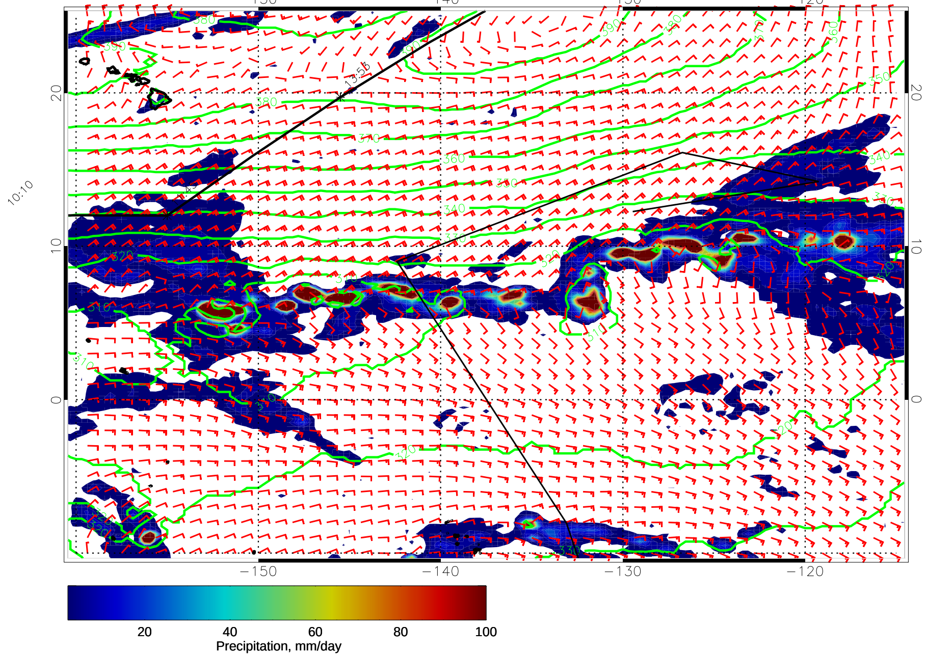
14121012, 36 hour forecast for 975mb Z, Precip., and Surface Winds (knots) -- NASA GEOS5
