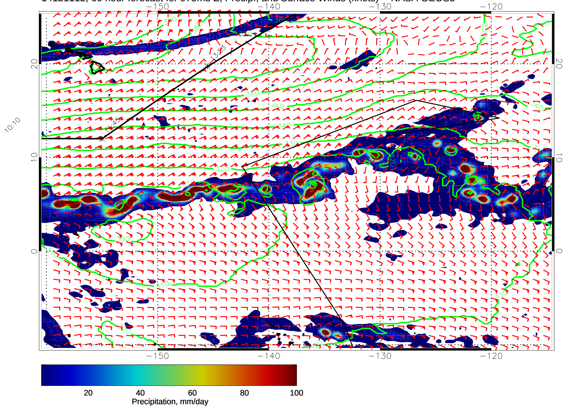
14121112, 60 hour forecast for 975mb Z, Precip., and Surface Winds (knots) -- NASA GEOS5
