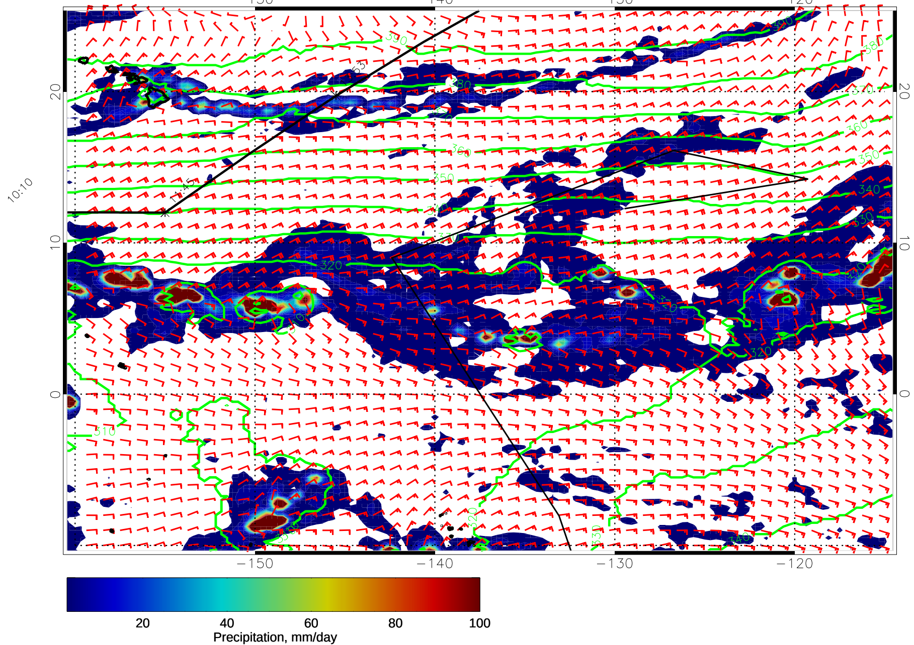
14121312, 108 hour forecast for 975mb Z, Precip., and Surface Winds (knots) -- NASA GEOS5
