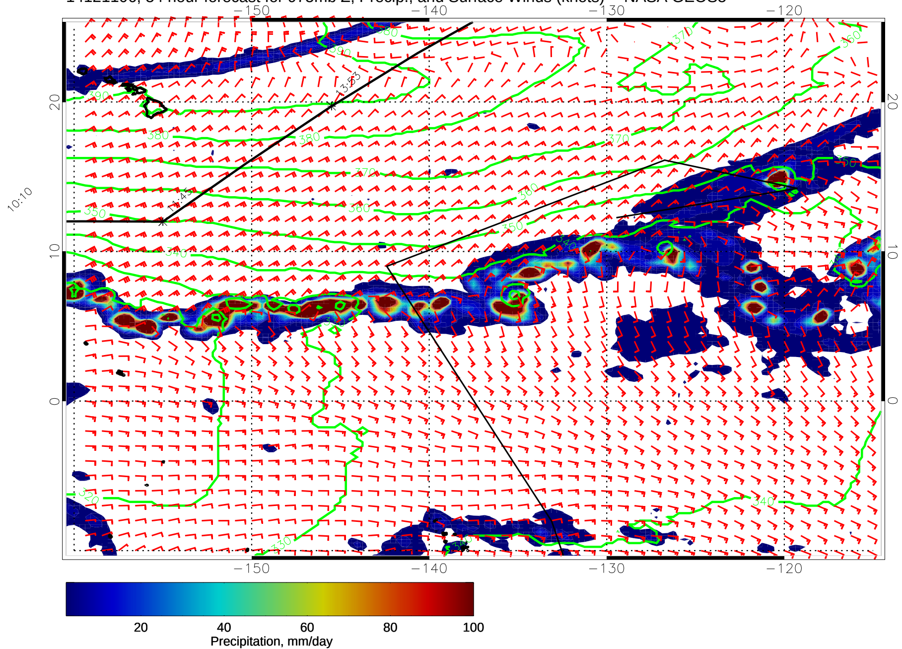
14121106, 54 hour forecast for 975mb Z, Precip., and Surface Winds (knots) -- NASA GEOS5
