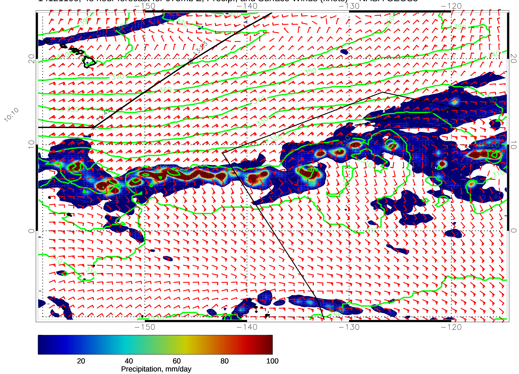
14121100, 48 hour forecast for 975mb Z, Precip., and Surface Winds (knots) -- NASA GEOS5
