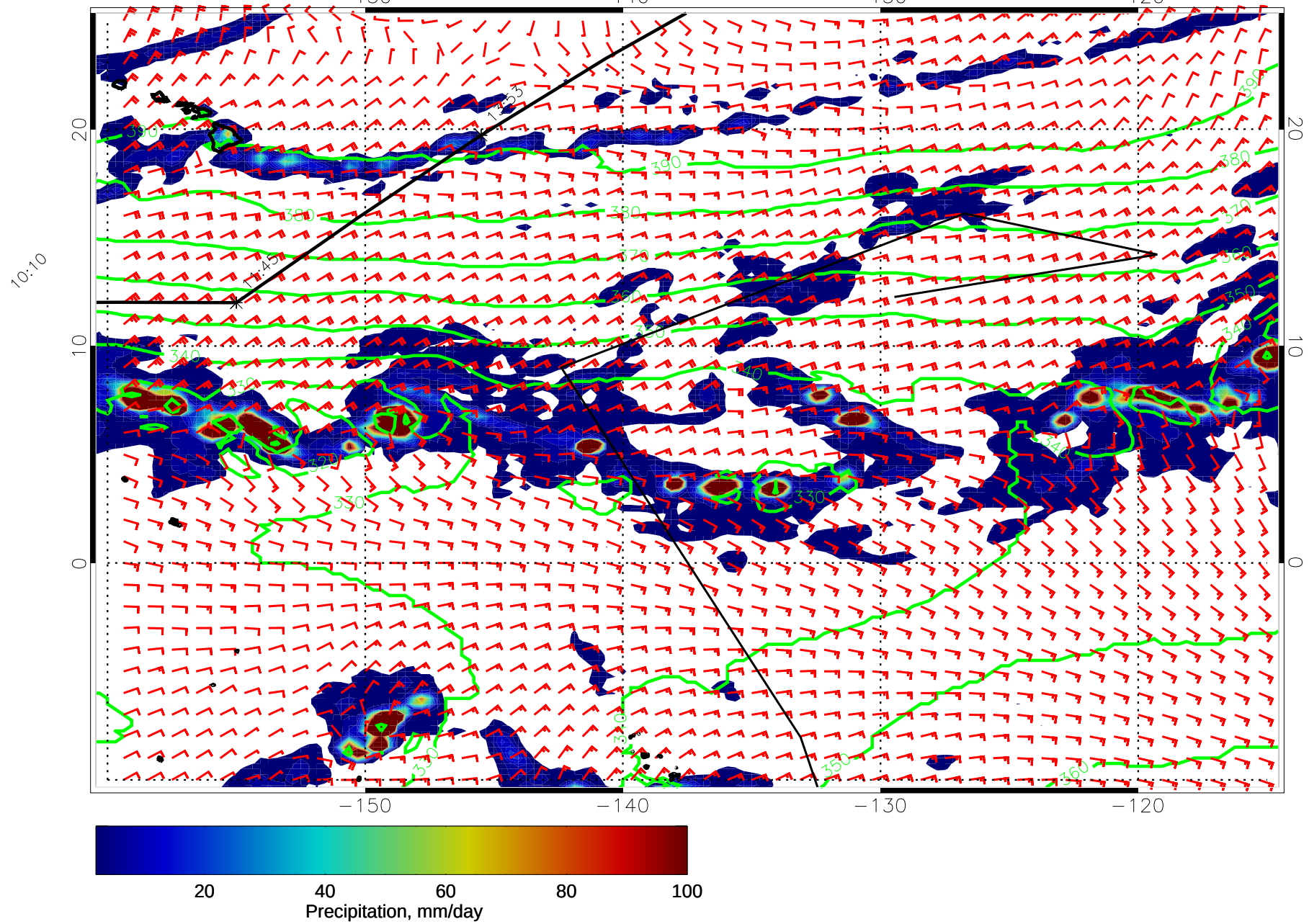
14121318, 114 hour forecast for 975mb Z, Precip., and Surface Winds (knots) -- NASA GEOS5
