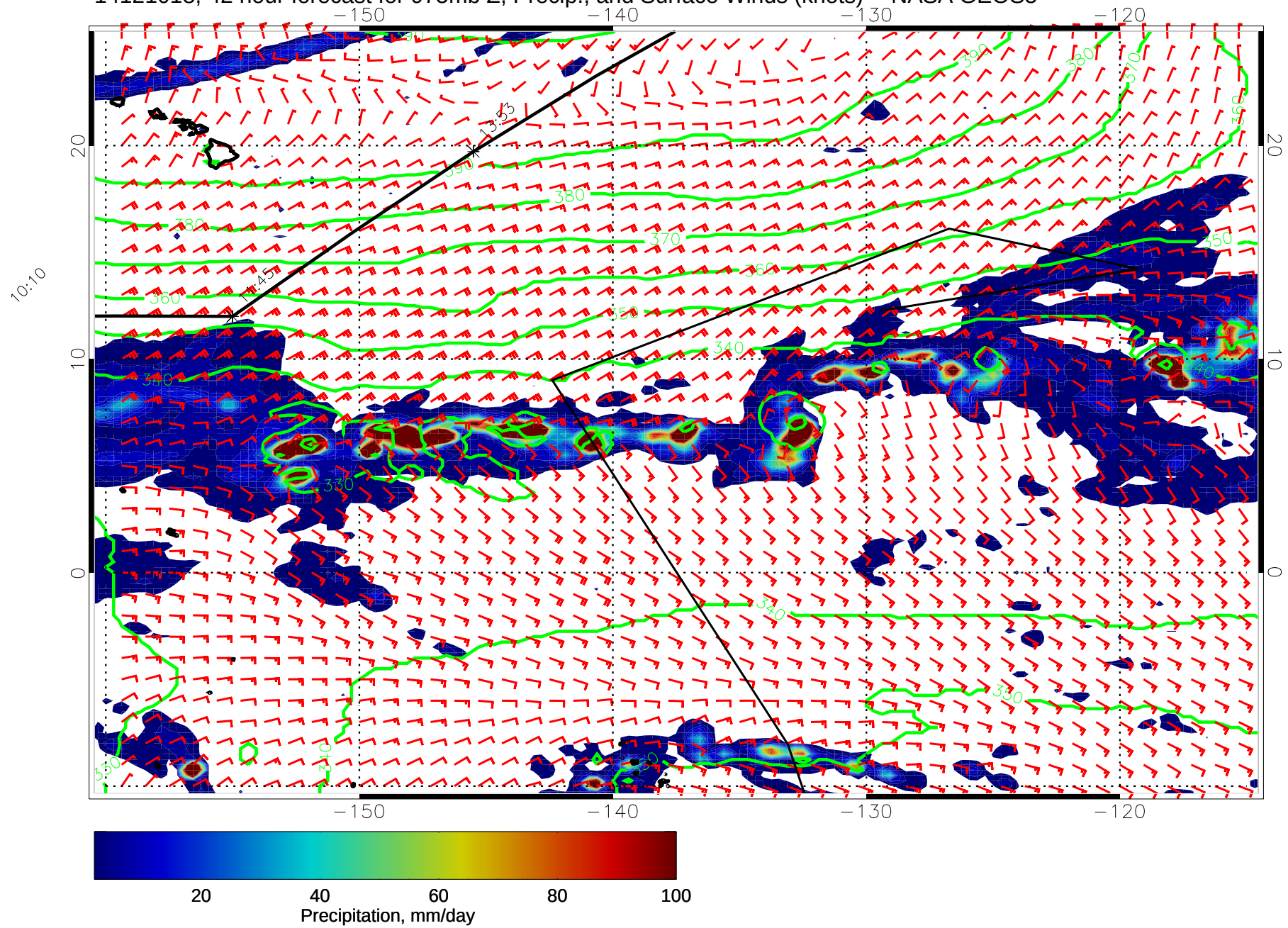
14121018, 42 hour forecast for 975mb Z, Precip., and Surface Winds (knots) -- NASA GEOS5
