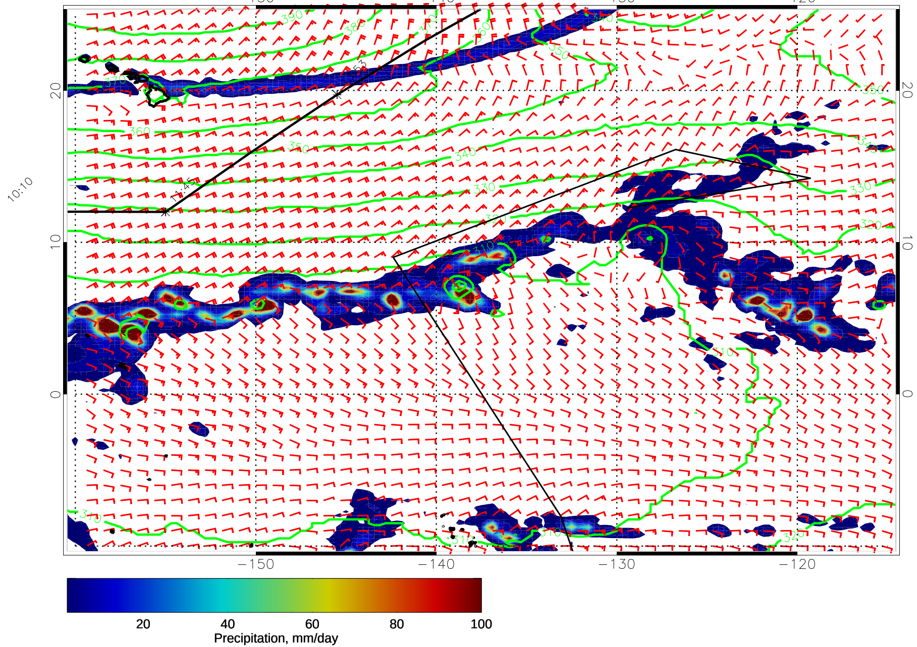
14121200, 72 hour forecast for 975mb Z, Precip., and Surface Winds (knots) -- NASA GEOS5
