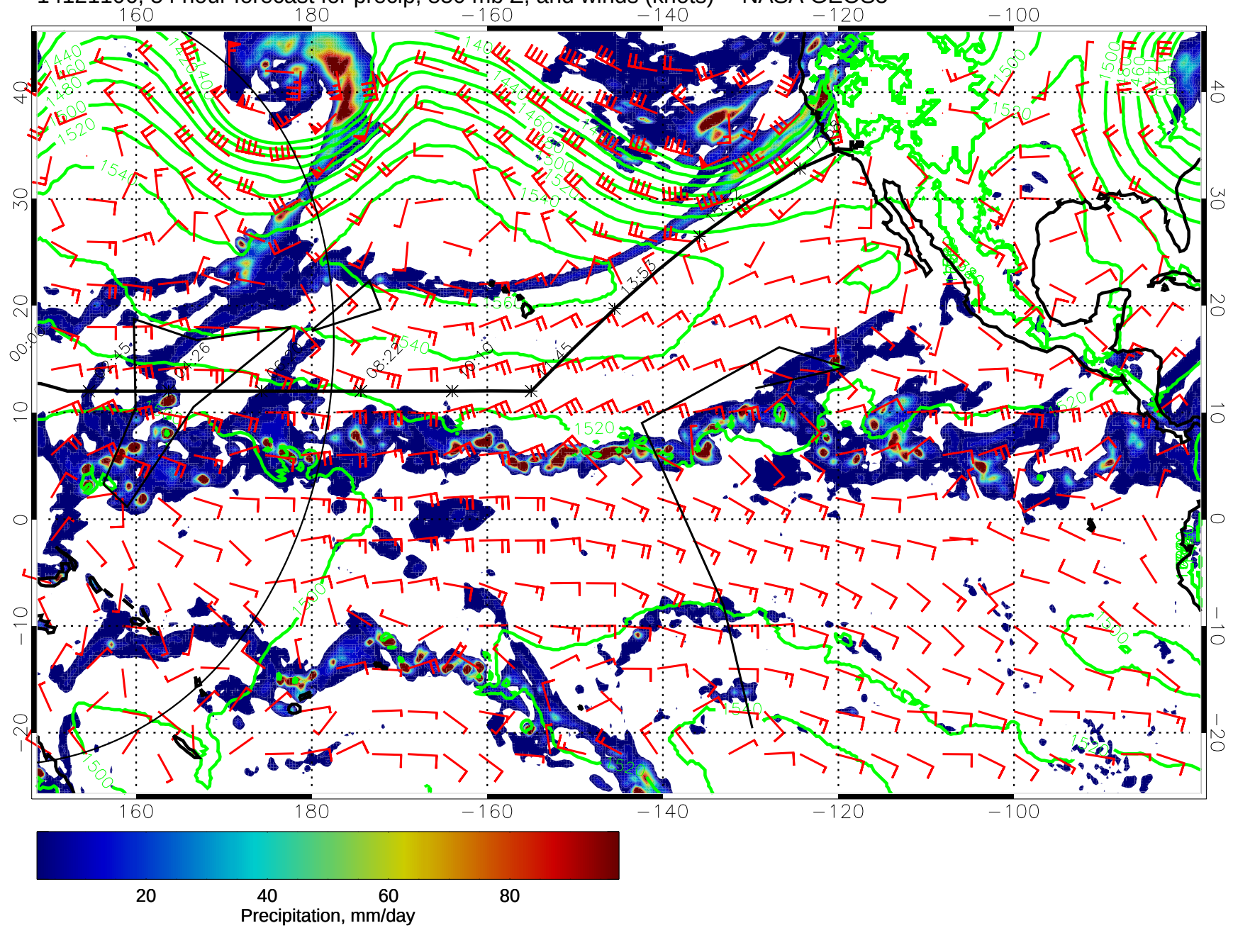
14121106, 54 hour forecast for precip, 850 mb Z, and winds (knots) -- NASA GEOS5
