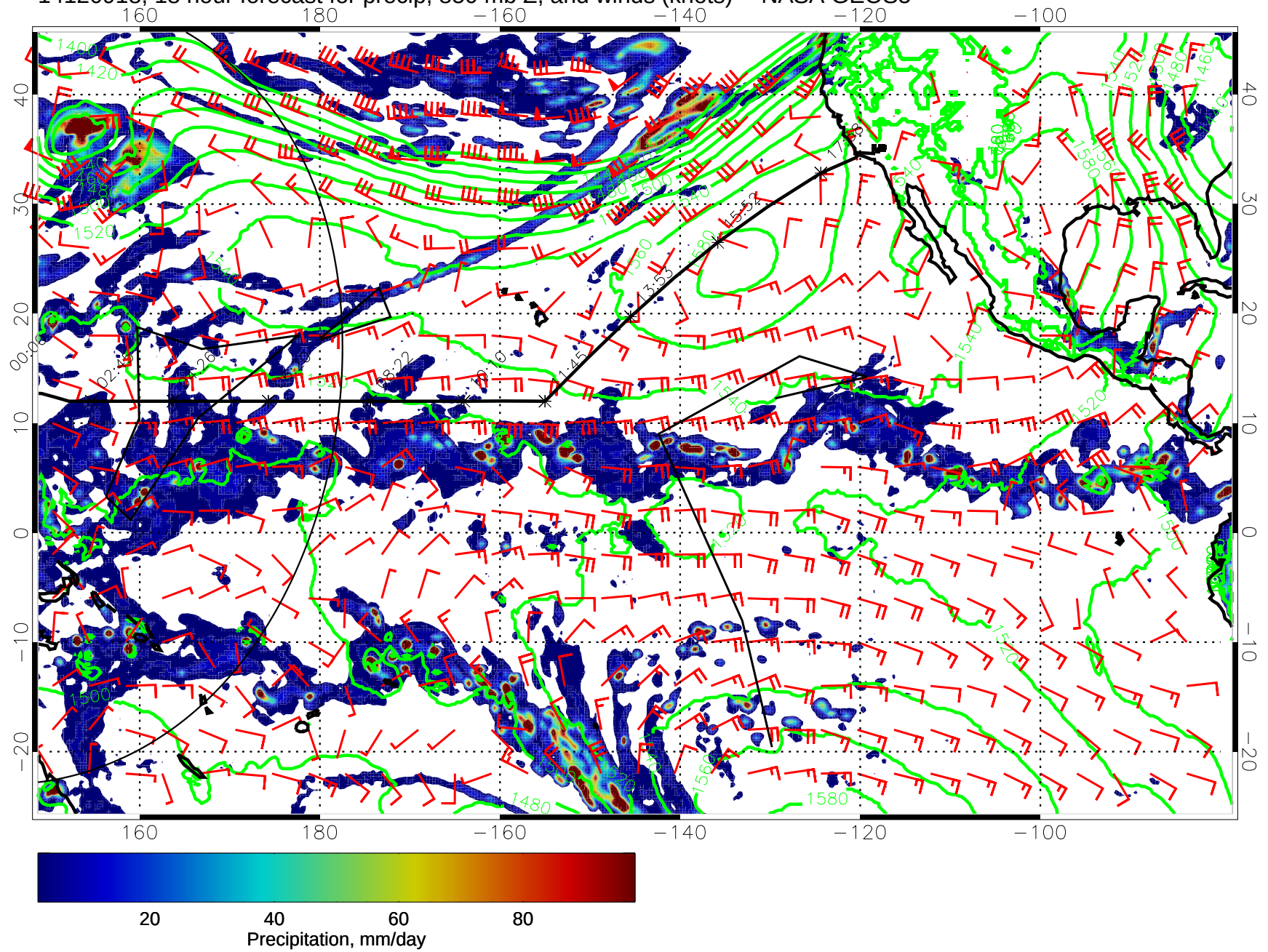
14120918, 18 hour forecast for precip, 850 mb Z, and winds (knots) -- NASA GEOS5
