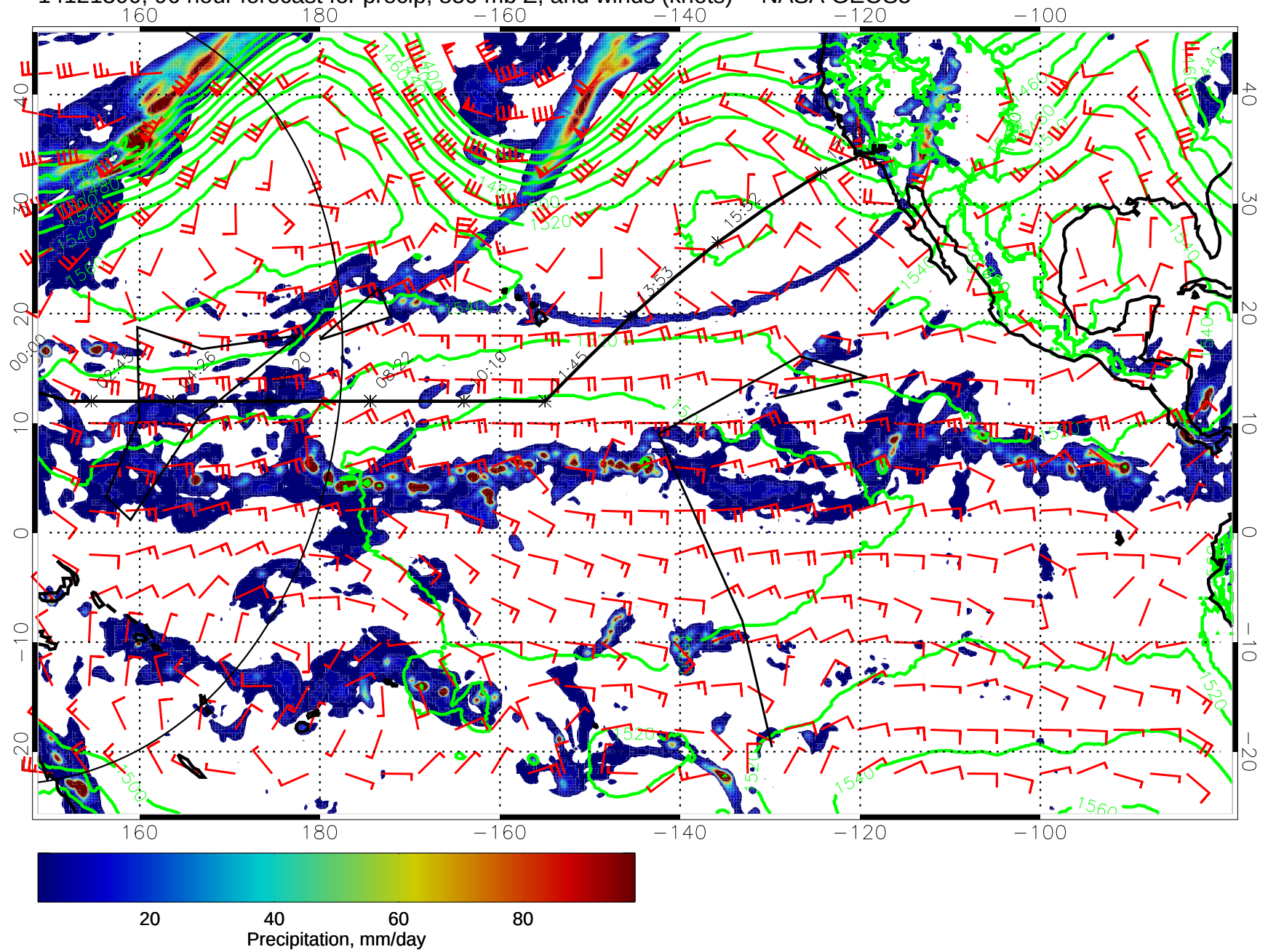
14121300, 96 hour forecast for precip, 850 mb Z, and winds (knots) -- NASA GEOS5
