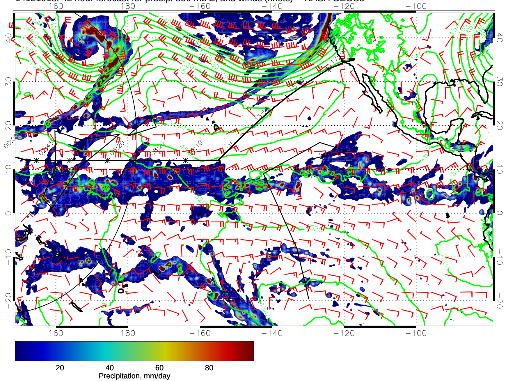
14121018, 42 hour forecast for precip, 850 mb Z, and winds (knots) -- NASA GEOS5
