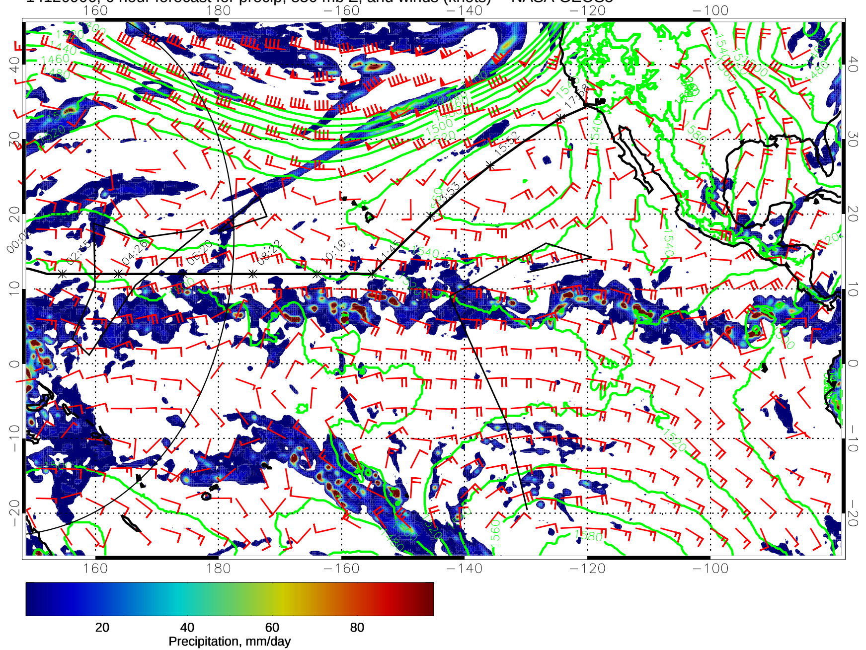
14120906, 6 hour forecast for precip, 850 mb Z, and winds (knots) -- NASA GEOS5
